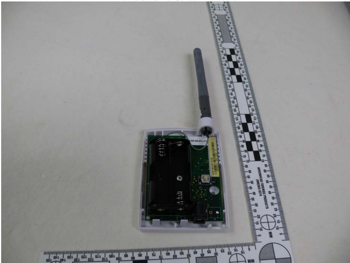
Sensor Board Front
