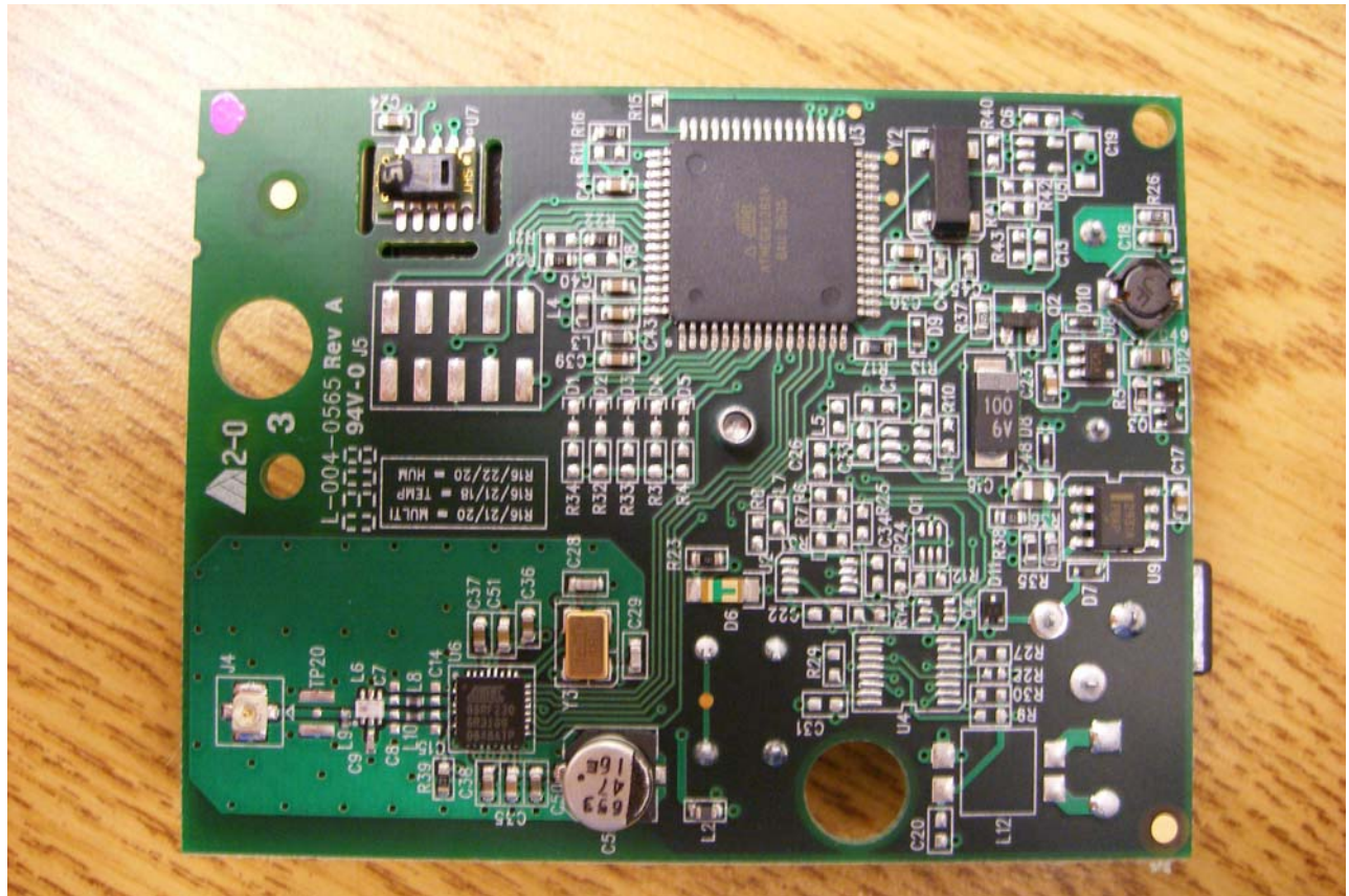
Winland Sensor – EA-WHS Back
