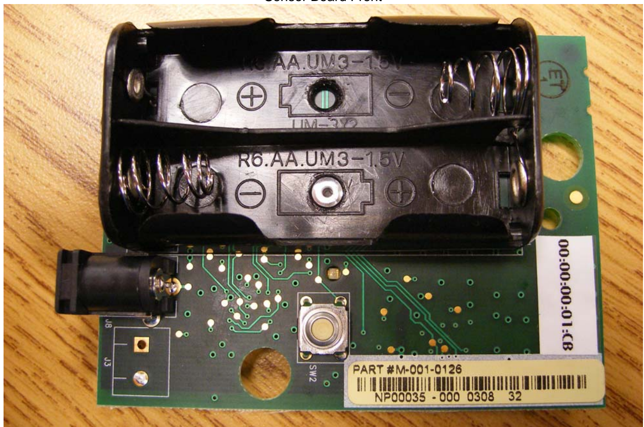
Sensor Board Front
