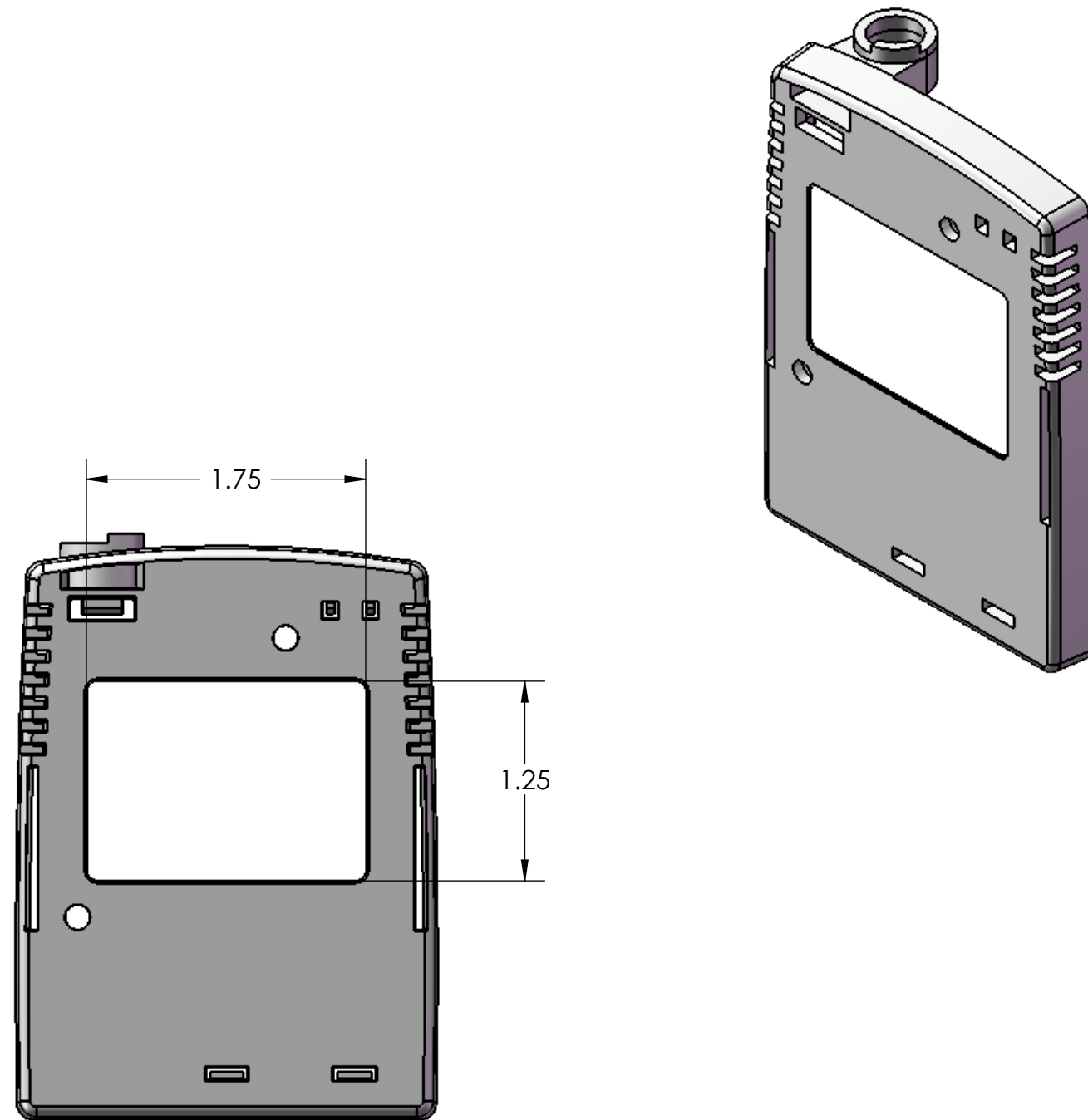
Wireless Sensor
