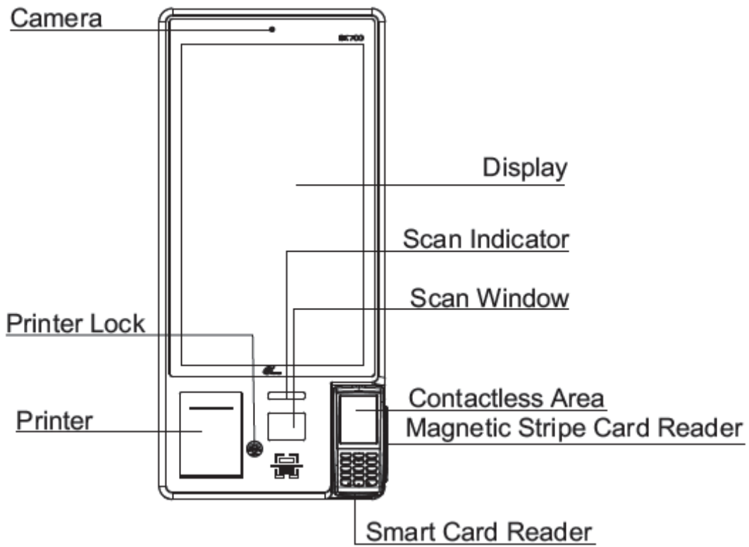
Front View
