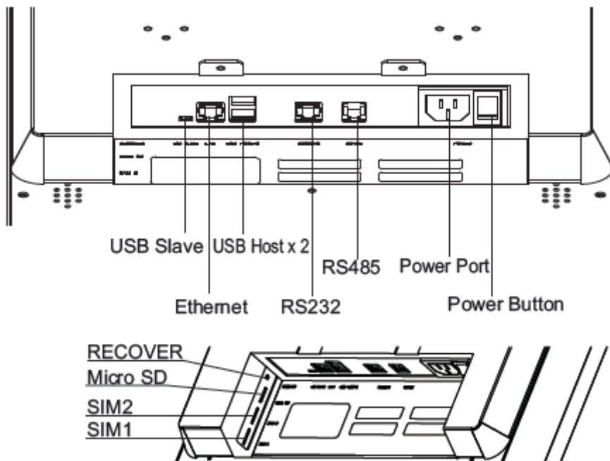
Interface Diagram
