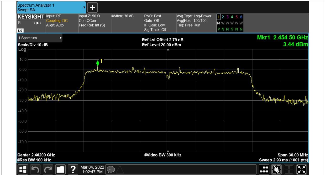
Band Edge NVNT n20 2462MHz Ant1 Emission
