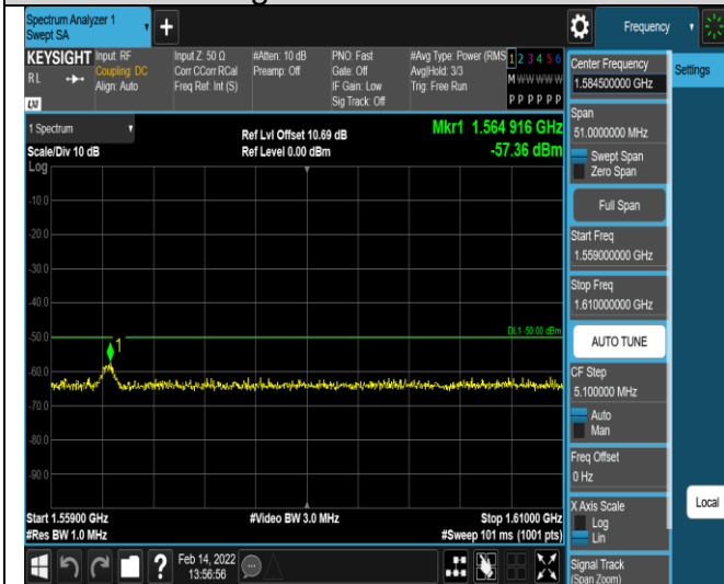
Band13-5MHz-16QAM-23205-1RB#0-
