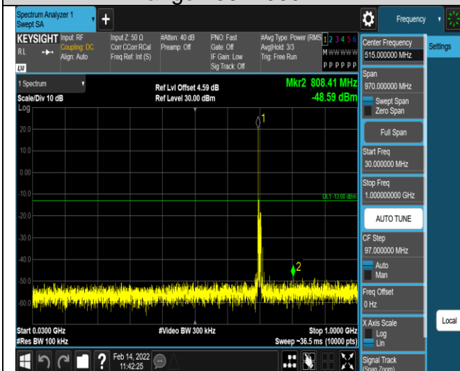
Band12-10MHz-QPSK-23130-1RB#0- Range1:30~1000MHz
