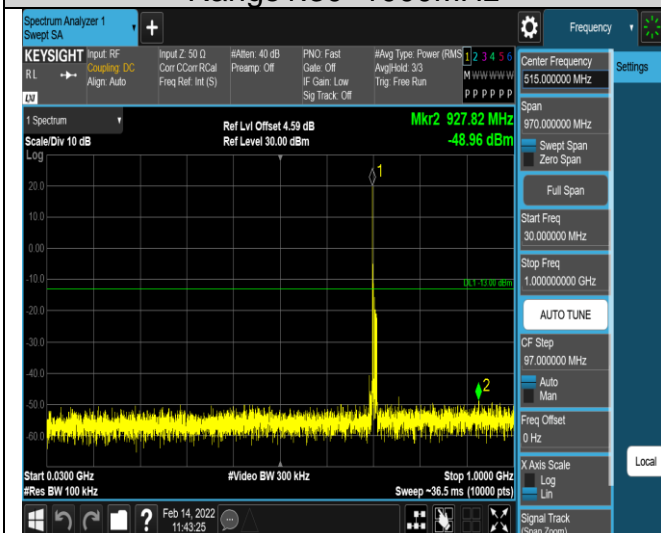
Band12-10MHz-16QAM-23060-1RB#0-
