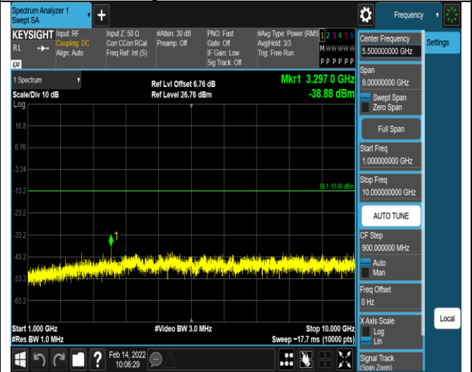
Band5-1.4MHz-QPSK-20525-1RB#0- Range2:1000~10000MHz
