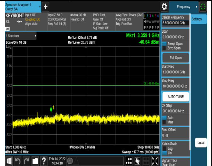
Band5-10MHz-16QAM-20450-1RB#0- Range2:1000~10000MHz
