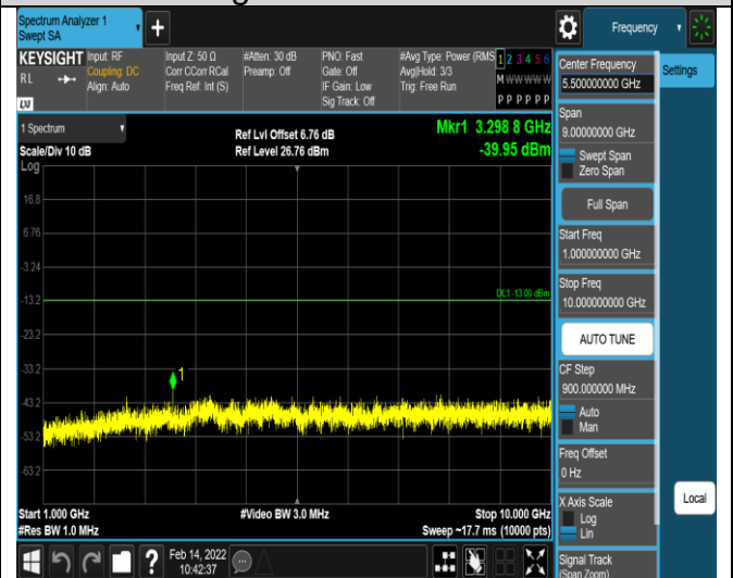
Band5-10MHz-16QAM-20525-1RB#0- Range2:1000~10000MHz
