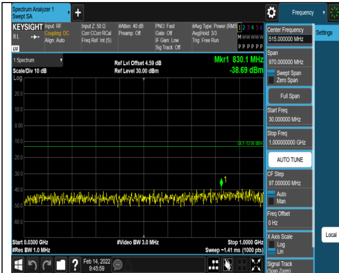
Band4-20MHz-QPSK-20175-1RB#0- Range1:30~1000MHz
