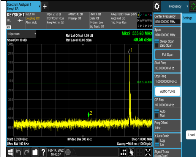
Band5-10MHz-16QAM-20450-1RB#0- Range1:30~1000MHz
