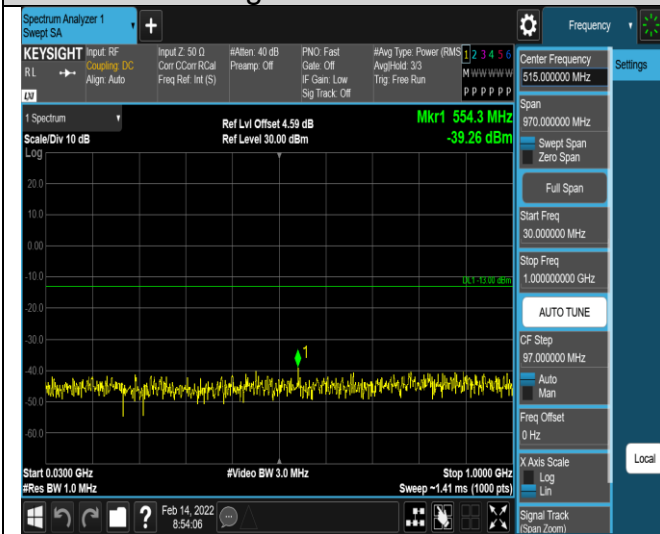
Band4-20MHz-QPSK-20050-1RB#0- Range1:30~1000MHz
