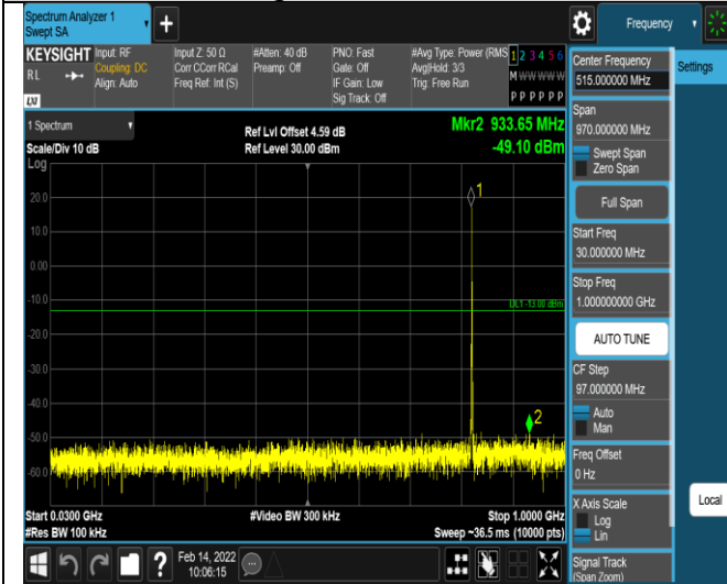
Band5-1.4MHz-QPSK-20525-1RB#0- Range1:30~1000MHz
