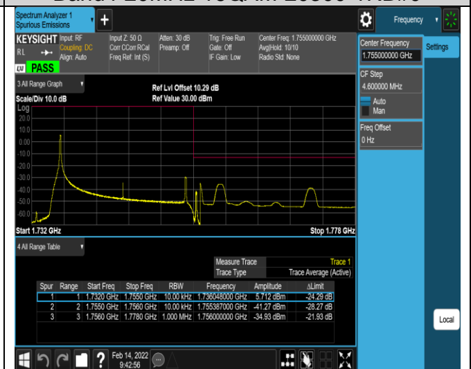
Band4-20MHz-16QAM-20300-100RB#0
