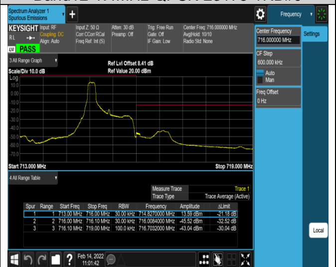
Band12-1.4MHz-QPSK-23173-6RB#0
