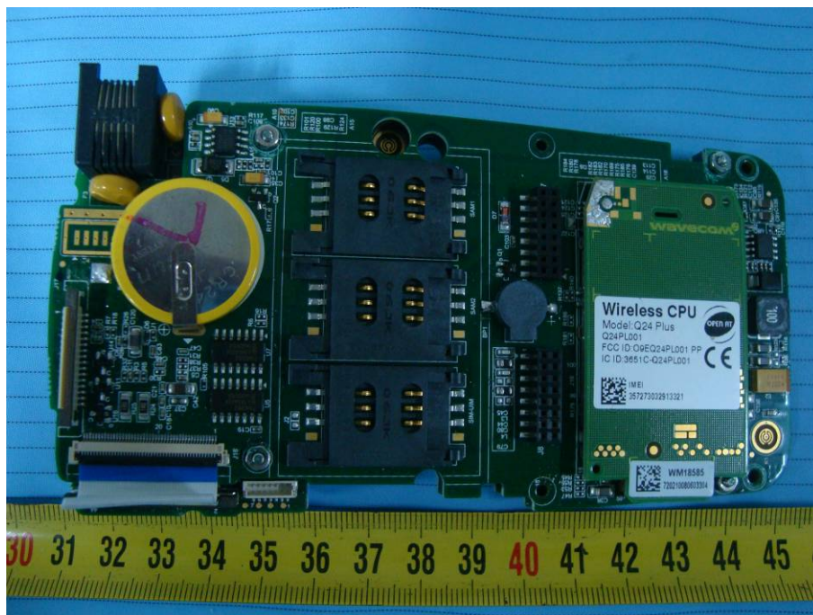
EUT –Main Board without Power Board Front View
