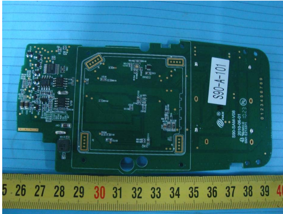
EUT – Main Board with Card Slots Rear View
