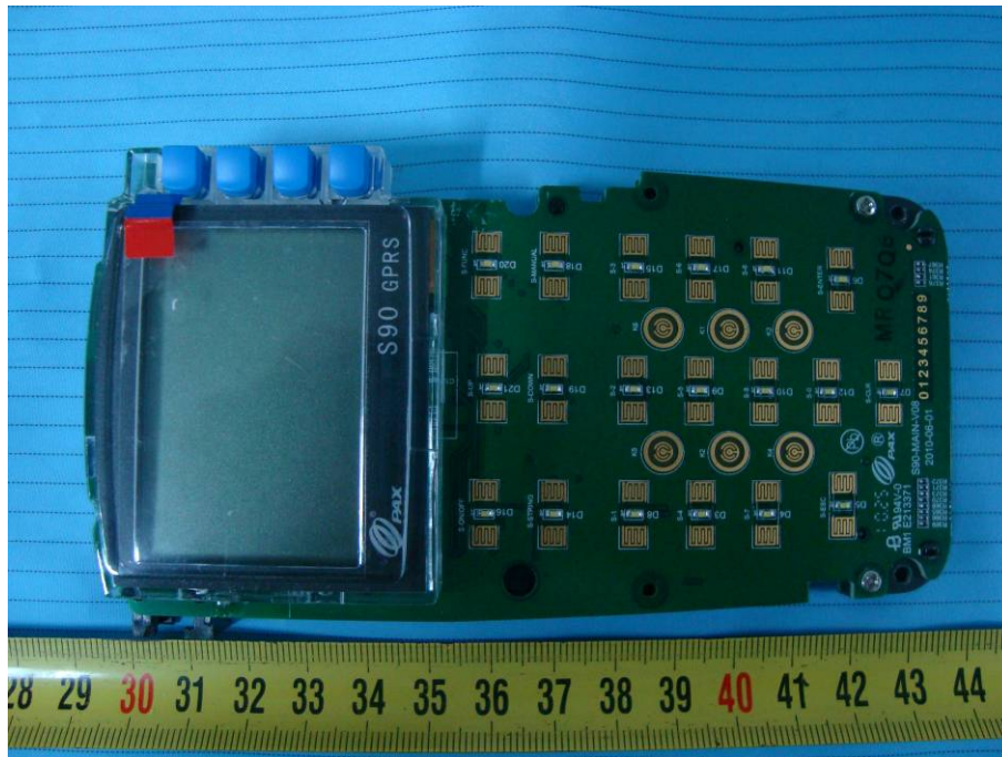
EUT – Main Board with LCD Front View
