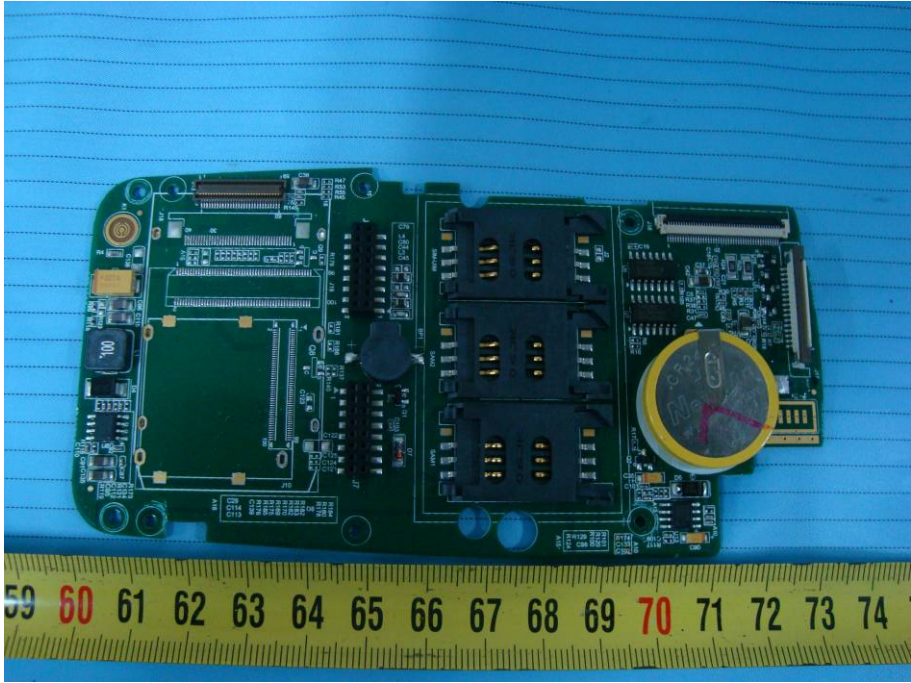
EUT – Main Board with Card Slots Front View
