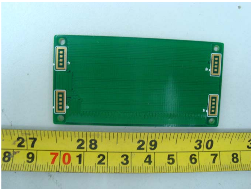
EUT – S80-MESH Top View
