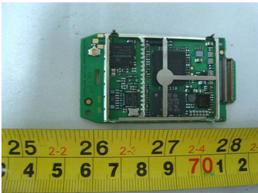
EUT – RF Module without Shielding View
