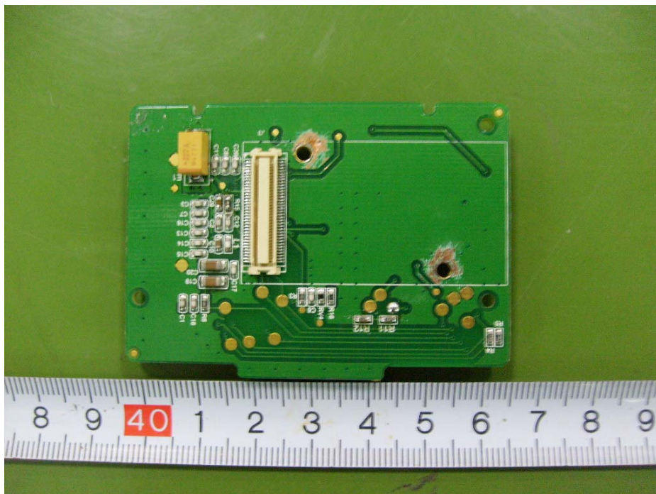
EUT – Board P90-G24-V07 Bottom View
