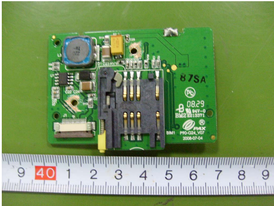
EUT – Board P90-G24-V07 Top View
