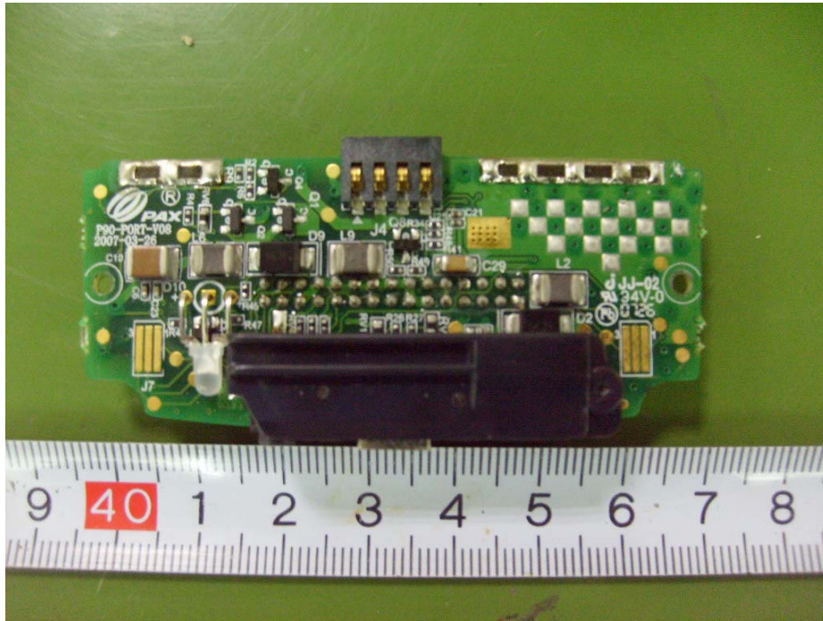
EUT – Board P90-port-Vo8 Top View
