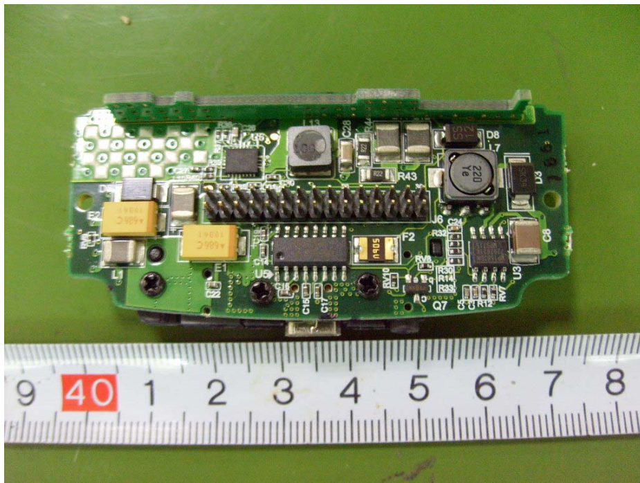
EUT – Board P90-port-Vo8 Bottom View
