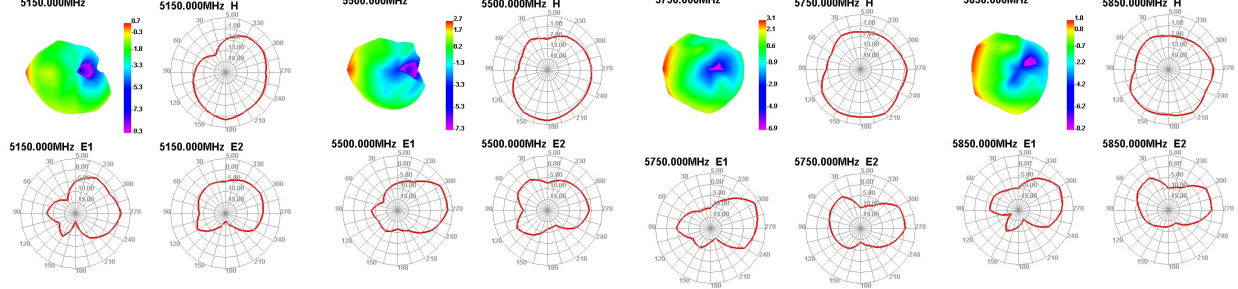
Wifi antenna
