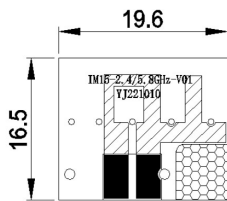
Wifi antenna
