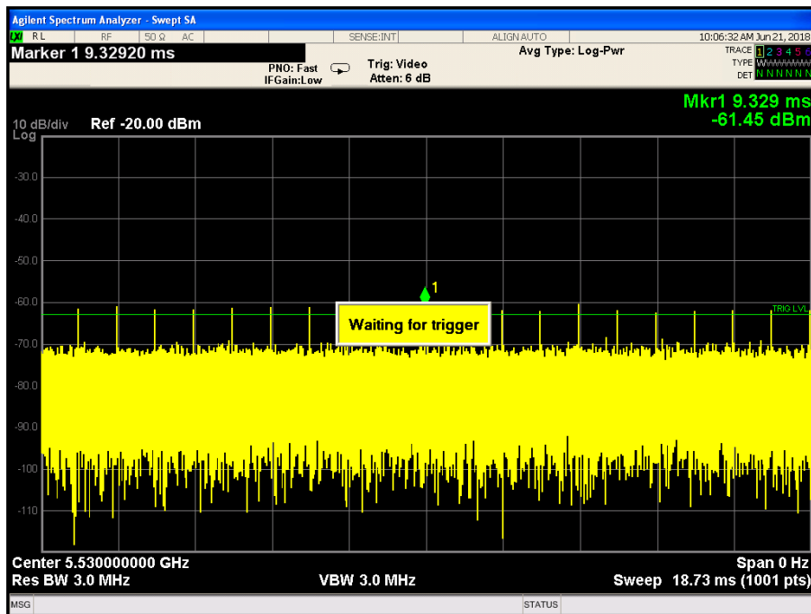
5530-Radar signal
