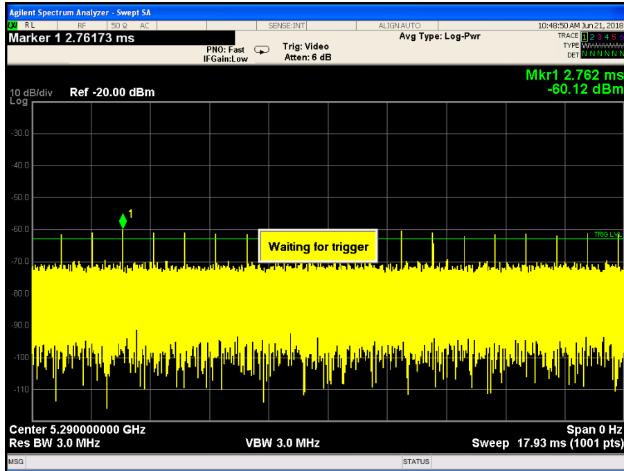
5290-Radar signal
