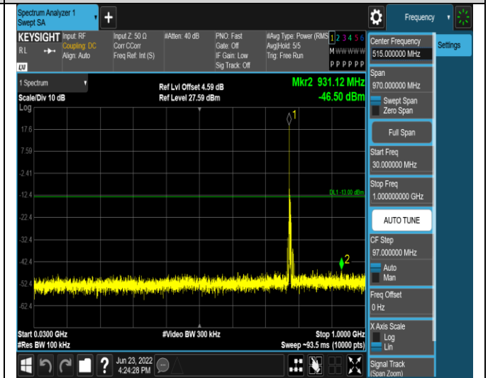
Band13-5MHz-16QAM-23205-1RB#0-
