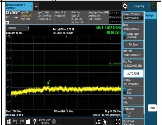
Band17-10MHz-QPSK-23800-1RB#0- Range2:1000~10000MHz
