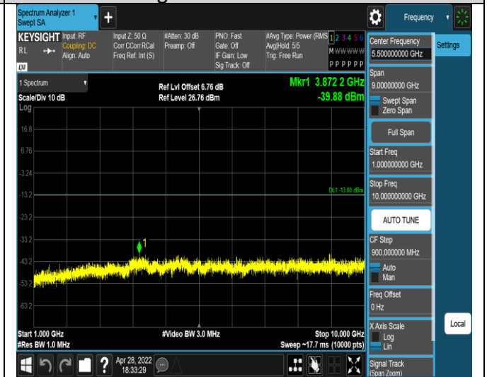
Band17-10MHz-16QAM-23780-1RB#0-
