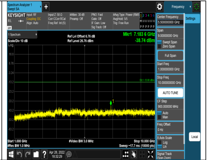
Band17-10MHz-QPSK-23790-1RB#0- Range2:1000~10000MHz
