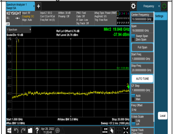
Band4-20MHz-16QAM-20050-1RB#0-
