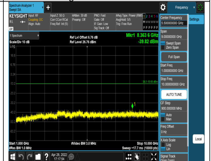
Band12-10MHz-16QAM-23060-1RB#0-
