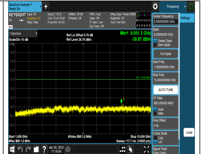
Band12-10MHz-QPSK-23095-1RB#0- Range2:1000~10000MHz
