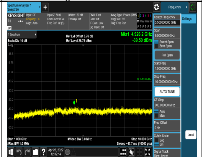
Band12-1.4MHz-QPSK-23095-1RB#0- Range2:1000~10000MHz
