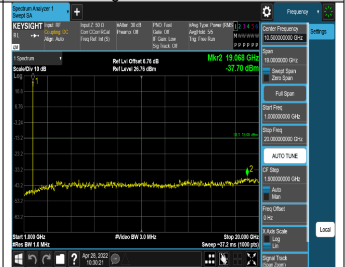
Band4-1.4MHz-16QAM-20393-1RB#0- Range2:1000~20000MHz
