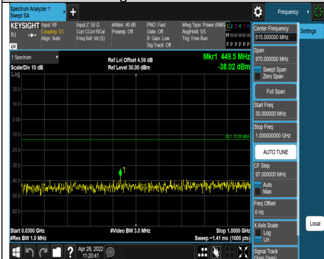
Band4-20MHz-16QAM-20050-1RB#0-
