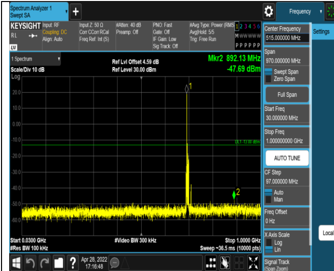
Band12-10MHz-QPSK-23095-1RB#0- Range1:30~1000MHz
