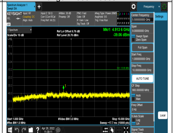
Band5-1.4MHz-16QAM-20525-1RB#0- Range2:1000~10000MHz
