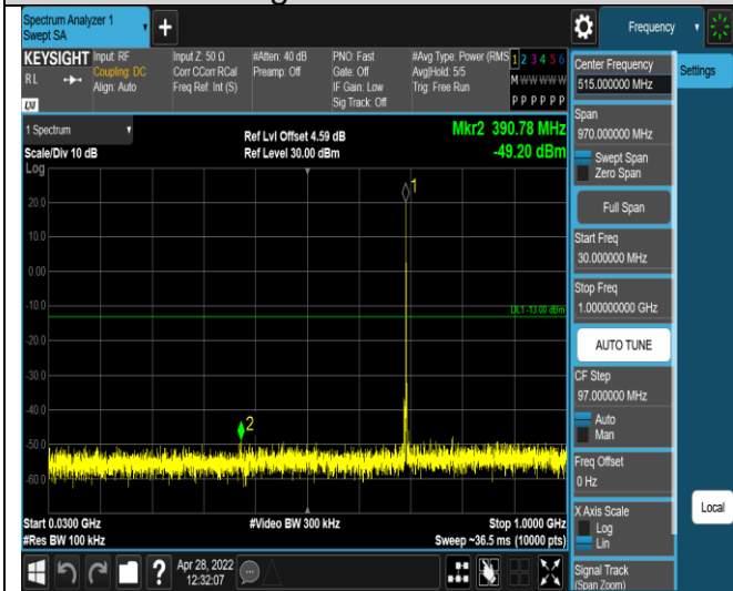
Band12-1.4MHz-QPSK-23095-1RB#0- Range1:30~1000MHz
