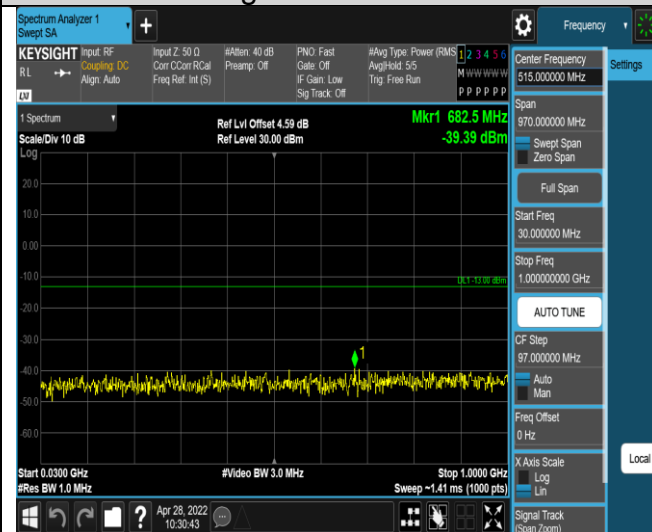
Band4-20MHz-QPSK-20050-1RB#0- Range1:30~1000MHz
