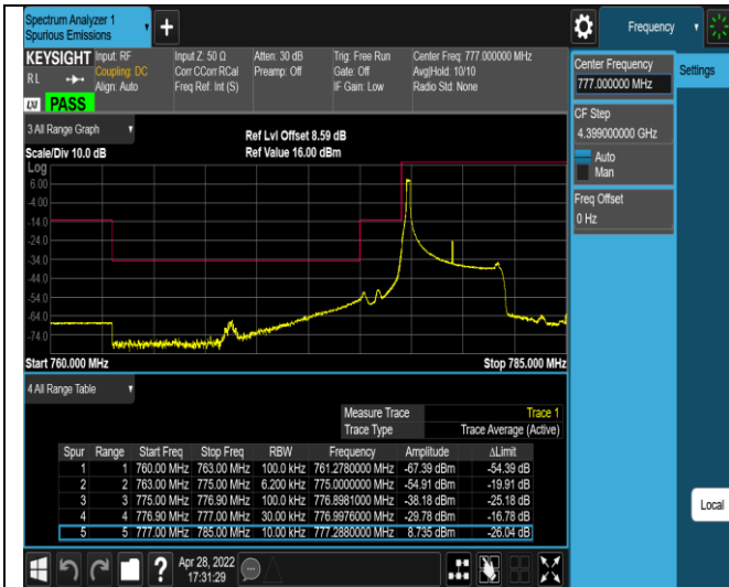
Band13-5MHz-QPSK-23205-25RB#0
