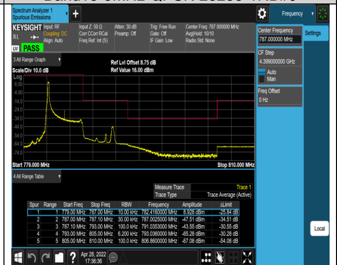
Band13-5MHz-QPSK-23255-25RB#0
