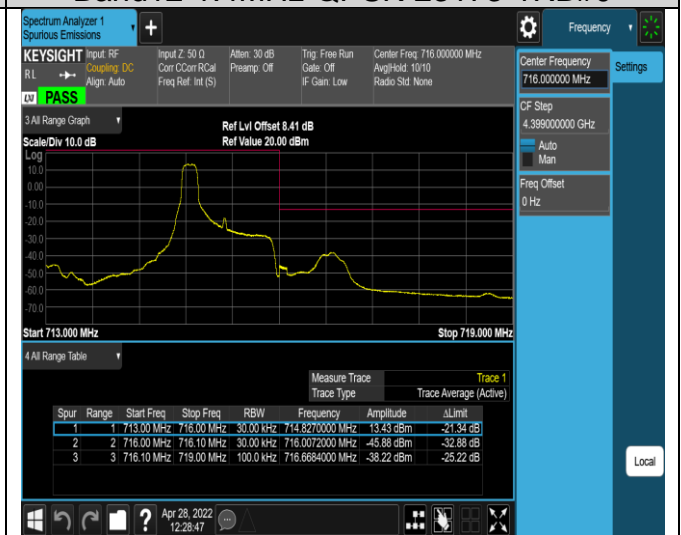
Band12-1.4MHz-QPSK-23173-6RB#0
