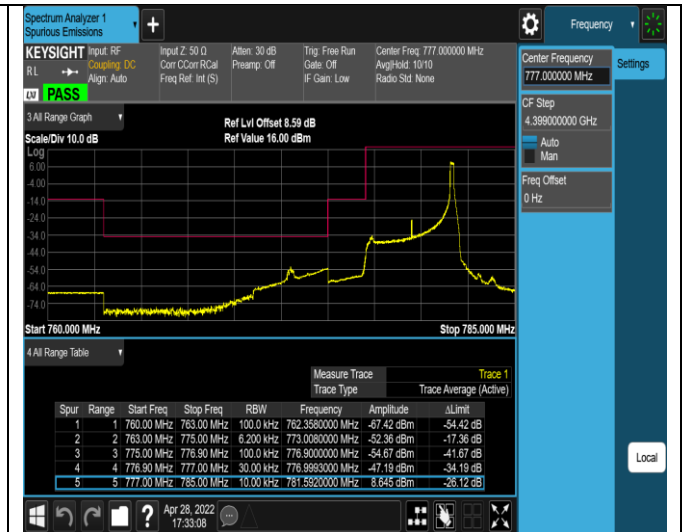
Band13-5MHz-QPSK-23255-1RB#0
