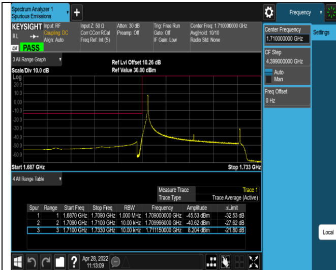
Band4-20MHz-16QAM-20050-100RB#0
