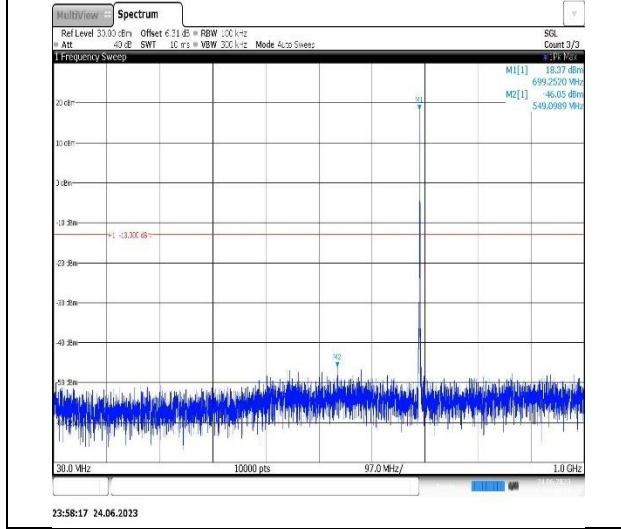
Band12-1.4MHz-QPSK-23095-1RB#0-Range1:30~1000MHz
