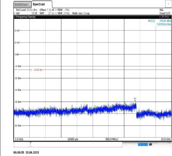
Band12-5MHz-16QAM-23095-1RB#0- Range2:1000~10000MHz
