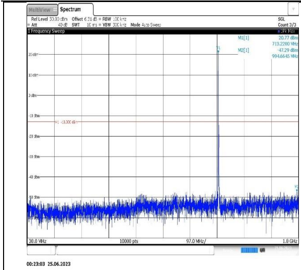
Band12-5MHz-QPSK-23035-1RB#0-Range1:30~1000MHz
