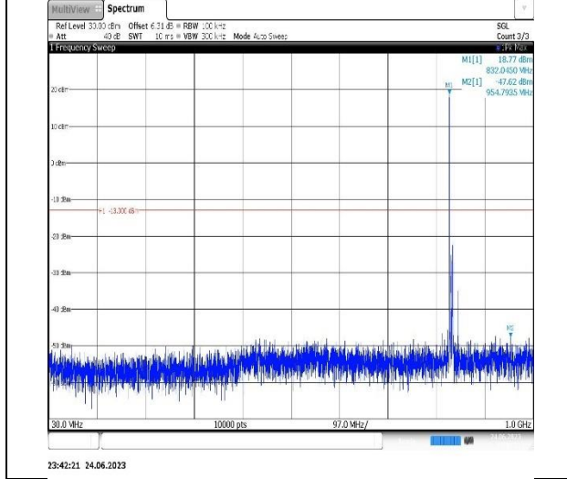
Band5-10MHz-16QAM-20600-1RB#0-Range1:30~1000MHz
