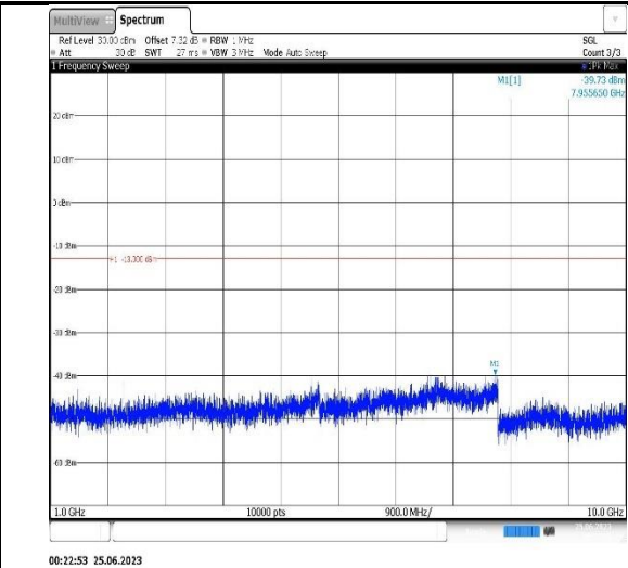
Band12-3MHz-16QAM-23025-1RB#0- Range2:1000~10000MHz
