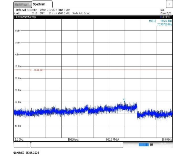
Band12-10MHz-16QAM-23130-1RB#0- Range2:1000~10000MHz
