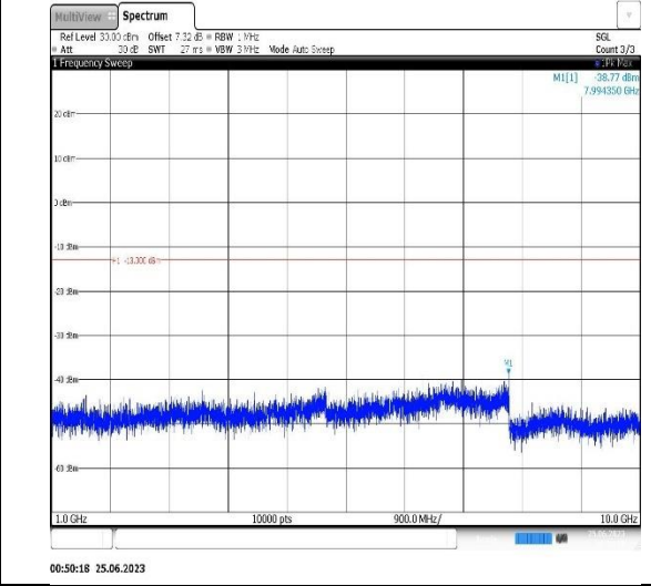
Band12-5MHz-QPSK-23095-1RB#0-Range2:1000~10000MHz
