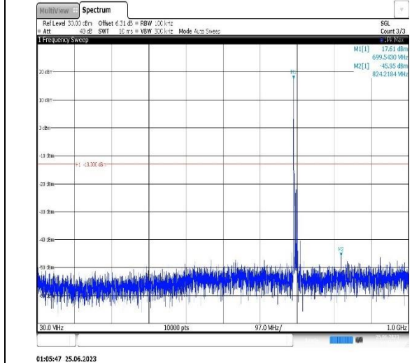
Band12-10MHz-QPSK-23095-1RB#0- Range1:30~1000MHz
