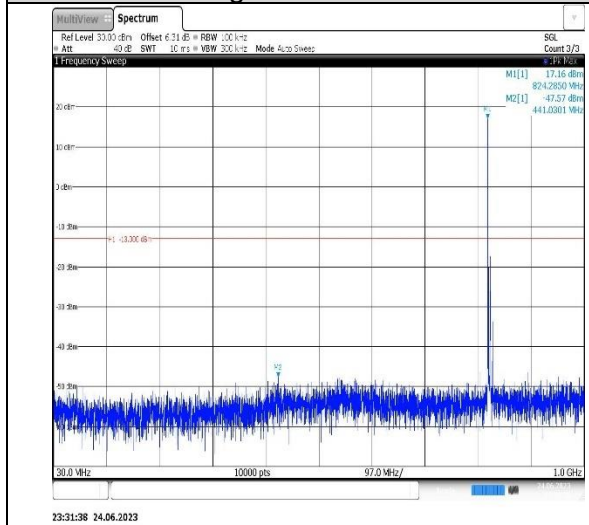
Band5-5MHz-16QAM-20525-1RB#0-Range1:30~1000MHz
