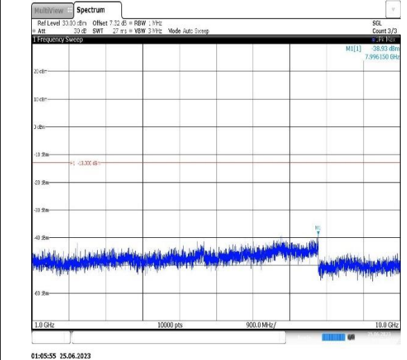
Band12-10MHz-QPSK-23095-1RB#0- Range2:1000~10000MHz
