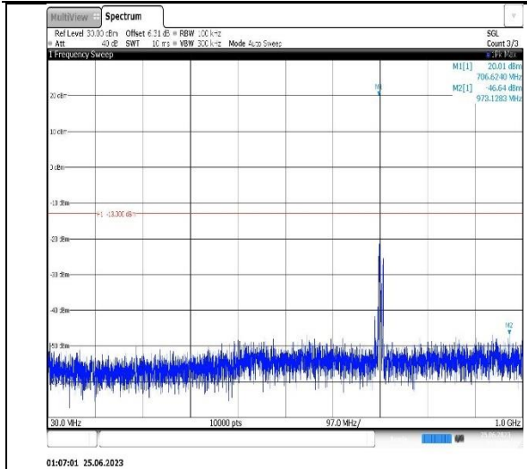
Band12-10MHz-16QAM-23060-1RB#0- Range1:30~1000MHz
