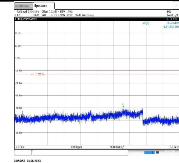
Band12-3MHz-QPSK-23025-1RB#0- Range2:1000~10000MHz
