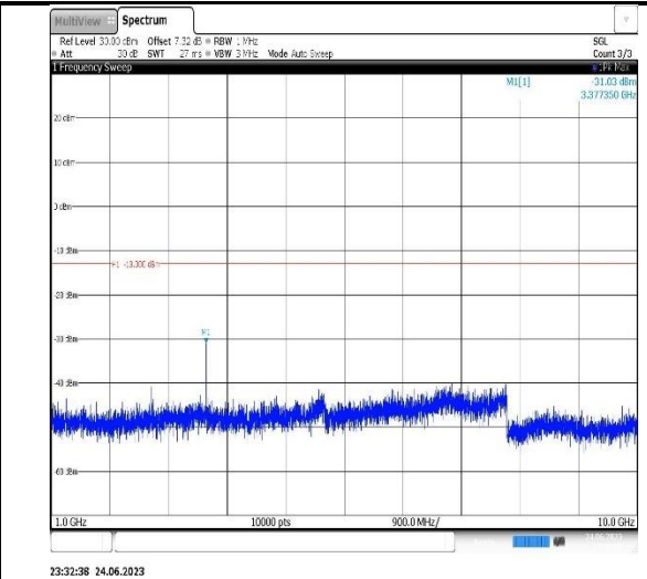
Band5-5MHz-16QAM-20425-1RB#0-Range2:1000~10000MHz
