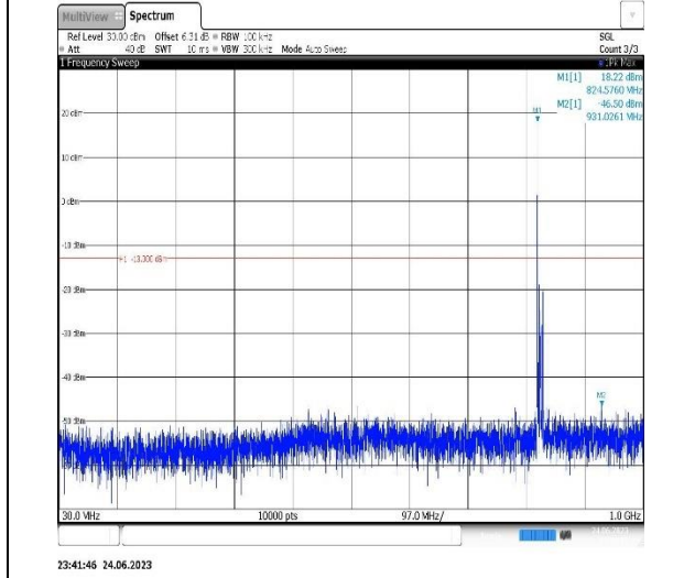
Band5-10MHz-16QAM-20525-1RB#0-Range1:30~1000MHz
