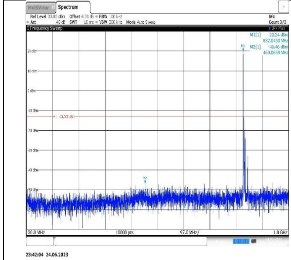
Band5-10MHz-QPSK-20600-1RB#0-Range1:30~1000MHz
