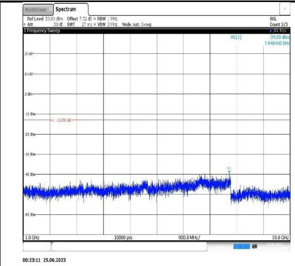
Band12-5MHz-QPSK-23035-1RB#0-Range2:1000~10000MHz
