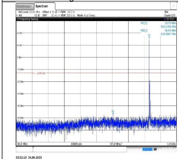
Band5-5MHz-16QAM-20625-1RB#0-Range1:30~1000MHz
