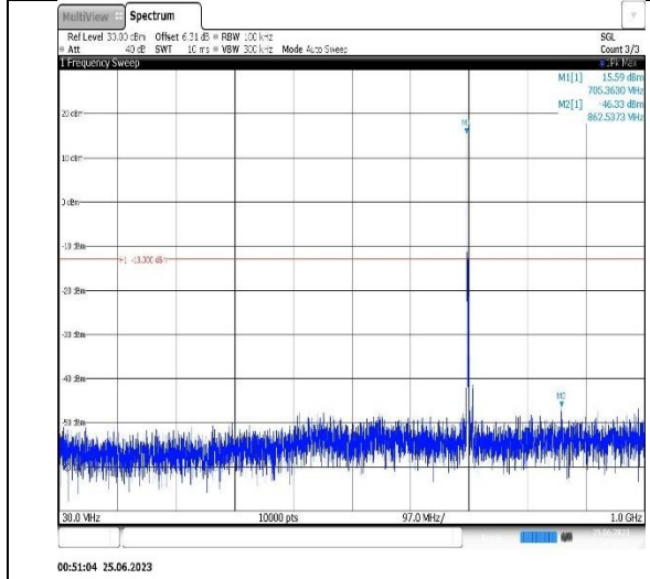
Band12-5MHz-16QAM-23155-1RB#0- Range1:30~1000MHz
