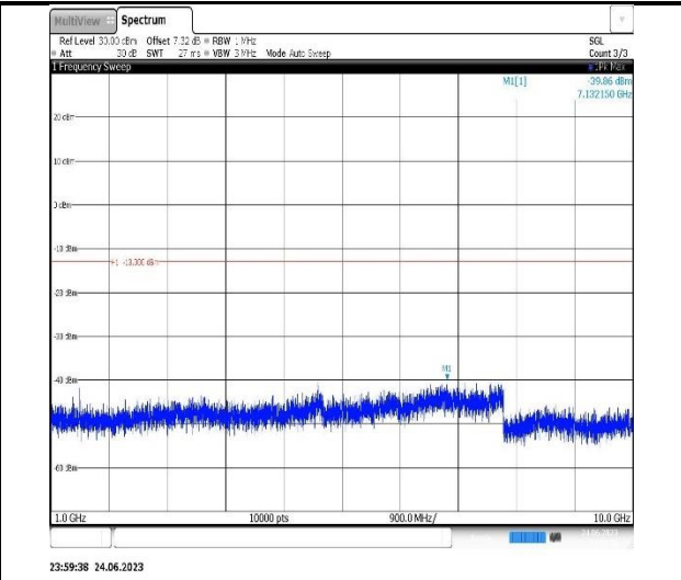
Band12-1.4MHz-16QAM-23017-1RB#0- Range2:1000~10000MHz
