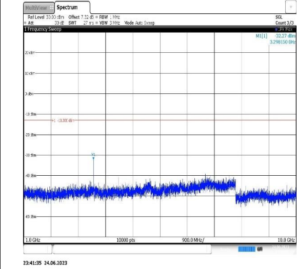
Band5-10MHz-QPSK-20525-1RB#0-Range2:1000~10000MHz
