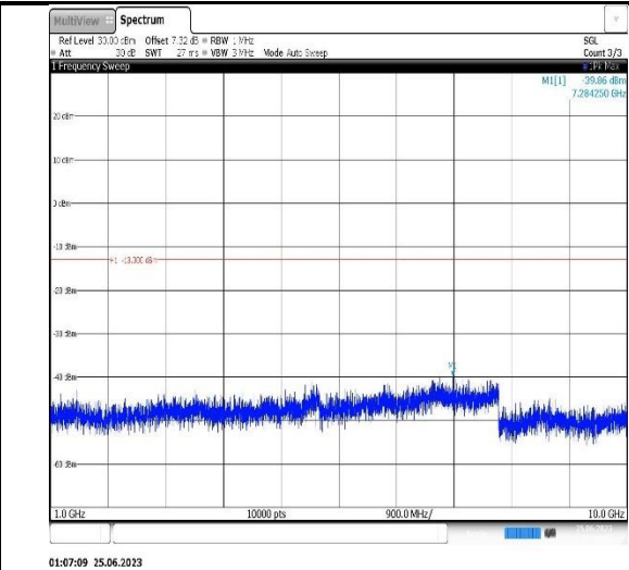
Band12-10MHz-16QAM-23060-1RB#0- Range2:1000~10000MHz
