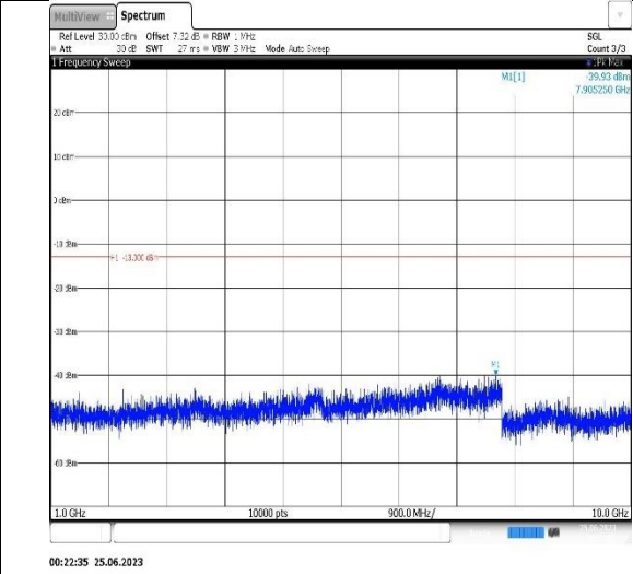
Band12-3MHz-16QAM-23165-1RB#0- Range2:1000~10000MHz
