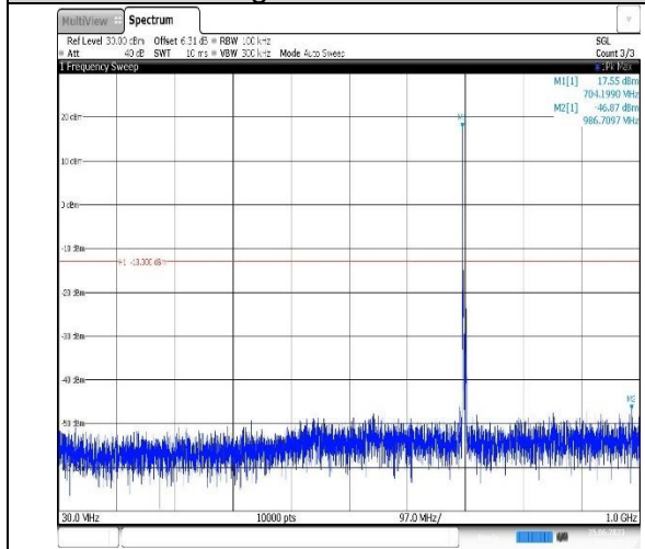
Band17-5MHz-QPSK-23755-1RB#0-Range1:30~1000MHz
