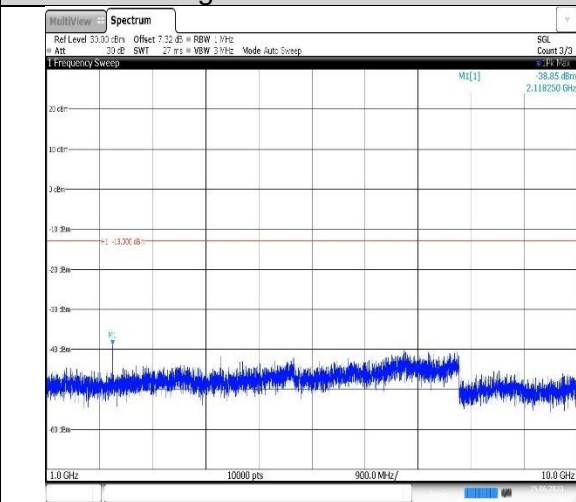
Band12-3MHz-QPSK-23165-1RB#0- Range2:1000~10000MHz
