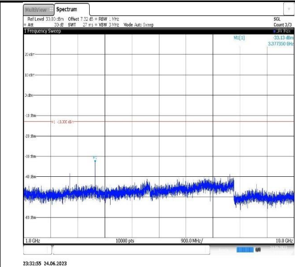
Band5-10MHz-QPSK-20450-1RB#0-Range2:1000~10000MHz
