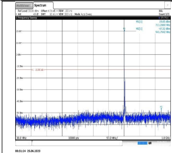
Band12-5MHz-16QAM-23035-1RB#0- Range1:30~1000MHz
