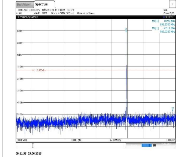
Band12-3MHz-16QAM-23095-1RB#0- Range1:30~1000MHz
