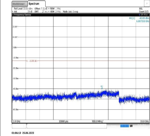
Band12-10MHz-16QAM-23095-1RB#0- Range2:1000~10000MHz
