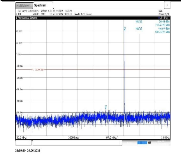
Band12-1.4MHz-16QAM-23017-1RB#0- Range1:30~1000MHz
