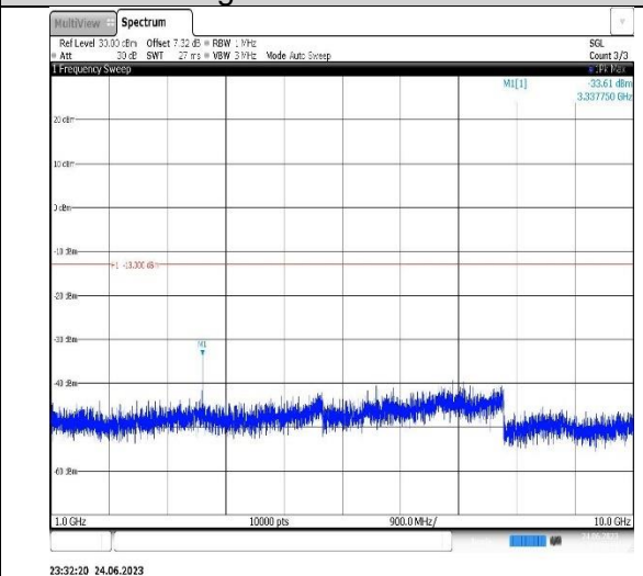
Band5-5MHz-16QAM-20625-1RB#0-Range2:1000~10000MHz
