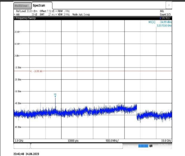
Band5-10MHz-16QAM-20450-1RB#0-Range2:1000~10000MHz
