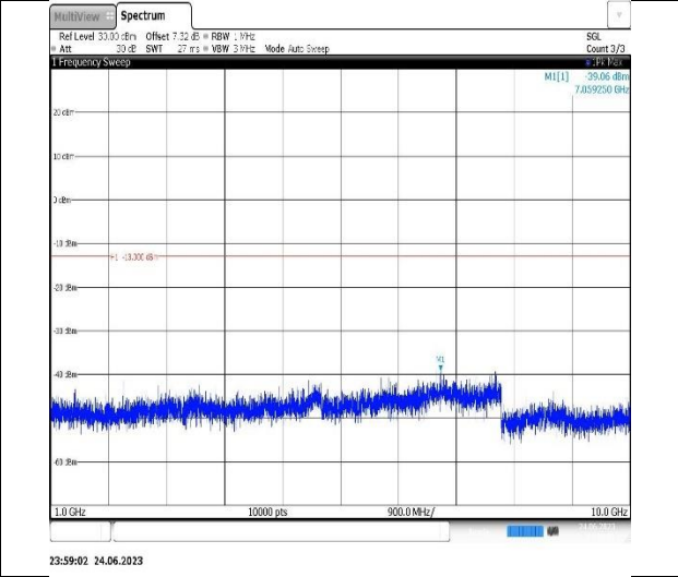
Band12-1.4MHz-QPSK-23173-1RB#0-Range2:1000~10000MHz
