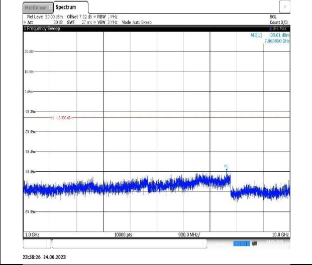
Band12-1.4MHz-QPSK-23095-1RB#0-Range2:1000~10000MHz
