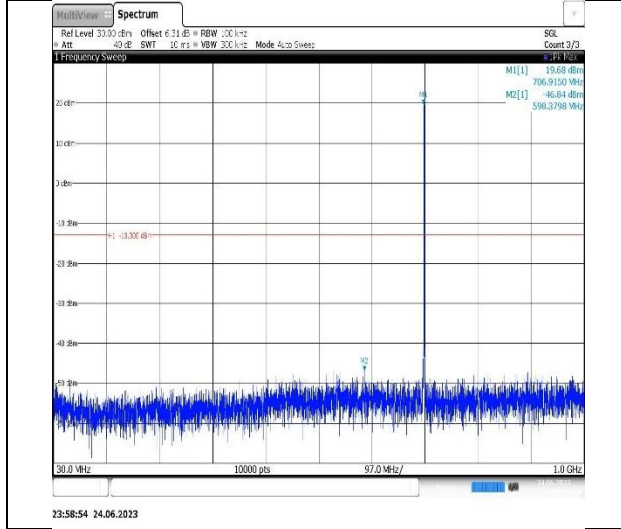
Band12-1.4MHz-QPSK-23173-1RB#0-Range1:30~1000MHz
