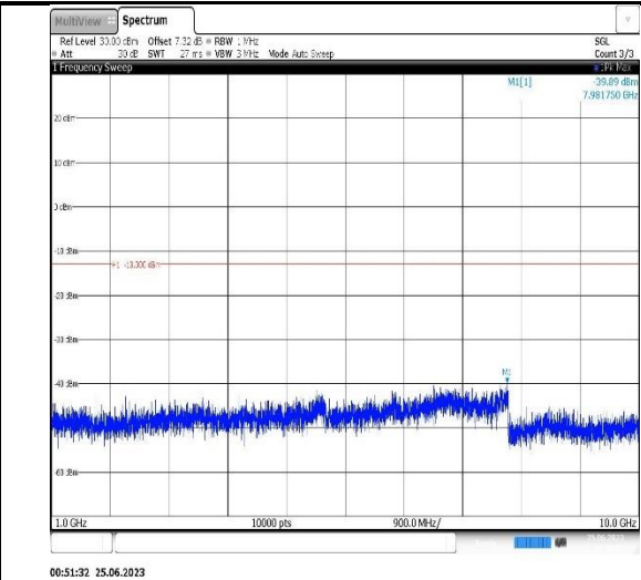
Band12-5MHz-16QAM-23035-1RB#0- Range2:1000~10000MHz
