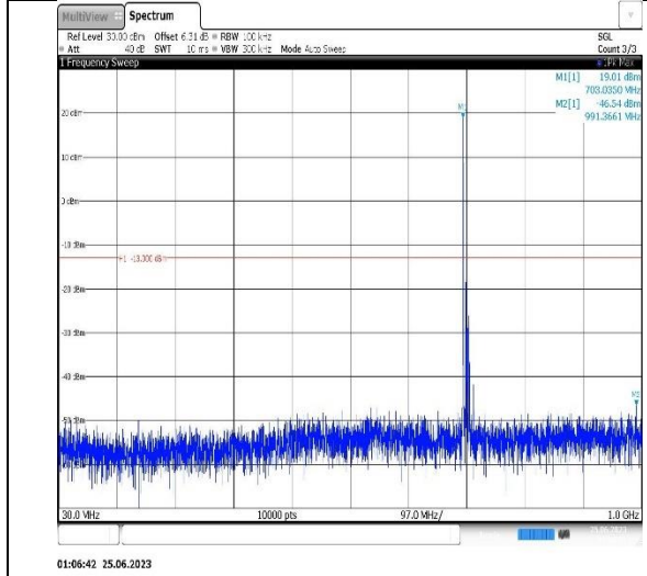
Band12-10MHz-16QAM-23130-1RB#0- Range1:30~1000MHz
