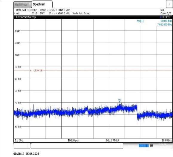
Band12-5MHz-16QAM-23155-1RB#0- Range2:1000~10000MHz
