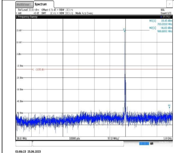
Band12-10MHz-QPSK-23130-1RB#0- Range1:30~1000MHz
