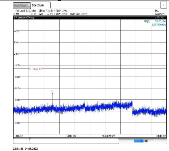
Band5-5MHz-16QAM-20525-1RB#0-Range2:1000~10000MHz
