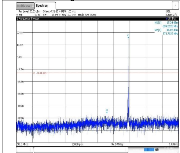
Band12-3MHz-QPSK-23025-1RB#0- Range1:30~1000MHz
