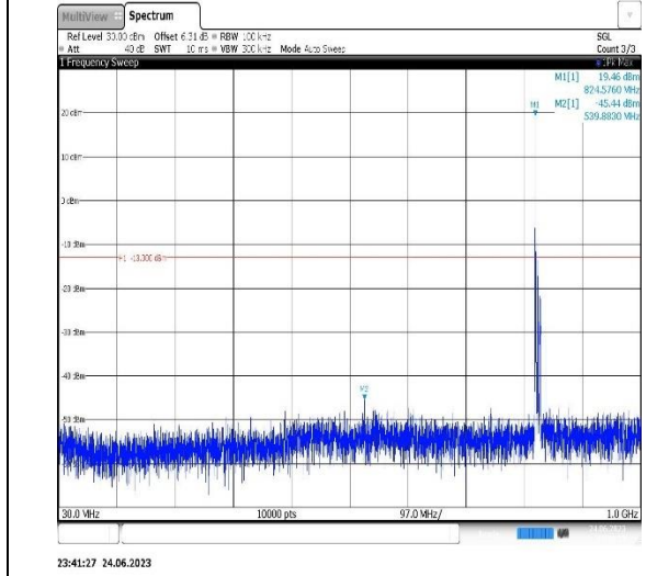
Band5-10MHz-QPSK-20525-1RB#0-Range1:30~1000MHz
