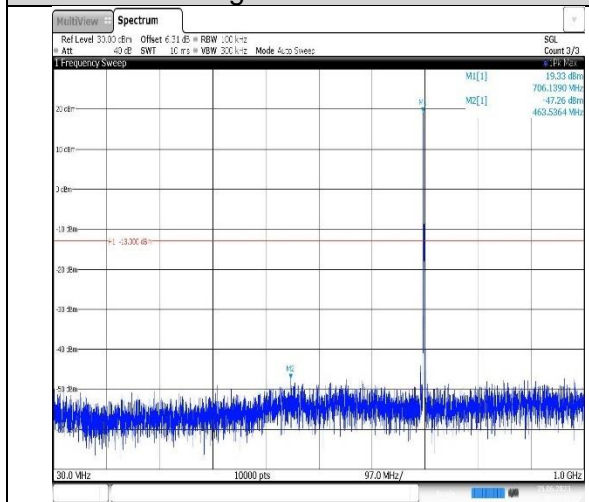
Band12-3MHz-QPSK-23165-1RB#0- Range1:30~1000MHz
