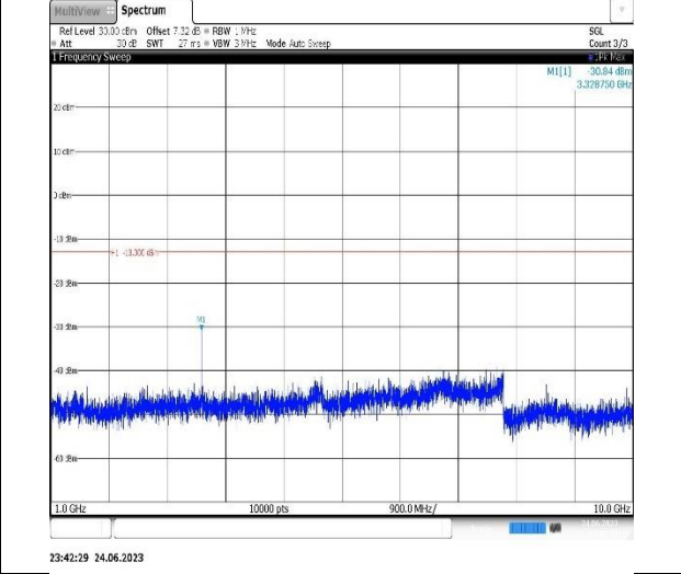
Band5-10MHz-16QAM-20600-1RB#0-Range2:1000~10000MHz
