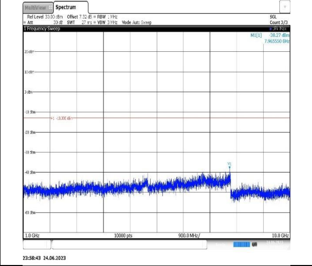
Band12-1.4MHz-16QAM-23095-1RB#0- Range2:1000~10000MHz
