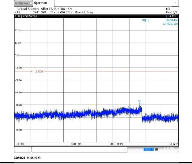
Band12-1.4MHz-16QAM-23173-1RB#0- Range2:1000~10000MHz
