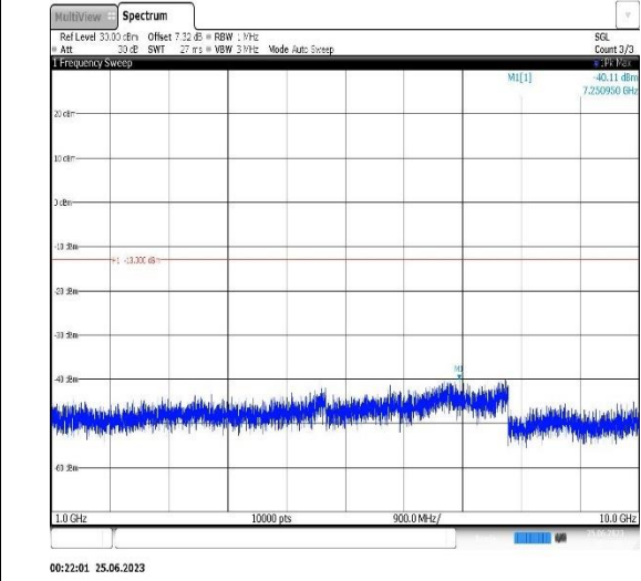
Band12-3MHz-16QAM-23095-1RB#0- Range2:1000~10000MHz
