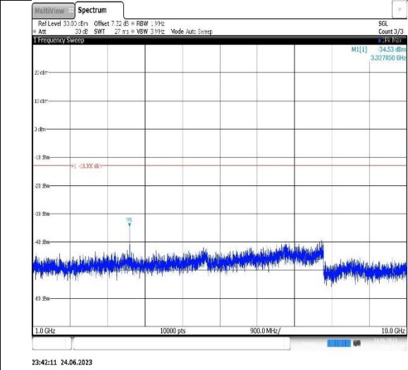
Band5-10MHz-QPSK-20600-1RB#0-Range2:1000~10000MHz
