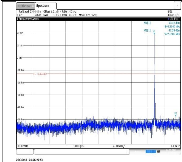
Band5-10MHz-QPSK-20450-1RB#0-Range1:30~1000MHz
