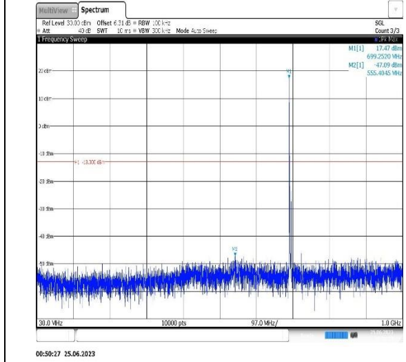
Band12-5MHz-16QAM-23095-1RB#0- Range1:30~1000MHz
