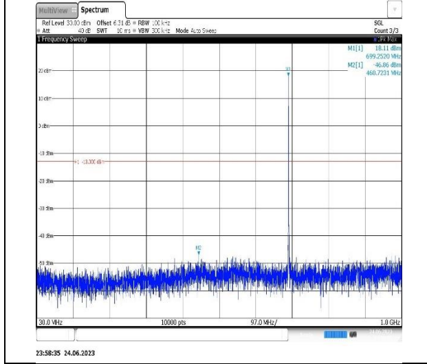
Band12-1.4MHz-16QAM-23095-1RB#0- Range1:30~1000MHz
