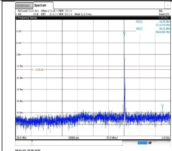
Band12-10MHz-QPSK-23060-1RB#0- Range1:30~1000MHz
