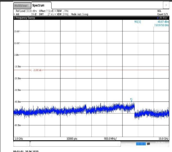
Band12-10MHz-QPSK-23060-1RB#0- Range2:1000~10000MHz
