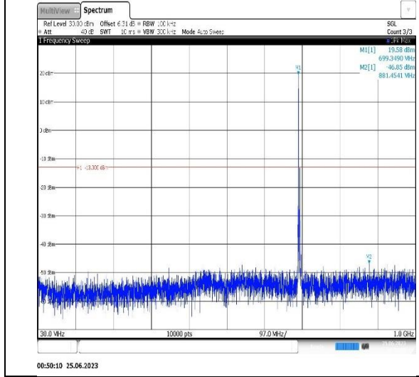
Band12-5MHz-QPSK-23095-1RB#0-Range1:30~1000MHz
