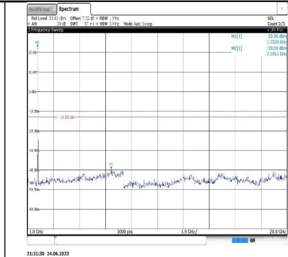
Band4-15MHz-16QAM-20025-1RB#0- Range2:1000~20000MHz
