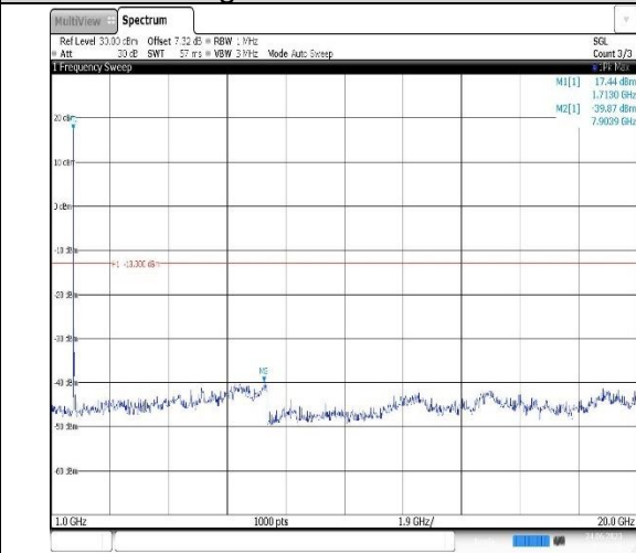
Band4-10MHz-16QAM-20000-1RB#0-Range2:1000~20000MHz
