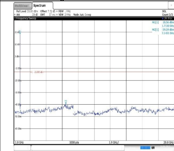
Band4-1.4MHz-16QAM-19957-1RB#0-Range2:1000~20000MHz
