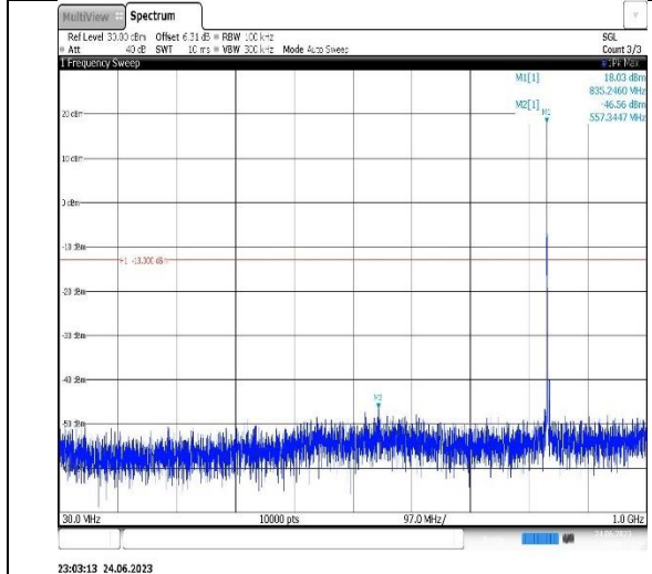
Band5-3MHz-16QAM-20635-1RB#0-Range1:30~1000MHz
