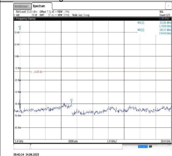
Band4-5MHz-16QAM-20375-1RB#0-Range2:1000~20000MHz
