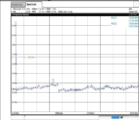
Band4-20MHz-16QAM-20050-1RB#0- Range2:1000~20000MHz
