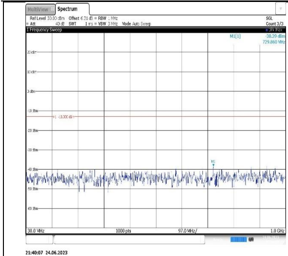
Band5-1.4MHz-QPSK-20407-1RB#0-Range1:30~1000MHz
