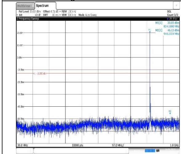
Band5-1.4MHz-QPSK-20407-1RB#0-Range1:30~1000MHz
