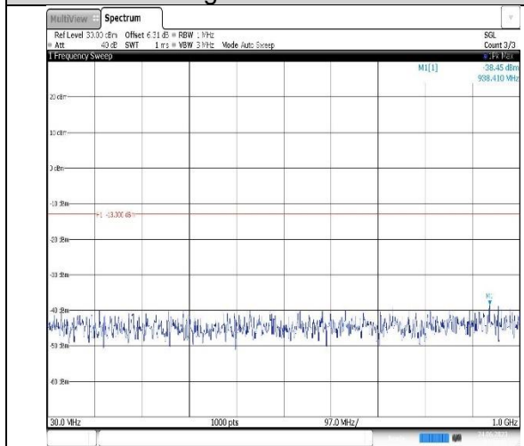
Band4-20MHz-16QAM-20300-1RB#0- Range1:30~1000MHz
