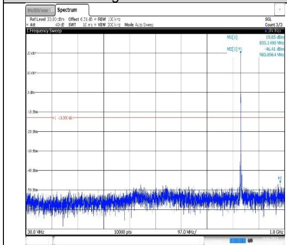
Band5-3MHz-QPSK-20635-1RB#0- Range1:30~1000MHz
