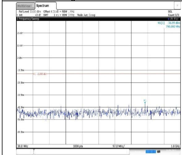
Band2-20MHz-16QAM-18700-1RB#0-Range1:30~1000MHz
