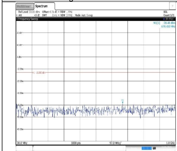
Band4-10MHz-QPSK-20350-1RB#0-Range1:30~1000MHz
