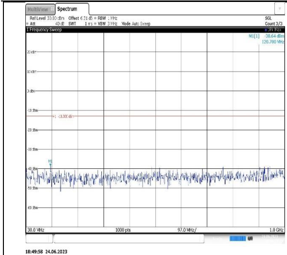
Band2-20MHz-16QAM-18700-1RB#0-Range1:30~1000MHz
