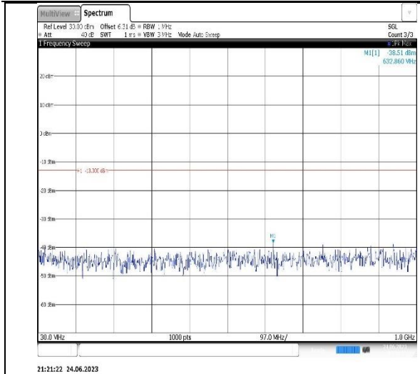
Band4-10MHz-16QAM-20000-1RB#0-Range1:30~1000MHz
