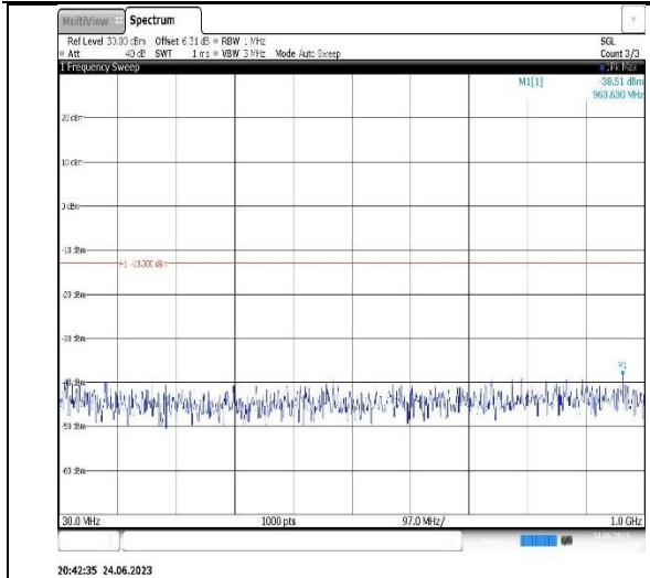
Band4-5MHz-16QAM-19975-1RB#0-Range1:30~1000MHz
