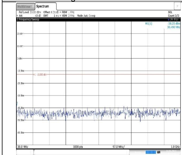
Band4-15MHz-QPSK-20325-1RB#0- Range1:30~1000MHz
