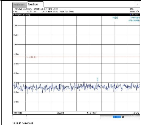
Band4-5MHz-QPSK-19975-1RB#0- Range1:30~1000MHz
