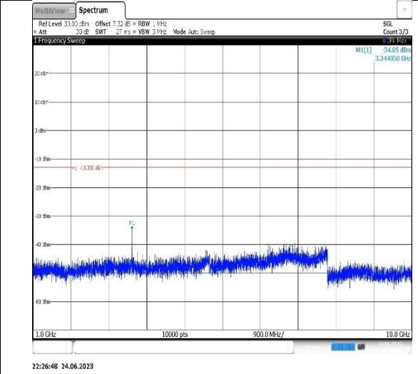
Band5-1.4MHz-16QAM-20643-1RB#0-Range2:1000~10000MHz
