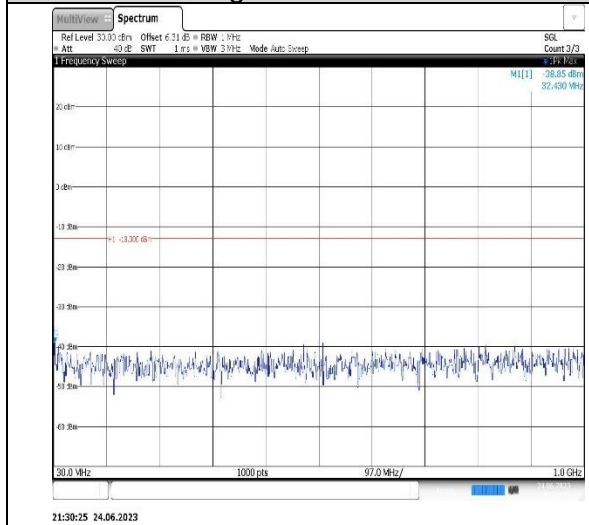
Band4-15MHz-16QAM-20175-1RB#0- Range1:30~1000MHz
