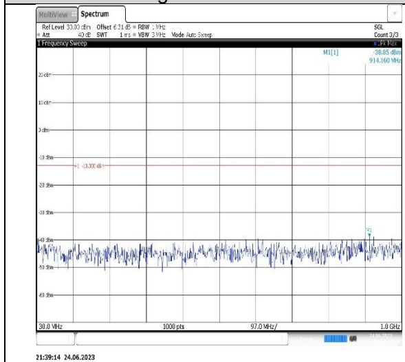
Band4-20MHz-QPSK-20300-1RB#0-Range1:30~1000MHz
