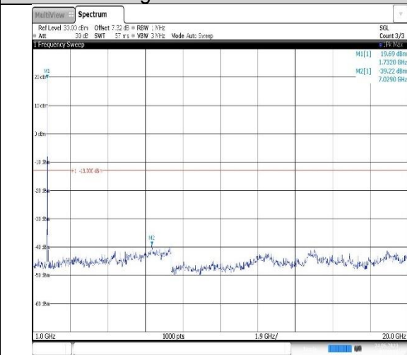
Band4-10MHz-16QAM-20350-1RB#0-Range2:1000~20000MHz
