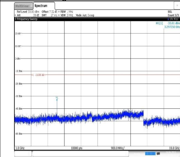
Band5-1.4MHz-QPSK-20407-1RB#0-Range2:1000~10000MHz
