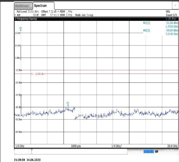
Band4-20MHz-16QAM-20050-1RB#0- Range2:1000~20000MHz
