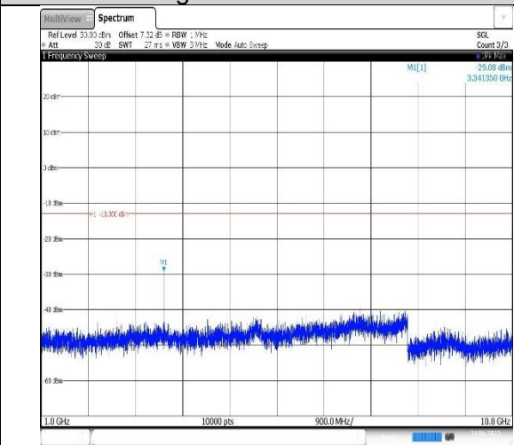
Band5-3MHz-QPSK-20635-1RB#0- Range2:1000~10000MHz
