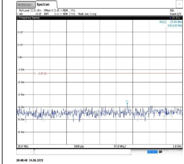
18:48:48 24.06.2023 Band2-20MHz-QPSK-18900-1RB#0-Range1:30~1000MHz
