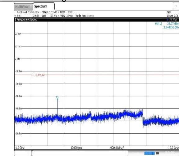
Band5-1.4MHz-QPSK-20643-1RB#0-Range2:1000~10000MHz
