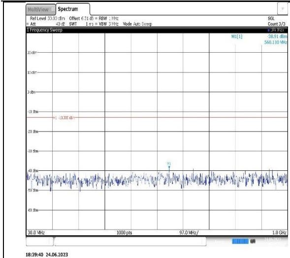
18:39:40 24.06.2023 Band2-20MHz-QPSK-18700-1RB#0-Range1:30~1000MHz
