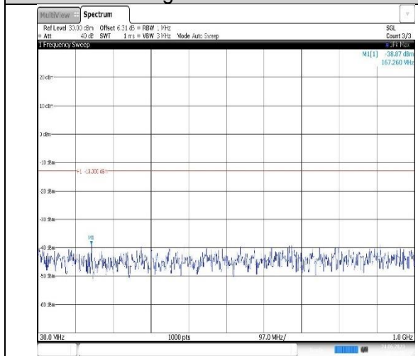
Band2-20MHz-16QAM-19100-1RB#0-Range1:30~1000MHz
