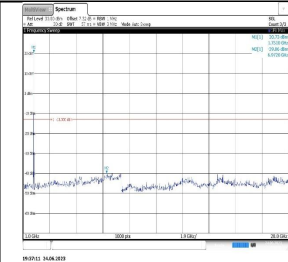
Band4-1.4MHz-16QAM-19957-1RB#0-Range2:1000~20000MHz
