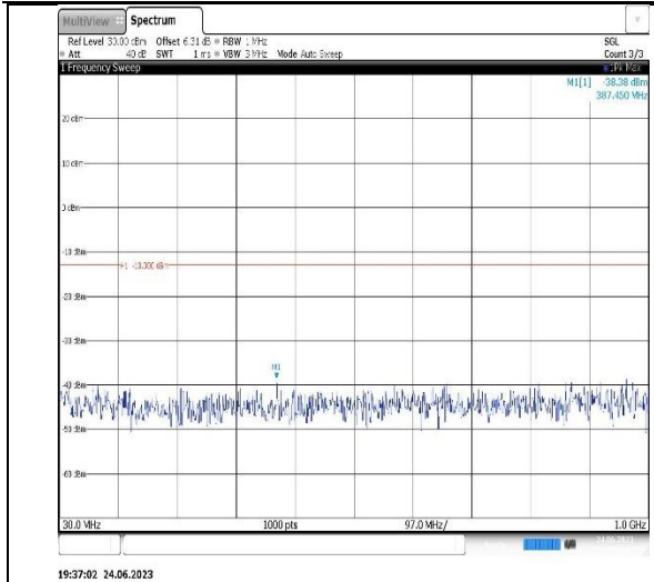
Band4-1.4MHz-16QAM-19957-1RB#0-Range1:30~1000MHz
