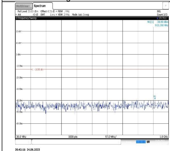
Band4-5MHz-16QAM-20375-1RB#0-Range1:30~1000MHz
