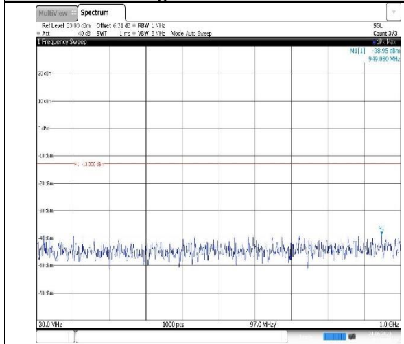
Band4-15MHz-QPSK-20025-1RB#0- Range1:30~1000MHz
