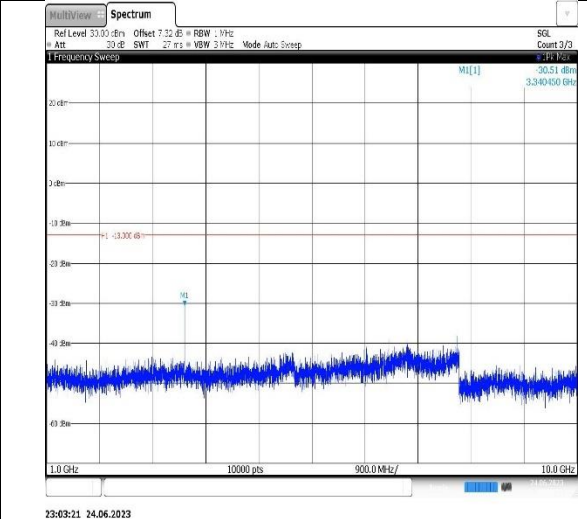
Band5-3MHz-16QAM-20635-1RB#0-Range2:1000~10000MHz
