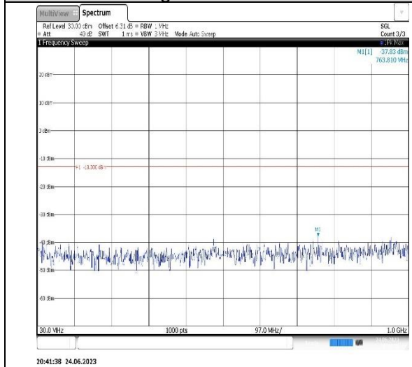
Band4-5MHz-16QAM-20175-1RB#0-Range1:30~1000MHz
