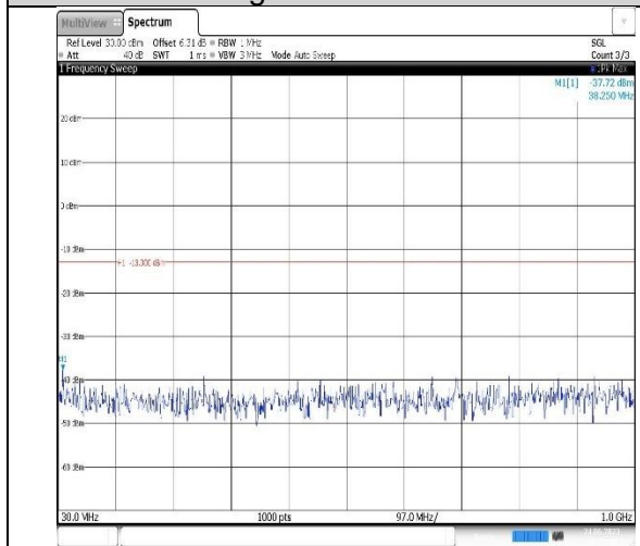
Band4-10MHz-16QAM-20350-1RB#0-Range1:30~1000MHz
