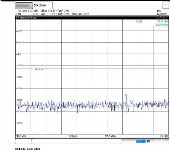
Band4-3MHz-16QAM-19965-1RB#0- Range1:30~1000MHz
