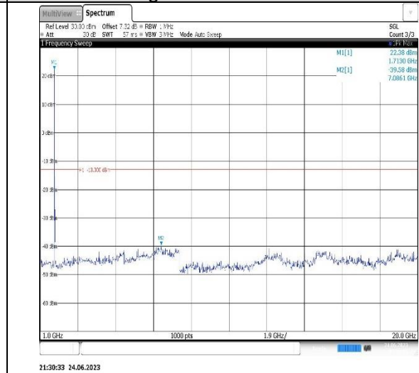
Band4-15MHz-16QAM-20175-1RB#0- Range2:1000~20000MHz
