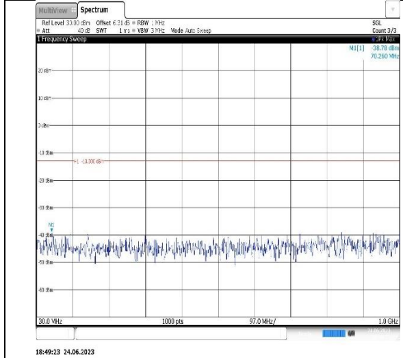
18:49:23 24.06.2023 Band2-20MHz-QPSK-19100-1RB#0-Range1:30~1000MHz
