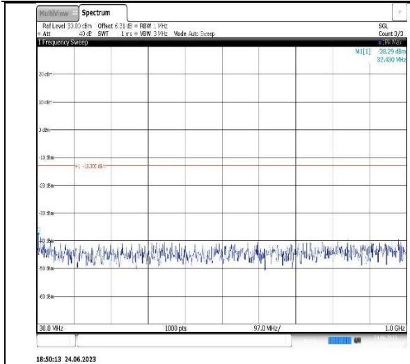
Band4-1.4MHz-QPSK-19957-1RB#0-Range1:30~1000MHz
