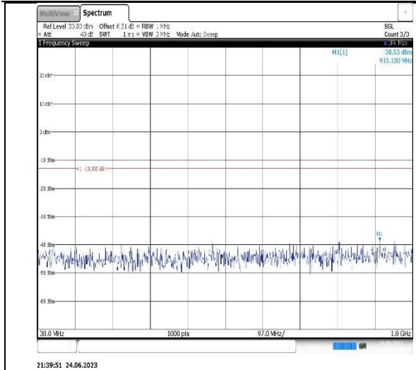
Band4-20MHz-16QAM-20050-1RB#0- Range1:30~1000MHz
