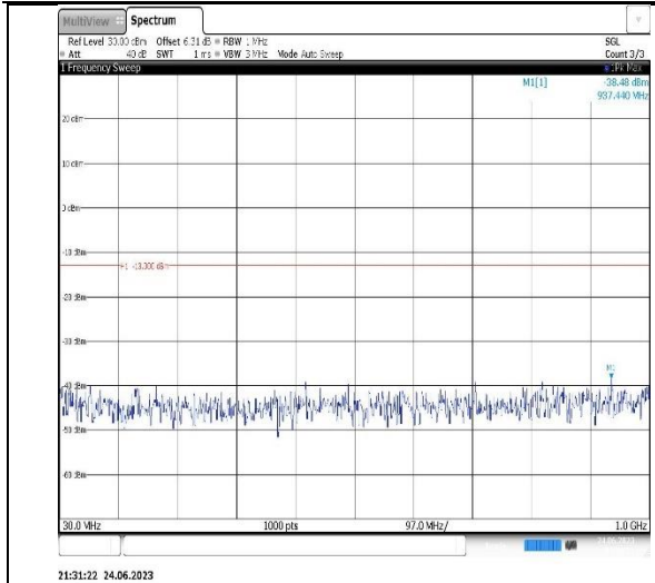
Band4-15MHz-16QAM-20025-1RB#0- Range1:30~1000MHz
