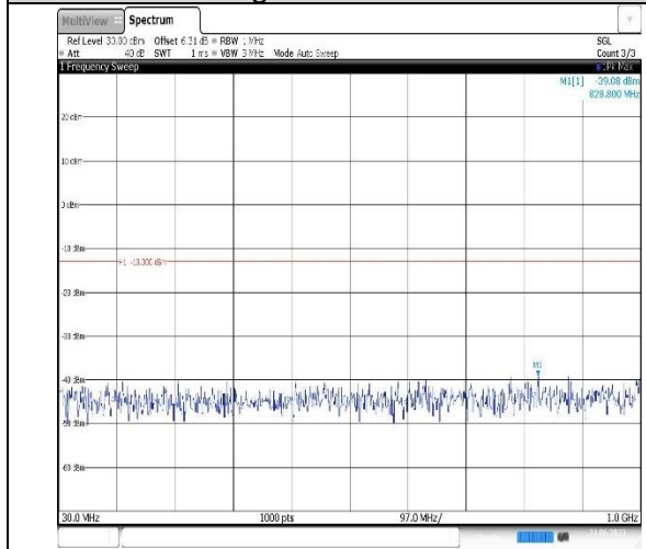
Band4-1.4MHz-QPSK-19957-1RB#0-Range1:30~1000MHz
