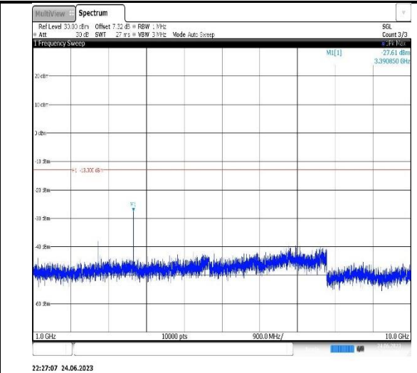
Band5-1.4MHz-16QAM-20407-1RB#0-Range2:1000~10000MHz
