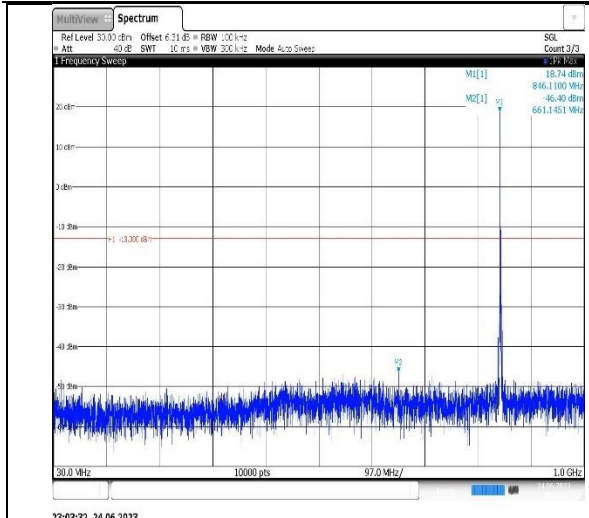
Band5-3MHz-16QAM-20415-1RB#0-Range1:30~1000MHz
