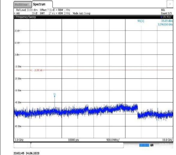
Band5-3MHz-16QAM-20525-1RB#0-Range2:1000~10000MHz
