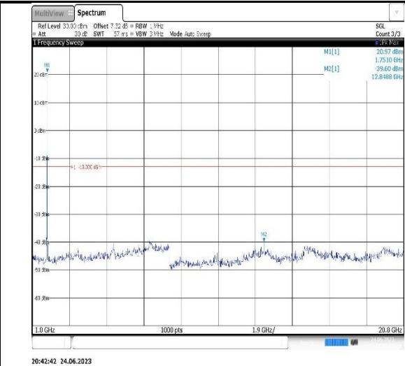
Band4-5MHz-16QAM-19975-1RB#0-Range2:1000~20000MHz
