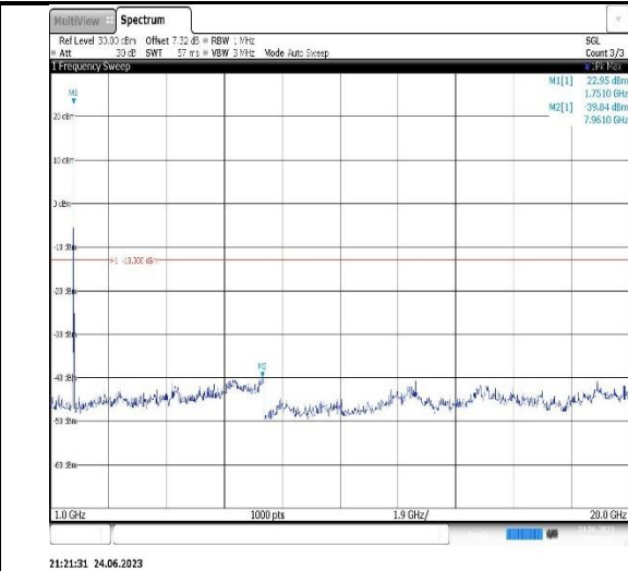
Band4-10MHz-16QAM-20000-1RB#0-Range2:1000~20000MHz
