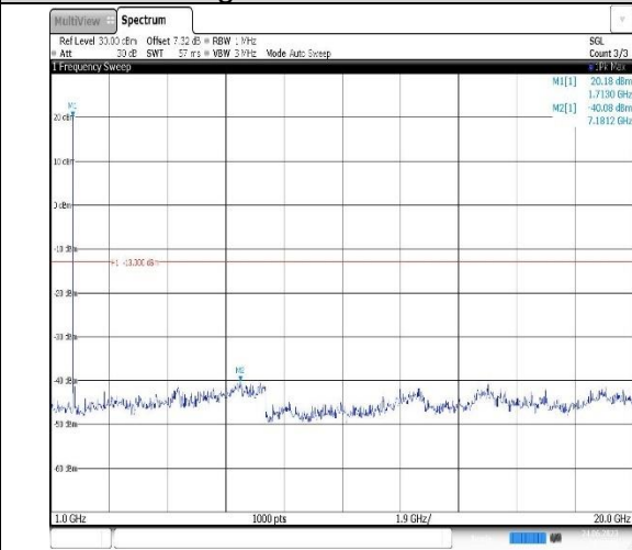
Band4-3MHz-16QAM-19965-1RB#0- Range2:1000~20000MHz
