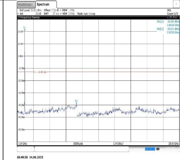
18:49:30 24.06.2023 Band2-20MHz-QPSK-19100-1RB#0-Range2:1000~20000MHz
