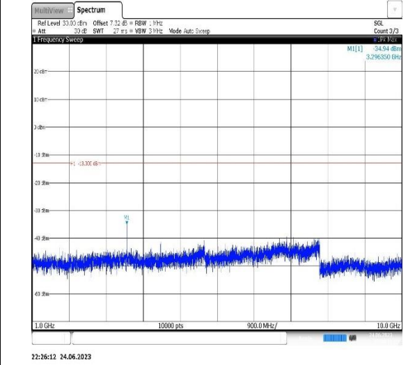
Band5-1.4MHz-16QAM-20525-1RB#0-Range2:1000~10000MHz
