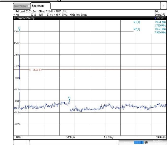
Band4-20MHz-16QAM-20300-1RB#0- Range2:1000~20000MHz
