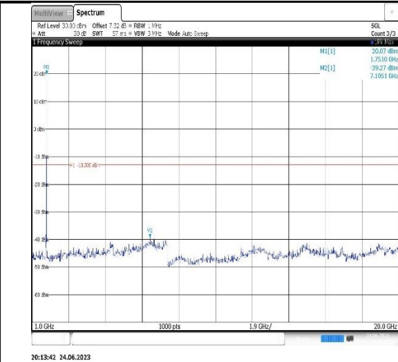
Band4-3MHz-16QAM-19965-1RB#0- Range2:1000~20000MHz
