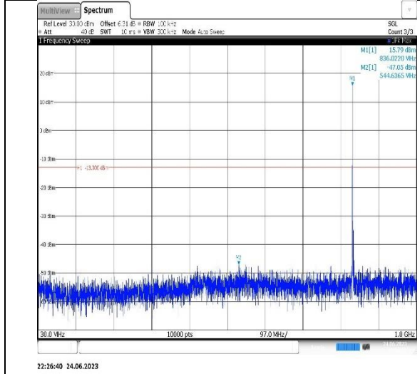
Band5-1.4MHz-16QAM-20643-1RB#0-Range1:30~1000MHz
