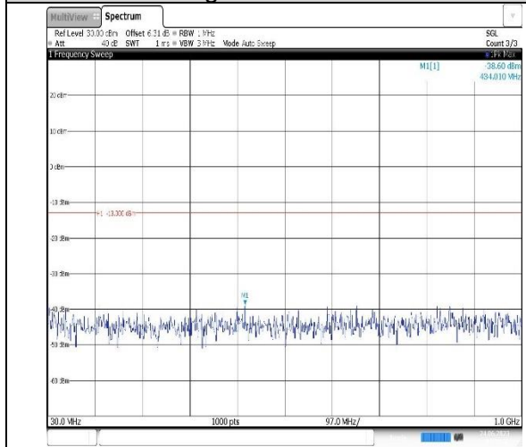
Band4-20MHz-16QAM-20050-1RB#0- Range1:30~1000MHz
