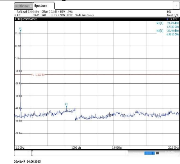
Band4-5MHz-16QAM-20175-1RB#0-Range2:1000~20000MHz
