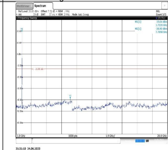
Band4-15MHz-16QAM-20325-1RB#0- Range2:1000~20000MHz
