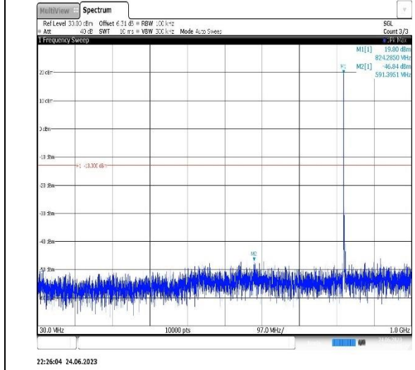
Band5-1.4MHz-16QAM-20525-1RB#0-Range1:30~1000MHz
