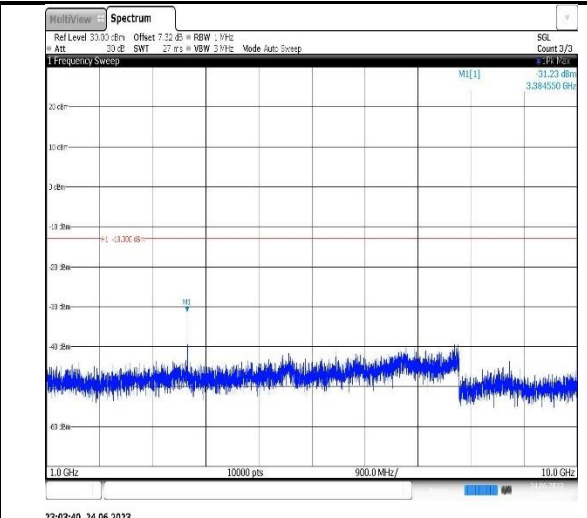
Band5-3MHz-16QAM-20415-1RB#0-Range2:1000~10000MHz
