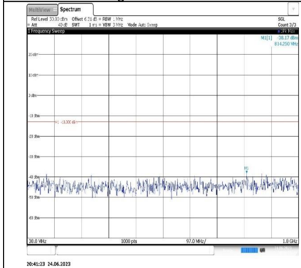
Band4-5MHz-QPSK-20175-1RB#0- Range1:30~1000MHz
