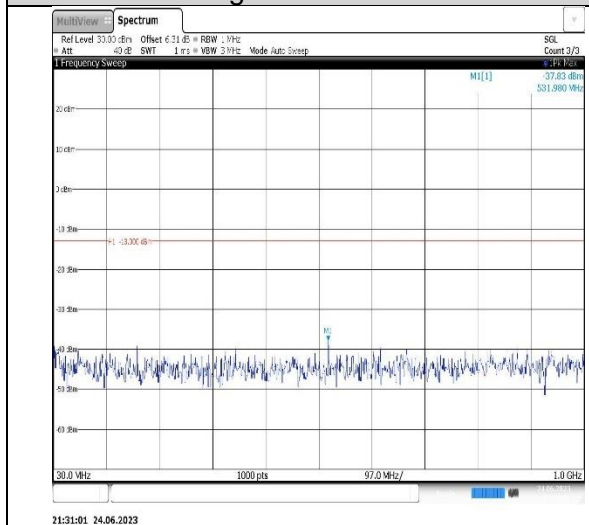
Band4-15MHz-16QAM-20325-1RB#0- Range1:30~1000MHz
