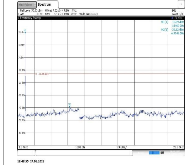
18:48:55 24.06.2023 Band2-20MHz-QPSK-18900-1RB#0-Range2:1000~20000MHz
