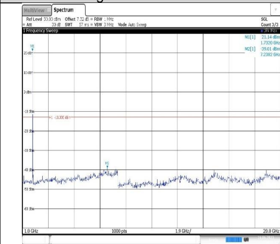
Band4-1.4MHz-16QAM-20393-1RB#0-Range2:1000~20000MHz
