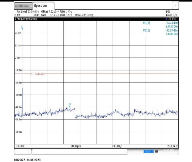
Band2-5MHz-16QAM-18625-1RB#0-Range2:1000~20000MHz
