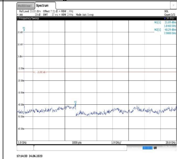
Band2-1.4MHz-16QAM-18900-1RB#0-Range2:1000~20000MHz
