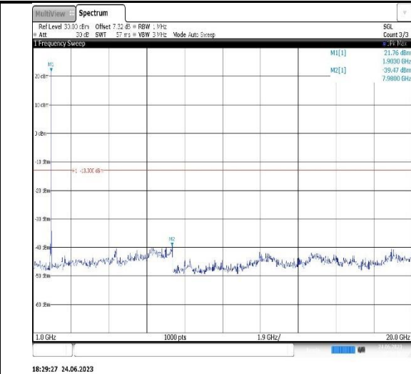
Band2-15MHz-QPSK-18675-1RB#0-Range2:1000~20000MHz
