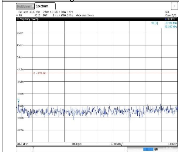
Band2-10MHz-QPSK-19150-1RB#0-Range1:30~1000MHz
