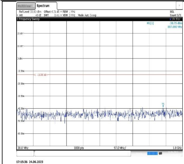
Band2-3MHz-QPSK-18615-1RB#0-Range1:30~1000MHz
