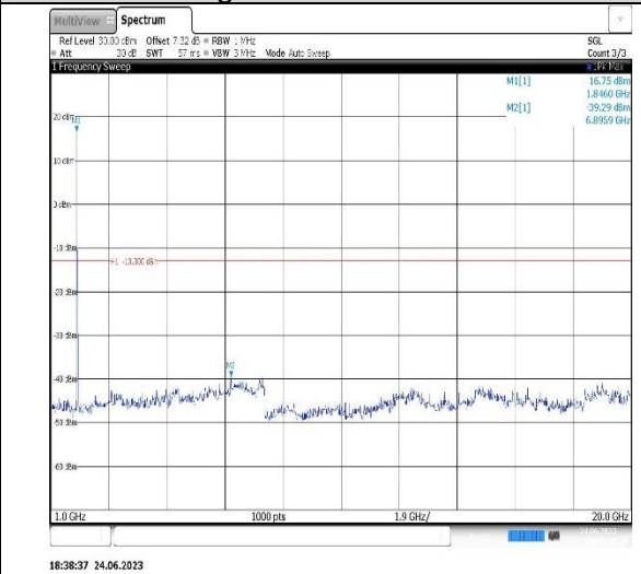
Band2-15MHz-16QAM-18900-1RB#0- Range2:1000~20000MHz
