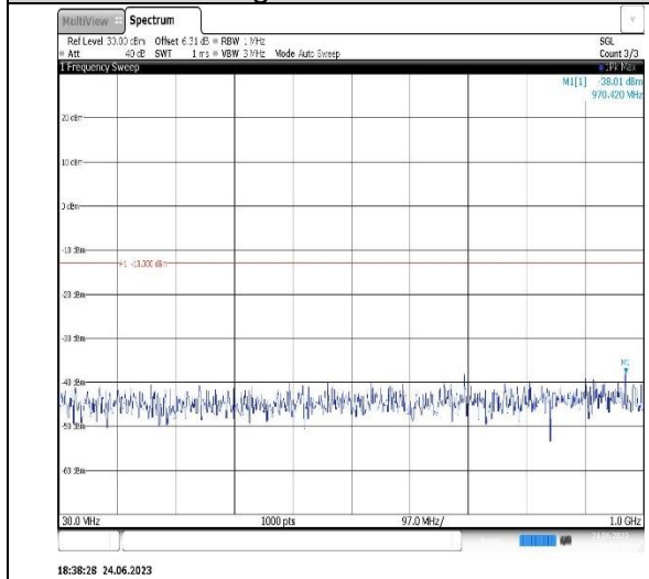
Band2-15MHz-16QAM-18900-1RB#0- Range1:30~1000MHz
