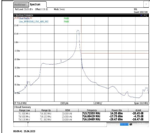
Band12-3MHz-16QAM-23025-1RB#0
