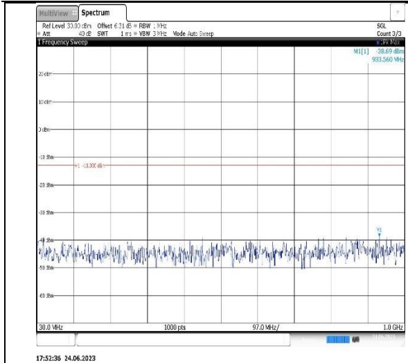
Band2-5MHz-QPSK-18625-1RB#0- Range1:30~1000MHz
