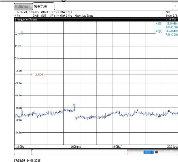
Band2-3MHz-16QAM-19185-1RB#0- Range2:1000~20000MHz
