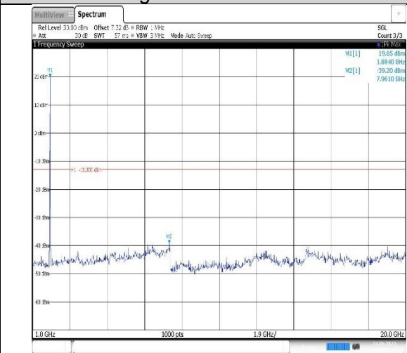
Band2-10MHz-16QAM-19150-1RB#0- Range2:1000~20000MHz
