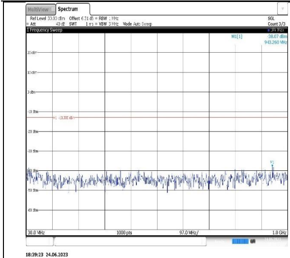
Band2-15MHz-16QAM-18675-1RB#0- Range1:30~1000MHz
