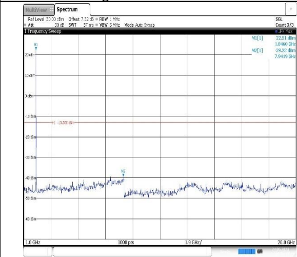
Band2-10MHz-16QAM-18650-1RB#0- Range2:1000~20000MHz
