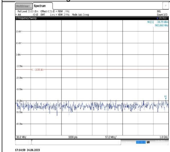
Band2-1.4MHz-16QAM-19193-1RB#0-Range1:30~1000MHz
