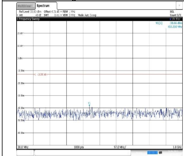
Band2-10MHz-16QAM-18650-1RB#0- Range1:30~1000MHz
