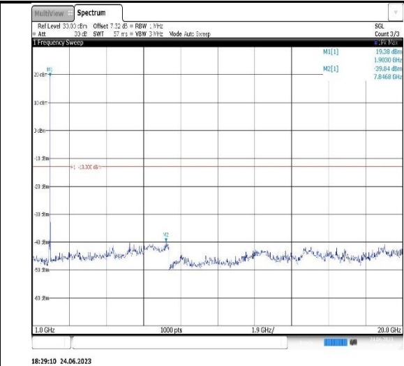
Band2-10MHz-16QAM-18650-1RB#0- Range2:1000~20000MHz
