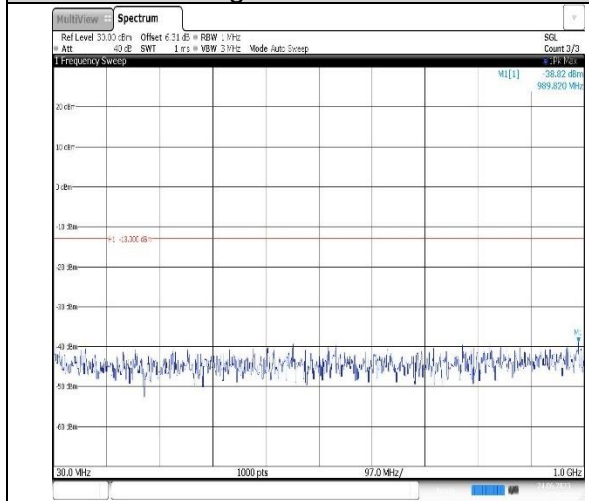
Band2-10MHz-QPSK-18650-1RB#0-Range1:30~1000MHz
