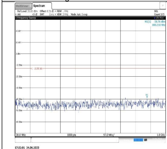
Band2-3MHz-16QAM-19185-1RB#0- Range1:30~1000MHz
