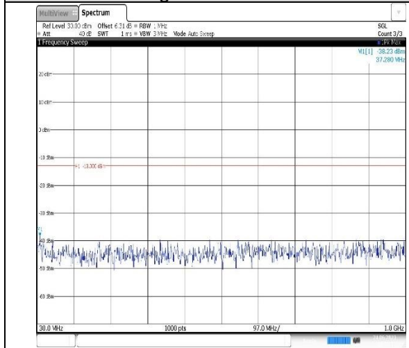
Band2-15MHz-QPSK-18675-1RB#0-Range1:30~1000MHz
