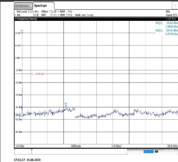
Band2-3MHz-16QAM-18615-1RB#0- Range2:1000~20000MHz
