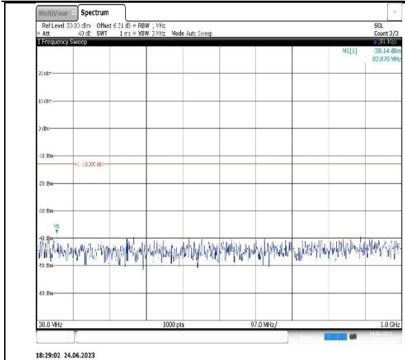
Band2-10MHz-16QAM-18650-1RB#0- Range1:30~1000MHz
