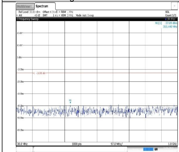
Band2-3MHz-QPSK-19185-1RB#0-Range1:30~1000MHz
