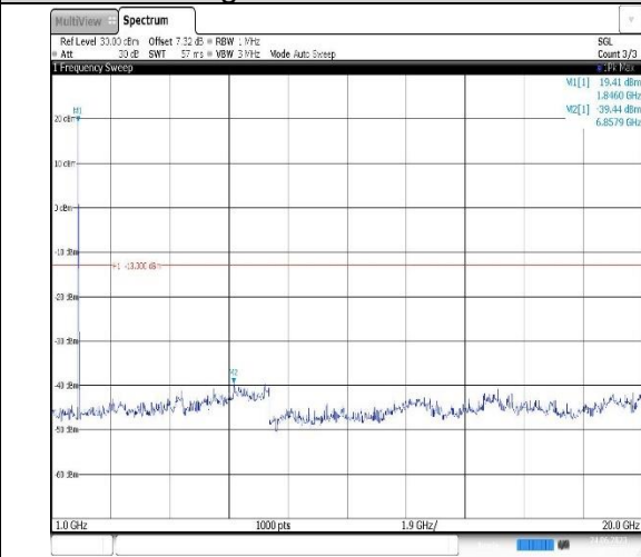
Band2-15MHz-QPSK-18675-1RB#0-Range2:1000~20000MHz
