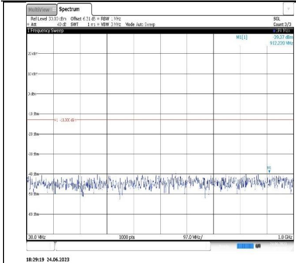
Band2-15MHz-QPSK-18675-1RB#0-Range1:30~1000MHz
