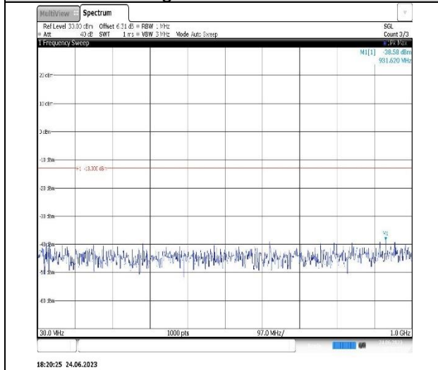
Band2-5MHz-16QAM-18900-1RB#0-Range1:30~1000MHz
