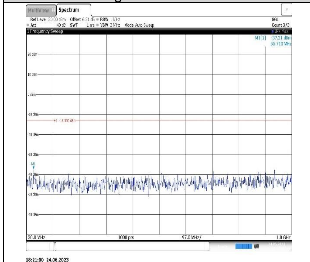
Band2-5MHz-16QAM-19175-1RB#0-Range1:30~1000MHz
