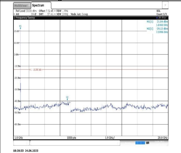
Band2-5MHz-16QAM-18900-1RB#0-Range2:1000~20000MHz
