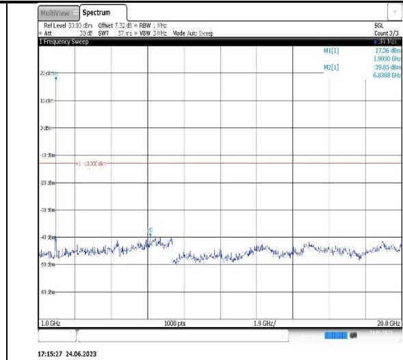
Band2-1.4MHz-16QAM-18607-1RB#0-Range2:1000~20000MHz
