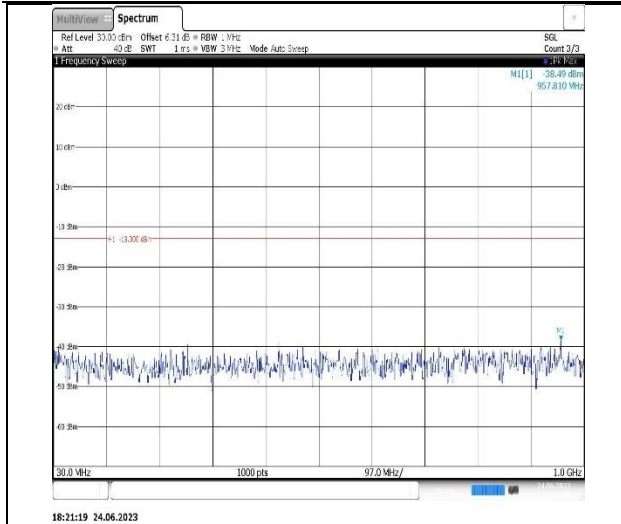
Band2-5MHz-16QAM-18625-1RB#0-Range1:30~1000MHz
