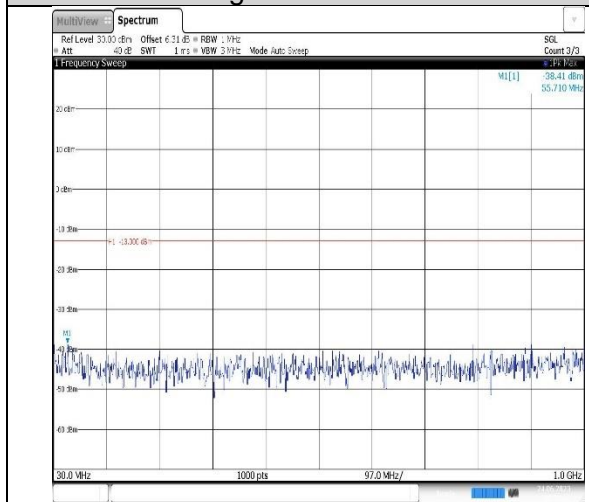
Band2-10MHz-16QAM-19150-1RB#0- Range1:30~1000MHz
