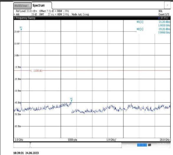
Band2-15MHz-16QAM-18675-1RB#0- Range2:1000~20000MHz
