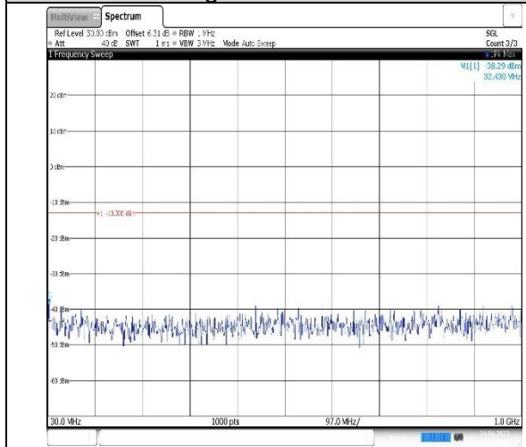
Band2-3MHz-QPSK-18615-1RB#0-Range1:30~1000MHz
