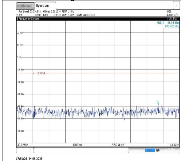
Band2-3MHz-16QAM-18900-1RB#0- Range1:30~1000MHz
