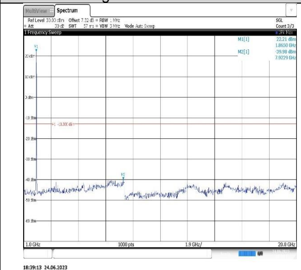
Band2-15MHz-16QAM-19125-1RB#0- Range2:1000~20000MHz
