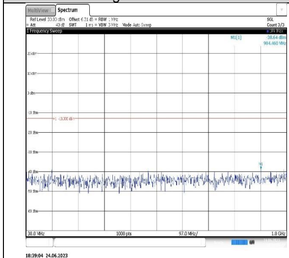
Band2-15MHz-16QAM-19125-1RB#0- Range1:30~1000MHz
