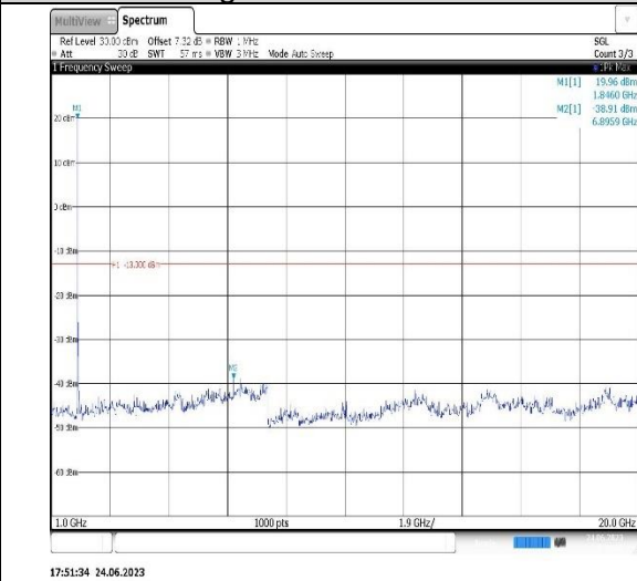
Band2-3MHz-16QAM-18900-1RB#0- Range2:1000~20000MHz
