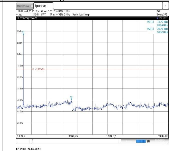
Band2-1.4MHz-16QAM-19193-1RB#0-Range2:1000~20000MHz
