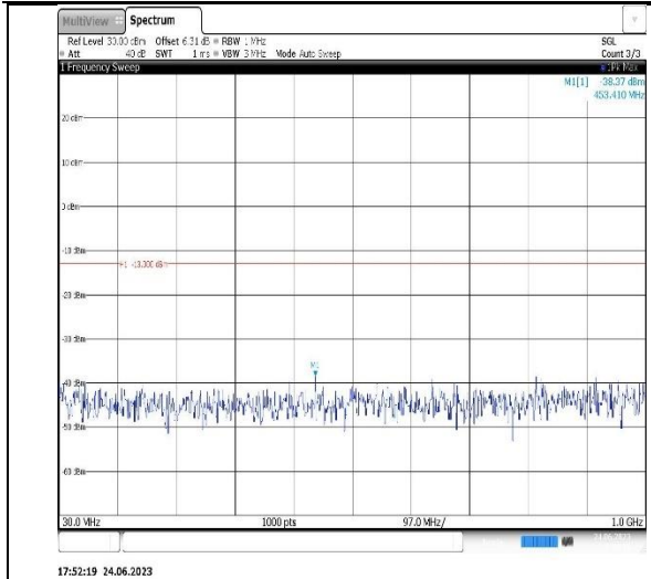
Band2-3MHz-16QAM-18615-1RB#0- Range1:30~1000MHz
