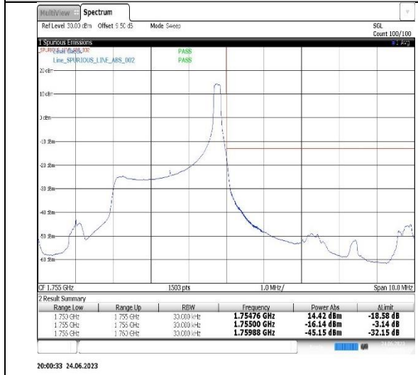
Band4-3MHz-QPSK-20385-15RB#0
