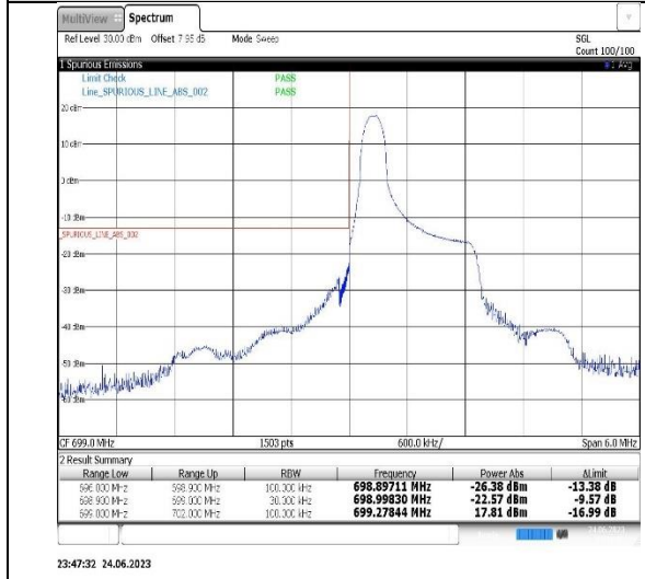
Band12-1.4MHz-QPSK-23017-1RB#0
