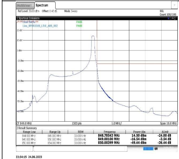
Band5-3MHz-16QAM-20635-15RB#0
