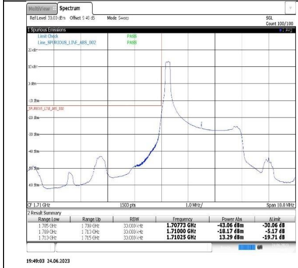
Band4-3MHz-16QAM-19965-1RB#0
