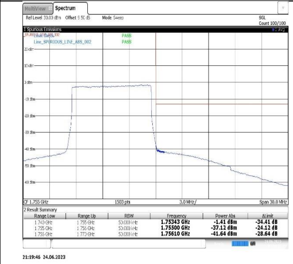
Band4-15MHz-QPSK-20025-75RB#0
