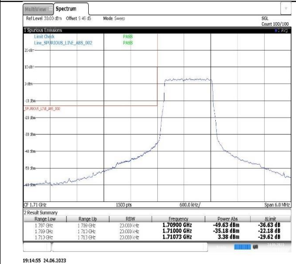
Band4-1.4MHz-16QAM-20393-6RB#0
