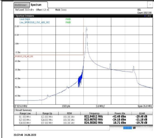
Band5-10MHz-16QAM-20450-1RB#0
