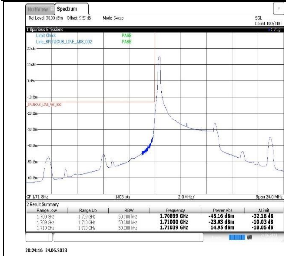
Band4-5MHz-16QAM-20375-1RB#24
