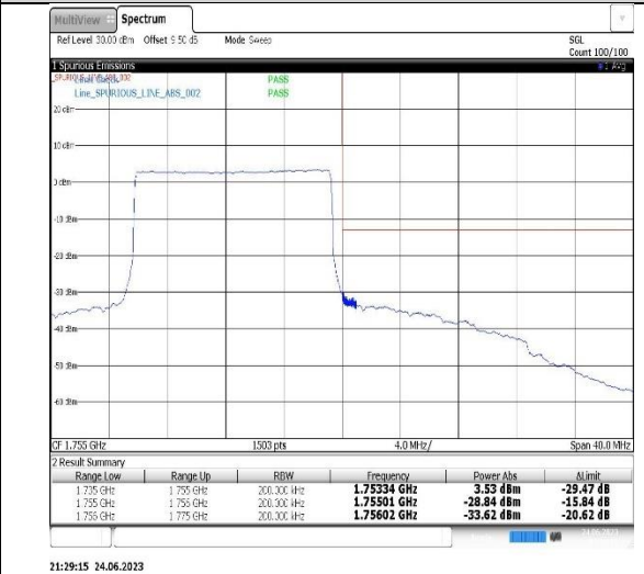
Band4-15MHz-QPSK-20325-75RB#0
