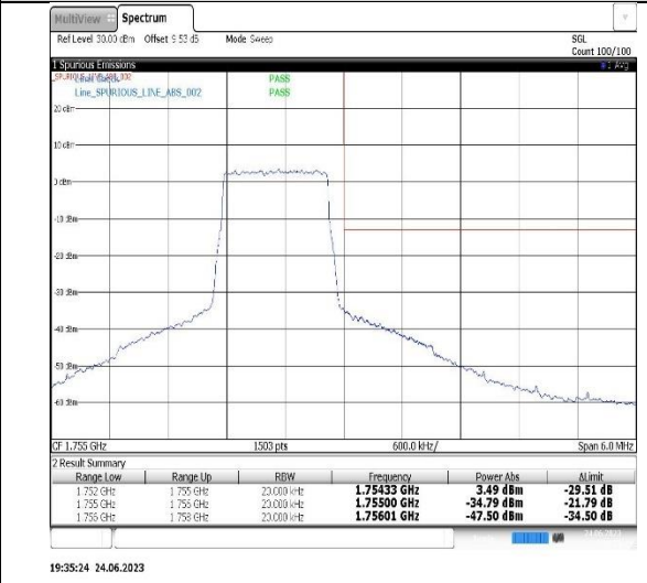
Band4-3MHz-QPSK-19965-15RB#0
