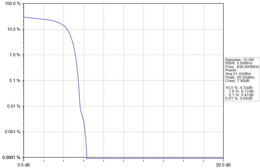
Band5_HSDPA_MCH_836.6MHz_Subtest 1_NTNV
