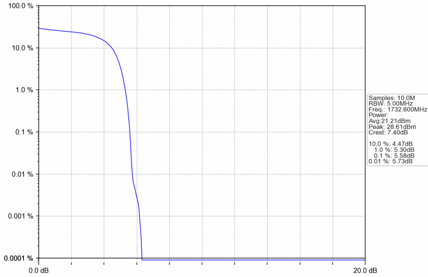
Band4_HSDPA_MCH_1732.6MHz_Subtest 1_NTNV
