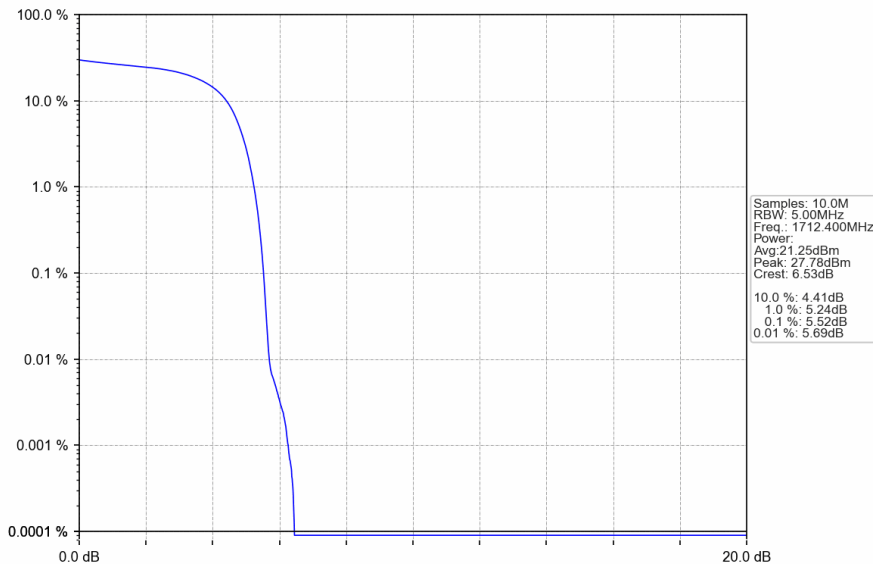
Band4_HSDPA_LCH_1712.4MHz_Subtest 1_NTNV
