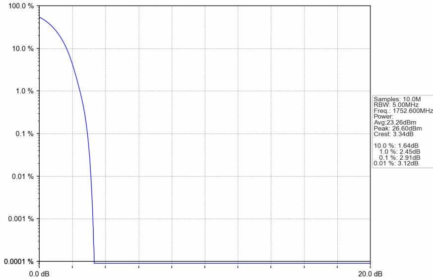
Band4_RMC_HCH_1752.6MHz_12.2kbps RMC_NTNV
