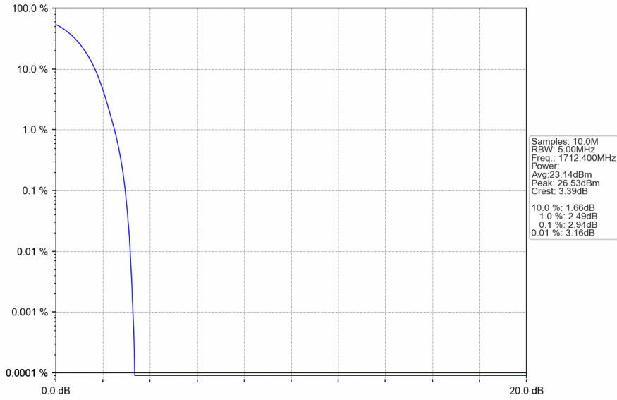
Band4_RMC_LCH_1712.4MHz_12.2kbps RMC_NTNV
