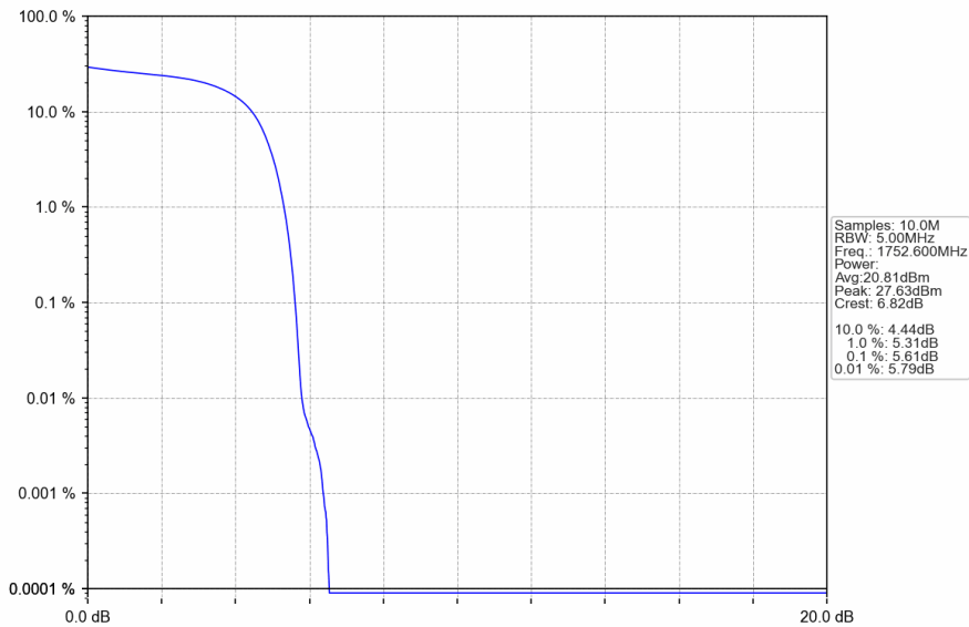
Band4_HSDPA_HCH_1752.6MHz_Subtest 1_NTNV
