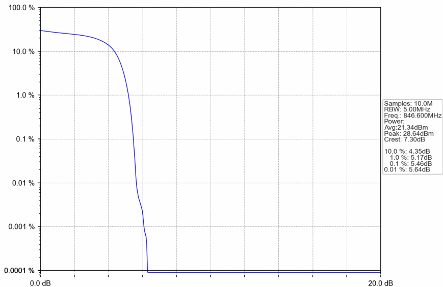
Band5_HSDPA_HCH_846.6MHz_Subtest 1_NTNV
