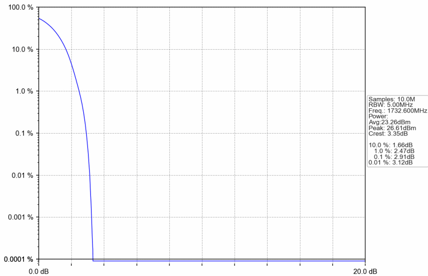
Band4_RMC_MCH_1732.6MHz_12.2kbps RMC_NTNV
