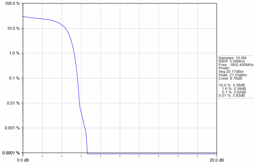
Band2_HSUPA_LCH_1852.4MHz_Subtest 1_NTNV
