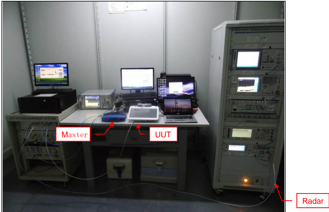
Set UUT as Client mode (Radar injected into Master)
