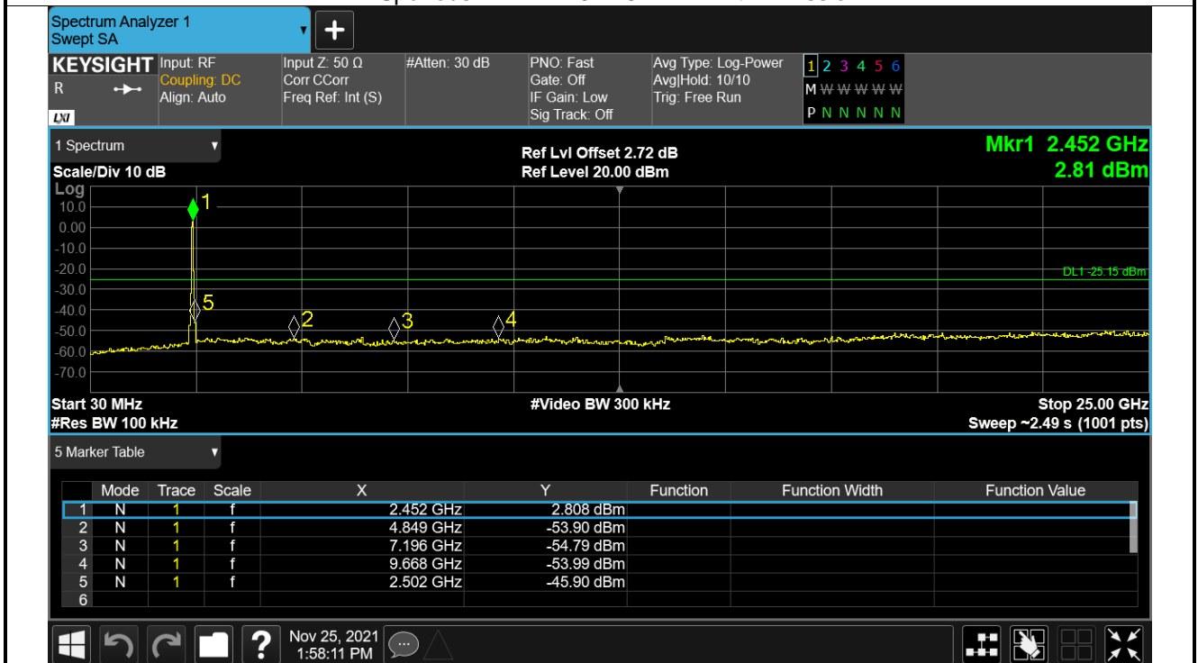
Tx. Spurious NVNT n40 2452MHz Ant1 Ref
