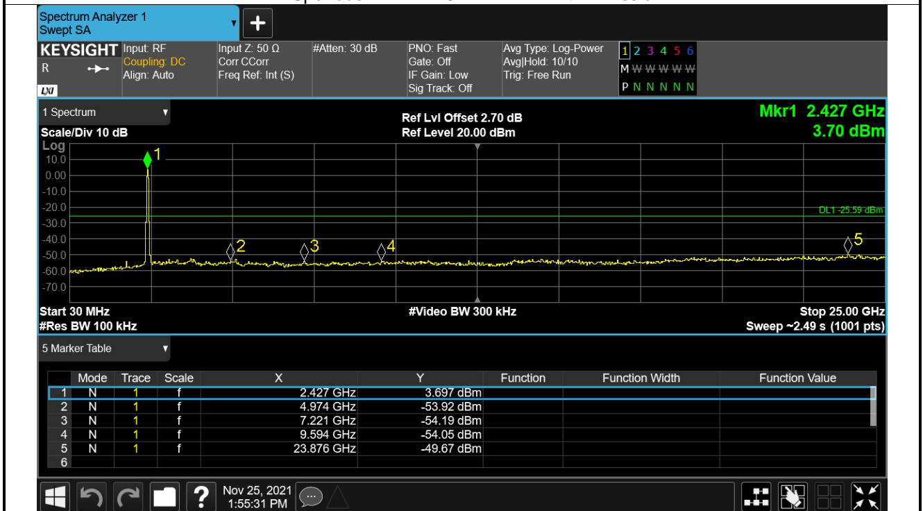
Tx. Spurious NVNT n40 2437MHz Ant1 Ref
