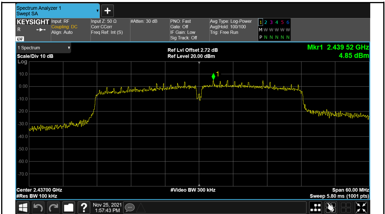
Tx. Spurious NVNT n40 2437MHz Ant1 Emission
