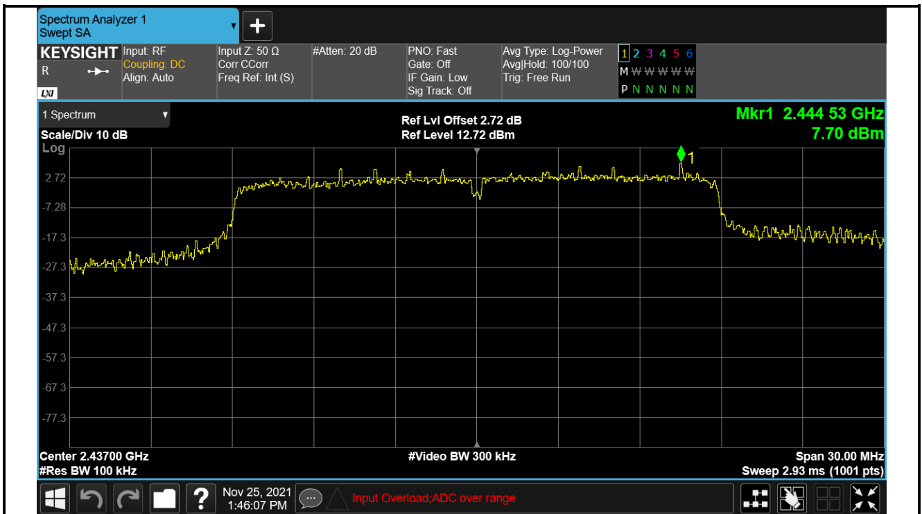
Tx. Spurious NVNT n20 2437MHz Ant1 Emission
