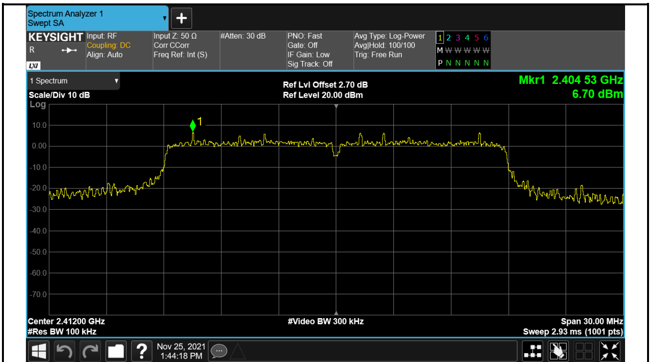
Tx. Spurious NVNT n20 2412MHz Ant1 Emission
