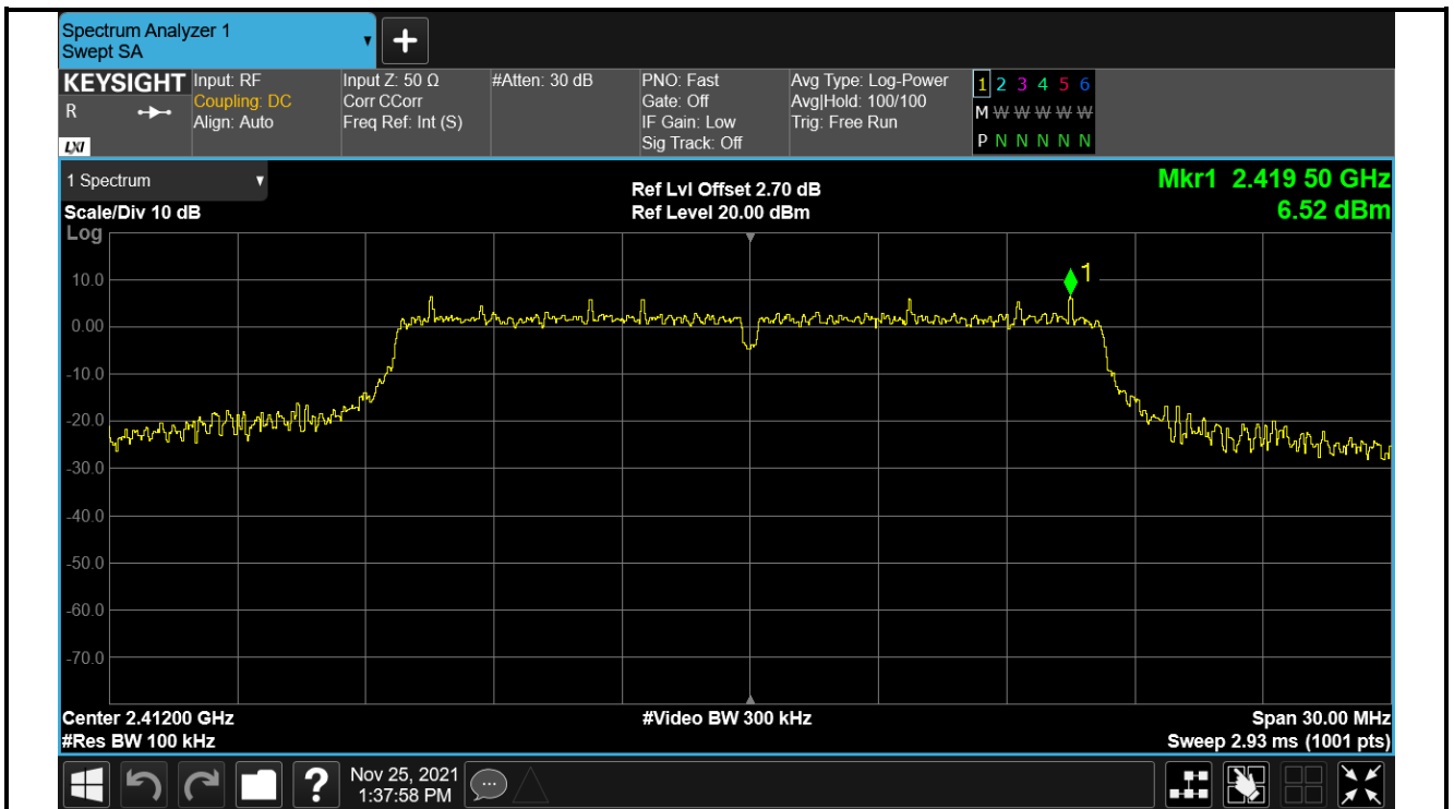
Band Edge NVNT g 2412MHz Ant1 Emission
