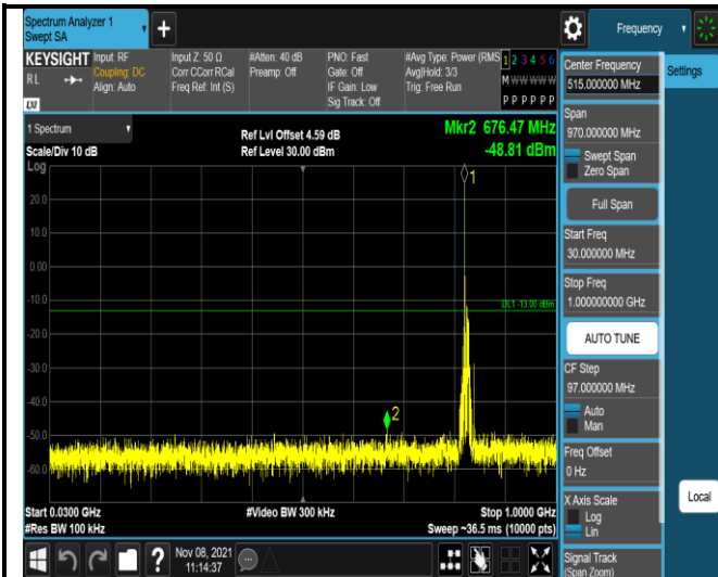
Band5-10MHz-16QAM-20450-1RB#0- Range1:30~1000MHz
