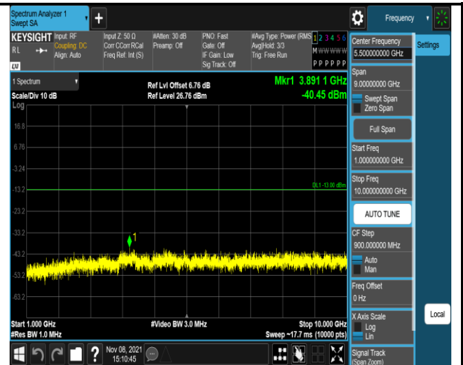
Band13-10MHz-QPSK-23230-1RB#0- Range2:1000~10000MHz
