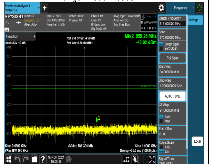
Band13-5MHz-16QAM-23205-1RB#0- Range1:30~1000MHz
