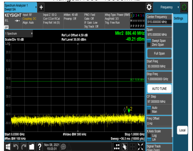
Band13-5MHz-16QAM-23255-1RB#0- Range1:30~1000MHz
