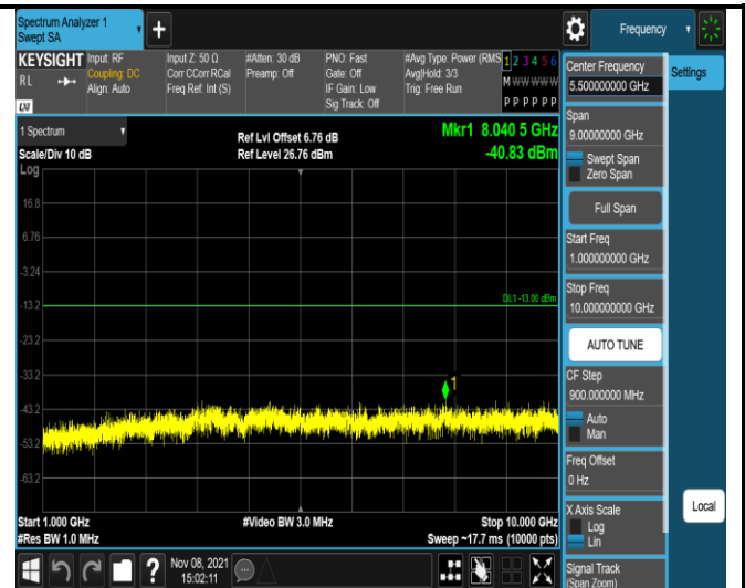
Band13-5MHz-16QAM-23230-1RB#0- Range2:1000~10000MHz
