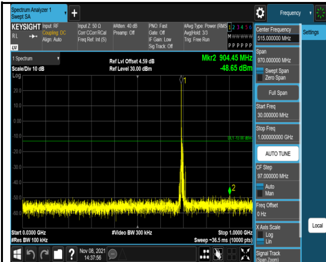
Band12-10MHz-16QAM-23060-1RB#0- Range1:30~1000MHz
