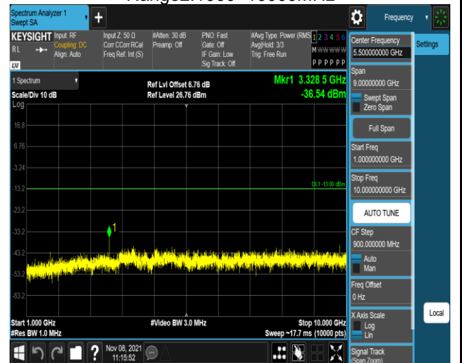
Band5-10MHz-16QAM-20525-1RB#0- Range2:1000~10000MHz
