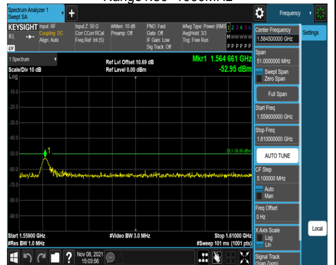
Band13-5MHz-16QAM-23255-1RB#0- Range3:1559~1610MHz
