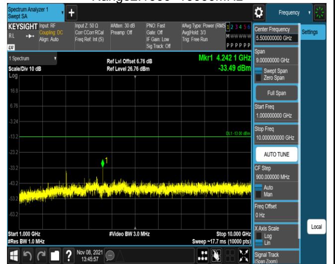
Band12-1.4MHz-16QAM-23095-1RB#0- Range2:1000~10000MHz
