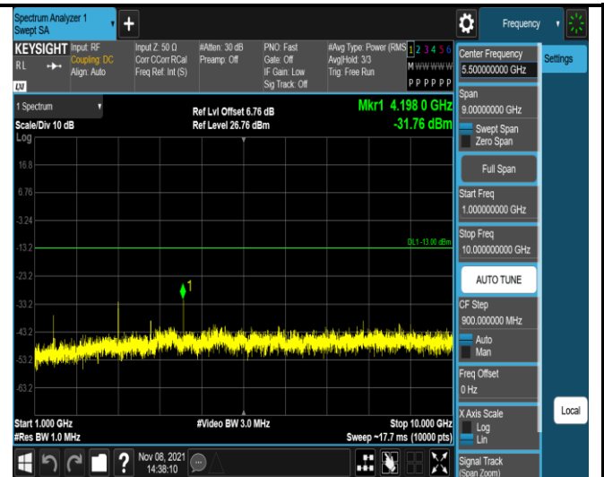
Band12-10MHz-16QAM-23060-1RB#0- Range2:1000~10000MHz
