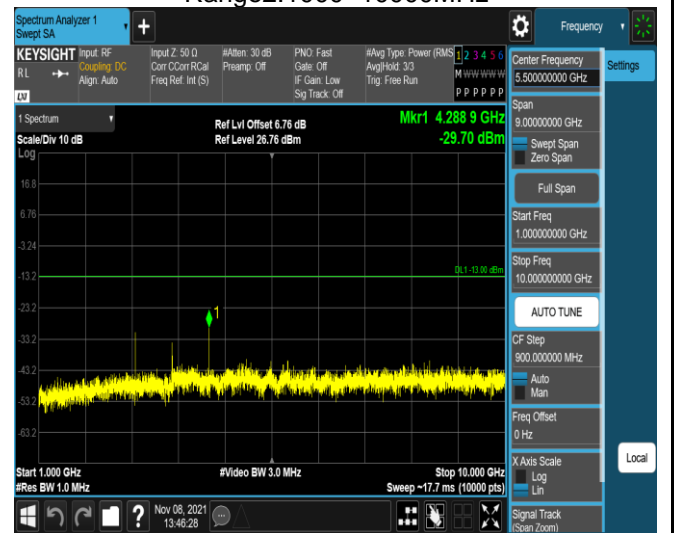
Band12-1.4MHz-QPSK-23173-1RB#0- Range2:1000~10000MHz
