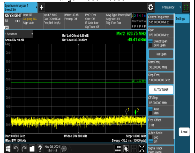
Band13-10MHz-16QAM-23230-1RB#0- Range1:30~1000MHz
