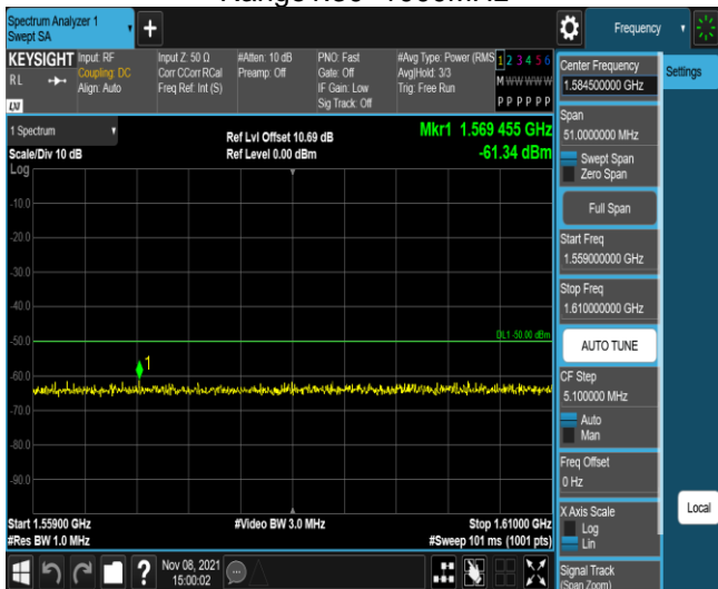
Band13-5MHz-QPSK-23205-1RB#0- Range3:1559~1610MHz
