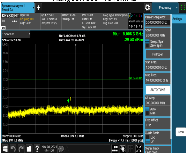
Band13-10MHz-16QAM-23230-1RB#0- Range2:1000~10000MHz
