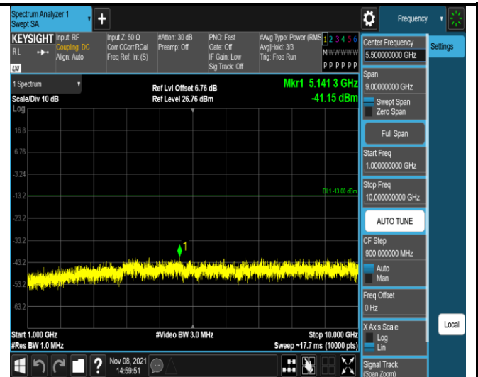
Band13-5MHz-QPSK-23205-1RB#0- Range2:1000~10000MHz
