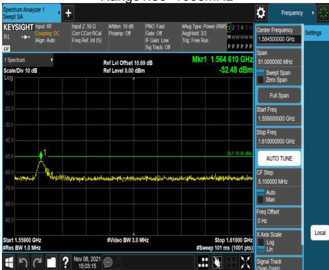
Band13-5MHz-QPSK-23255-1RB#0- Range3:1559~1610MHz
