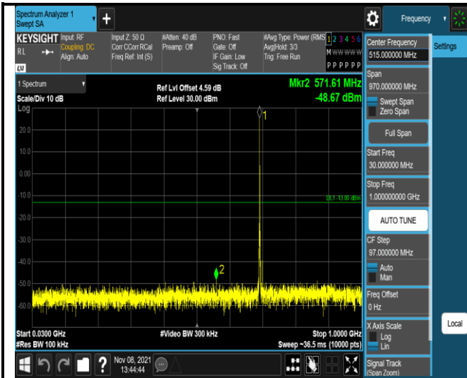
Band12-1.4MHz-16QAM-23017-1RB#0- Range1:30~1000MHz
