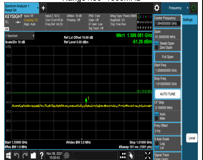
Band13-5MHz-16QAM-23205-1RB#0- Range3:1559~1610MHz
