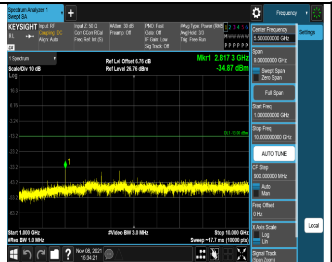
Band17-5MHz-QPSK-23755-1RB#0- Range2:1000~10000MHz
