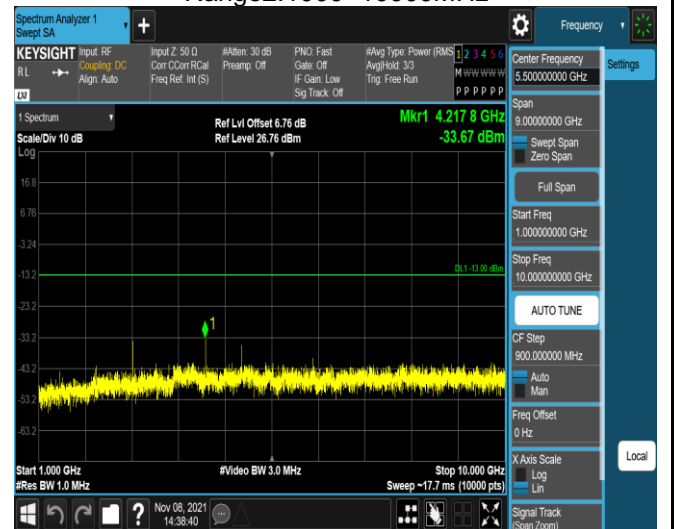
Band12-10MHz-QPSK-23095-1RB#0- Range2:1000~10000MHz
