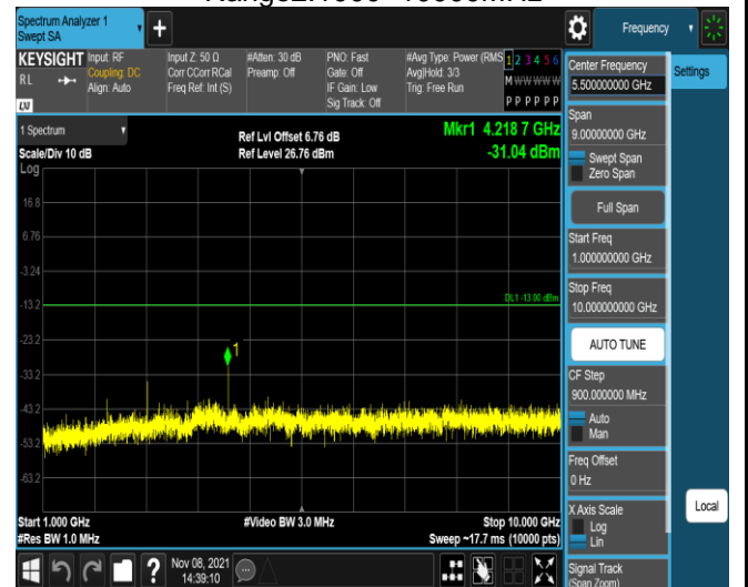
Band12-10MHz-16QAM-23095-1RB#0- Range2:1000~10000MHz
