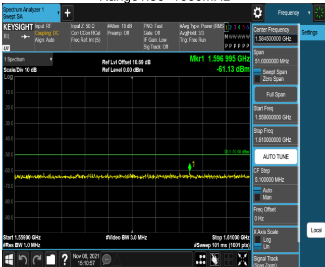
Band13-10MHz-QPSK-23230-1RB#0- Range3:1559~1610MHz
