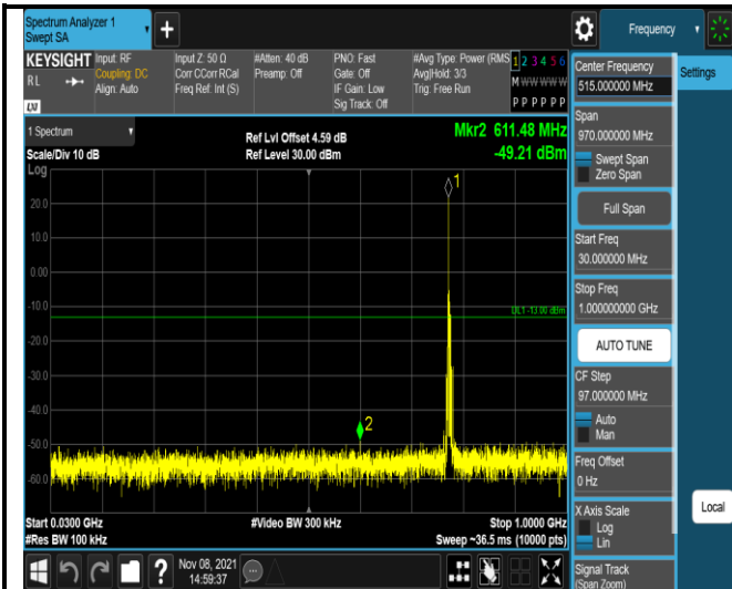
Band13-5MHz-QPSK-23205-1RB#0- Range1:30~1000MHz
