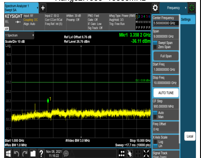
Band5-10MHz-QPSK-20600-1RB#0- Range2:1000~10000MHz
