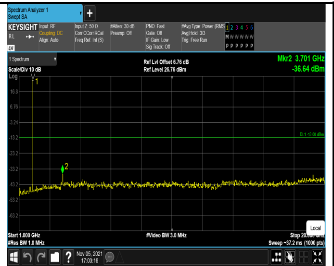
Band2-1.4MHz-16QAM-18607-1RB#0- Range2:1000~20000MHz
