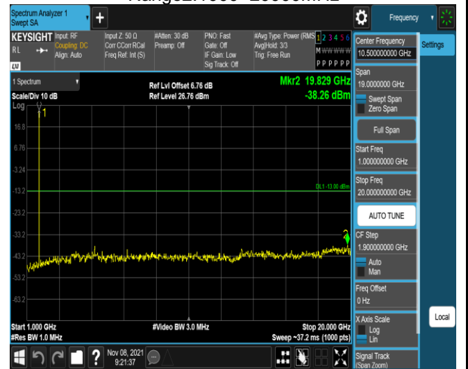
Band4-1.4MHz-16QAM-20175-1RB#0- Range2:1000~20000MHz
