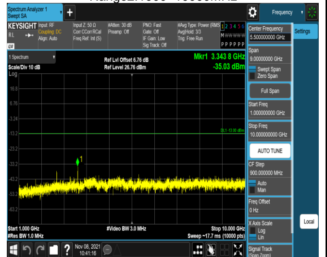
Band5-1.4MHz-QPSK-20525-1RB#0- Range2:1000~10000MHz
