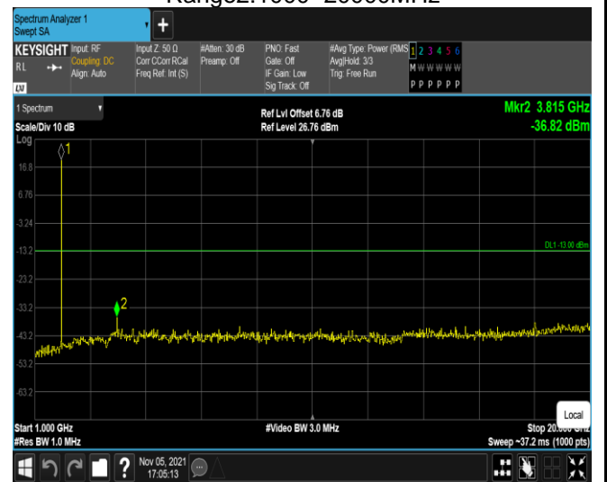
Band2-1.4MHz-16QAM-19193-1RB#0- Range2:1000~20000MHz
