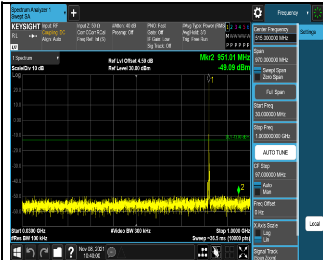
Band5-1.4MHz-QPSK-20407-1RB#0- Range1:30~1000MHz
