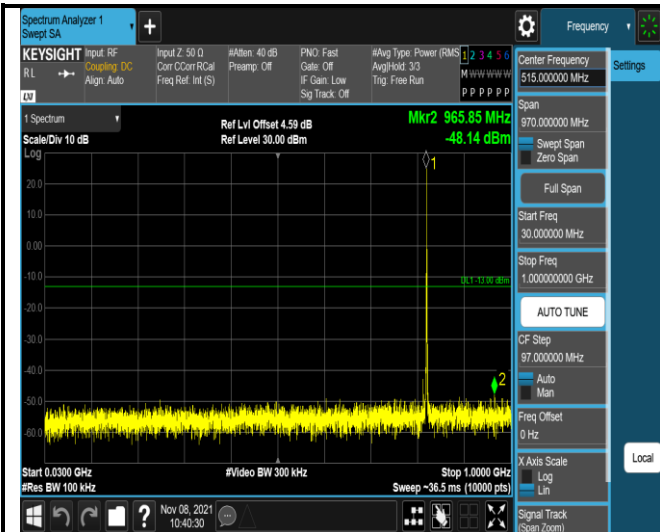
Band5-1.4MHz-16QAM-20407-1RB#0- Range1:30~1000MHz
