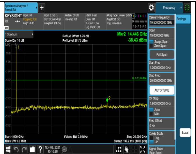
Band4-20MHz-16QAM-20050-1RB#0- Range2:1000~20000MHz
