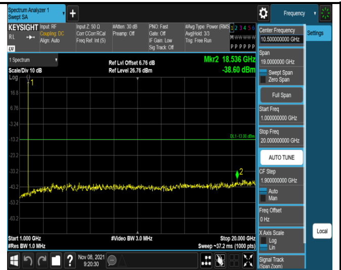
Band4-1.4MHz-16QAM-19957-1RB#0- Range2:1000~20000MHz
