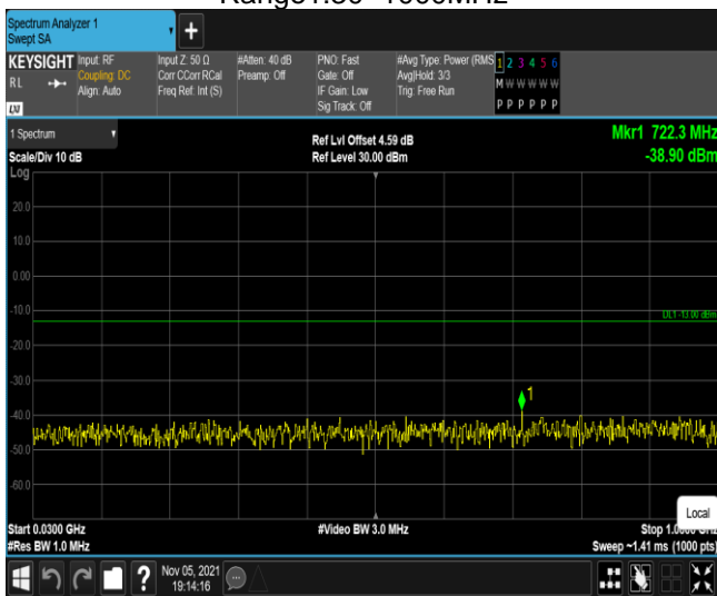
Band2-20MHz-QPSK-19100-1RB#0-Range1:30~1000MHz
