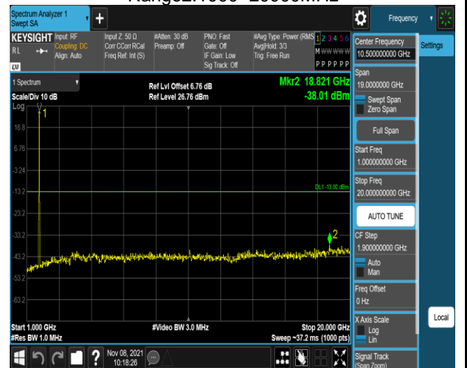
Band4-20MHz-16QAM-20300-1RB#0- Range2:1000~20000MHz
