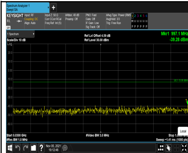
Band2-20MHz-16QAM-18700-1RB#0- Range1:30~1000MHz
