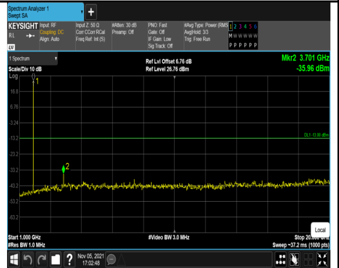
Band2-1.4MHz-QPSK-18607-1RB#0- Range2:1000~20000MHz
