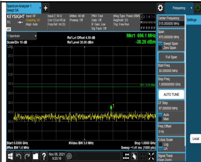
Band4-1.4MHz-16QAM-19957-1RB#0- Range1:30~1000MHz
