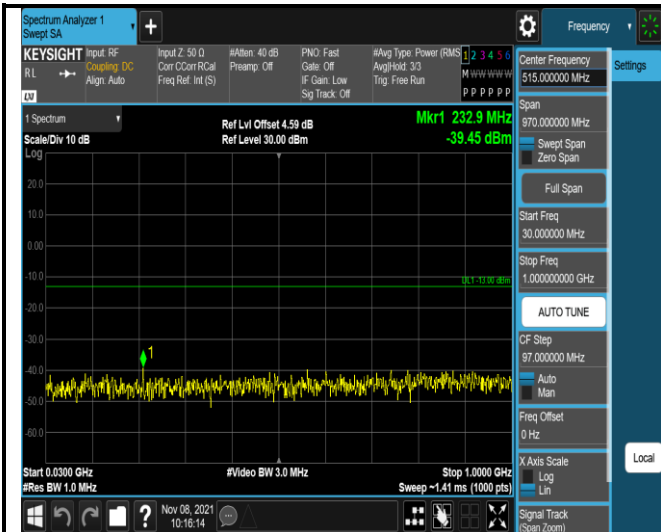
Band4-20MHz-16QAM-20050-1RB#0- Range1:30~1000MHz
