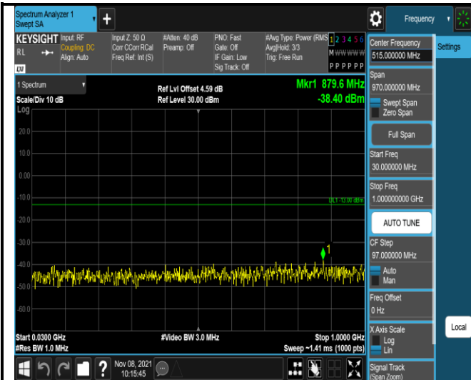
Band4-20MHz-QPSK-20050-1RB#0- Range1:30~1000MHz
