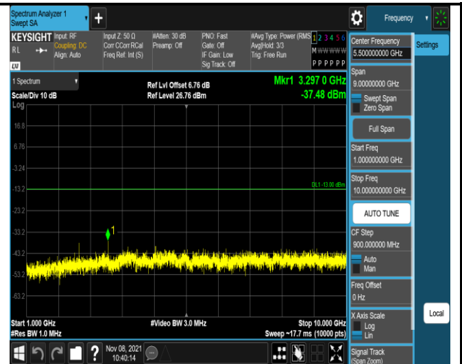
Band5-1.4MHz-QPSK-20407-1RB#0- Range2:1000~10000MHz
