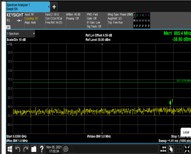
Band2-1.4MHz-QPSK-18607-1RB#0- Range1:30~1000MHz
