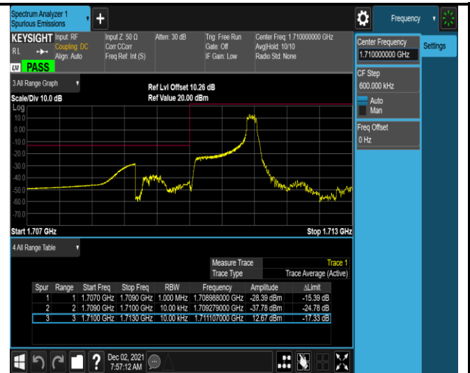
Band4-1.4MHz-QPSK-19957-1RB#5
