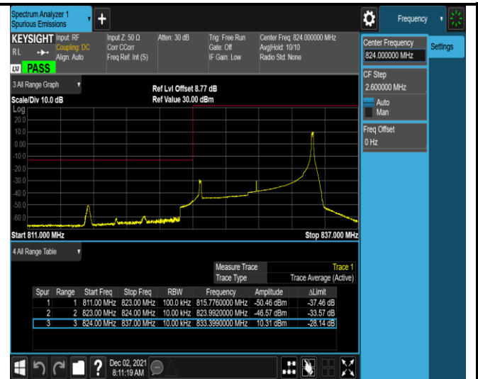
Band5-10MHz-16QAM-20450-1RB#49
