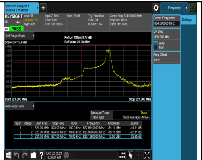
Band5-1.4MHz-QPSK-20407-1RB#5
