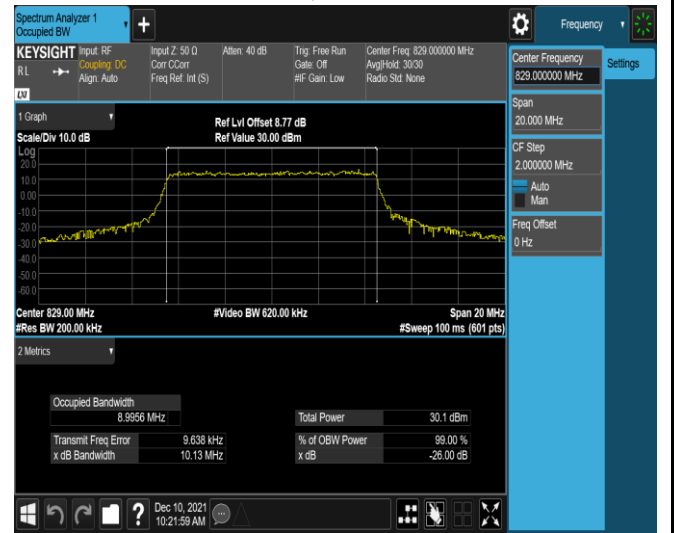
Band5-10MHz-16QAM-20450-50RB#0
