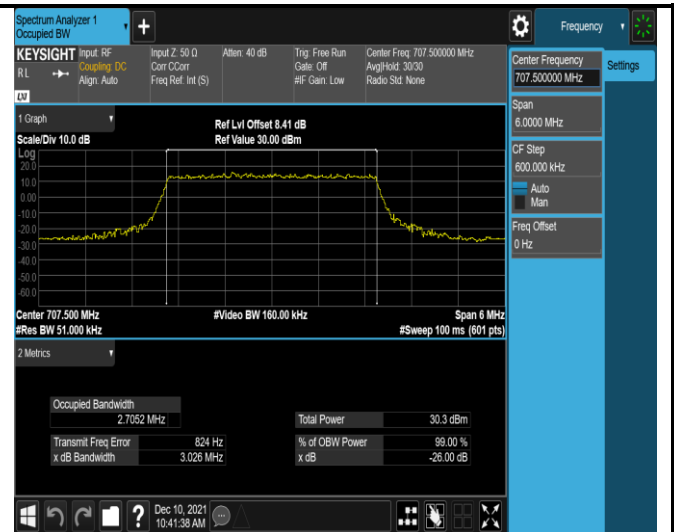
Band12-3MHz-QPSK-23095-15RB#0
