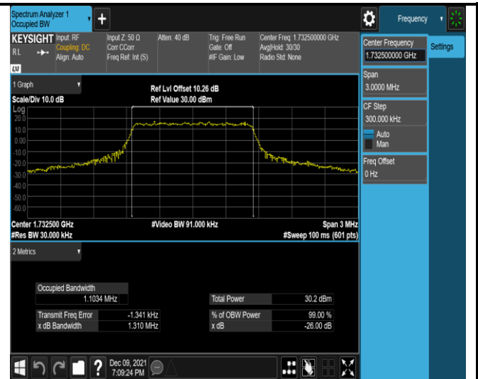
Band4-1.4MHz-QPSK-20175-6RB#0
