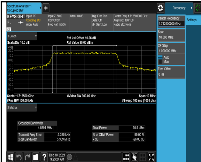
Band4-5MHz-QPSK-19975-25RB#0
