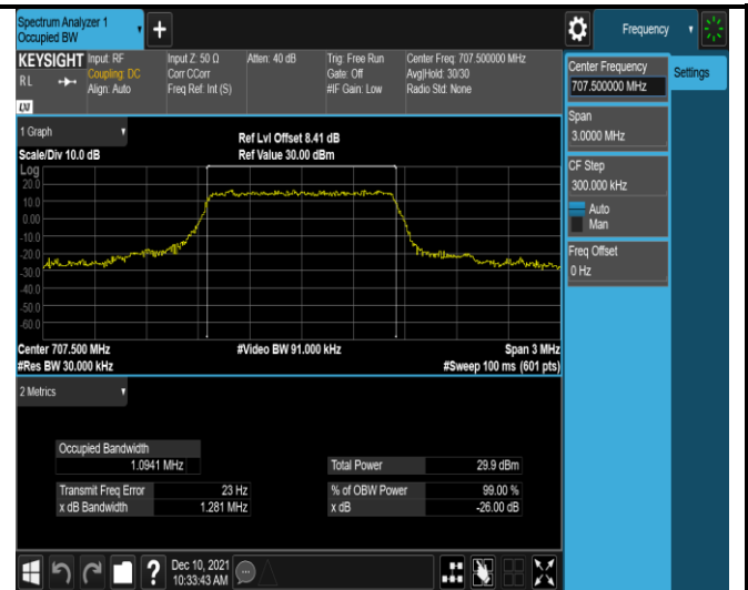
Band12-1.4MHz-QPSK-23095-6RB#0
