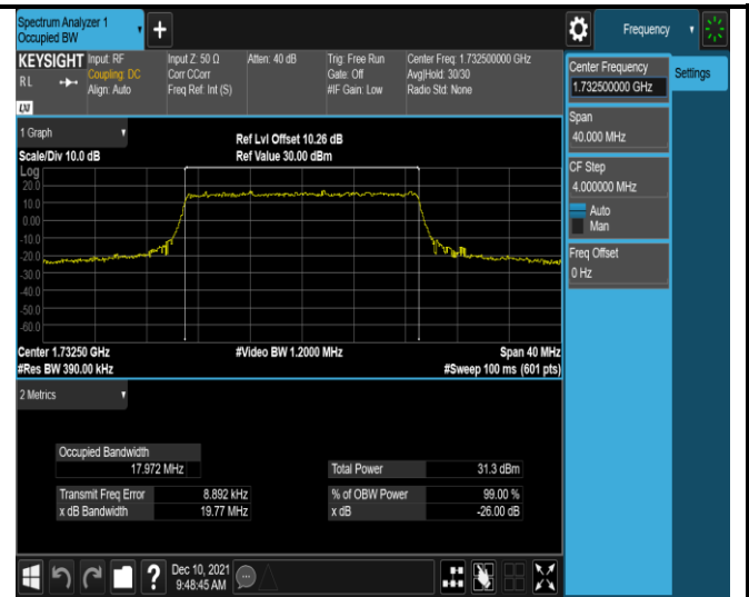
Band4-20MHz-QPSK-20175-100RB#0
