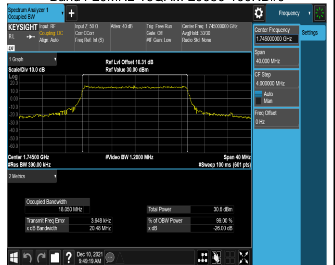
Band4-20MHz-16QAM-20300-100RB#0
