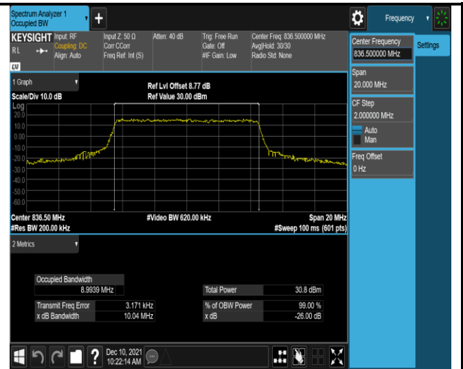
Band5-10MHz-QPSK-20525-50RB#0
