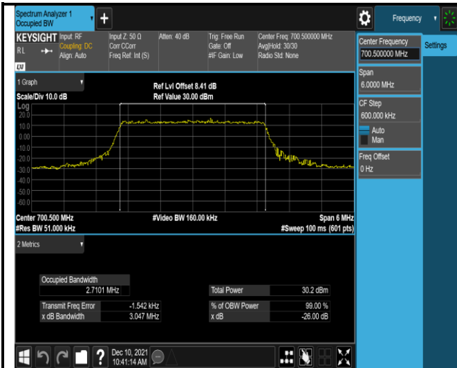
Band12-3MHz-QPSK-23025-15RB#0
