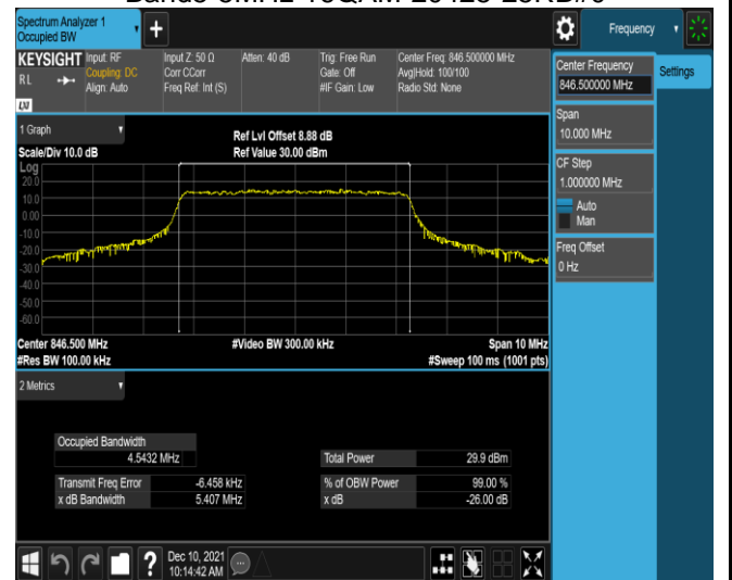
Band5-5MHz-16QAM-20625-25RB#0
