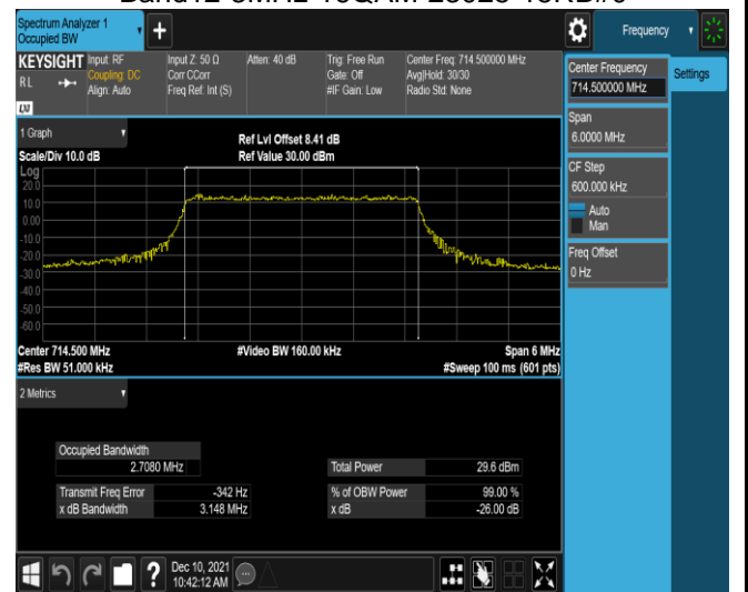
Band12-3MHz-16QAM-23165-15RB#0
