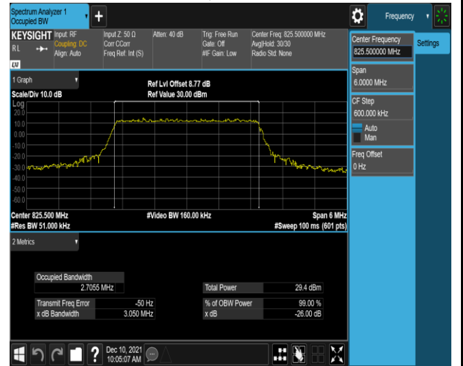
Band5-3MHz-16QAM-20415-15RB#0
