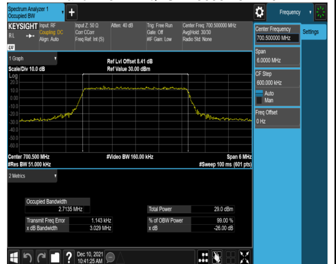
Band12-3MHz-16QAM-23025-15RB#0
