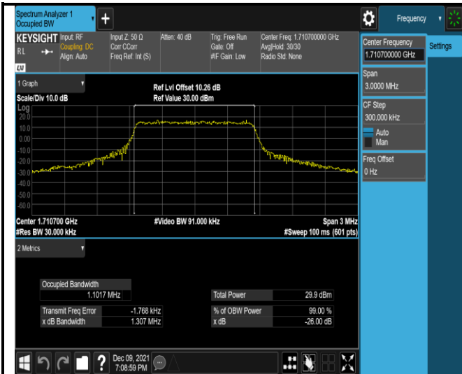
Band4-1.4MHz-QPSK-19957-6RB#0
