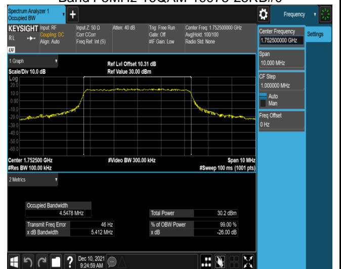
Band4-5MHz-16QAM-20375-25RB#0
