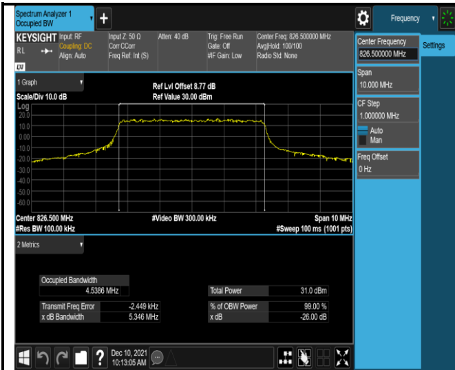
Band5-5MHz-QPSK-20425-25RB#0
