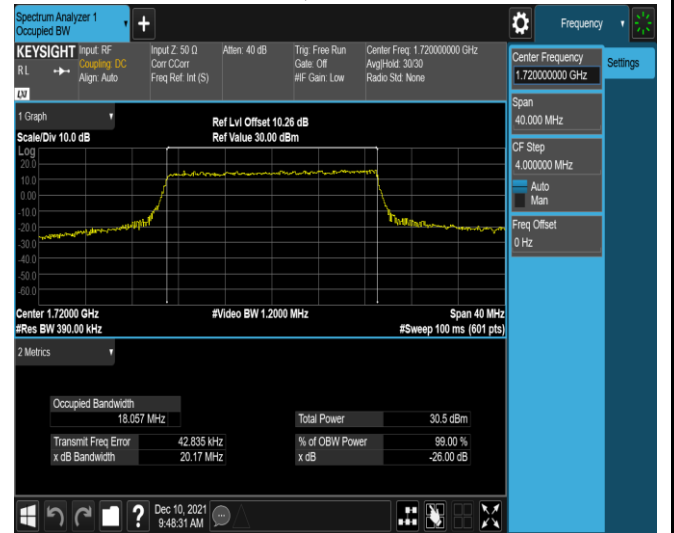
Band4-20MHz-16QAM-20050-100RB#0
