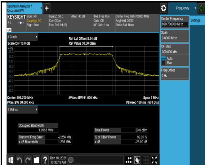
Band12-1.4MHz-QPSK-23017-6RB#0
