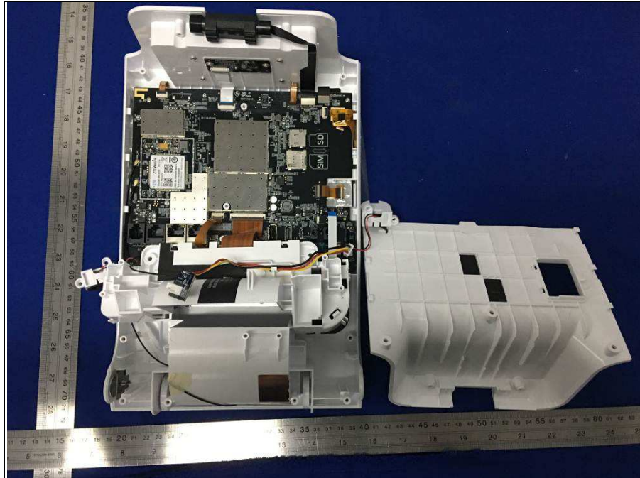
Diversity Antenna
