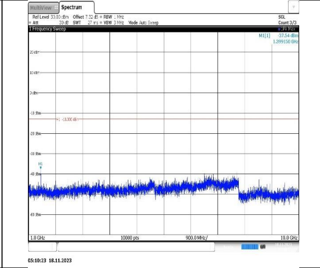
Band12-10MHz-QPSK-23095-1RB#0-Range2:1000~10000MHz
