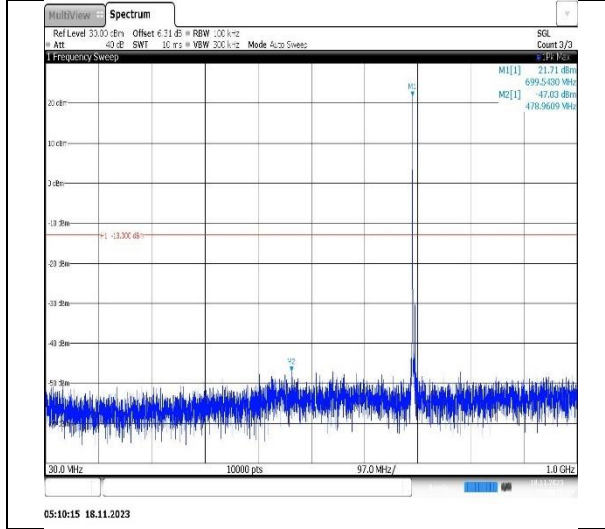
Band12-10MHz-QPSK-23095-1RB#0-Range1:30~1000MHz
