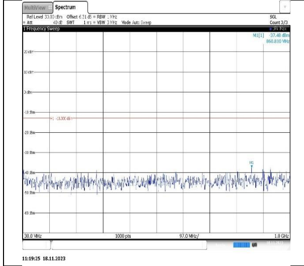
Band66-1.4MHz-QPSK-132322-1RB#0-Range1:30~1000MHz
