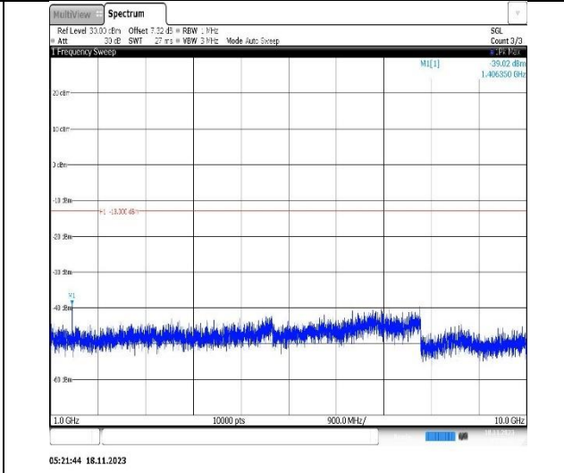
Band12-10MHz-QPSK-23130-1RB#0-Range2:1000~10000MHz
