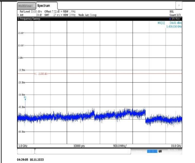
Band12-5MHz-QPSK-23035-1RB#0-Range2:1000~10000MHz
