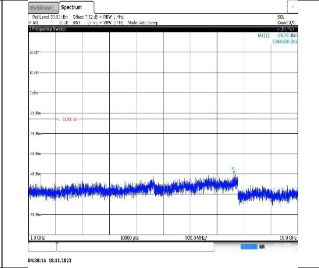
Band12-5MHz-QPSK-23095-1RB#0-Range2:1000~10000MHz
