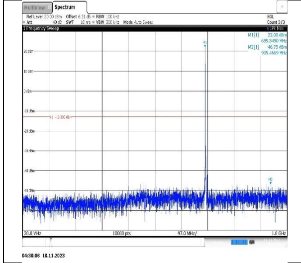
Band12-5MHz-QPSK-23095-1RB#0-Range1:30~1000MHz
