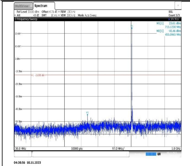
Band12-5MHz-QPSK-23035-1RB#0-Range1:30~1000MHz
