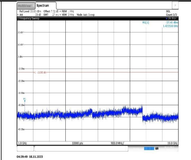
Band12-10MHz-QPSK-23060-1RB#0-Range2:1000~10000MHz
