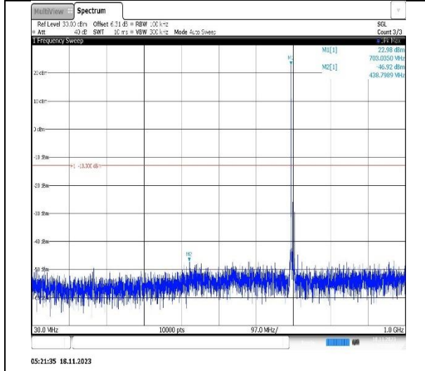
Band12-10MHz-QPSK-23130-1RB#0-Range1:30~1000MHz
