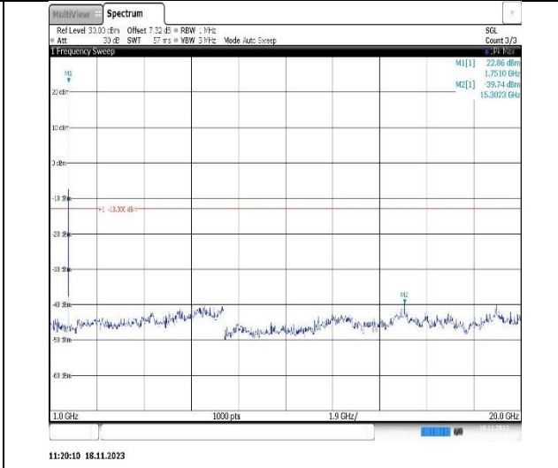
Band66-1.4MHz-QPSK-132665-1RB#0-Range2:1000~20000MHz
