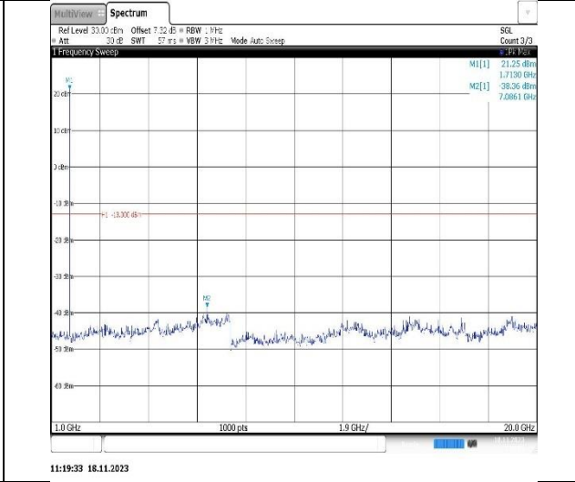
Band66-1.4MHz-QPSK-132322-1RB#0-Range2:1000~20000MHz
