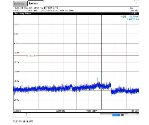
Band5-5MHz-QPSK-20525-1RB#0-Range2:1000~10000MHz
