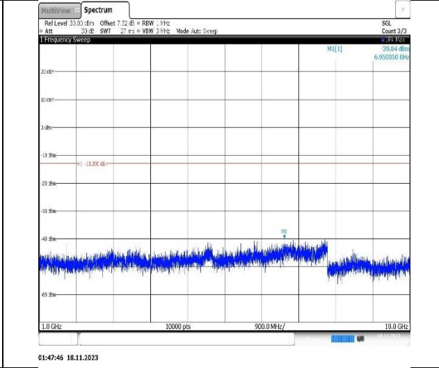
Band5-1.4MHz-16QAM-20525-1RB#0-Range2:1000~10000MHz
