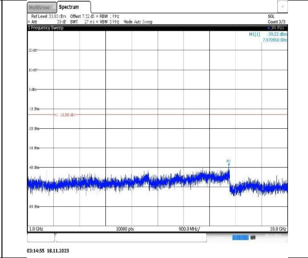
Band5-10MHz-QPSK-20525-1RB#0-Range2:1000~10000MHz
