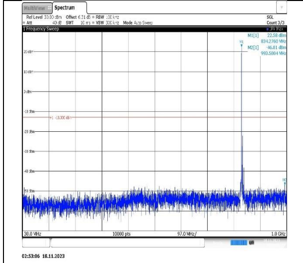
Band5-5MHz-QPSK-20625-1RB#0-Range1:30~1000MHz
