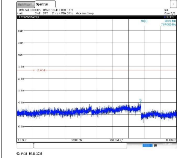
Band5-3MHz-16QAM-20525-1RB#0-Range2:1000~10000MHz
