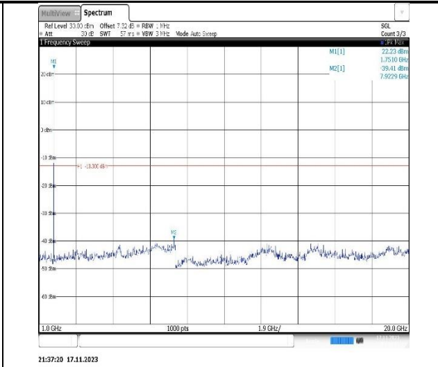
Band4-1.4MHz-16QAM-19957-1RB#0-Range2:1000~20000MHz
