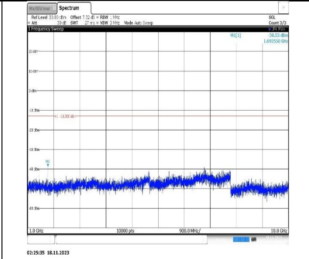
Band5-5MHz-QPSK-20425-1RB#0-Range2:1000~10000MHz
