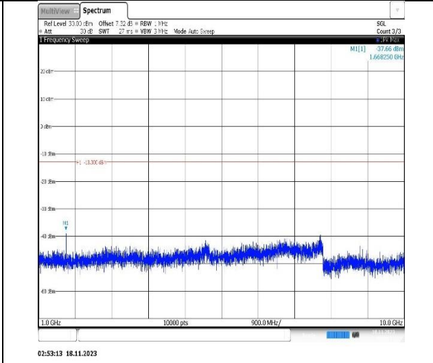
Band5-5MHz-QPSK-20625-1RB#0-Range2:1000~10000MHz
