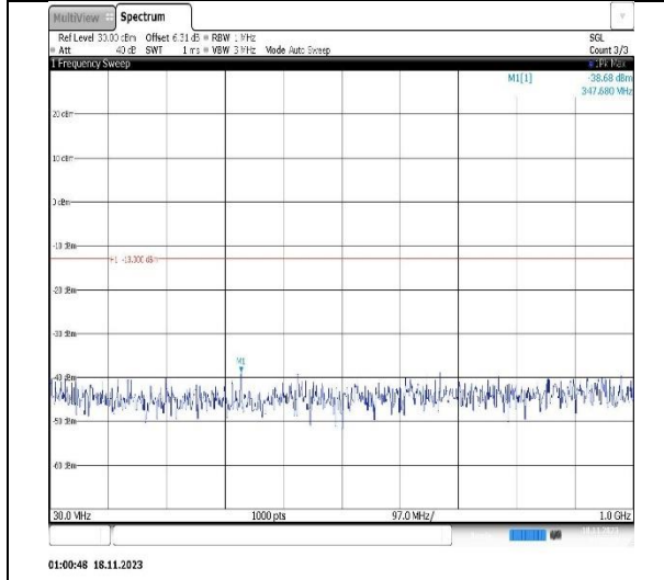
Band4-20MHz-QPSK-20300-1RB#0-Range1:30~1000MHz
