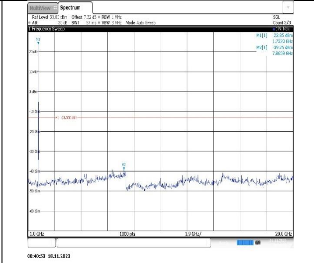
Band4-15MHz-QPSK-20325-1RB#0-Range2:1000~20000MHz
