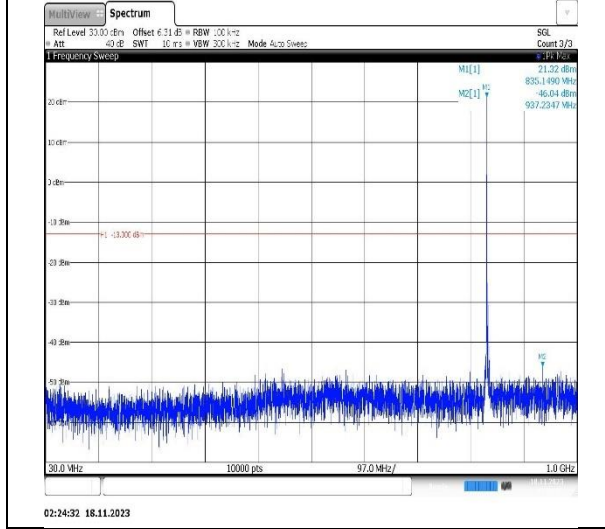
Band5-3MHz-QPSK-20635-1RB#0-Range1:30~1000MHz
