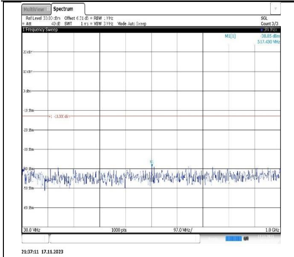
Band4-1.4MHz-16QAM-19957-1RB#0-Range1:30~1000MHz
