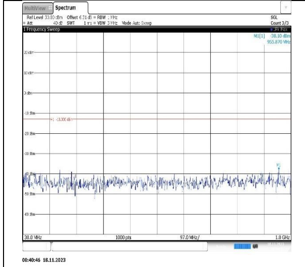
Band4-15MHz-QPSK-20325-1RB#0-Range1:30~1000MHz
