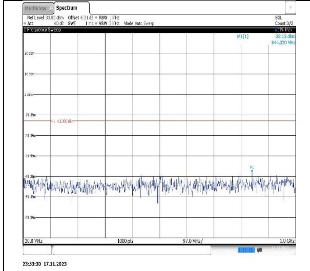
Band4-10MHz-QPSK-20350-1RB#0- Range1:30~1000MHz
