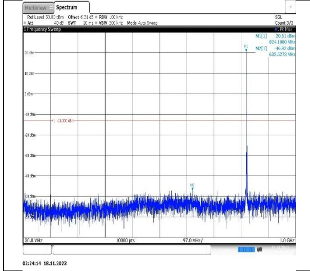
Band5-3MHz-16QAM-20525-1RB#0-Range1:30~1000MHz
