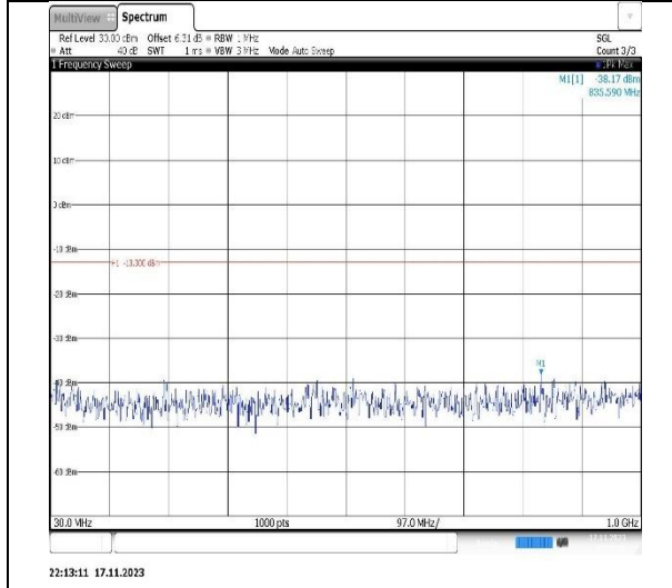
Band4-3MHz-QPSK-20385-1RB#0-Range1:30~1000MHz
