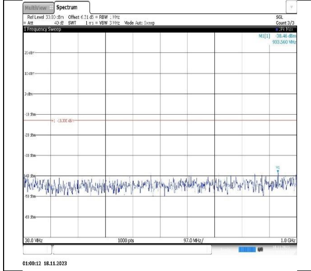
Band4-20MHz-QPSK-20175-1RB#0-Range1:30~1000MHz
