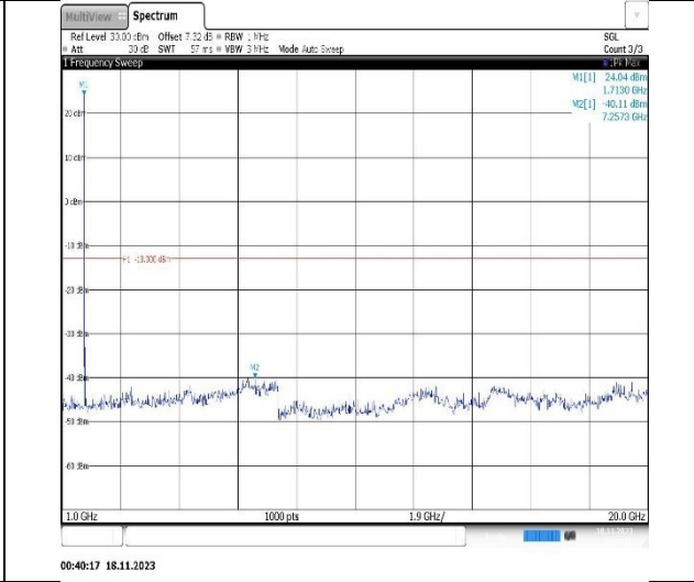
Band4-15MHz-QPSK-20175-1RB#0-Range2:1000~20000MHz
