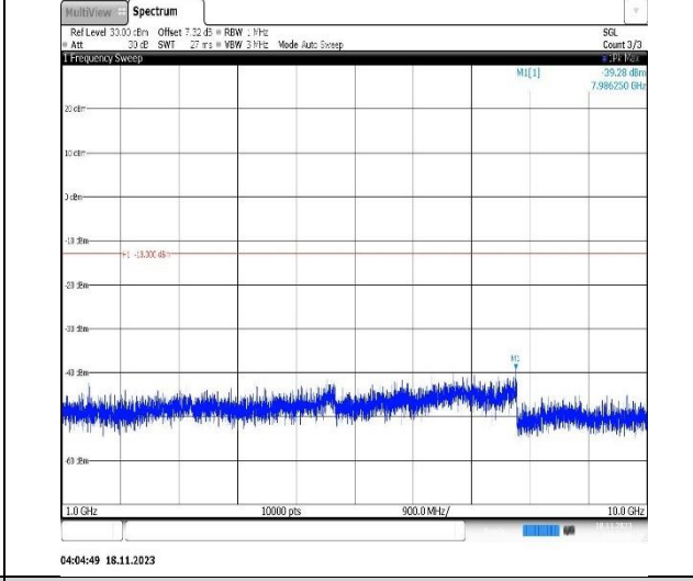
Band12-1.4MHz-QPSK-23173-1RB#0-Range2:1000~10000MHz
