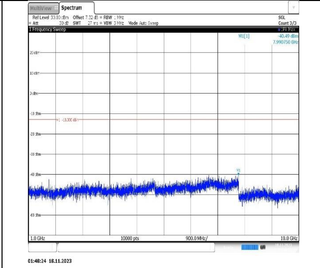
Band5-1.4MHz-16QAM-20643-1RB#0-Range2:1000~10000MHz
