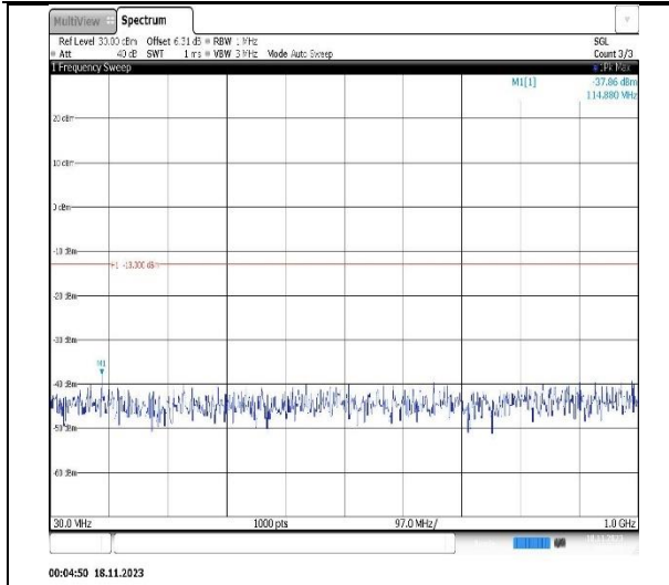
Band4-15MHz-QPSK-20025-1RB#0-Range1:30~1000MHz
