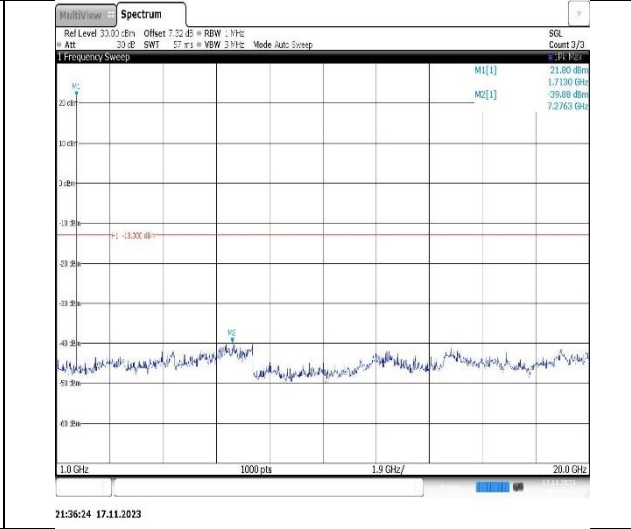
Band4-1.4MHz-16QAM-20175-1RB#0-Range2:1000~20000MHz
