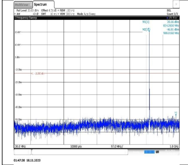
Band5-1.4MHz-16QAM-20525-1RB#0-Range1:30~1000MHz
