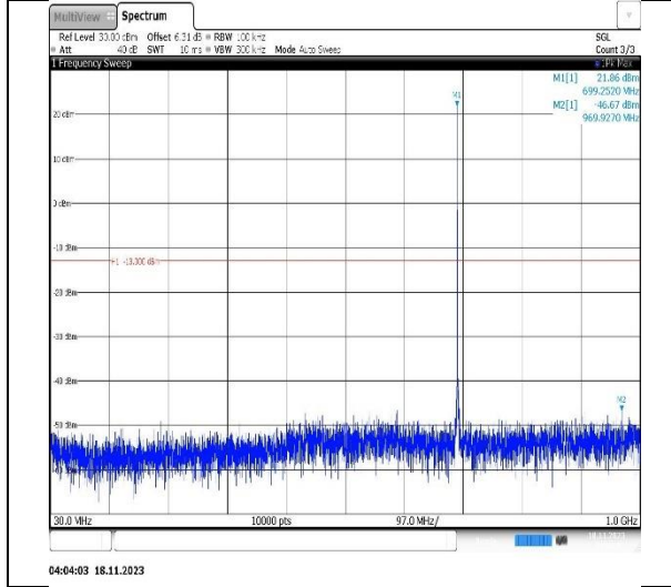
Band12-1.4MHz-QPSK-23095-1RB#0-Range1:30~1000MHz
