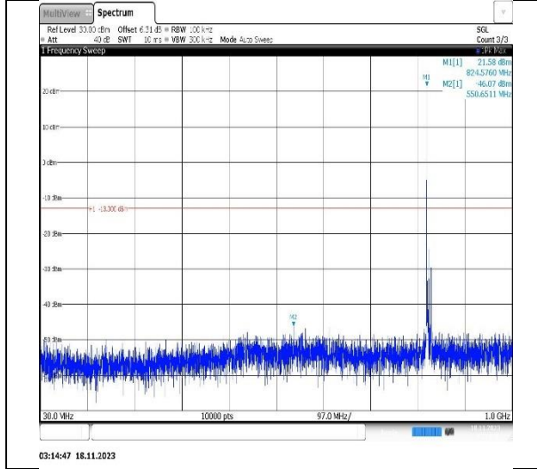
Band5-10MHz-QPSK-20525-1RB#0-Range1:30~1000MHz
