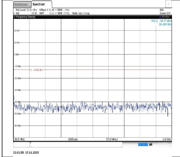
Band4-3MHz-QPSK-20175-1RB#0-Range1:30~1000MHz
