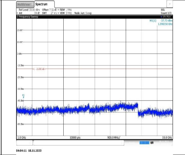
Band12-1.4MHz-QPSK-23095-1RB#0-Range2:1000~10000MHz
