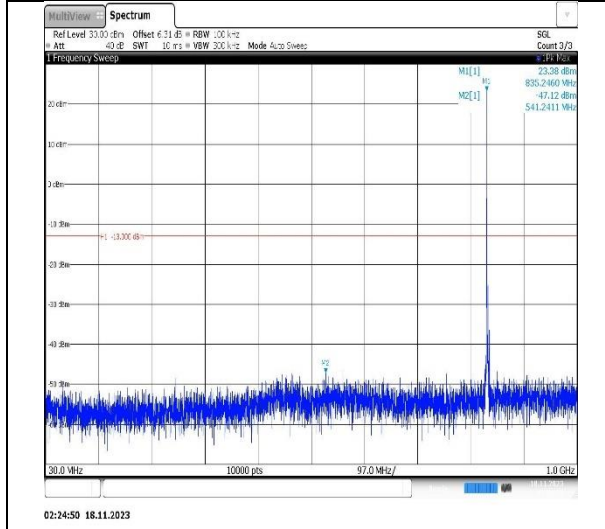
Band5-3MHz-16QAM-20635-1RB#0-Range1:30~1000MHz
