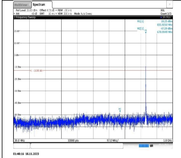
Band5-1.4MHz-16QAM-20643-1RB#0-Range1:30~1000MHz
