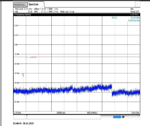
Band5-1.4MHz-16QAM-20407-1RB#0-Range2:1000~10000MHz
