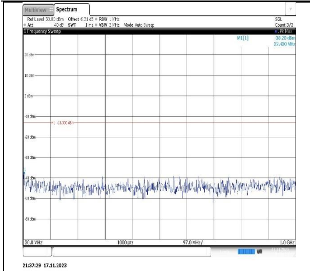
Band4-3MHz-QPSK-19965-1RB#0-Range1:30~1000MHz
