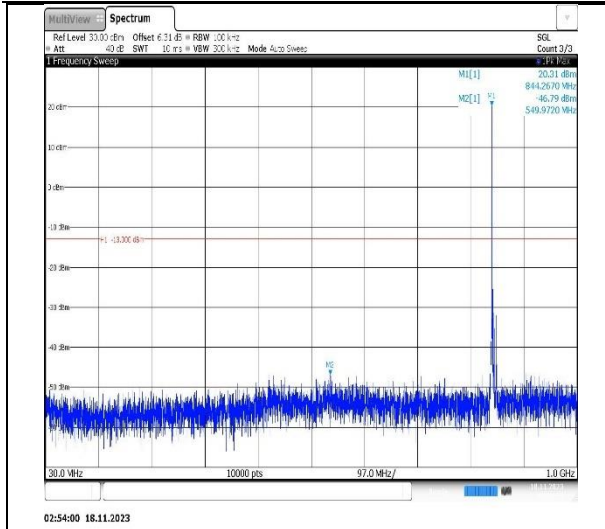
Band5-10MHz-QPSK-20450-1RB#0-Range1:30~1000MHz
