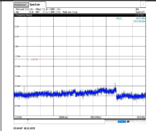
Band5-10MHz-QPSK-20450-1RB#0-Range2:1000~10000MHz
