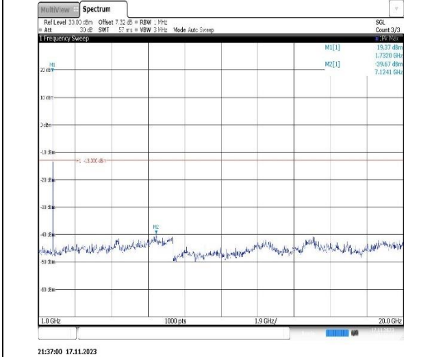
Band4-1.4MHz-16QAM-20393-1RB#0-Range2:1000~20000MHz
