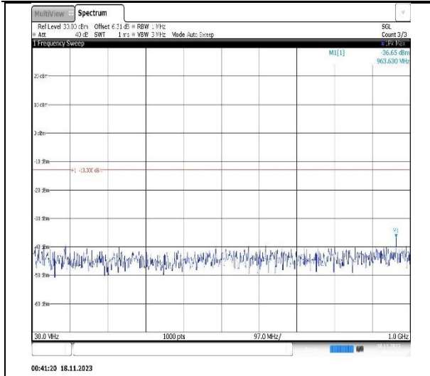
Band4-20MHz-QPSK-20050-1RB#0-Range1:30~1000MHz
