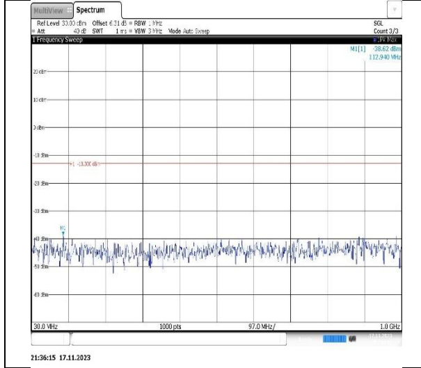
Band4-1.4MHz-16QAM-20175-1RB#0-Range1:30~1000MHz
