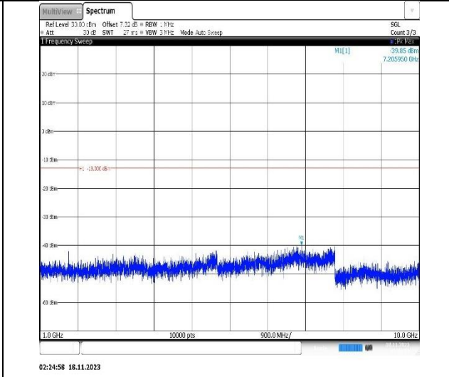
Band5-3MHz-16QAM-20635-1RB#0-Range2:1000~10000MHz
