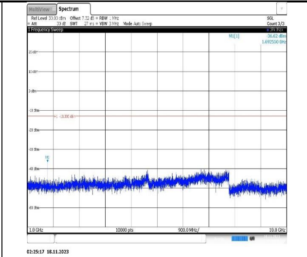
Band5-3MHz-16QAM-20415-1RB#0-Range2:1000~10000MHz
