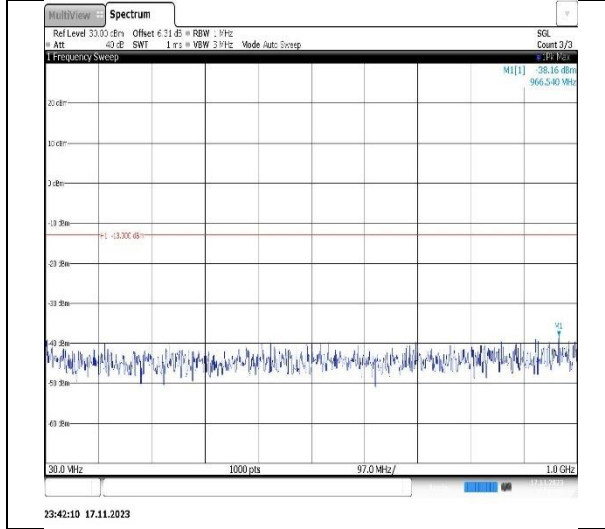
Band4-10MHz-QPSK-20175-1RB#0- Range1:30~1000MHz
