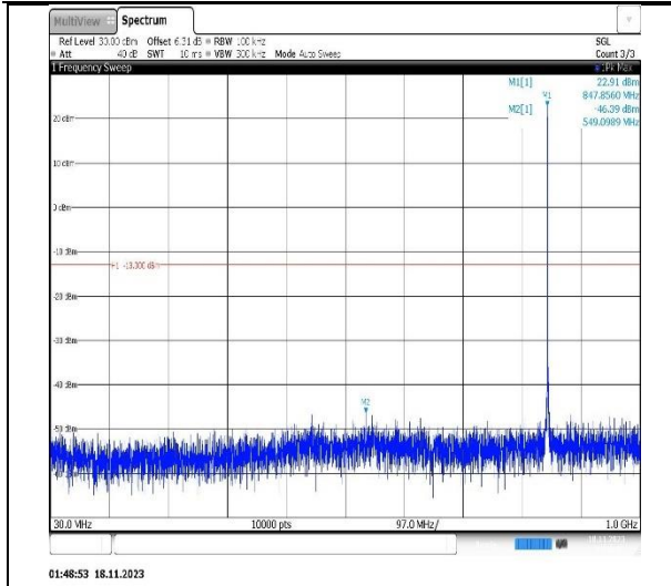
Band5-3MHz-QPSK-20415-1RB#0-Range1:30~1000MHz
