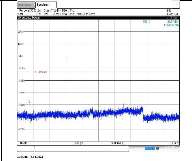
Band5-10MHz-QPSK-20600-1RB#0-Range2:1000~10000MHz
