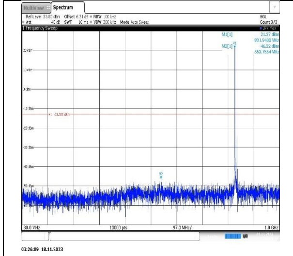
Band5-10MHz-QPSK-20600-1RB#0-Range1:30~1000MHz
