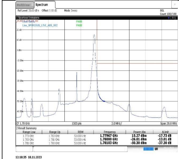
Band66-5MHz-16QAM-132647-1RB#24
