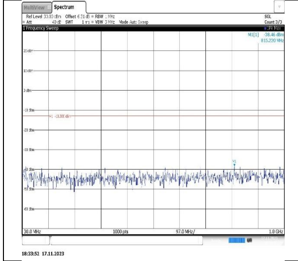
Band2-5MHz-QPSK-18900-1RB#0-Range1:30~1000MHz
