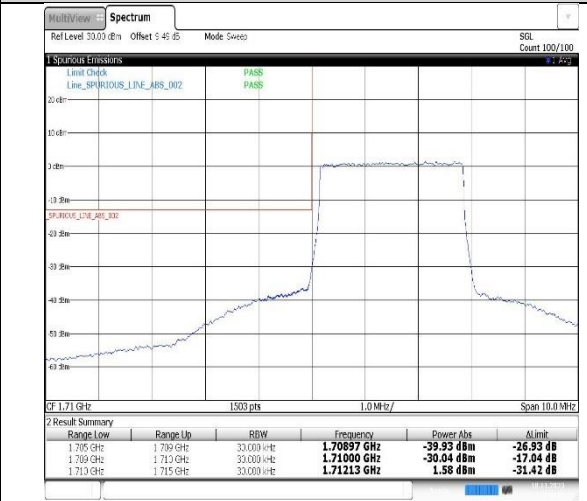
Band66-3MHz-16QAM-131987-1RB#0
