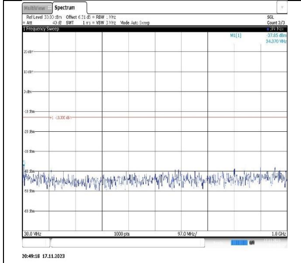
Band2-20MHz-QPSK-19100-1RB#0-Range1:30~1000MHz
