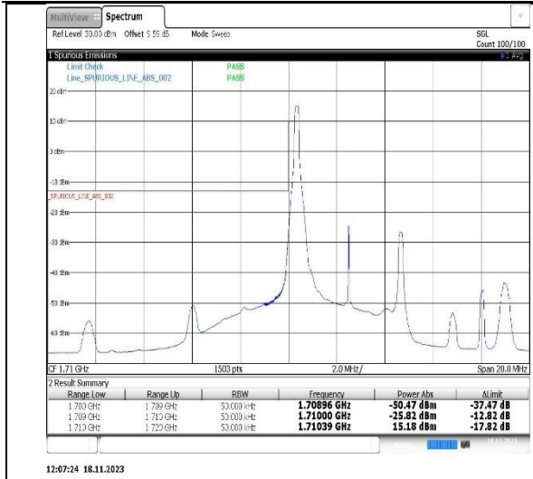
Band66-5MHz-16QAM-132647-1RB#24
