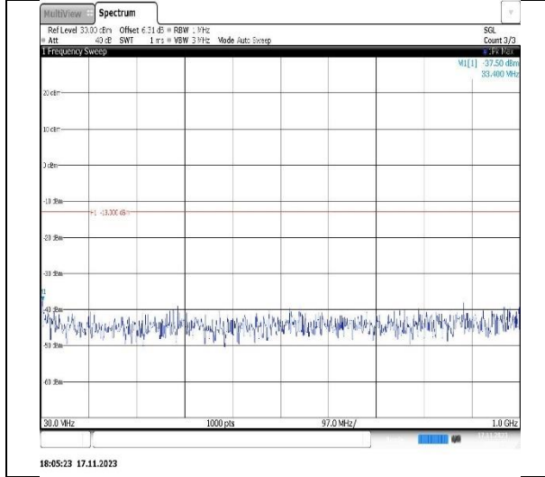
Band2-3MHz-QPSK-18900-1RB#0-Range1:30~1000MHz
