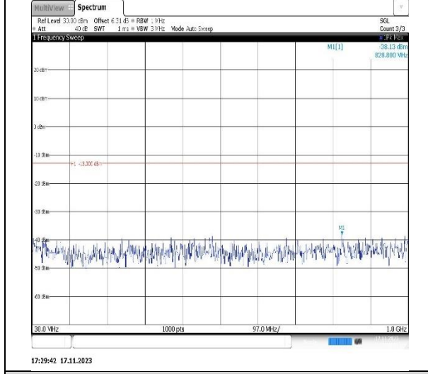
Band2-1.4MHz-16QAM-19193-1RB#0-Range1:30~1000MHz
