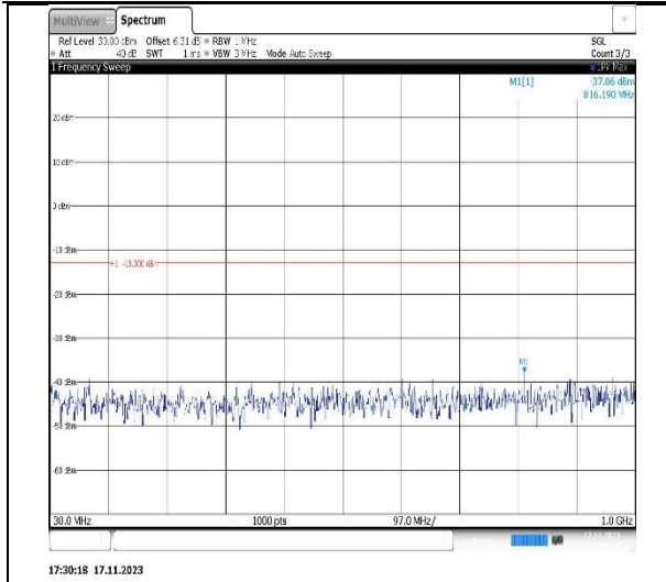
Band2-3MHz-QPSK-18615-1RB#0-Range1:30~1000MHz
