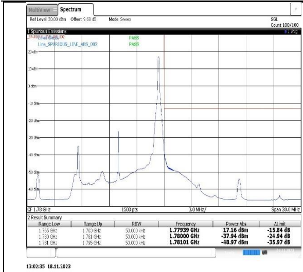
Band66-15MHz-QPSK-132047-1RB#0
