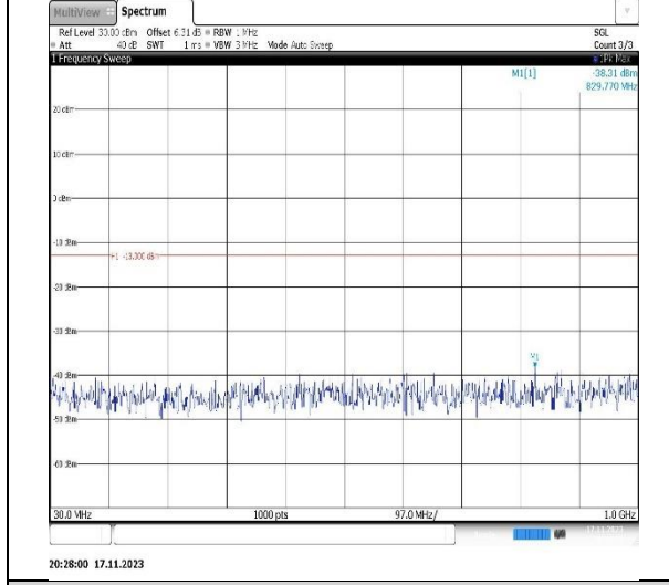
Band2-15MHz-QPSK-19125-1RB#0-Range1:30~1000MHz
