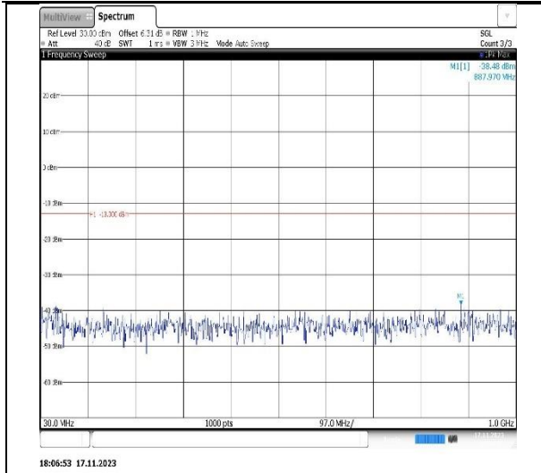
Band2-5MHz-QPSK-18625-1RB#0-Range1:30~1000MHz
