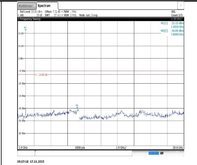
Band2-15MHz-QPSK-18675-1RB#0-Range2:1000~20000MHz
