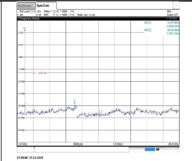
Band2-1.4MHz-16QAM-18607-1RB#0-Range2:1000~20000MHz
