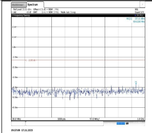
Band2-15MHz-QPSK-18675-1RB#0-Range1:30~1000MHz
