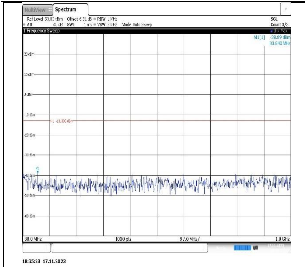
Band2-10MHz-QPSK-18650-1RB#0-Range1:30~1000MHz
