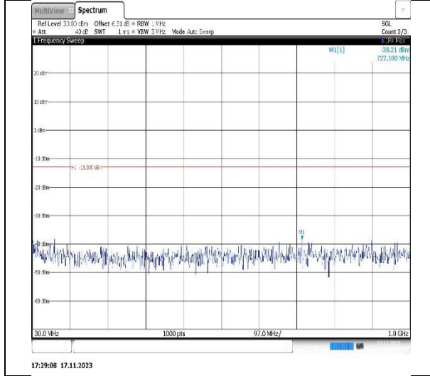
Band2-1.4MHz-16QAM-18900-1RB#0-Range1:30~1000MHz
