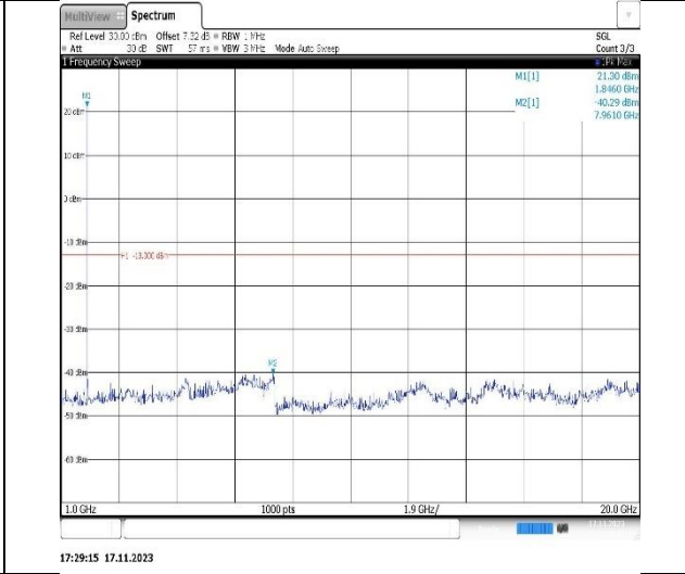
Band2-1.4MHz-16QAM-18900-1RB#0-Range2:1000~20000MHz
