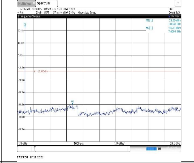
Band2-1.4MHz-16QAM-19193-1RB#0-Range2:1000~20000MHz
