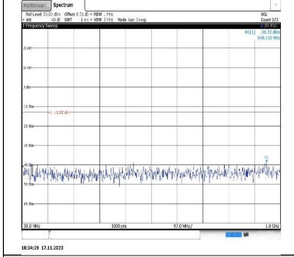
Band2-5MHz-QPSK-19175-1RB#0-Range1:30~1000MHz
