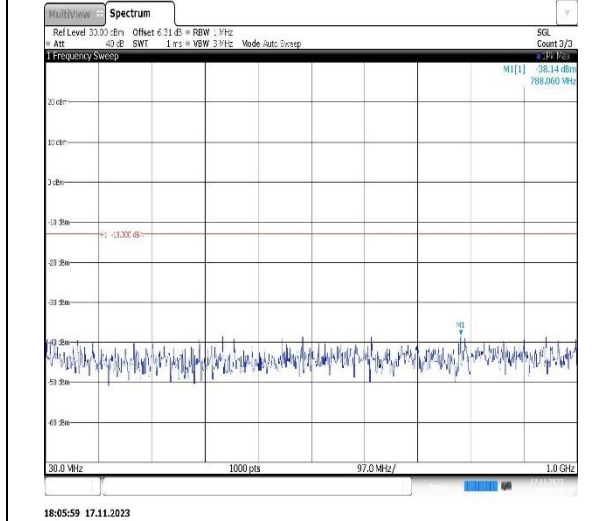
Band2-3MHz-QPSK-19185-1RB#0-Range1:30~1000MHz
