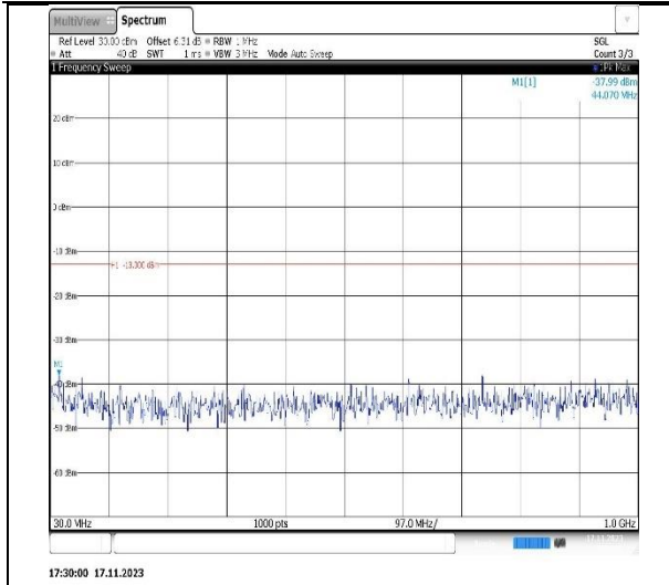
Band2-1.4MHz-16QAM-18607-1RB#0-Range1:30~1000MHz
