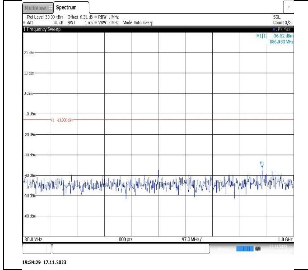
Band2-10MHz-QPSK-18900-1RB#0-Range1:30~1000MHz
