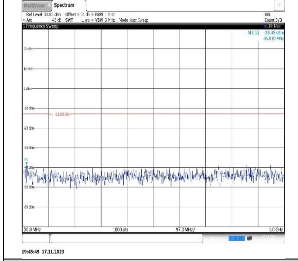
Band2-10MHz-QPSK-19150-1RB#0-Range1:30~1000MHz
