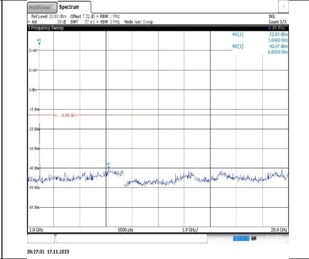
Band2-15MHz-QPSK-18900-1RB#0-Range2:1000~20000MHz
