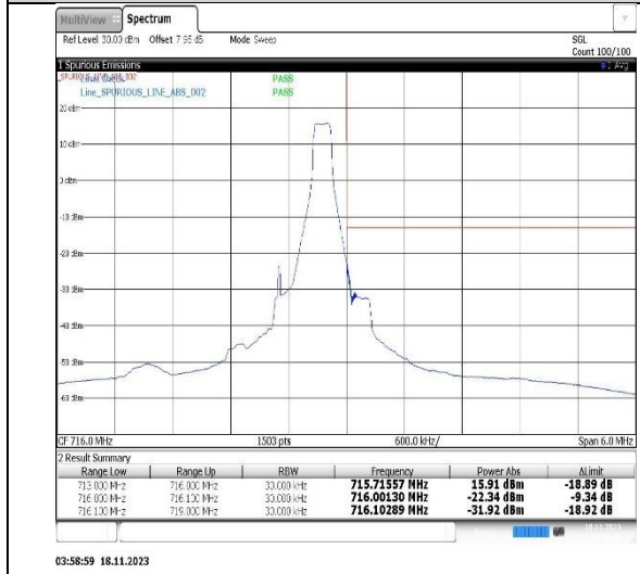
Band12-3MHz-QPSK-23025-1RB#0
