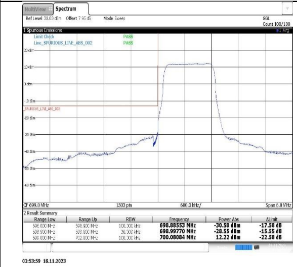
Band12-1.4MHz-QPSK-23173-6RB#0
