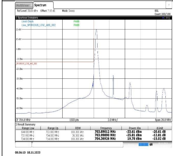
Band17-10MHz-QPSK-23780-1RB#0
