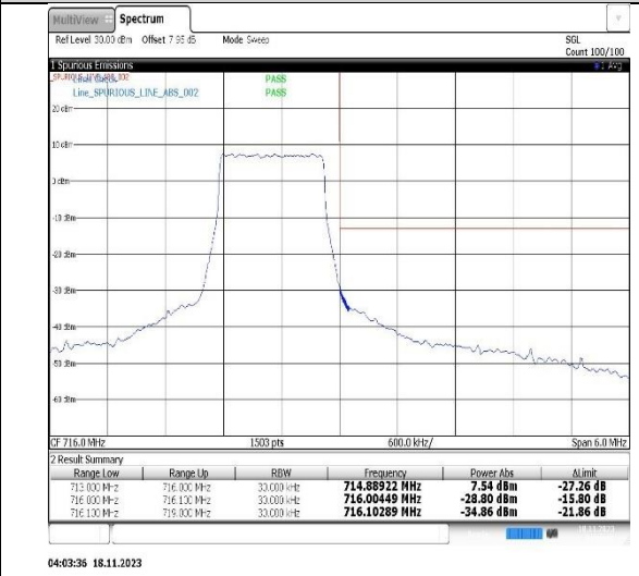
Band12-3MHz-QPSK-23025-15RB#0
