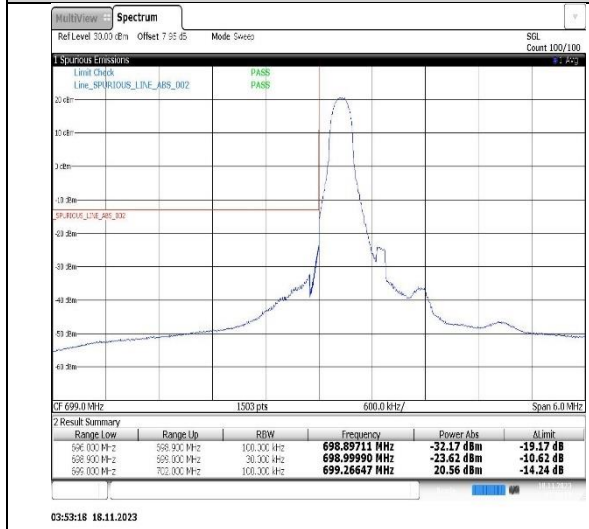
Band12-1.4MHz-QPSK-23173-1RB#5
