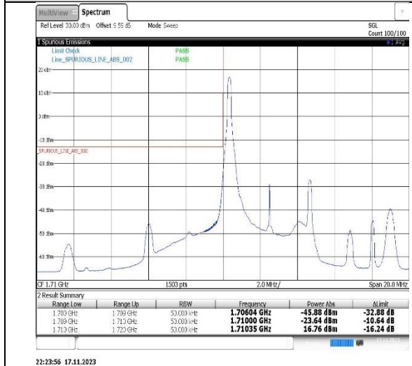
Band4-5MHz-16QAM-20375-1RB#24
