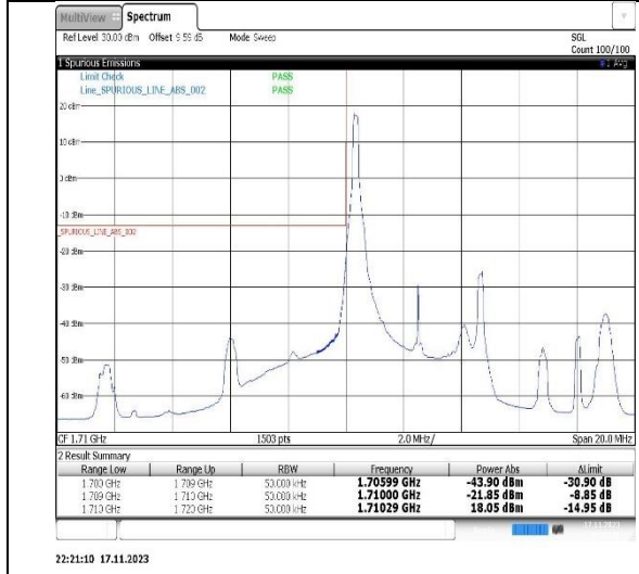
Band4-5MHz-QPSK-19975-1RB#0
