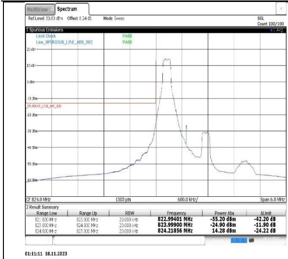
Band5-1.4MHz-QPSK-20643-1RB#5
