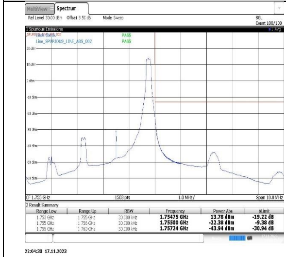
Band4-3MHz-16QAM-20385-1RB#14
