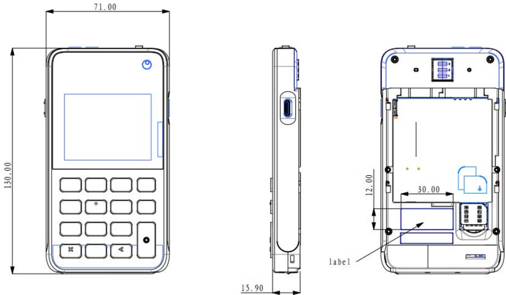
Open the battery cover , The label is carved with radius next to the battery compartment.
