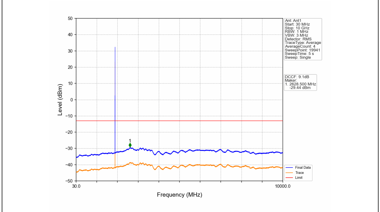
PCS1900_GPRS_HCH_1909.8MHz_1 TX Slot_NTNV
