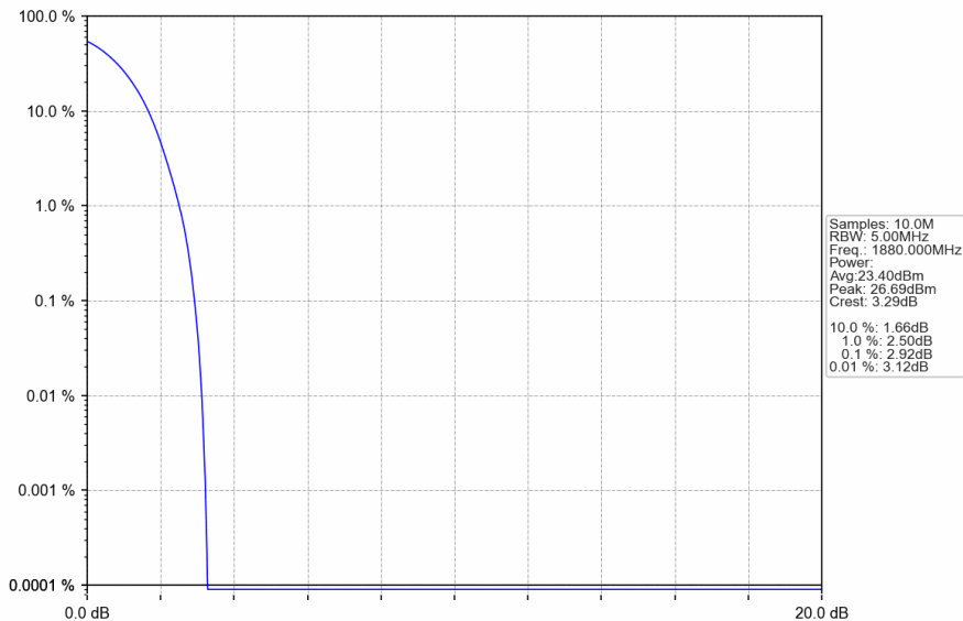
Band2_RMC_MCH_1880MHz_12.2kbps RMC_NTNV
