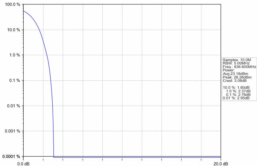
Band5_RMC_MCH_836.6MHz_12.2kbps RMC_NTNV
