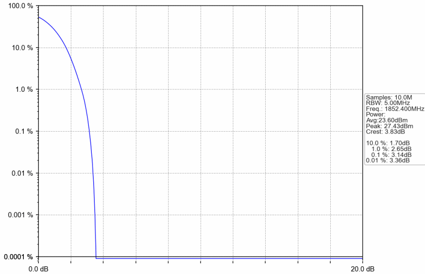
Band2_RMC_LCH_1852.4MHz_12.2kbps RMC_NTNV
