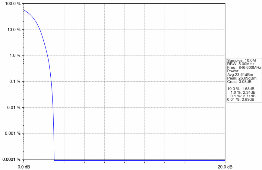
Band5_RMC_HCH_846.6MHz_12.2kbps RMC_NTNV
