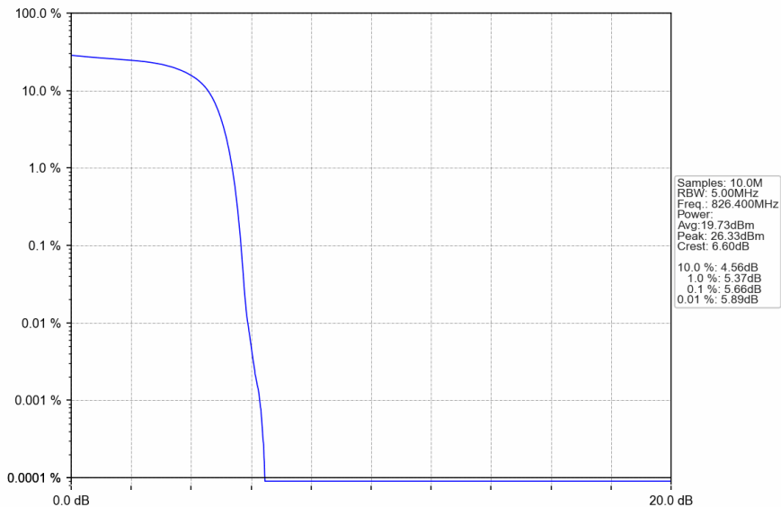
Band5_HSDPA_LCH_826.4MHz_Subtest 1_NTNV
