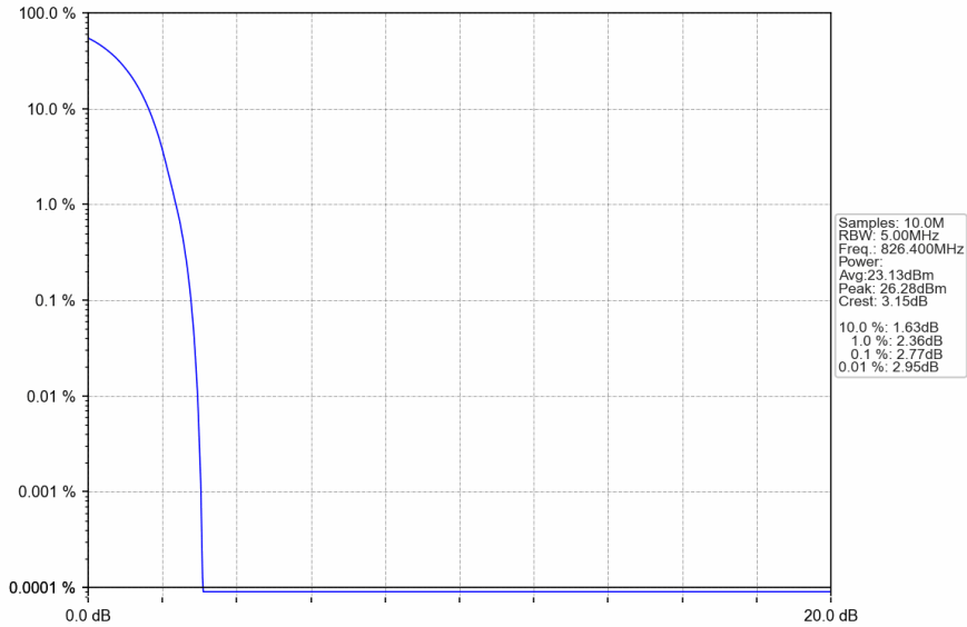
Band5_RMC_LCH_826.4MHz_12.2kbps RMC_NTNV
