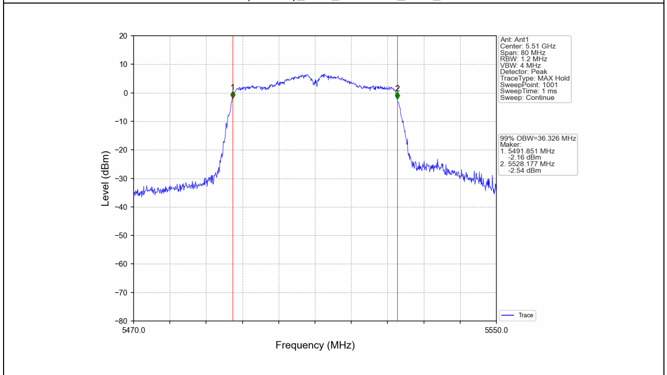
802.11ac(VHT40)_LCH_5510MHz_Ant1_NTNV
