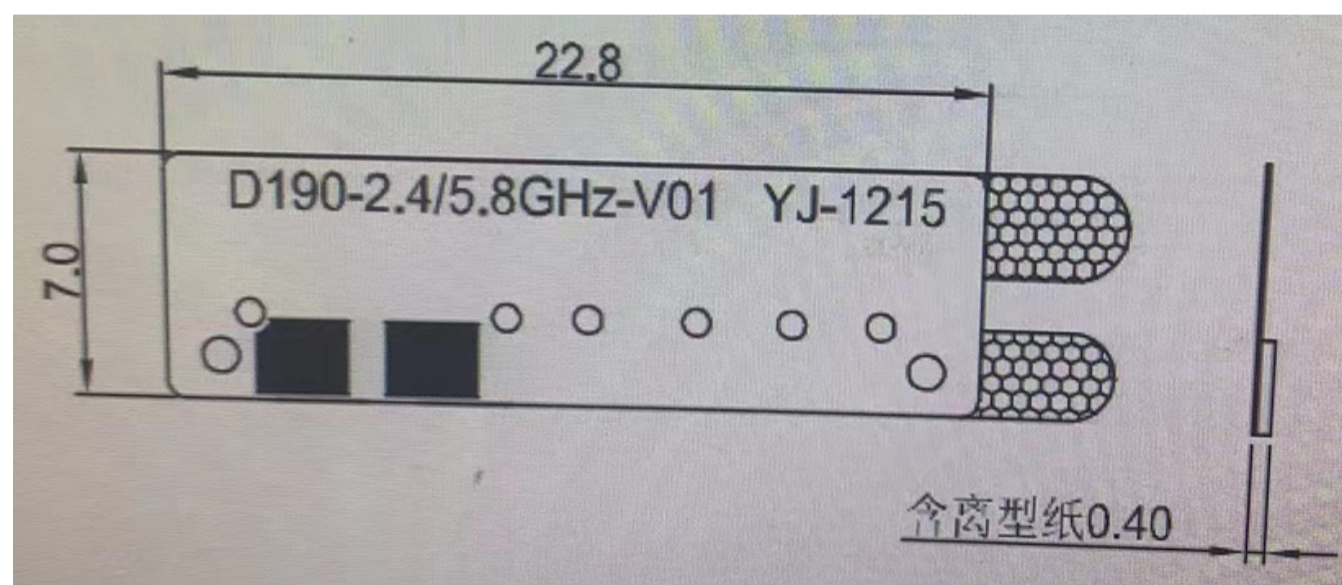
WiFi antenna(unit:mm): Model: YJ-1215
