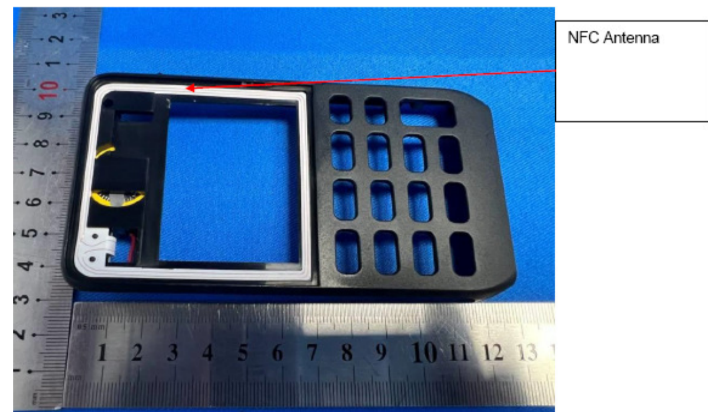
NFC antenna: 6.2cm*5.8cm(2 laps) Model: YJ-0214
