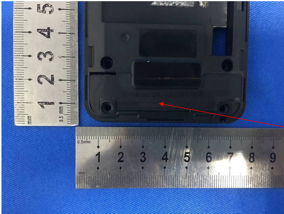
2G/3G antenna
