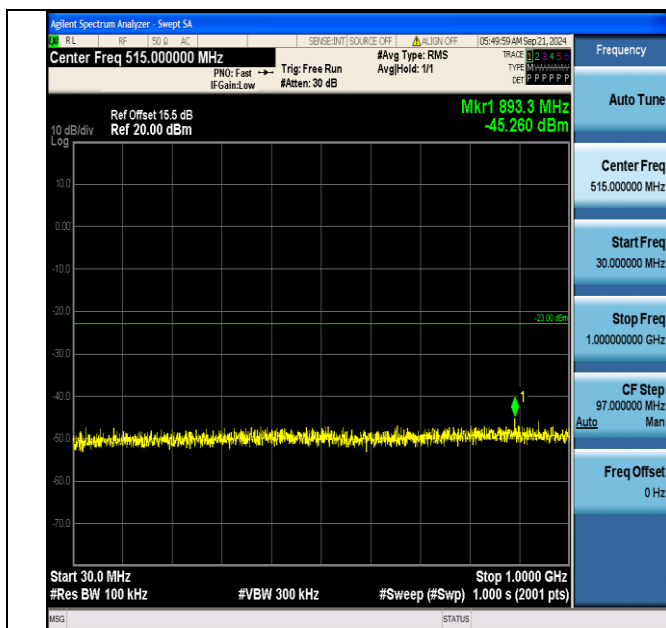
Band66_20MHz_QPSK_132322_1RB#99_30~1000_30~1000
