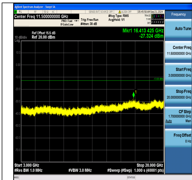
Band66_15MHz_QPSK_132597_75RB#0_3000~20000_3000~20000
