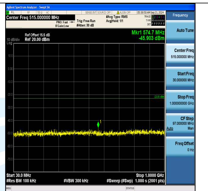
Band66_15MHz_16QAM_132047_1RB#0_30~1000_30~1000
