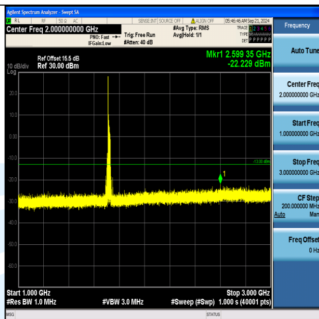
Band66_20MHz_QPSK_132072_1RB#0_1000~3000_1000~3000
