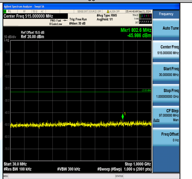
Band66_15MHz_QPSK_132597_1RB#74_30~1000_30~1000
