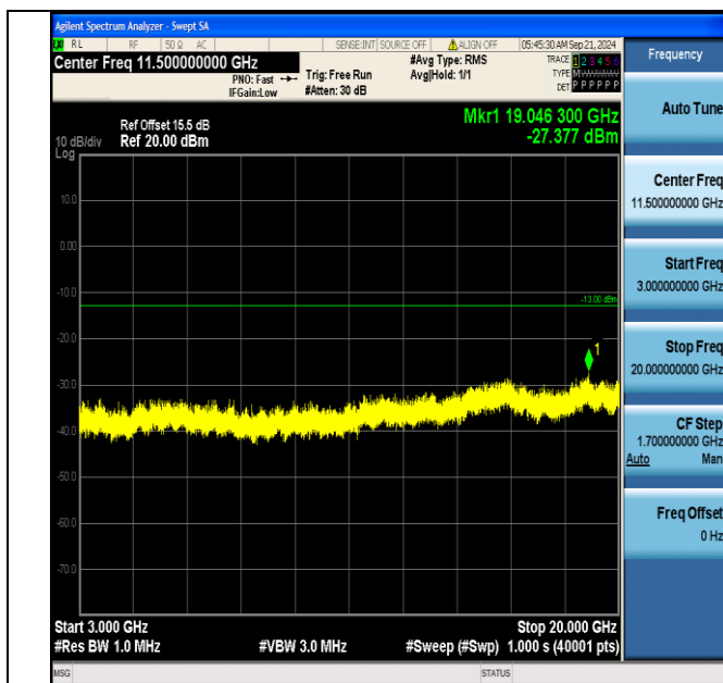
Band66_15MHz_16QAM_132597_1RB#74_3000~20000_3000~20000
