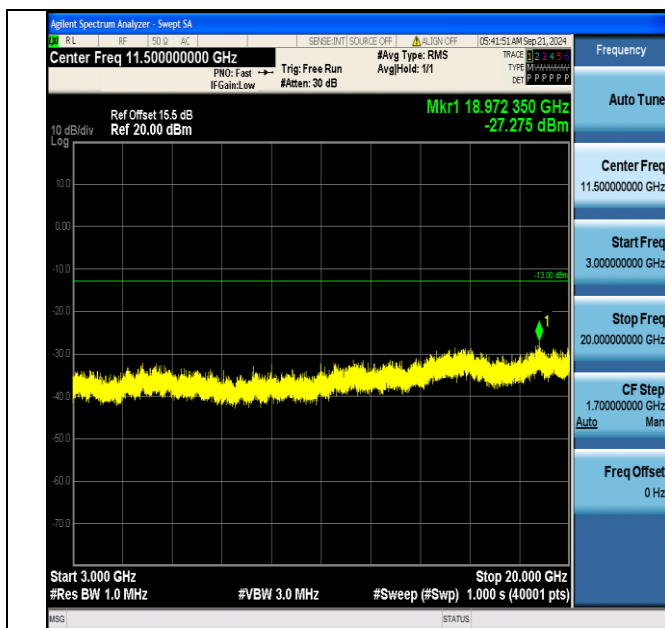
Band66_15MHz_16QAM_132322_1RB#0_3000~20000_3000~20000
