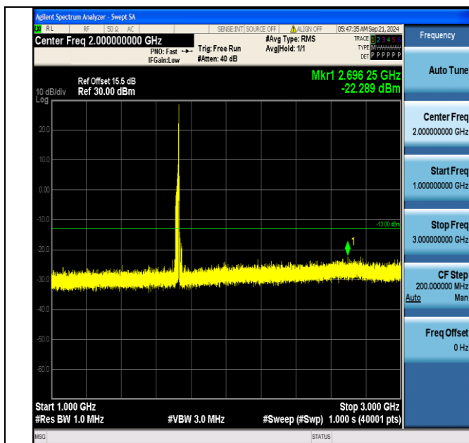
Band66_20MHz_QPSK_132072_1RB#99_1000~3000_1000~3000
