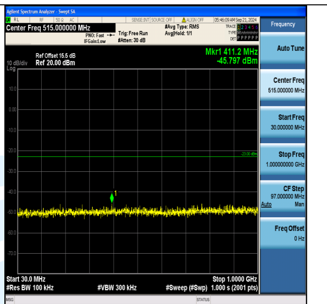
Band66_15MHz_16QAM_132597_75RB#0_30~1000_30~1000
