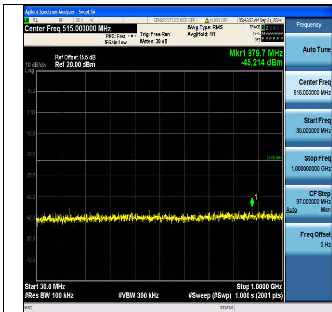
Band66_15MHz_16QAM_132322_75RB#0_30~1000_30~1000
