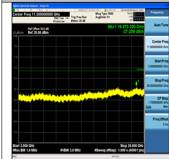
Band66_15MHz_QPSK_132597_1RB#0_3000~20000_3000~20000
