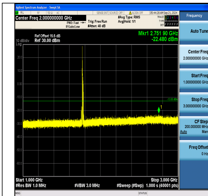
Band66_15MHz_16QAM_132597_1RB#0_1000~3000_1000~3000
