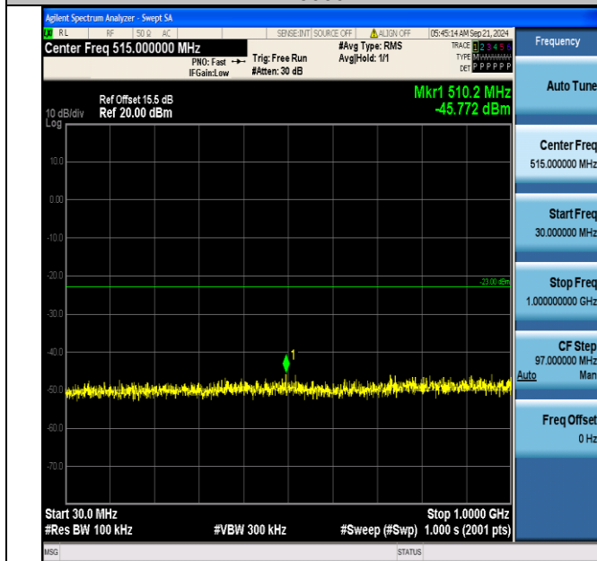
Band66_15MHz_16QAM_132597_1RB#74_30~1000_30~1000
