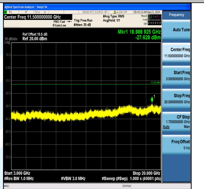
Band66_15MHz_QPSK_132322_75RB#0_3000~20000_3000~20000
