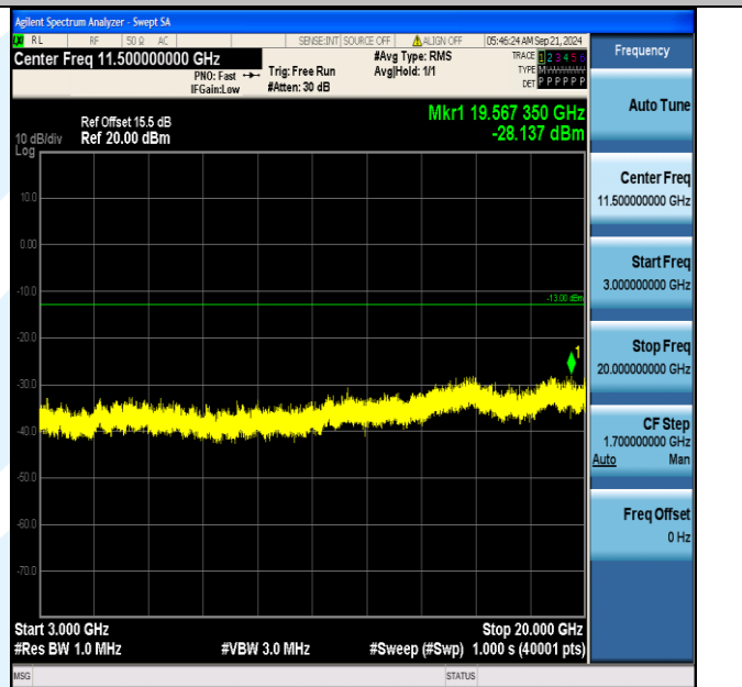
Band66_15MHz_16QAM_132597_75RB#0_3000~20000_3000~20000
