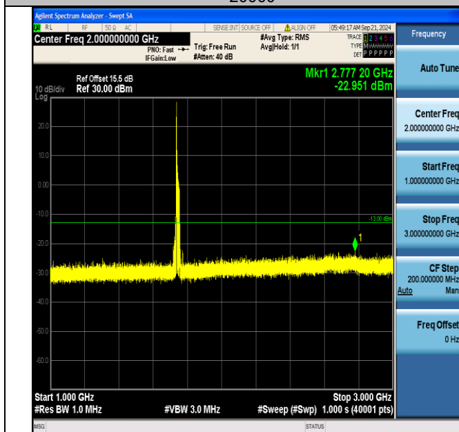
Band66_20MHz_QPSK_132322_1RB#0_1000~3000_1000~3000
