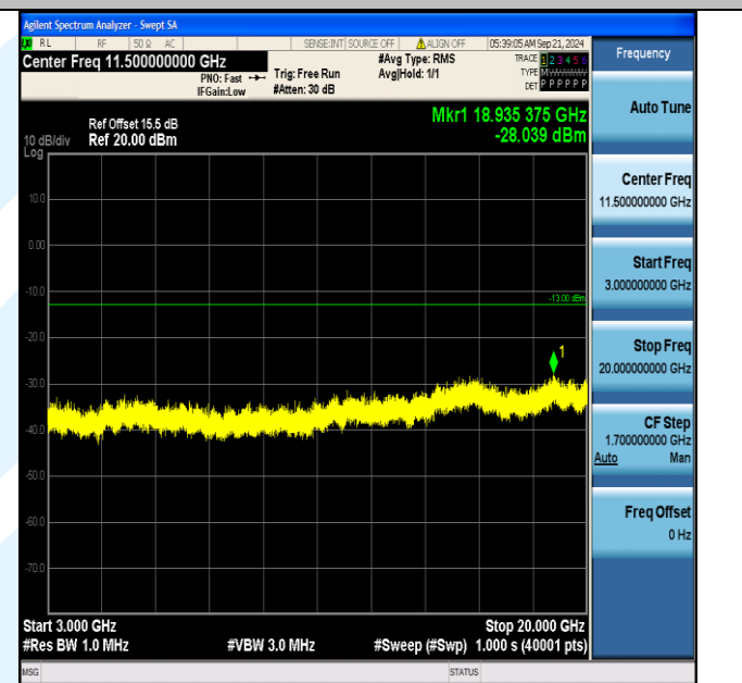
Band66_15MHz_16QAM_132047_1RB#0_3000~20000_3000~20000
