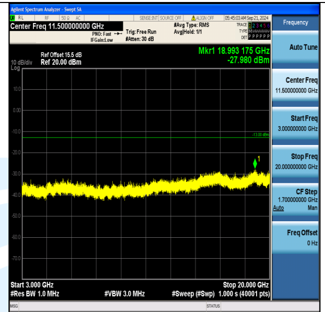
Band66_15MHz_QPSK_132597_1RB#74_3000~20000_3000~20000
