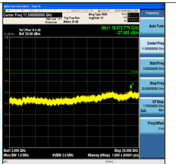
Band66_20MHz_QPSK_132072_1RB#99_3000~20000_3000~20000
