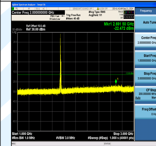
Band66_15MHz_16QAM_132322_1RB#0_1000~3000_1000~3000
