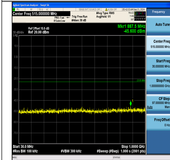
Band66_15MHz_QPSK_132322_1RB#74_30~1000_30~1000
