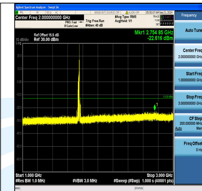
Band66_20MHz_QPSK_132322_1RB#99_1000~3000_1000~3000
