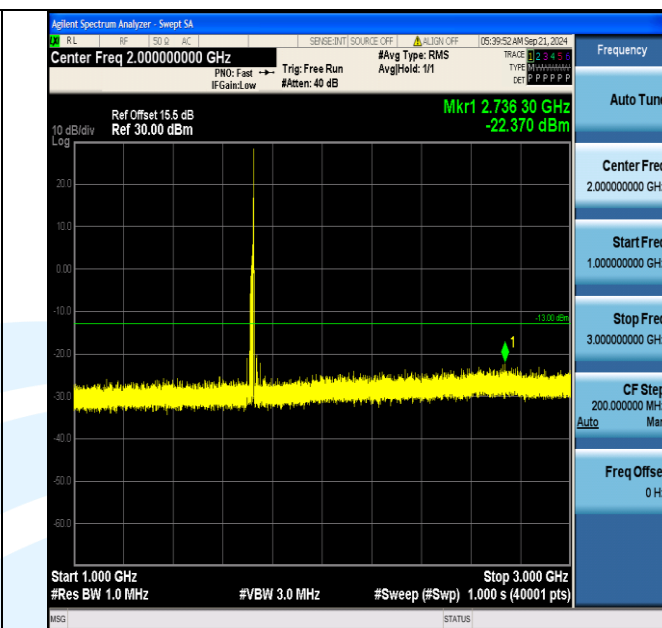
Band66_15MHz_16QAM_132047_1RB#74_1000~3000_1000~3000
