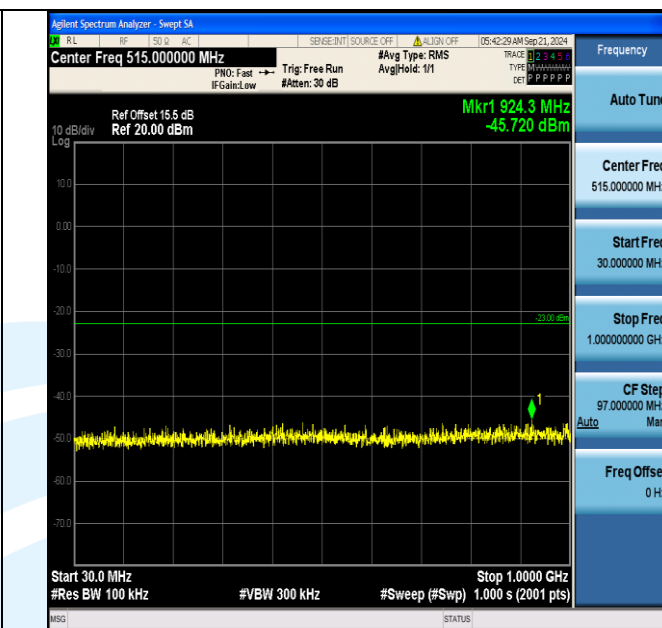
Band66_15MHz_16QAM_132322_1RB#74_30~1000_30~1000
