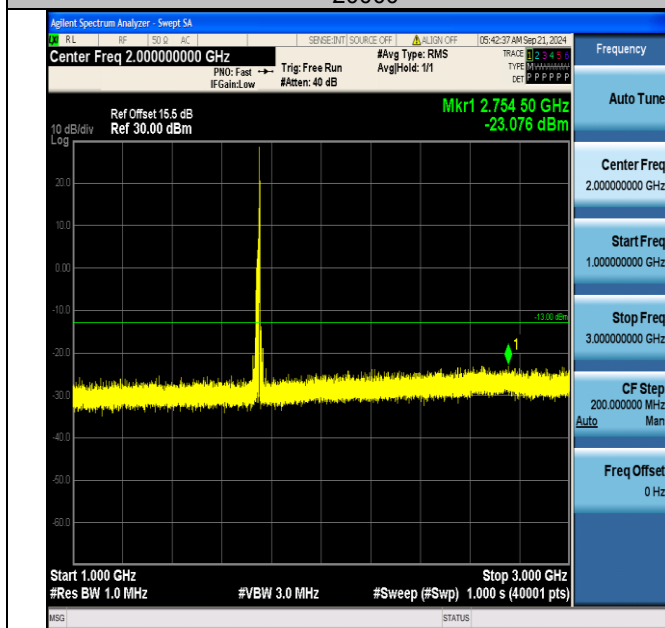
Band66_15MHz_16QAM_132322_1RB#74_1000~3000_1000~3000
