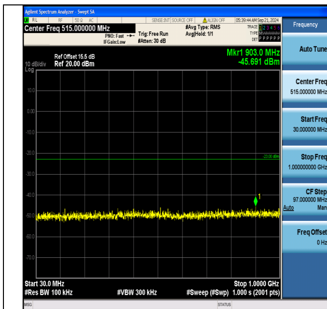
Band66_15MHz_16QAM_132047_1RB#74_30~1000_30~1000
