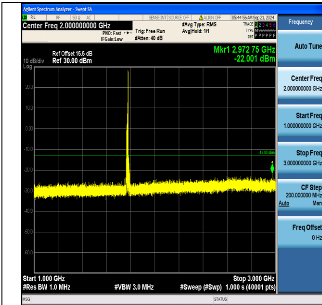
Band66_15MHz_QPSK_132597_1RB#74_1000~3000_1000~3000
