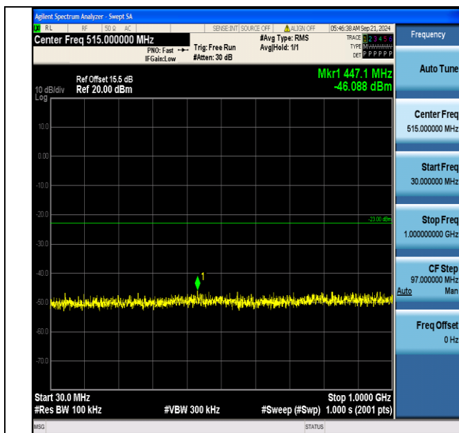
Band66_20MHz_QPSK_132072_1RB#0_30~1000_30~1000
