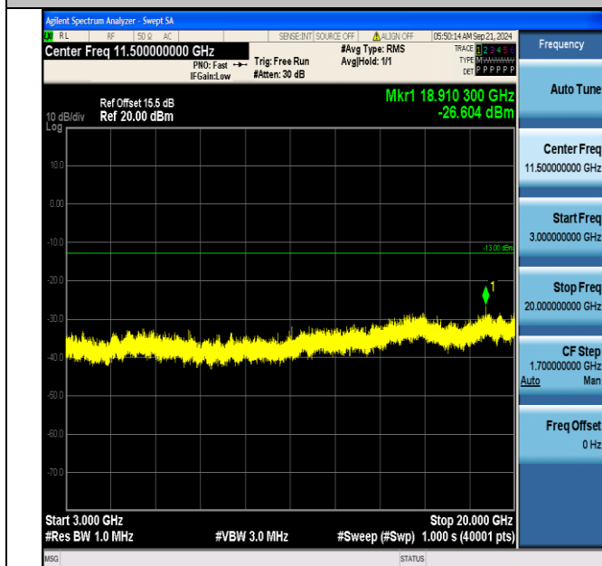
Band66_20MHz_QPSK_132322_1RB#99_3000~20000_3000~20000
