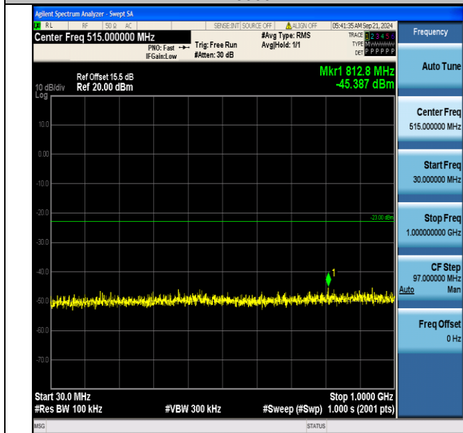
Band66_15MHz_16QAM_132322_1RB#0_30~1000_30~1000
