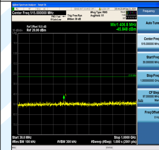
Band66_15MHz_16QAM_132597_1RB#0_30~1000_30~1000
