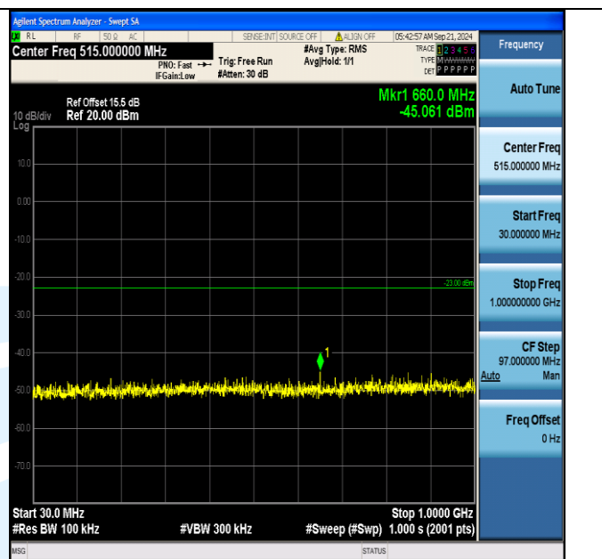
Band66_15MHz_QPSK_132322_75RB#0_30~1000_30~1000
