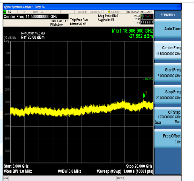
Band66_15MHz_16QAM_132597_1RB#0_3000~20000_3000~20000
