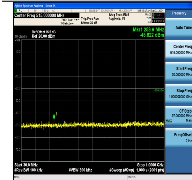
Band66_20MHz_QPSK_132072_100RB#0_30~1000_30~1000
