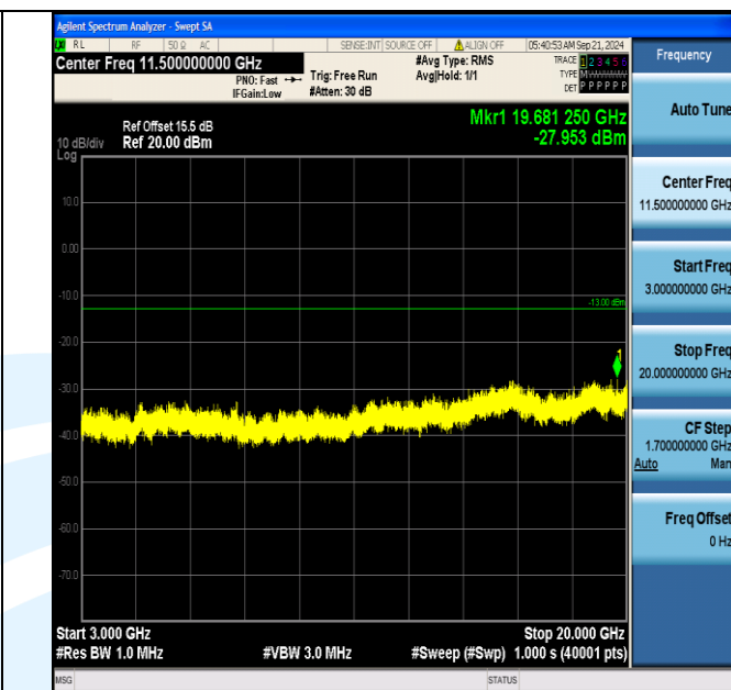
Band66_15MHz_16QAM_132047_75RB#0_3000~20000_3000~20000
