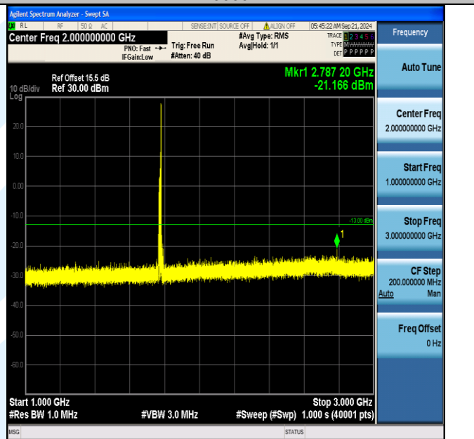
Band66_15MHz_16QAM_132597_1RB#74_1000~3000_1000~3000
