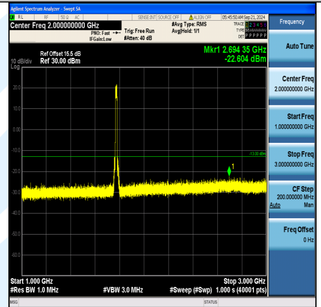
Band66_15MHz_QPSK_132597_75RB#0_1000~3000_1000~3000
