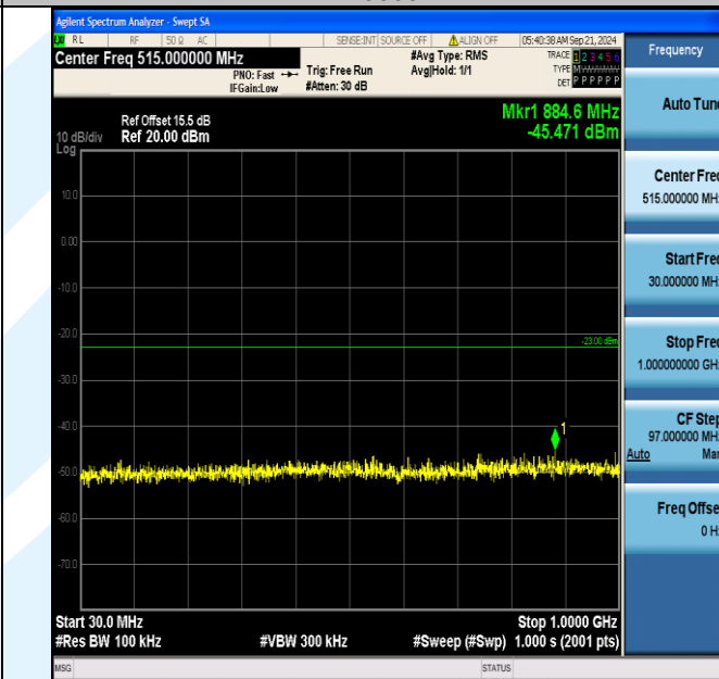
Band66_15MHz_16QAM_132047_75RB#0_30~1000_30~1000
