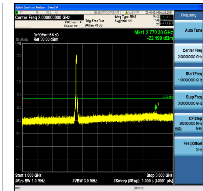
Band66_15MHz_16QAM_132047_75RB#0_1000~3000_1000~3000
