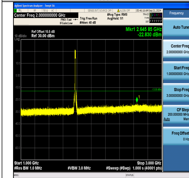
Band66_15MHz_16QAM_132597_75RB#0_1000~3000_1000~3000
