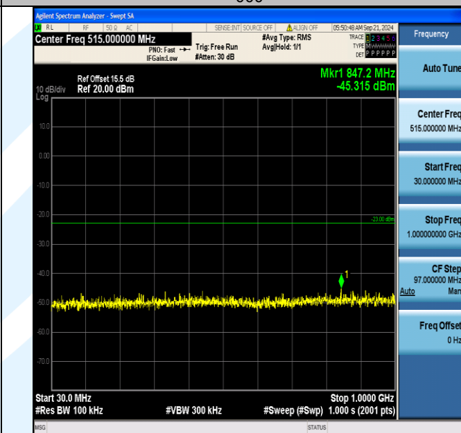
Band66_20MHz_QPSK_132322_100RB#0_30~1000_30~1000
