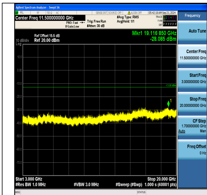
Band66_15MHz_QPSK_132322_1RB#74_3000~20000_3000~20000
