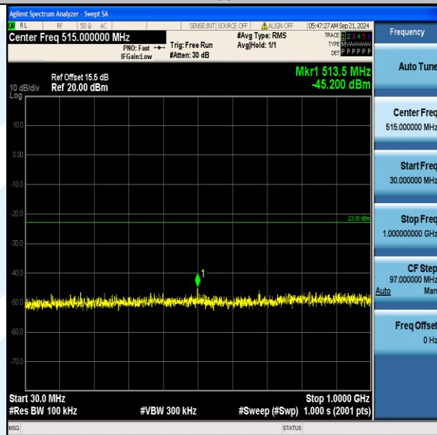
Band66_20MHz_QPSK_132072_1RB#99_30~1000_30~1000
