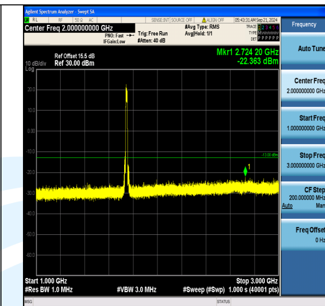
Band66_15MHz_16QAM_132322_75RB#0_1000~3000_1000~3000
