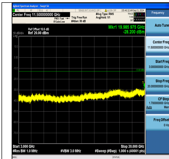
Band66_20MHz_QPSK_132072_100RB#0_3000~20000_3000~20000
