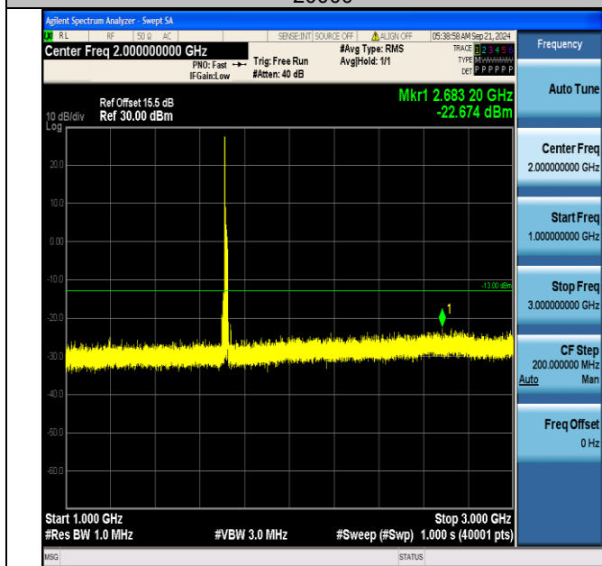
Band66_15MHz_16QAM_132047_1RB#0_1000~3000_1000~3000
