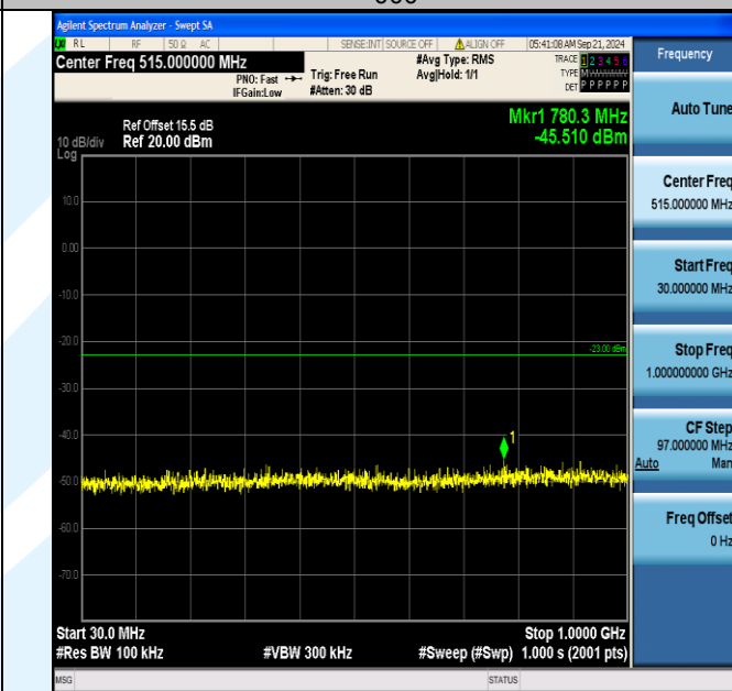
Band66_15MHz_QPSK_132322_1RB#0_30~1000_30~1000
