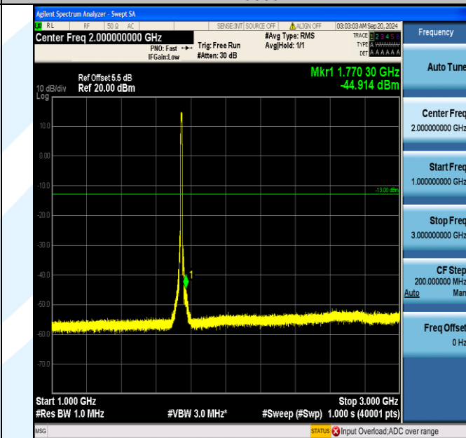
Band66_10MHz_16QAM_132322_50RB#0_1000~3000_1000~3000
