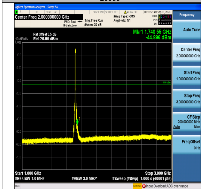
Band66_10MHz_16QAM_132022_50RB#0_1000~3000_1000~3000
