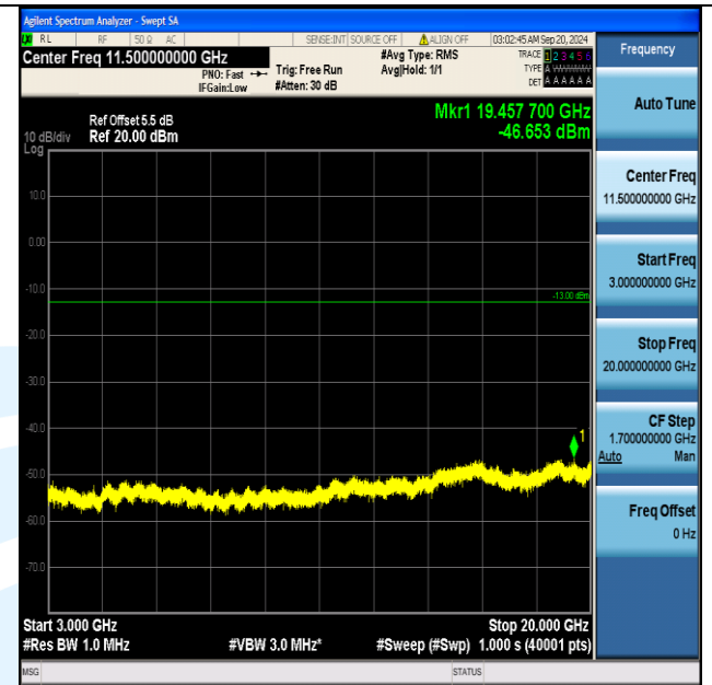
Band66_10MHz_QPSK_132322_50RB#0_3000~20000_3000~20000
