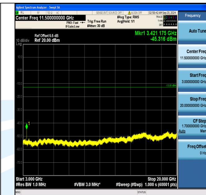
Band66_10MHz_16QAM_132022_1RB#0_3000~20000_3000~20000
