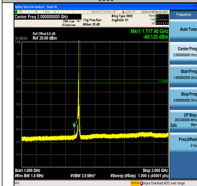
Band66_10MHz_QPSK_132622_1RB#49_1000~3000_1000~3000
