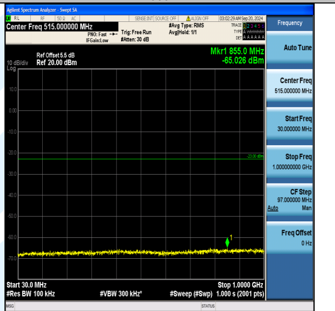
Band66_10MHz_QPSK_132322_50RB#0_30~1000_30~1000
