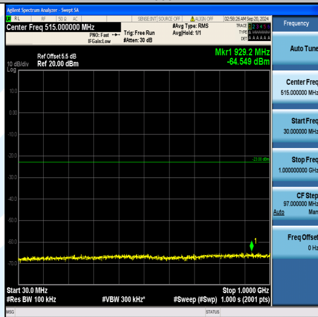
Band66_10MHz_16QAM_132022_1RB#0_30~1000_30~1000
