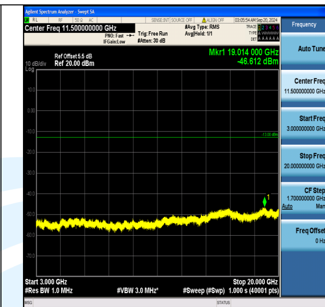
Band66_10MHz_16QAM_132622_50RB#0_3000~20000_3000~20000
