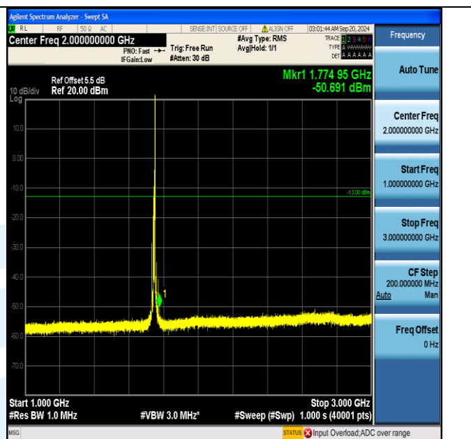
Band66_10MHz_QPSK_132322_1RB#49_1000~3000_1000~3000
