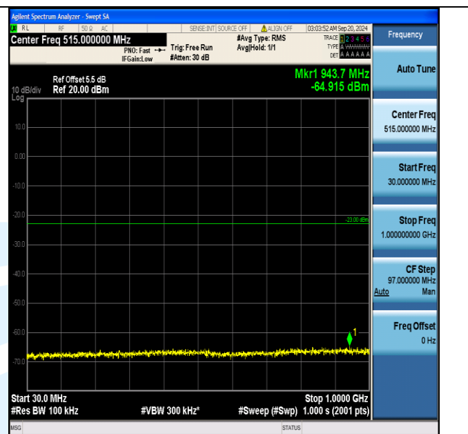
Band66_10MHz_16QAM_132622_1RB#0_30~1000_30~1000
