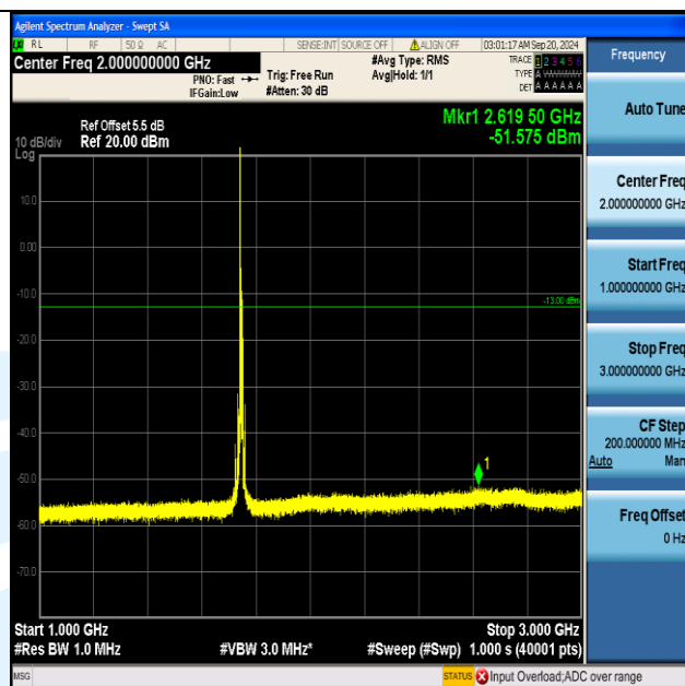
Band66_10MHz_16QAM_132322_1RB#0_1000~3000_1000~3000
