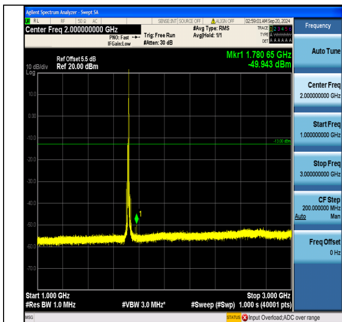
Band66_10MHz_QPSK_132022_1RB#49_1000~3000_1000~3000
