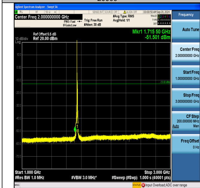
Band66_10MHz_QPSK_132322_1RB#0_1000~3000_1000~3000
