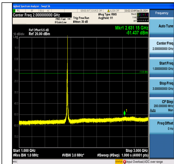
Band66_10MHz_16QAM_132322_1RB#49_1000~3000_1000~3000
