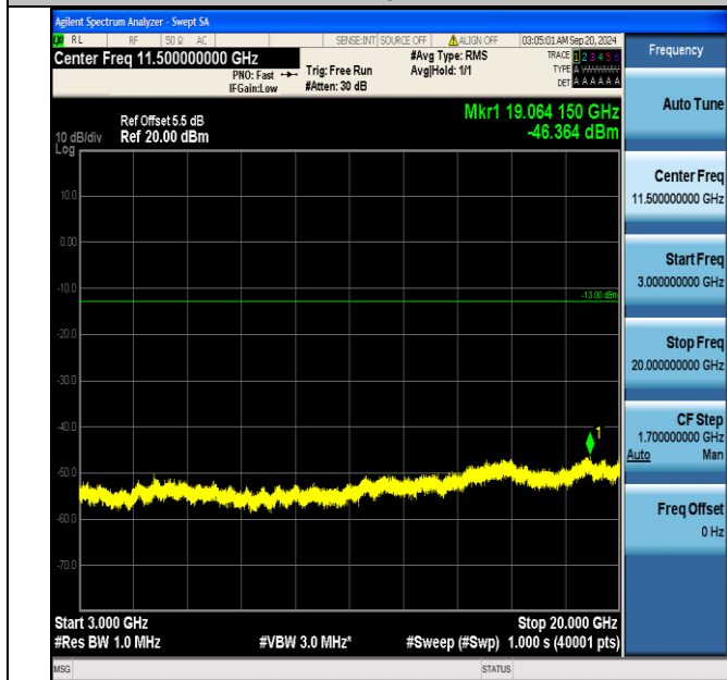
Band66_10MHz_16QAM_132622_1RB#49_3000~20000_3000~20000
