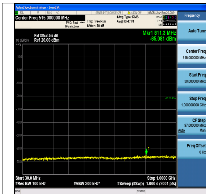
Band66_10MHz_QPSK_132622_50RB#0_30~1000_30~1000
