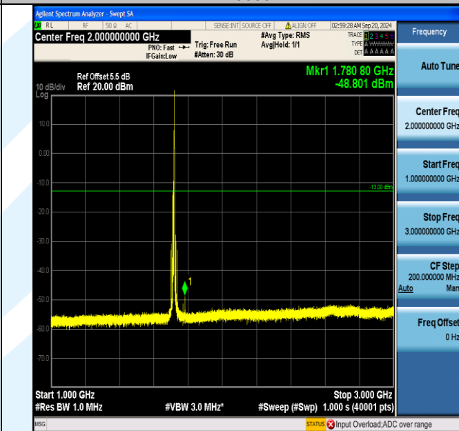
Band66_10MHz_16QAM_132022_1RB#49_1000~3000_1000~3000
