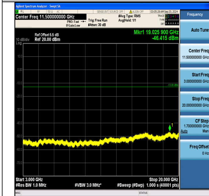
Band66_10MHz_QPSK_132622_50RB#0_3000~20000_3000~20000
