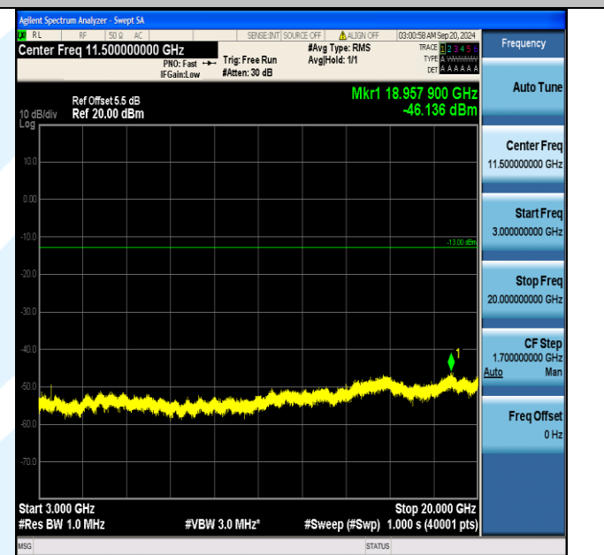
Band66_10MHz_QPSK_132322_1RB#0_3000~20000_3000~20000
