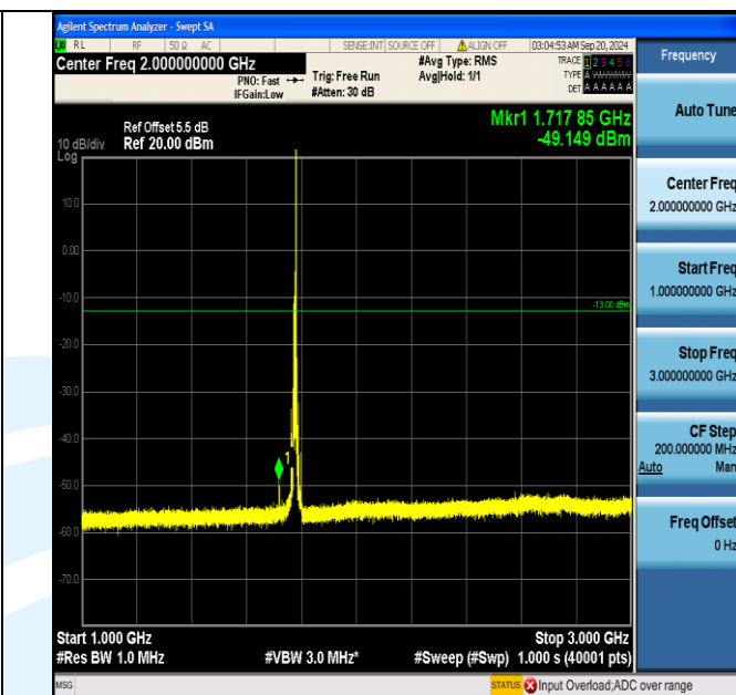
Band66_10MHz_16QAM_132622_1RB#49_1000~3000_1000~3000
