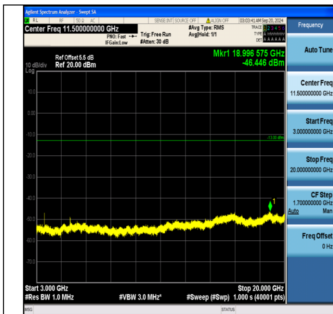
Band66_10MHz_QPSK_132622_1RB#0_3000~20000_3000~20000
