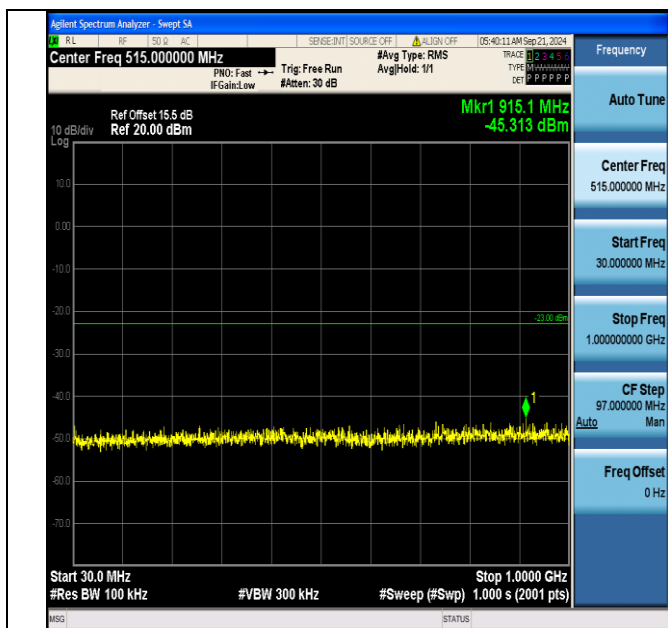
Band66_15MHz_QPSK_132047_75RB#0_30~1000_30~1000
