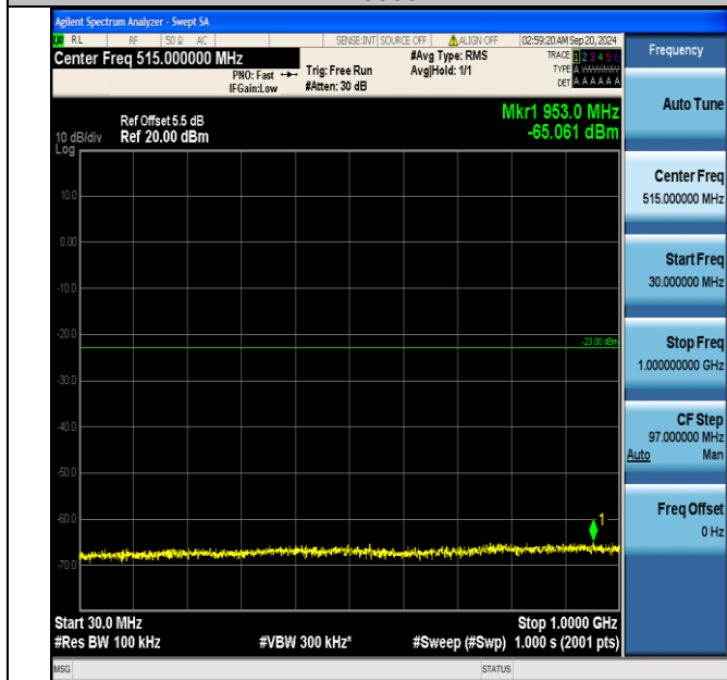
Band66_10MHz_16QAM_132022_1RB#49_30~1000_30~1000
