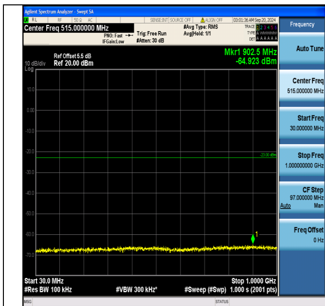
Band66_10MHz_QPSK_132322_1RB#49_30~1000_30~1000
