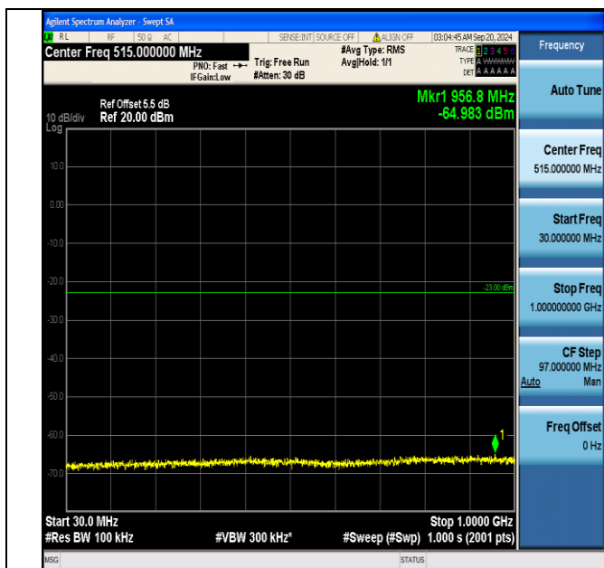
Band66_10MHz_16QAM_132622_1RB#49_30~1000_30~1000
