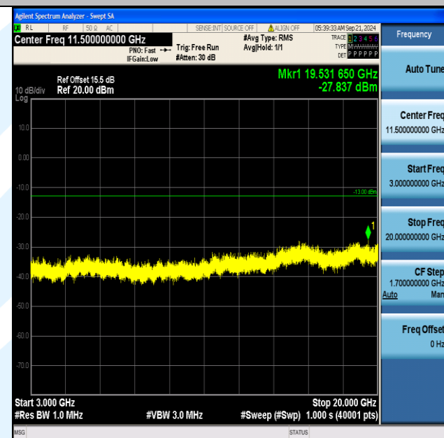
Band66_15MHz_QPSK_132047_1RB#74_3000~20000_3000~20000
