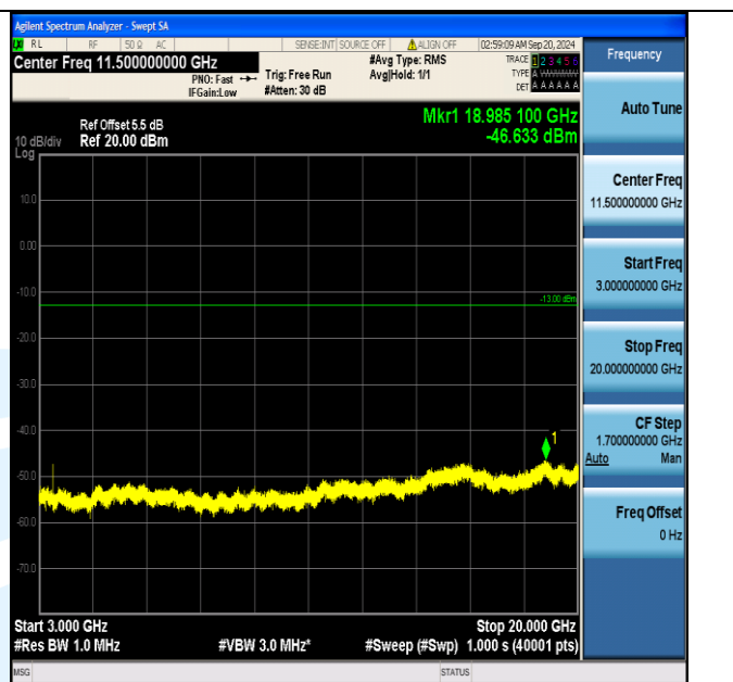
Band66_10MHz_QPSK_132022_1RB#49_3000~20000_3000~20000
