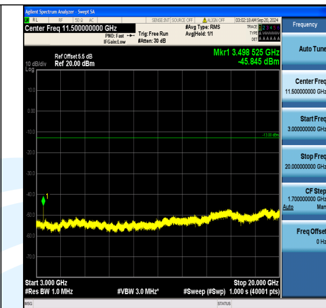
Band66_10MHz_16QAM_132322_1RB#49_3000~20000_3000~20000
