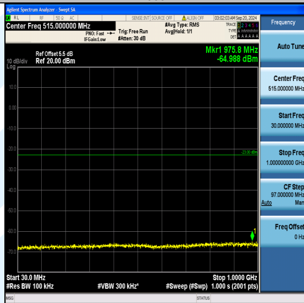
Band66_10MHz_16QAM_132322_1RB#49_30~1000_30~1000
