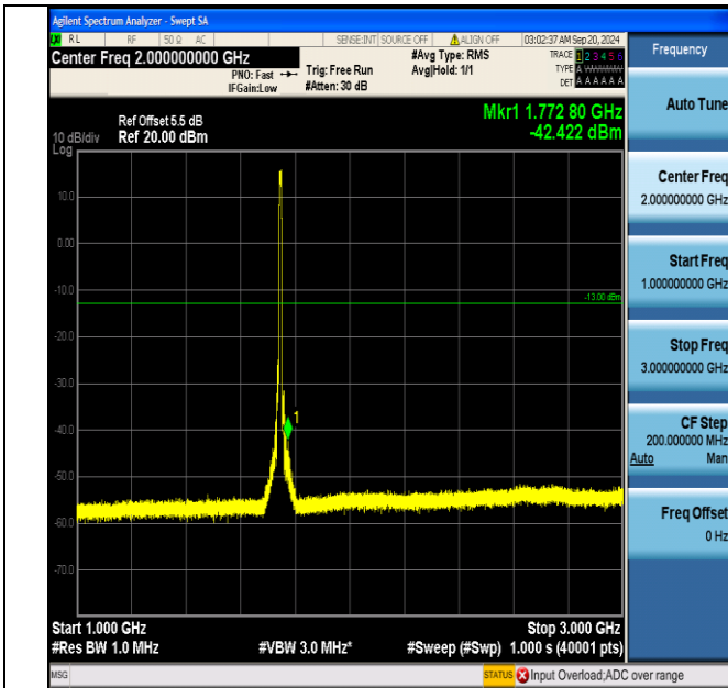
Band66_10MHz_QPSK_132322_50RB#0_1000~3000_1000~3000
