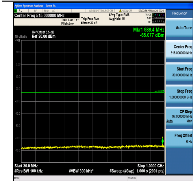
Band66_10MHz_16QAM_132322_50RB#0_30~1000_30~1000
