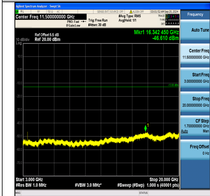
Band66_10MHz_QPSK_132322_1RB#49_3000~20000_3000~20000
