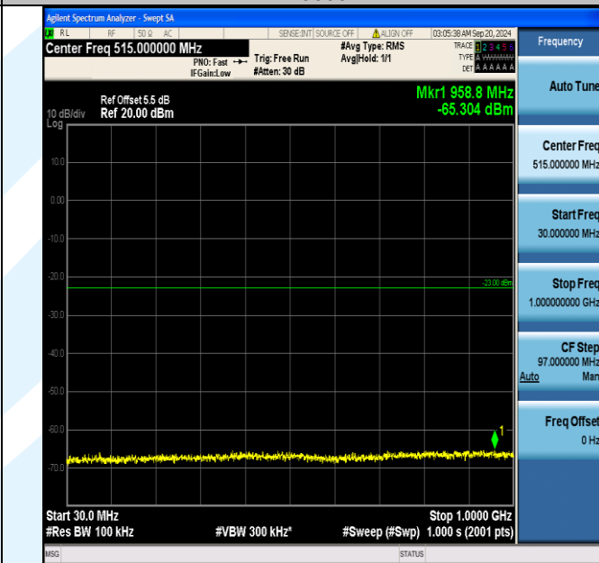
Band66_10MHz_16QAM_132622_50RB#0_30~1000_30~1000
