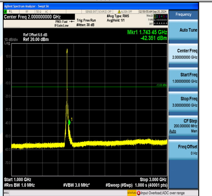
Band66_10MHz_QPSK_132022_50RB#0_1000~3000_1000~3000
