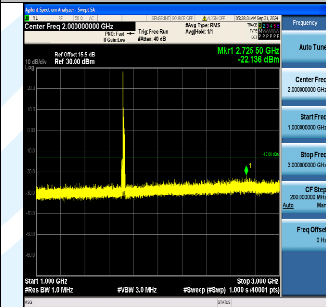
Band66_15MHz_QPSK_132047_1RB#0_1000~3000_1000~3000
