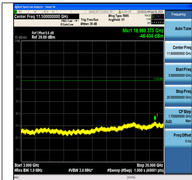
Band66_10MHz_QPSK_132022_50RB#0_3000~20000_3000~20000
