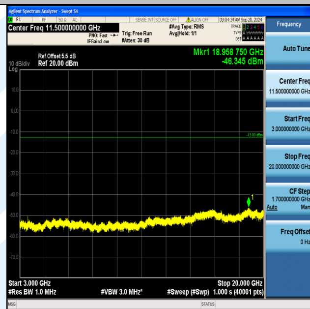
Band66_10MHz_QPSK_132622_1RB#49_3000~20000_3000~20000
