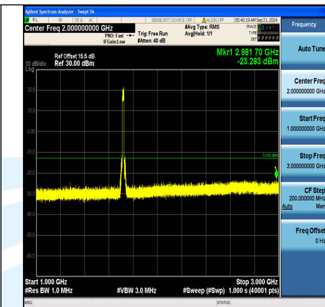
Band66_15MHz_QPSK_132047_75RB#0_1000~3000_1000~3000
