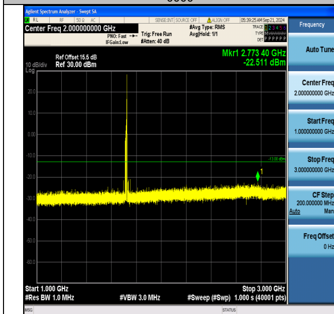
Band66_15MHz_QPSK_132047_1RB#74_1000~3000_1000~3000
