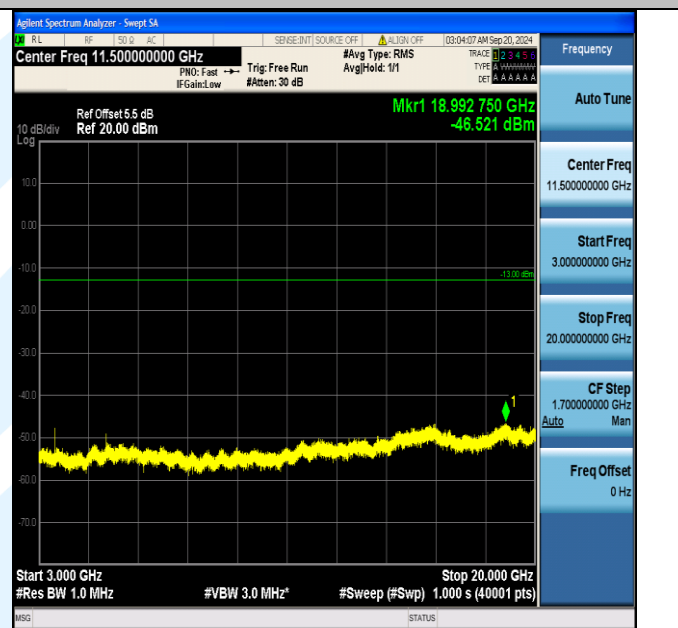
Band66_10MHz_16QAM_132622_1RB#0_3000~20000_3000~20000
