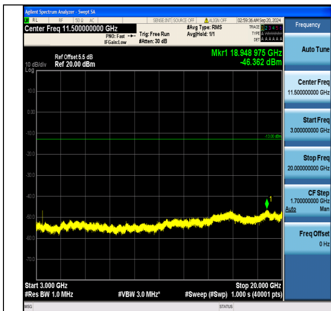
Band66_10MHz_16QAM_132022_1RB#49_3000~20000_3000~20000
