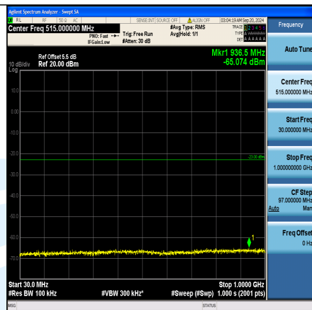
Band66_10MHz_QPSK_132622_1RB#49_30~1000_30~1000
