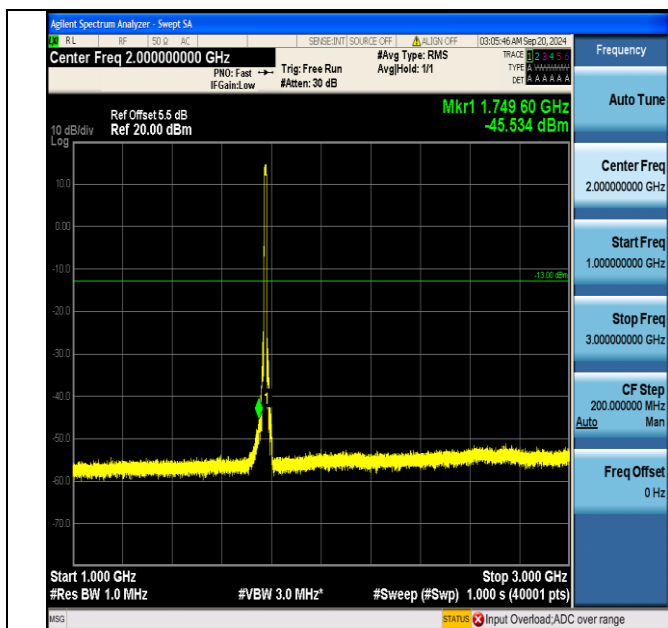
Band66_10MHz_16QAM_132622_50RB#0_1000~3000_1000~3000
