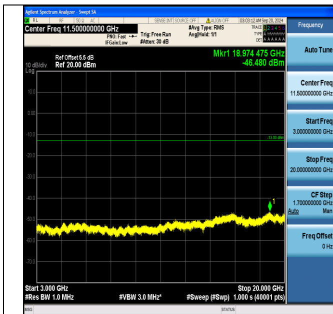
Band66_10MHz_16QAM_132322_50RB#0_3000~20000_3000~20000
