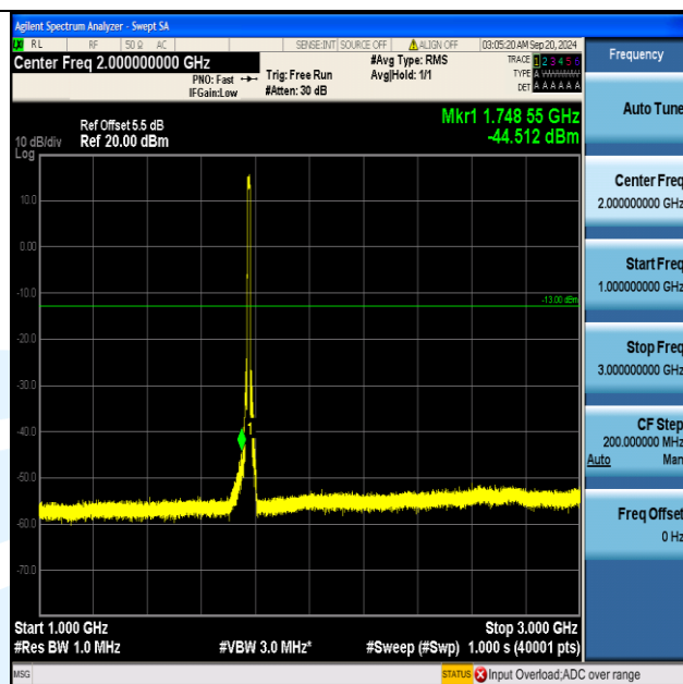
Band66_10MHz_QPSK_132622_50RB#0_1000~3000_1000~3000
