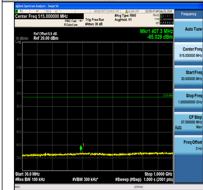
Band66_10MHz_QPSK_132022_50RB#0_30~1000_30~1000
