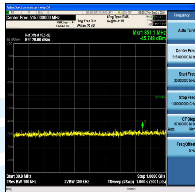
Band66_15MHz_QPSK_132047_1RB#74_30~1000_30~1000
