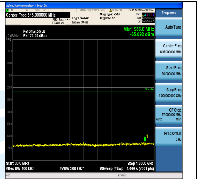
Band66_5MHz_16QAM_131997_1RB#0_30~1000_30~1000
