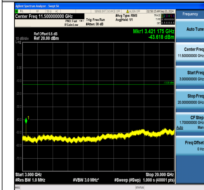
Band66_10MHz_QPSK_132022_1RB#0_3000~20000_3000~20000
