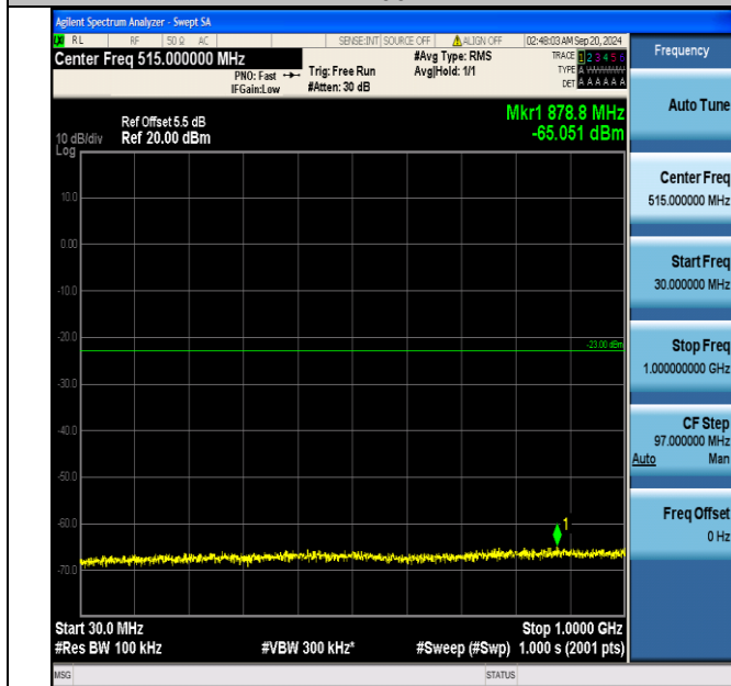
Band66_5MHz_QPSK_132647_25RB#0_30~1000_30~1000
