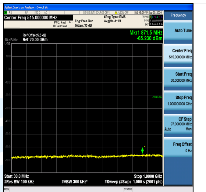
Band66_5MHz_16QAM_132647_25RB#0_30~1000_30~1000
