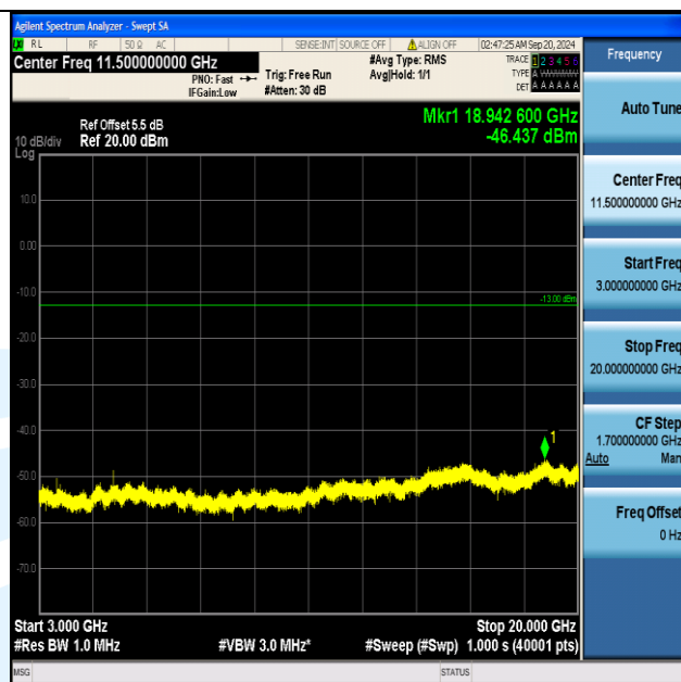
Band66_5MHz_QPSK_132647_1RB#24_3000~20000_3000~20000
