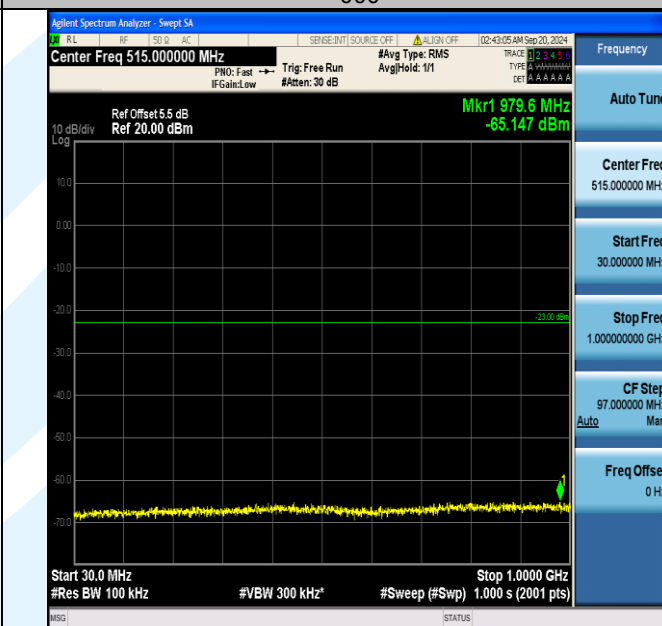
Band66_5MHz_16QAM_131997_25RB#0_30~1000_30~1000
