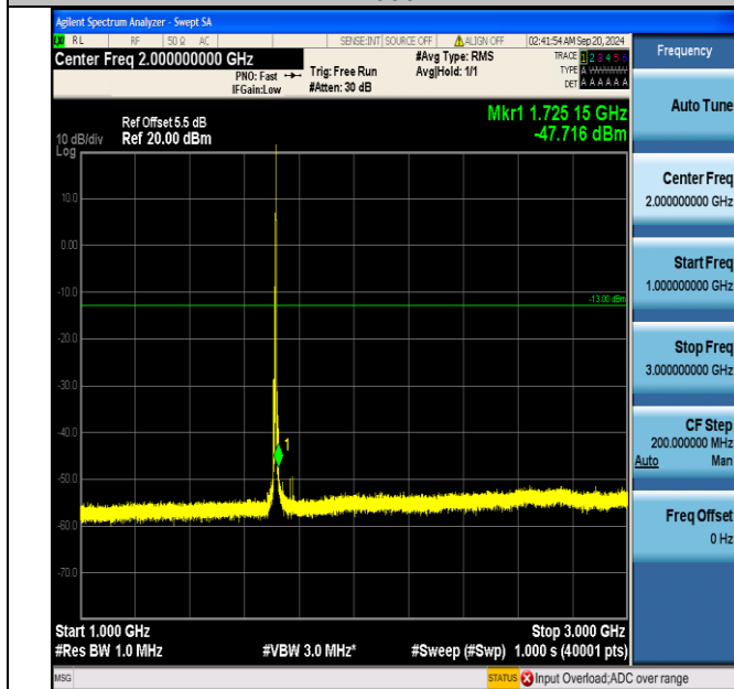
Band66_5MHz_QPSK_131997_1RB#24_1000~3000_1000~3000
