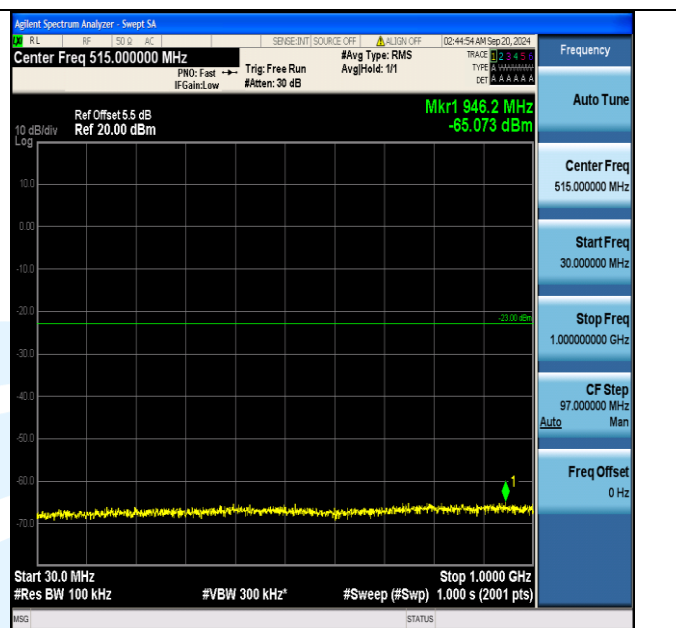
Band66_5MHz_16QAM_132322_1RB#24_30~1000_30~1000
