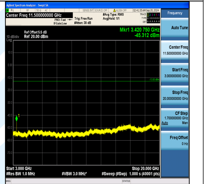
Band66_5MHz_16QAM_131997_1RB#0_3000~20000_3000~20000
