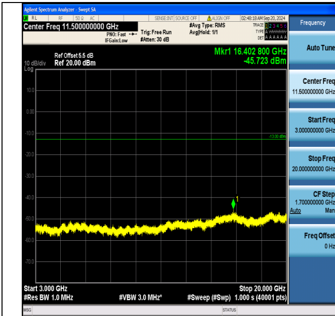
Band66_5MHz_QPSK_132647_25RB#0_3000~20000_3000~20000
