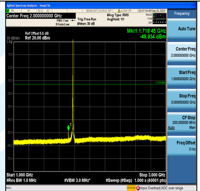
Band66_5MHz_16QAM_132647_1RB#24_1000~3000_1000~3000
