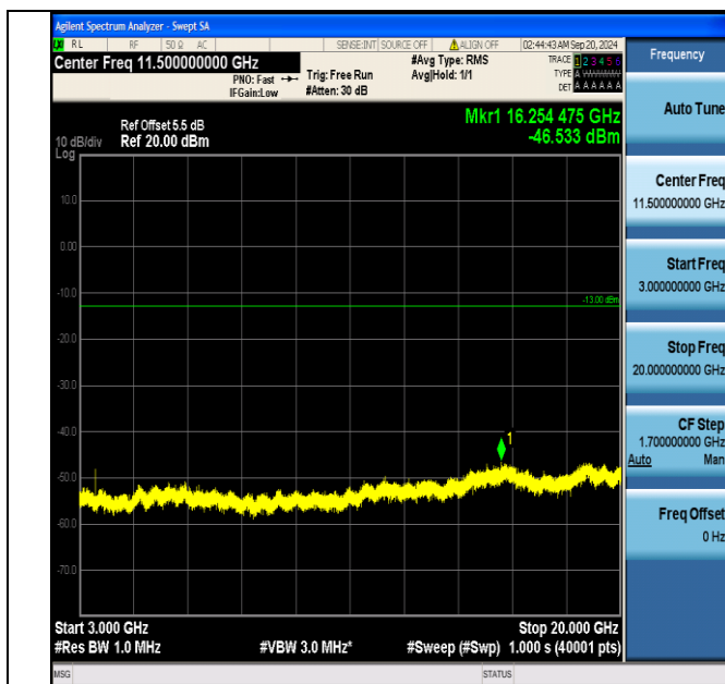
Band66_5MHz_QPSK_132322_1RB#24_3000~20000_3000~20000
