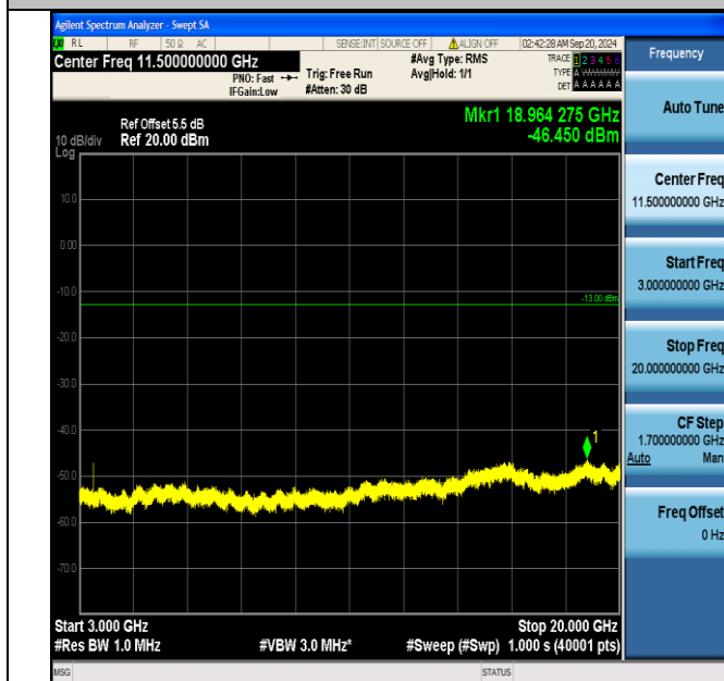
Band66_5MHz_16QAM_131997_1RB#24_3000~20000_3000~20000
