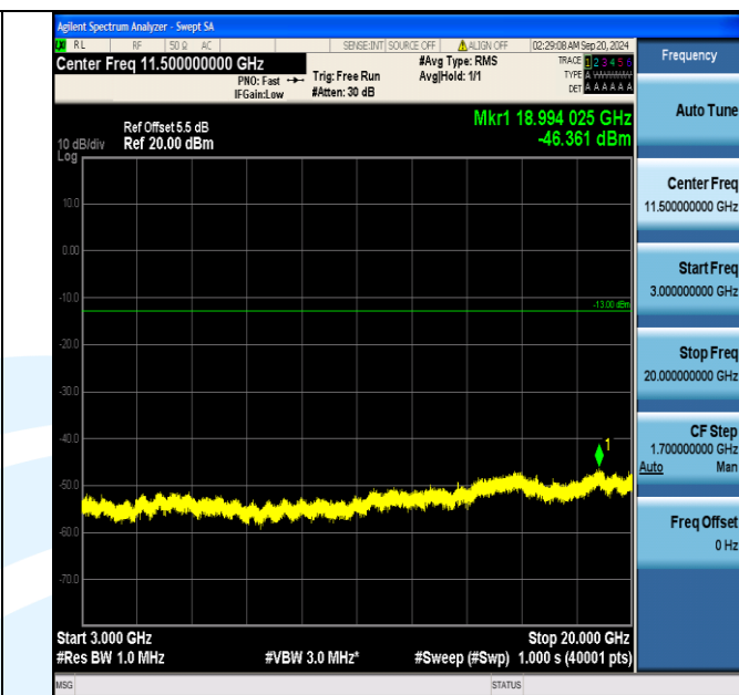
Band66_3MHz_16QAM_132657_15RB#0_3000~20000_3000~20000
