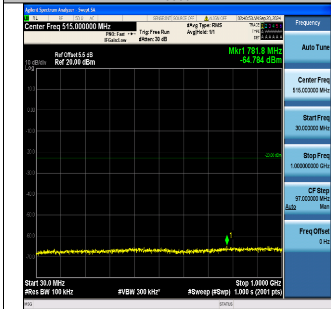
Band66_5MHz_QPSK_131997_1RB#0_30~1000_30~1000
