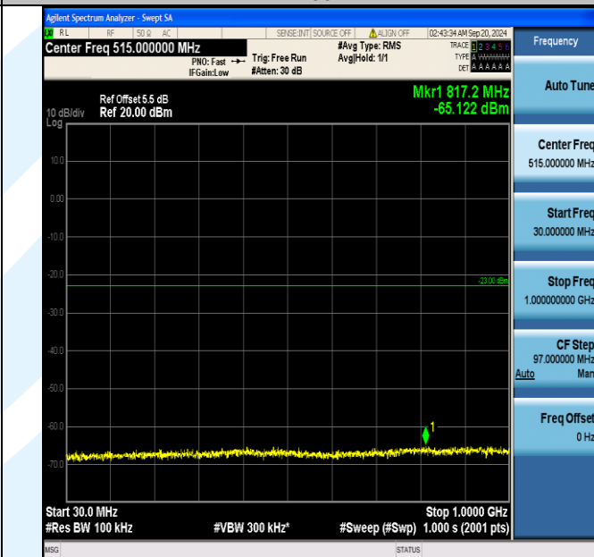
Band66_5MHz_QPSK_132322_1RB#0_30~1000_30~1000
