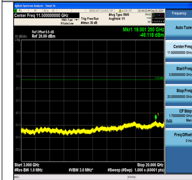
Band66_5MHz_16QAM_132322_25RB#0_3000~20000_3000~20000
