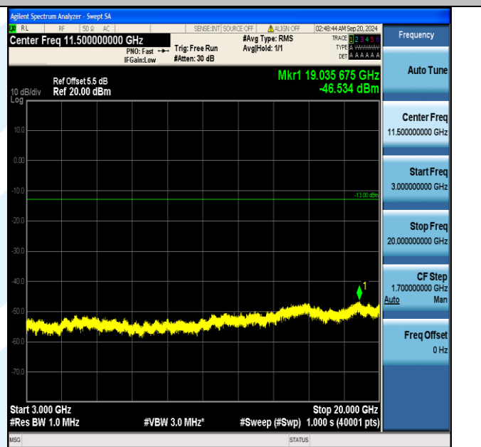
Band66_5MHz_16QAM_132647_25RB#0_3000~20000_3000~20000
