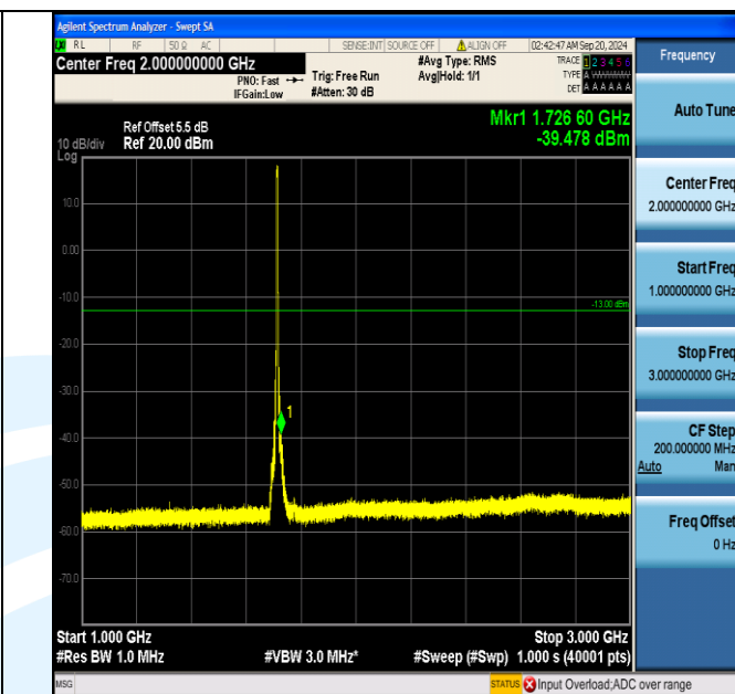
Band66_5MHz_QPSK_131997_25RB#0_1000~3000_1000~3000
