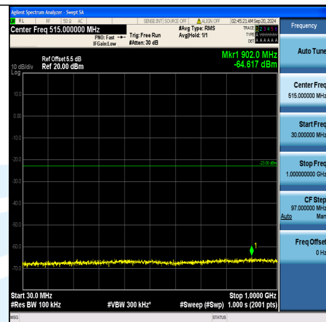
Band66_5MHz_QPSK_132322_25RB#0_30~1000_30~1000
