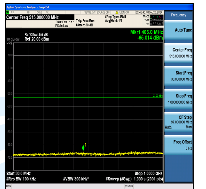
Band66_5MHz_QPSK_131997_1RB#24_30~1000_30~1000
