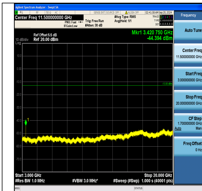
Band66_5MHz_QPSK_131997_1RB#0_3000~20000_3000~20000
