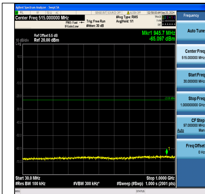
Band66_10MHz_QPSK_132022_1RB#0_30~1000_30~1000
