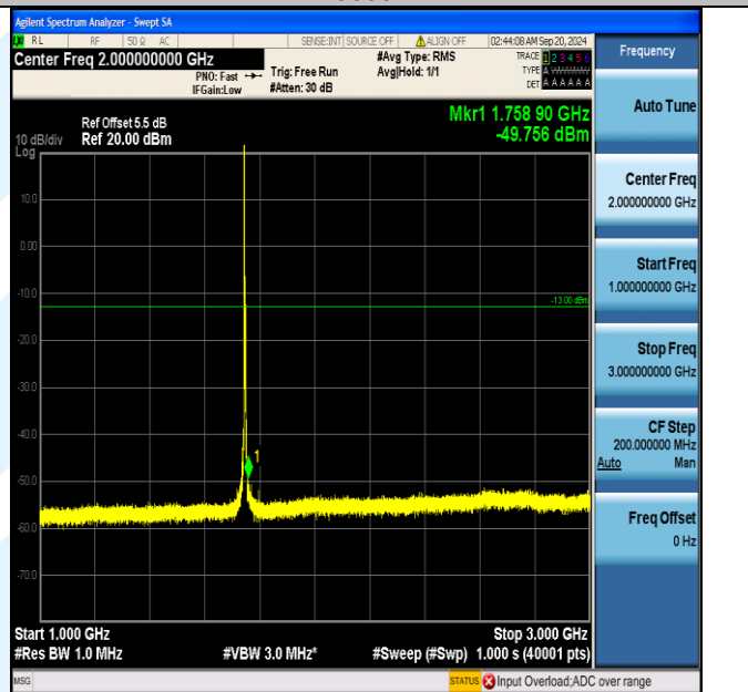
Band66_5MHz_16QAM_132322_1RB#0_1000~3000_1000~3000
