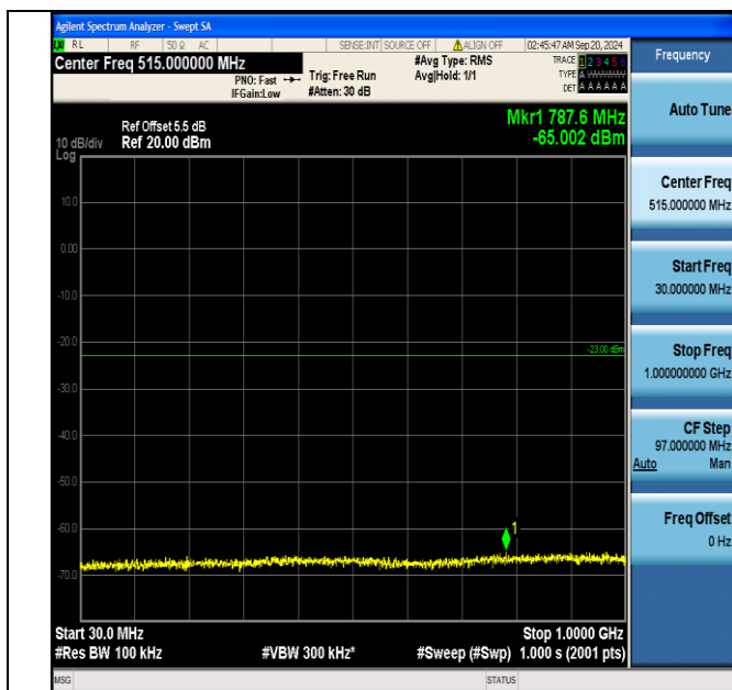
Band66_5MHz_16QAM_132322_25RB#0_30~1000_30~1000
