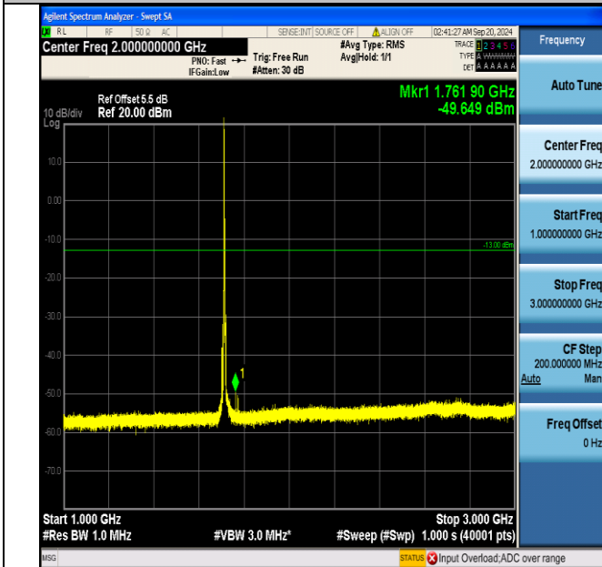
Band66_5MHz_16QAM_131997_1RB#0_1000~3000_1000~3000
