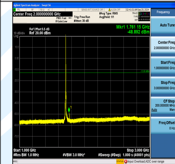
Band66_5MHz_QPSK_131997_1RB#0_1000~3000_1000~3000 0
