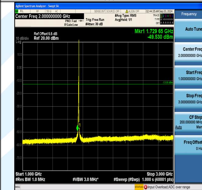
Band66_5MHz_QPSK_132322_1RB#24_1000~3000_1000~3000
