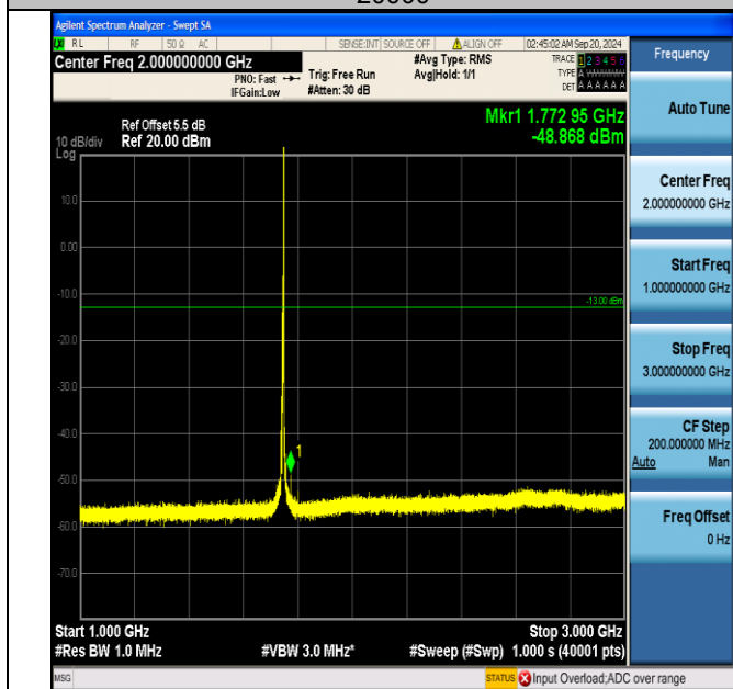
Band66_5MHz_16QAM_132322_1RB#24_1000~3000_1000~3000
