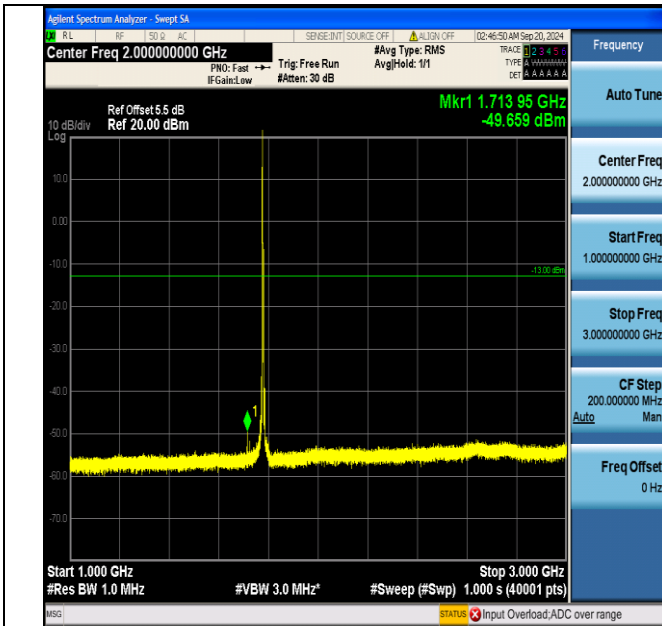
Band66_5MHz_16QAM_132647_1RB#0_1000~3000_1000~3000
