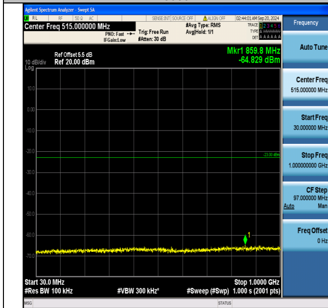
Band66_5MHz_16QAM_132322_1RB#0_30~1000_30~1000
