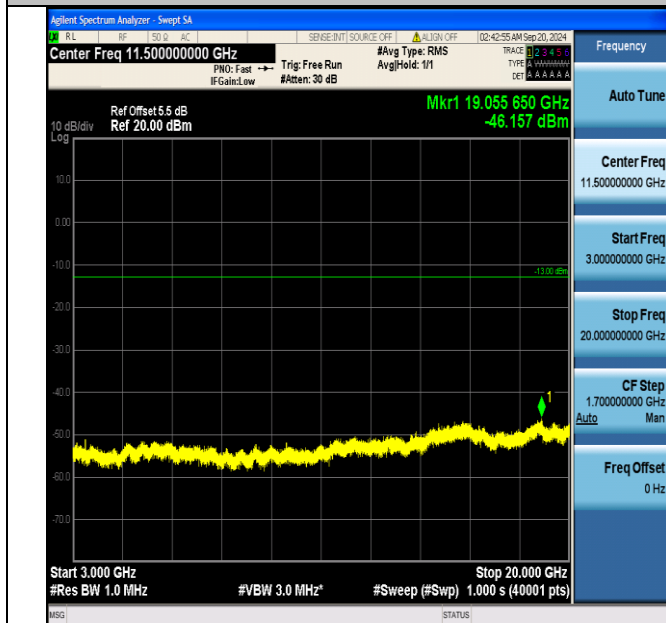
Band66_5MHz_QPSK_131997_25RB#0_3000~20000_3000~20000
