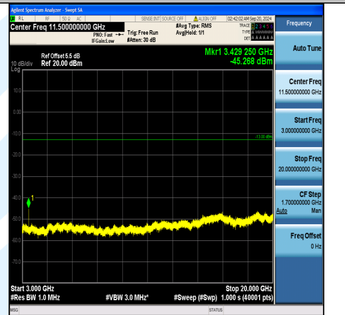
Band66_5MHz_QPSK_131997_1RB#24_3000~20000_3000~20000
