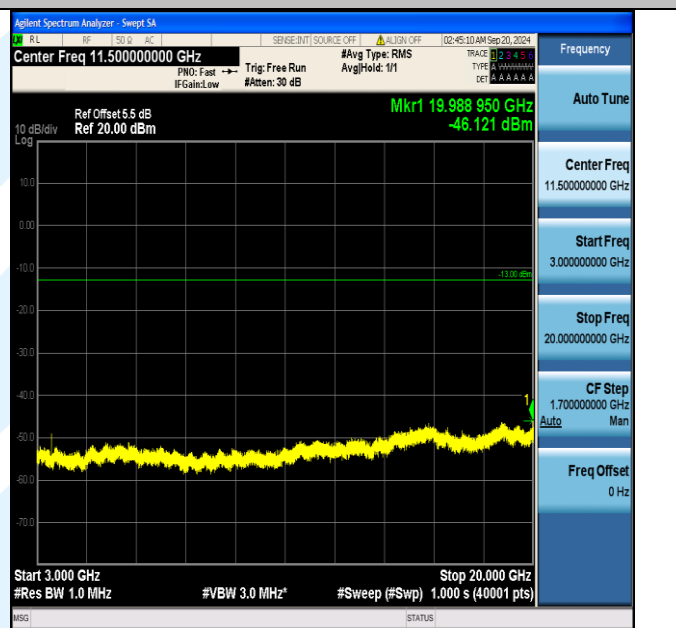
Band66_5MHz_16QAM_132322_1RB#24_3000~20000_3000~20000
