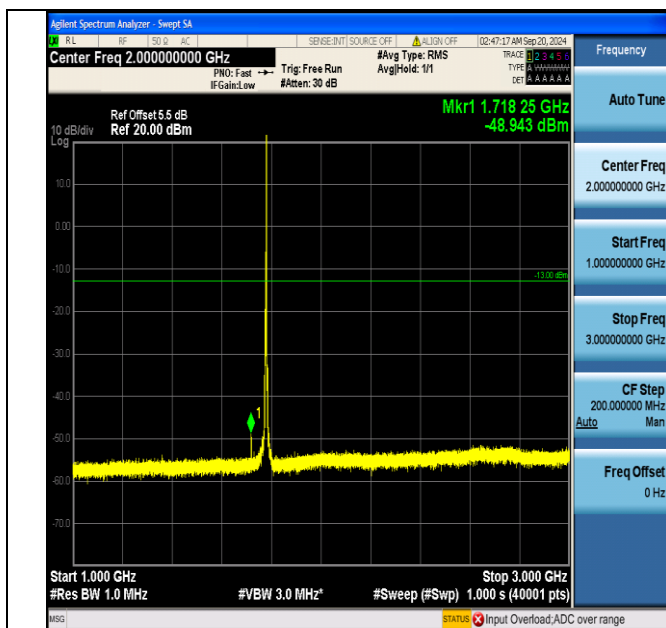
Band66_5MHz_QPSK_132647_1RB#24_1000~3000_1000~3000
