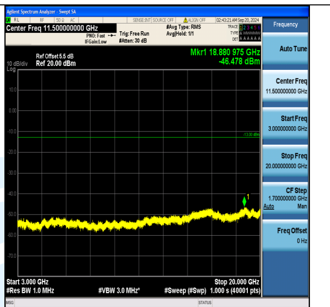
Band66_5MHz_16QAM_131997_25RB#0_3000~20000_3000~20000
