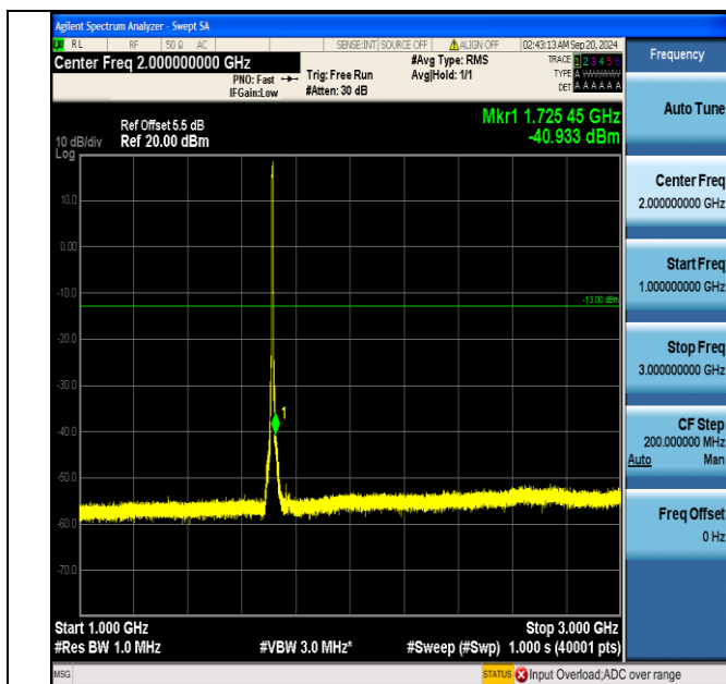
Band66_5MHz_16QAM_131997_25RB#0_1000~3000_1000~3000
