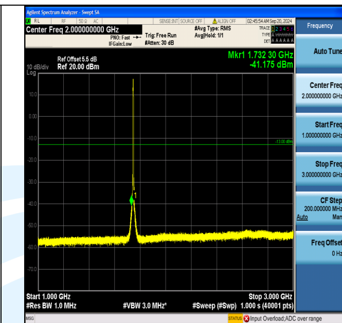
Band66_5MHz_16QAM_132322_25RB#0_1000~3000_1000~3000
