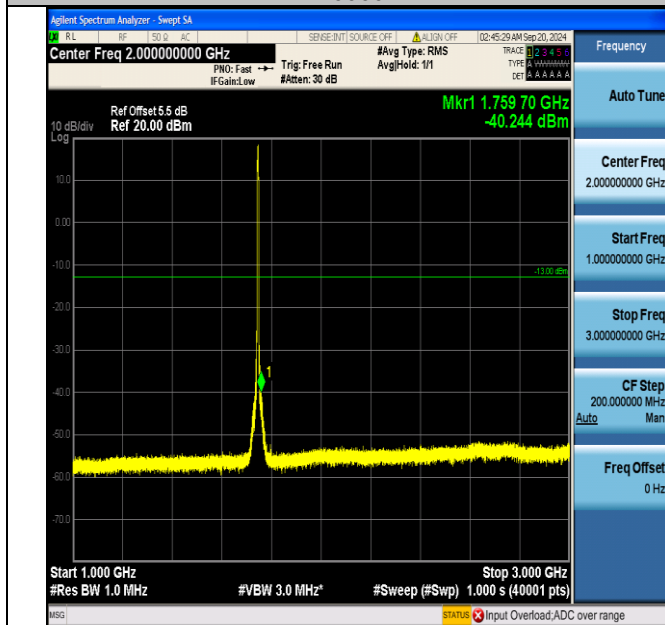
Band66_5MHz_QPSK_132322_25RB#0_1000~3000_1000~3000
