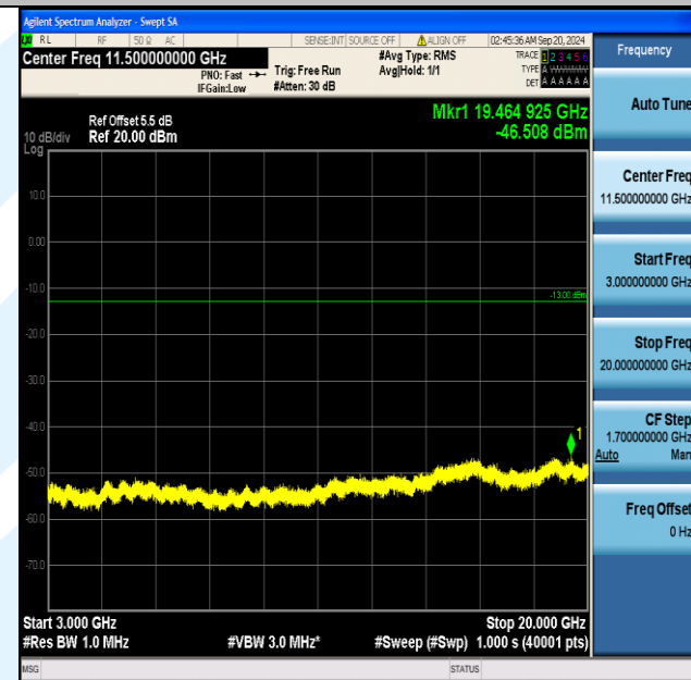
Band66_5MHz_QPSK_132322_25RB#0_3000~20000_3000~20000
