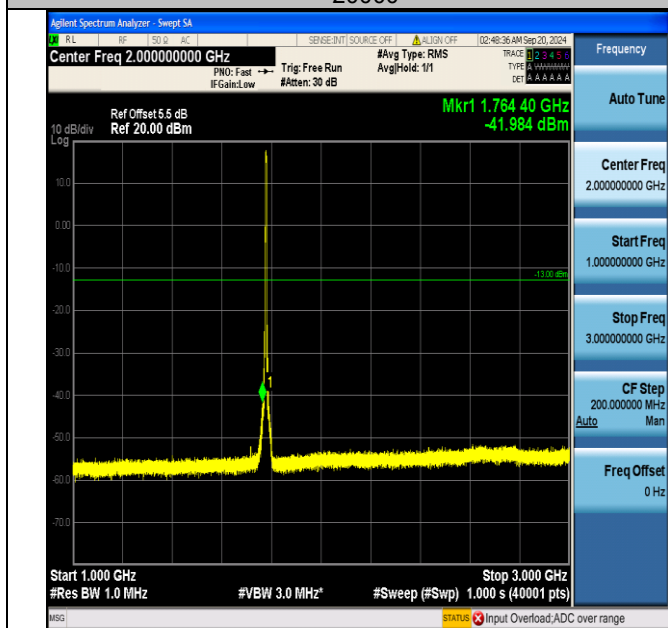
Band66_5MHz_16QAM_132647_25RB#0_1000~3000_1000~3000
