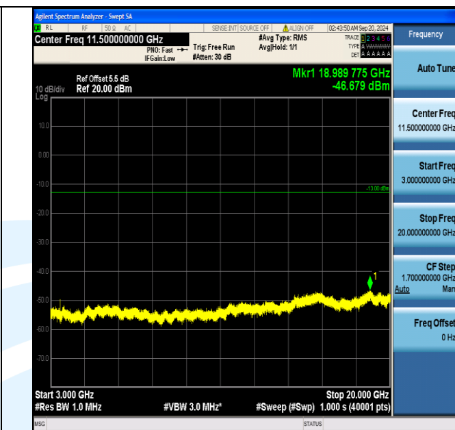
Band66_5MHz_QPSK_132322_1RB#0_3000~20000_3000~20000
