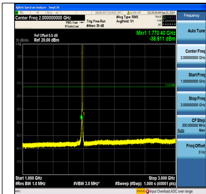
Band66_3MHz_16QAM_132657_15RB#0_1000~3000_1000~3000
