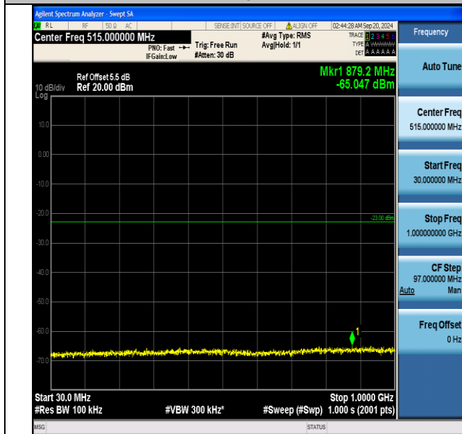
Band66_5MHz_QPSK_132322_1RB#24_30~1000_30~1000
