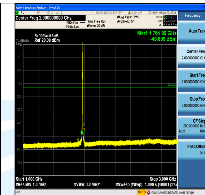
Band66_5MHz_QPSK_132647_1RB#0_1000~3000_1000~3000
