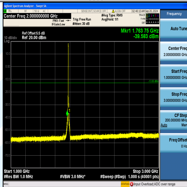
Band66_5MHz_QPSK_132647_25RB#0_1000~3000_1000~3000
