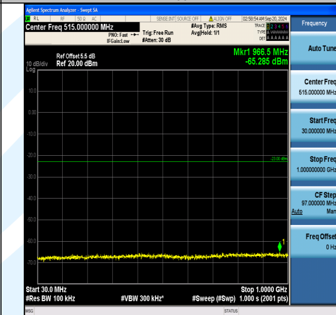
Band66_10MHz_QPSK_132022_1RB#49_30~1000_30~1000
