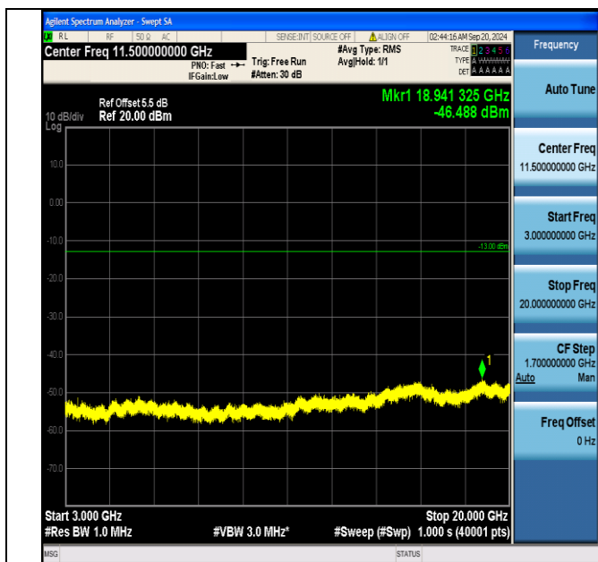
Band66_5MHz_16QAM_132322_1RB#0_3000~20000_3000~20000
