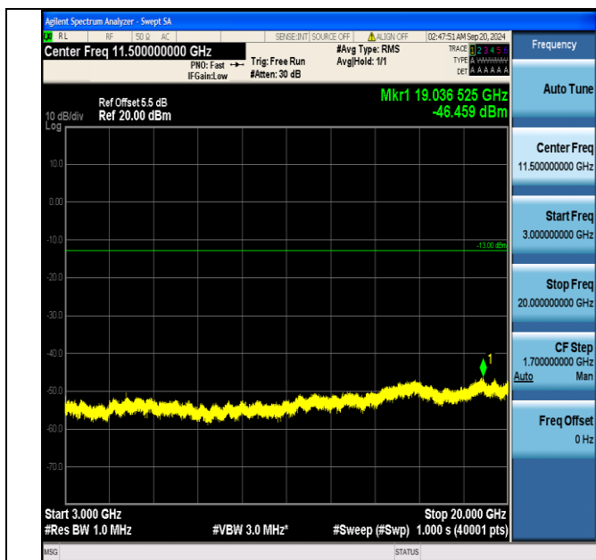
Band66_5MHz_16QAM_132647_1RB#24_3000~20000_3000~20000
