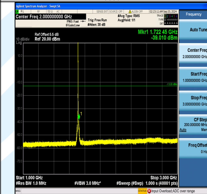
Band66_3MHz_QPSK_131987_15RB#0_1000~3000_1000~3000
