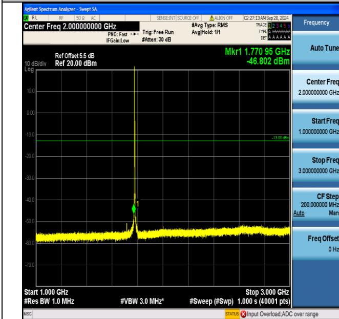
Band66_3MHz_16QAM_132657_1RB#0_1000~3000_1000~3000
