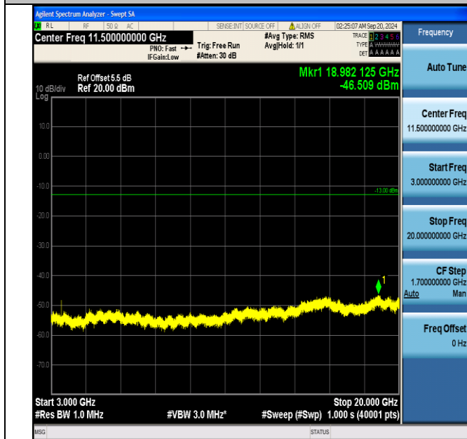
Band66_3MHz_QPSK_132322_1RB#14_3000~20000_3000~20000
