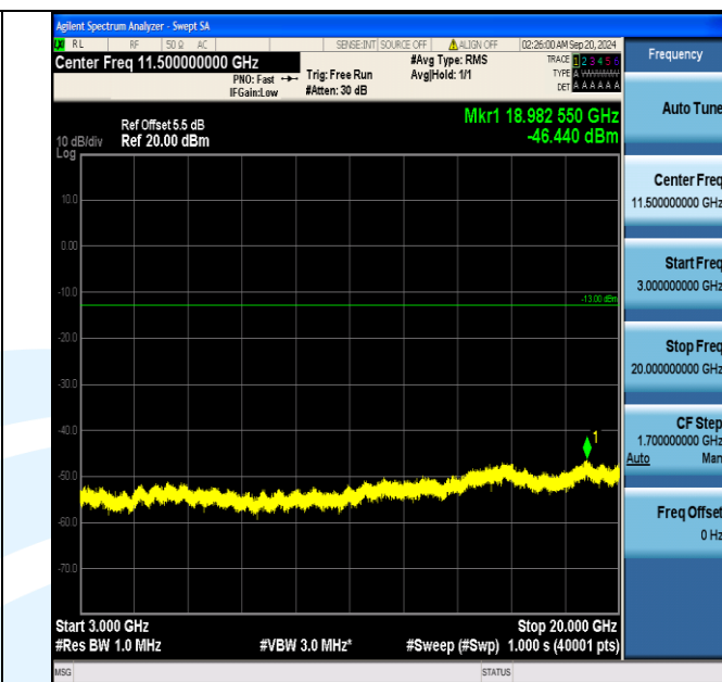
Band66_3MHz_QPSK_132322_15RB#0_3000~20000_3000~20000
