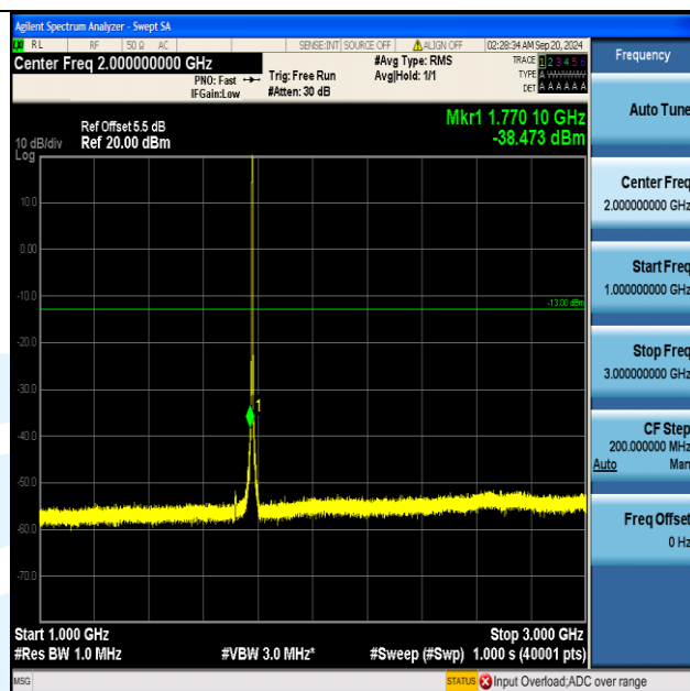
Band66_3MHz_QPSK_132657_15RB#0_1000~3000_1000~3000
