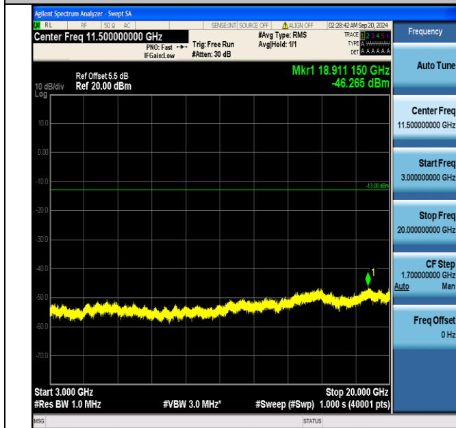
Band66_3MHz_QPSK_132657_15RB#0_3000~20000_3000~20000
