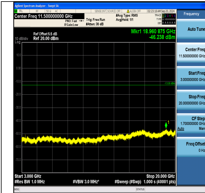
Band66_3MHz_QPSK_131987_15RB#0_3000~20000_3000~20000
