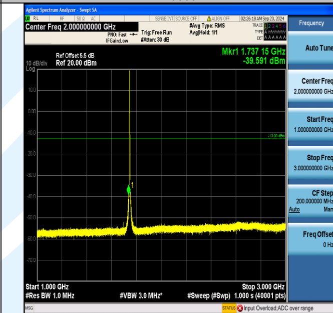
Band66_3MHz_16QAM_132322_15RB#0_1000~3000_1000~3000
