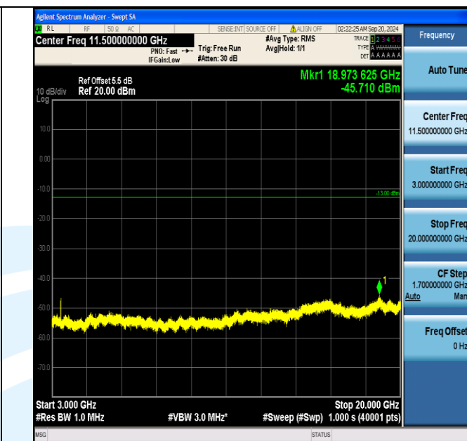
Band66_3MHz_QPSK_131987_1RB#14_3000~20000_3000~20000
