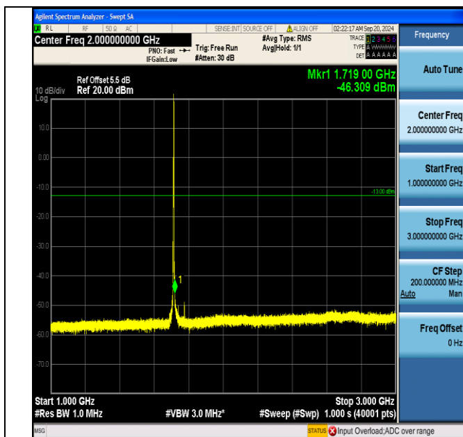
Band66_3MHz_QPSK_131987_1RB#14_1000~3000_1000~3000
