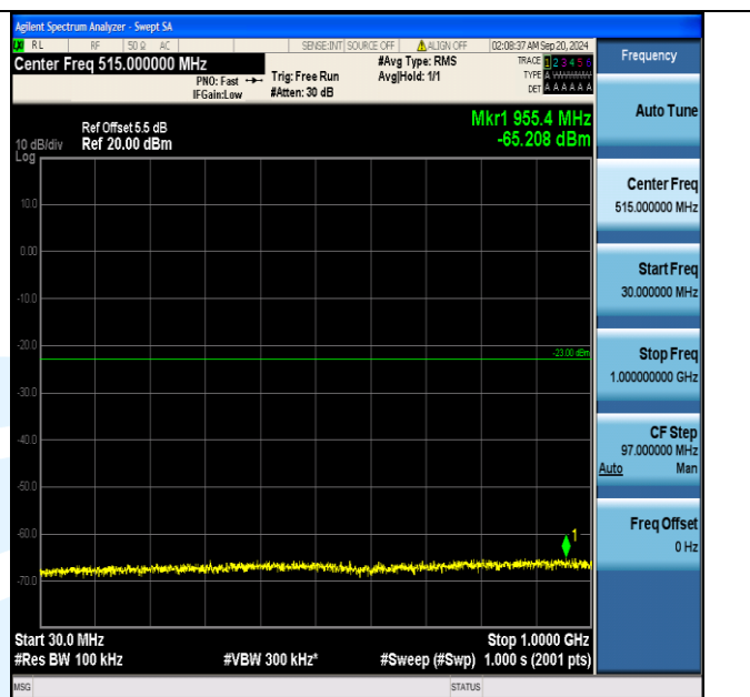
Band66_1.4MHz_16QAM_132665_6RB#0_30~1000_30~1000
