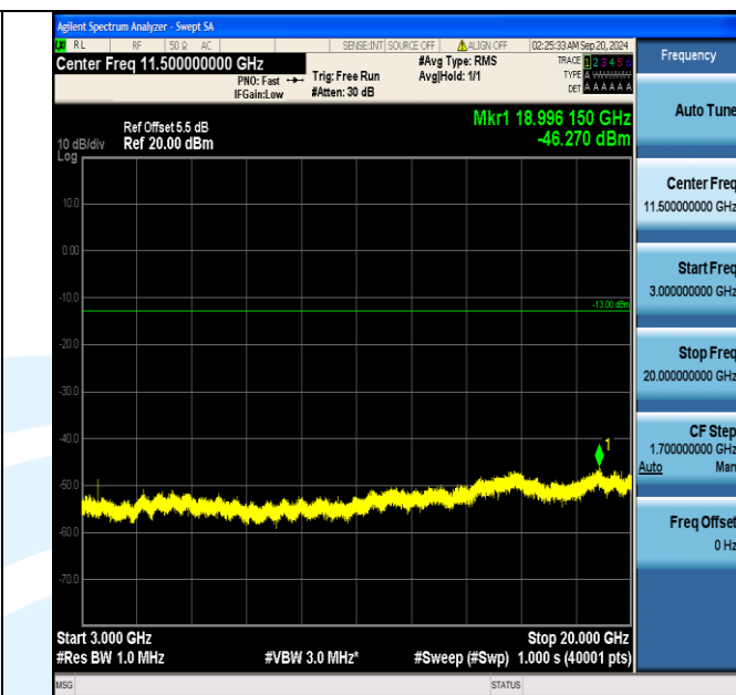
Band66_3MHz_16QAM_132322_1RB#14_3000~20000_3000~20000
