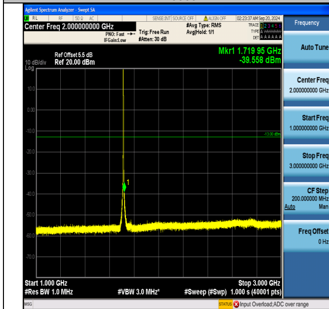
Band66_3MHz_16QAM_131987_15RB#0_1000~3000_1000~3000
