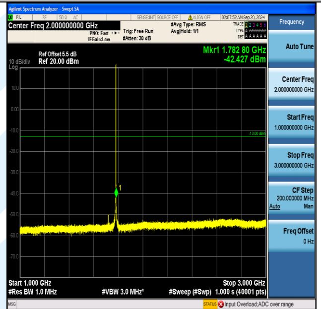
Band66_1.4MHz_16QAM_132665_1RB#5_1000~3000_1000~3000
