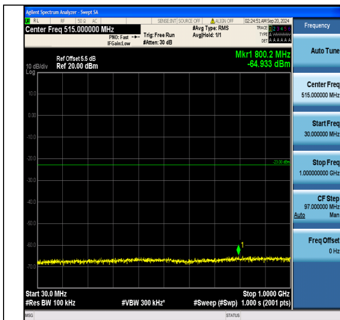
Band66_3MHz_QPSK_132322_1RB#14_30~1000_30~1000
