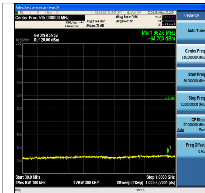
Band66_3MHz_QPSK_132657_15RB#0_30~1000_30~1000
