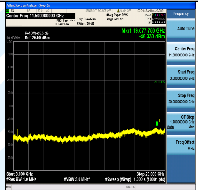
Band66_3MHz_QPSK_132322_1RB#0_3000~20000_3000~20000
