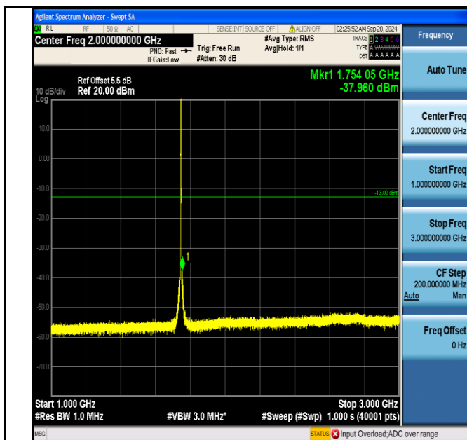
Band66_3MHz_QPSK_132322_15RB#0_1000~3000_1000~3000
