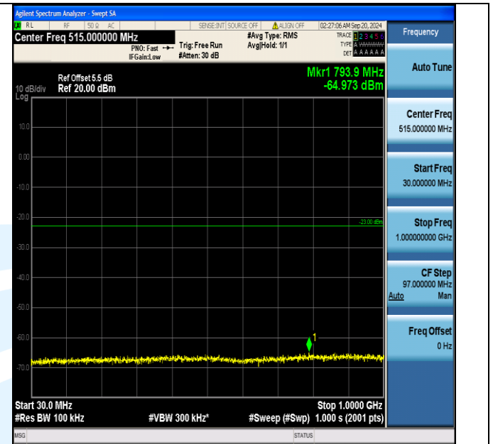
Band66_3MHz_16QAM_132657_1RB#0_30~1000_30~1000
