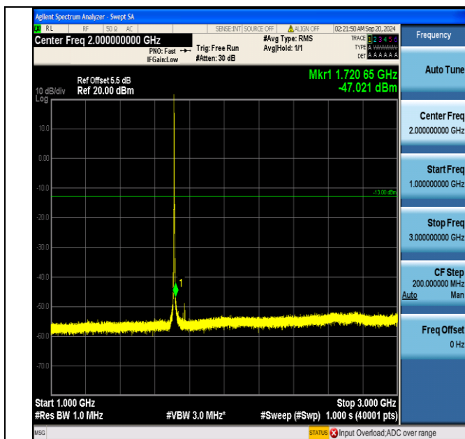
Band66_3MHz_16QAM_131987_1RB#0_1000~3000_1000~3000
