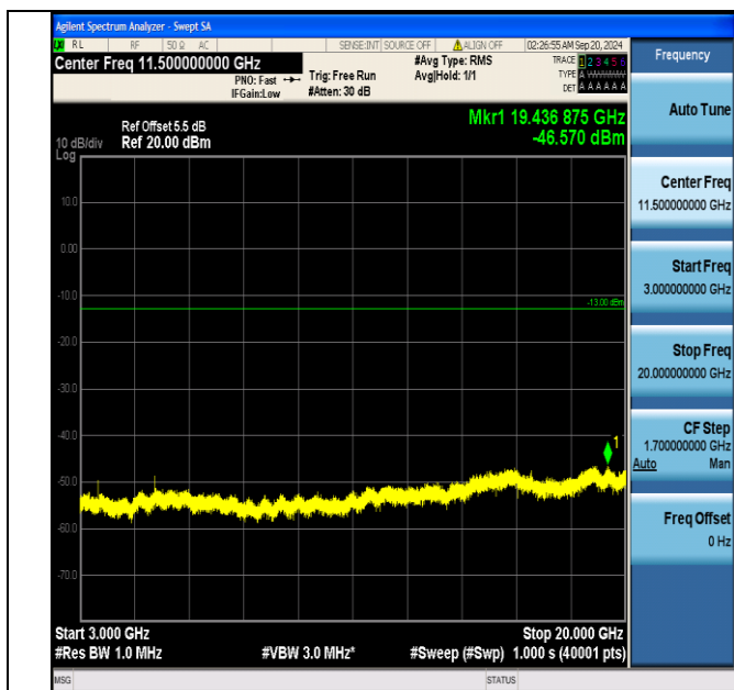
Band66_3MHz_QPSK_132657_1RB#0_3000~20000_3000~20000
