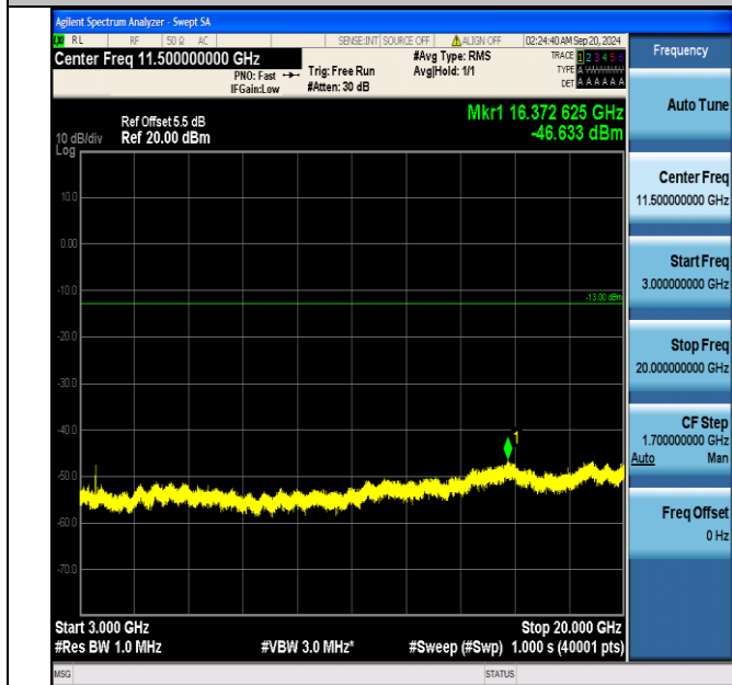
Band66_3MHz_16QAM_132322_1RB#0_3000~20000_3000~20000
