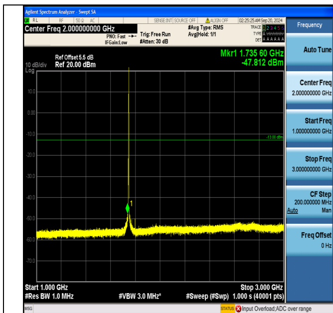
Band66_3MHz_16QAM_132322_1RB#14_1000~3000_1000~3000
