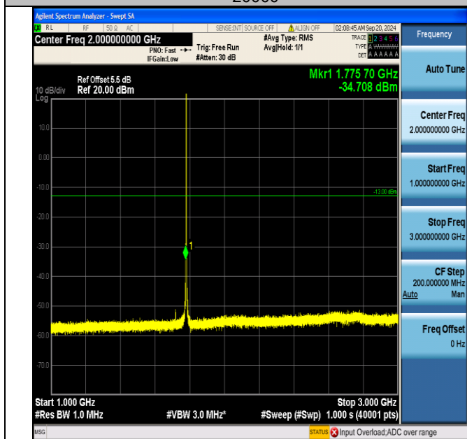
Band66_1.4MHz_16QAM_132665_6RB#0_1000~3000_1000~3000
