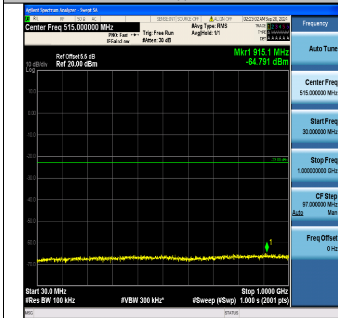
Band66_3MHz_QPSK_131987_15RB#0_30~1000_30~1000
