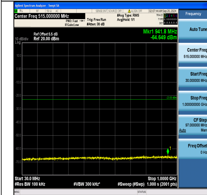
Band66_1.4MHz_16QAM_132665_1RB#5_30~1000_30~1000
