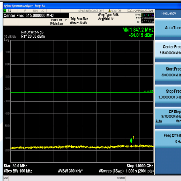
Band66_3MHz_16QAM_131987_1RB#0_30~1000_30~1000
