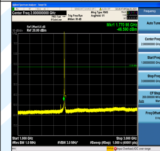
Band66_3MHz_QPSK_132657_1RB#0_1000~3000_1000~3000
