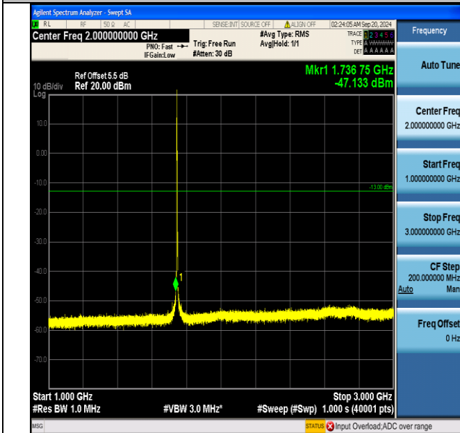
Band66_3MHz_QPSK_132322_1RB#0_1000~3000_1000~3000
