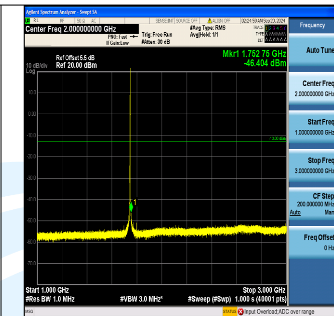
Band66_3MHz_QPSK_132322_1RB#14_1000~3000_1000~3000
