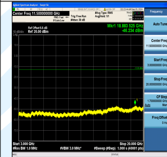
Band66_3MHz_16QAM_131987_15RB#0_3000~20000_3000~20000
