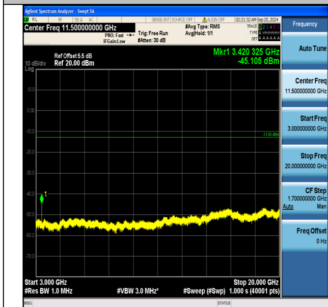
Band66_3MHz_QPSK_131987_1RB#0_3000~20000_3000~20000
