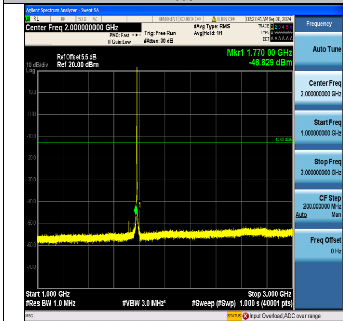
Band66_3MHz_QPSK_132657_1RB#14_1000~3000_1000~3000
