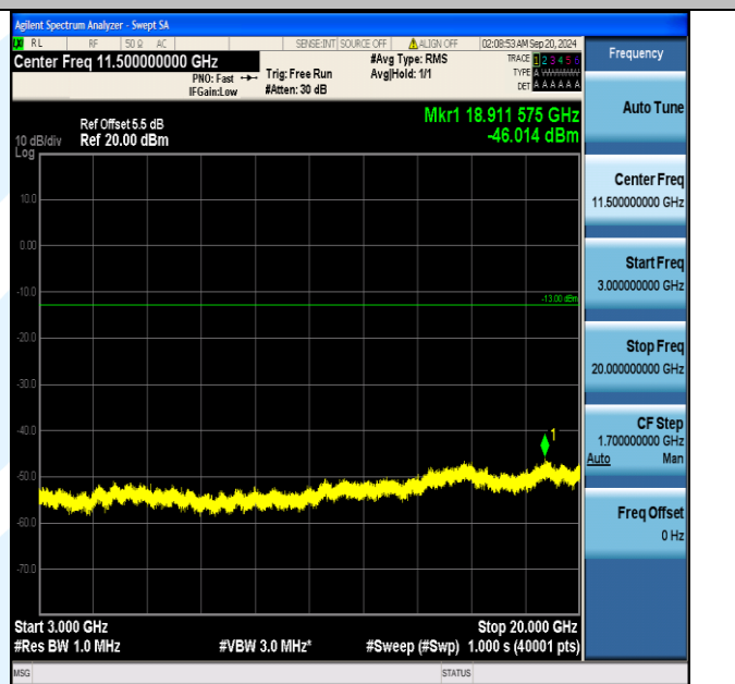
Band66_1.4MHz_16QAM_132665_6RB#0_3000~20000_3000~20000
