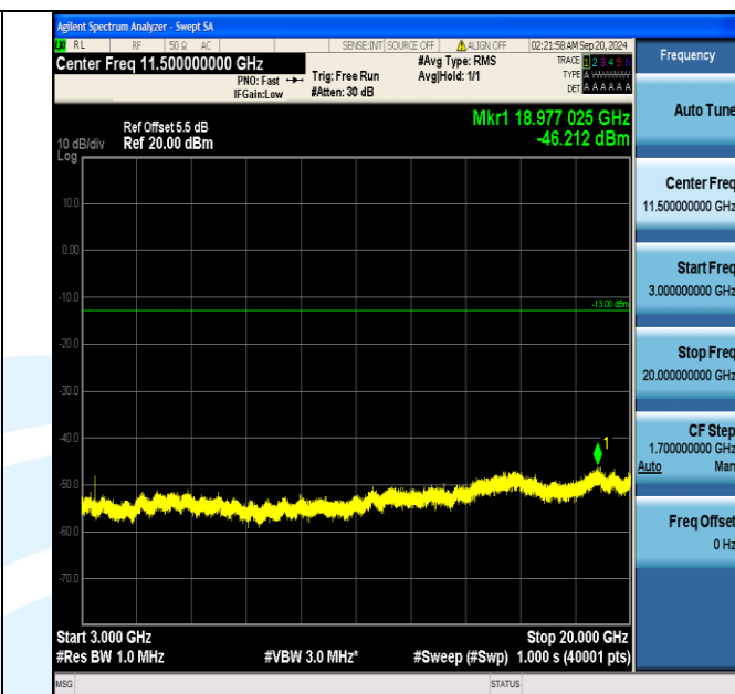
Band66_3MHz_16QAM_131987_1RB#0_3000~20000_3000~20000
