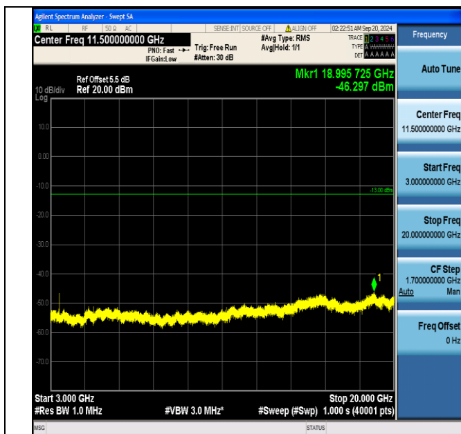
Band66_3MHz_16QAM_131987_1RB#14_3000~20000_3000~20000
