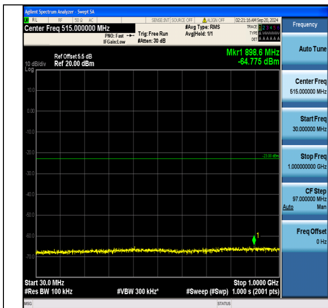
Band66_3MHz_QPSK_131987_1RB#0_30~1000_30~1000
