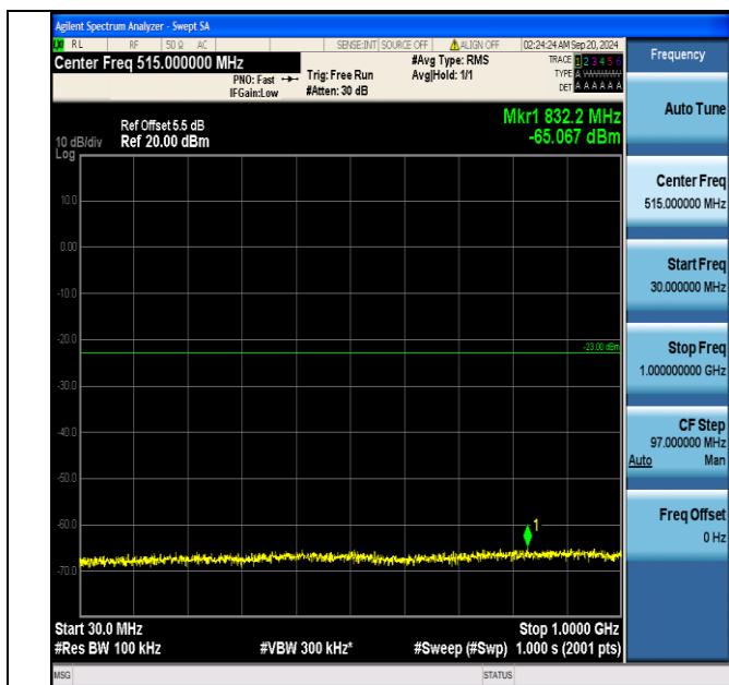
Band66_3MHz_16QAM_132322_1RB#0_30~1000_30~1000
