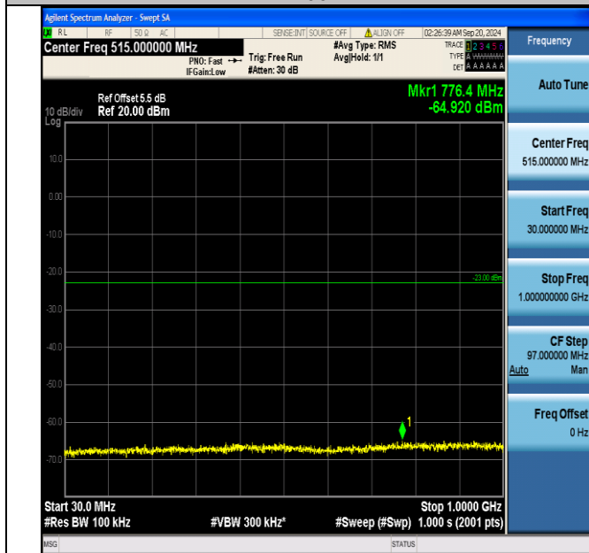
Band66_3MHz_QPSK_132657_1RB#0_30~1000_30~1000
