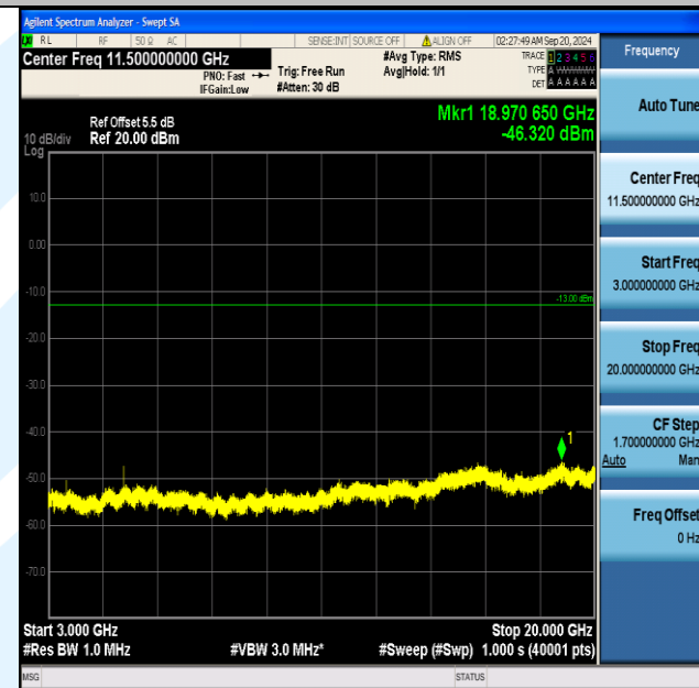
Band66_3MHz_QPSK_132657_1RB#14_3000~20000_3000~20000
