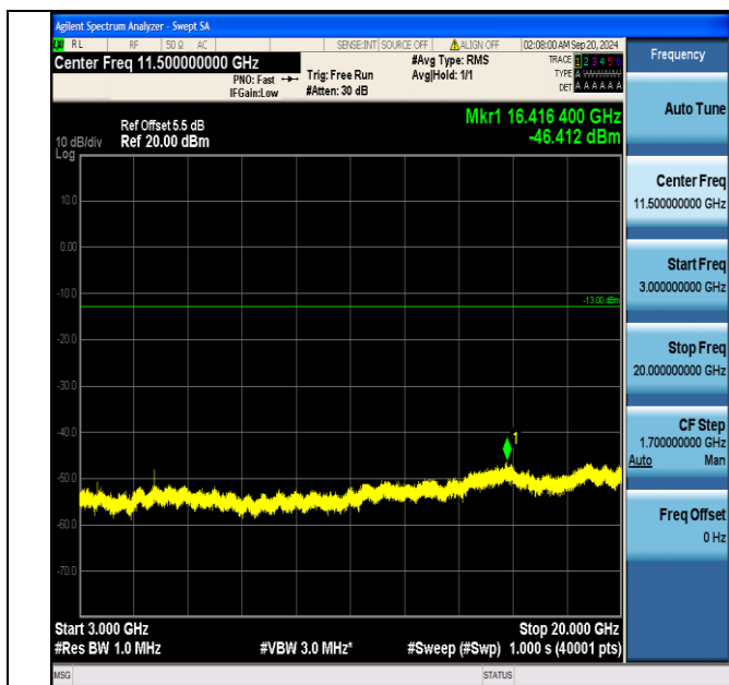
Band66_1.4MHz_16QAM_132665_1RB#5_3000~20000_3000~20000
