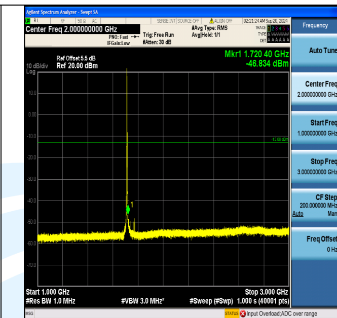
Band66_3MHz_QPSK_131987_1RB#0_1000~3000_1000~3000
