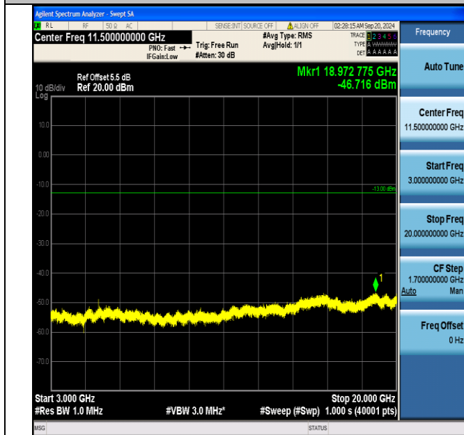
Band66_3MHz_16QAM_132657_1RB#14_3000~20000_3000~20000
