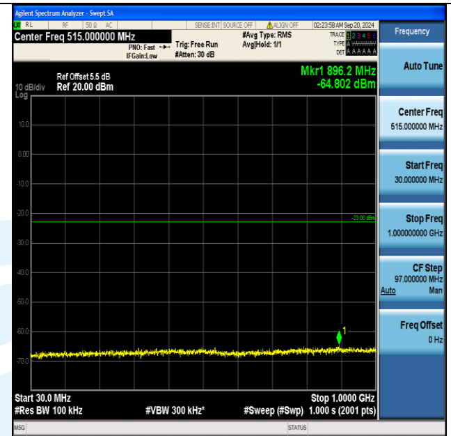
Band66_3MHz_QPSK_132322_1RB#0_30~1000_30~1000
