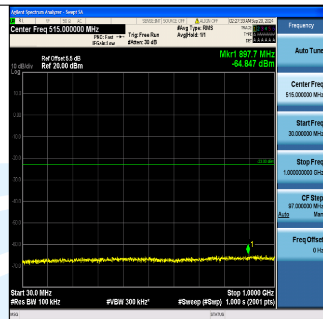
Band66_3MHz_QPSK_132657_1RB#14_30~1000_30~1000
