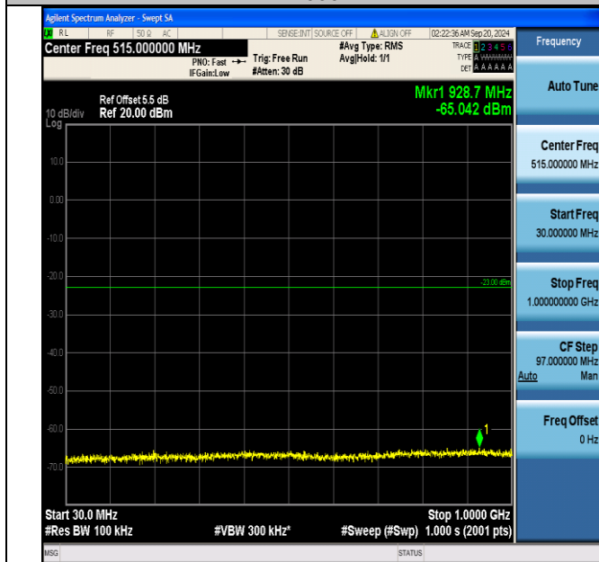
Band66_3MHz_16QAM_131987_1RB#14_30~1000_30~1000
