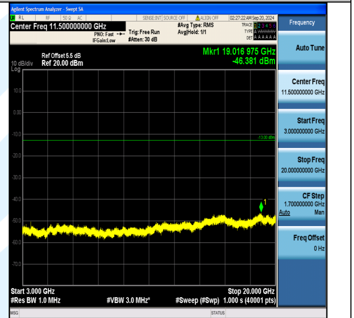
Band66_3MHz_16QAM_132657_1RB#0_3000~20000_3000~20000
