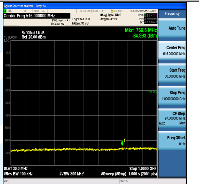
Band66_3MHz_16QAM_132657_15RB#0_30~1000_30~1000
