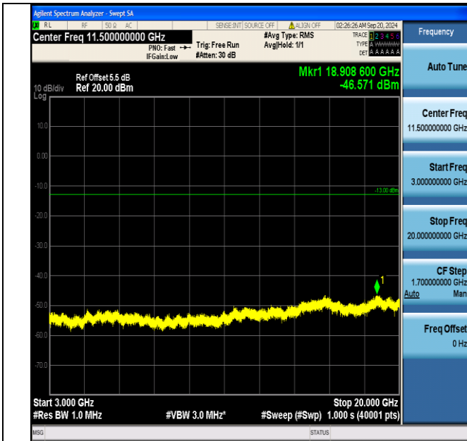
Band66_3MHz_16QAM_132322_15RB#0_3000~20000_3000~20000
