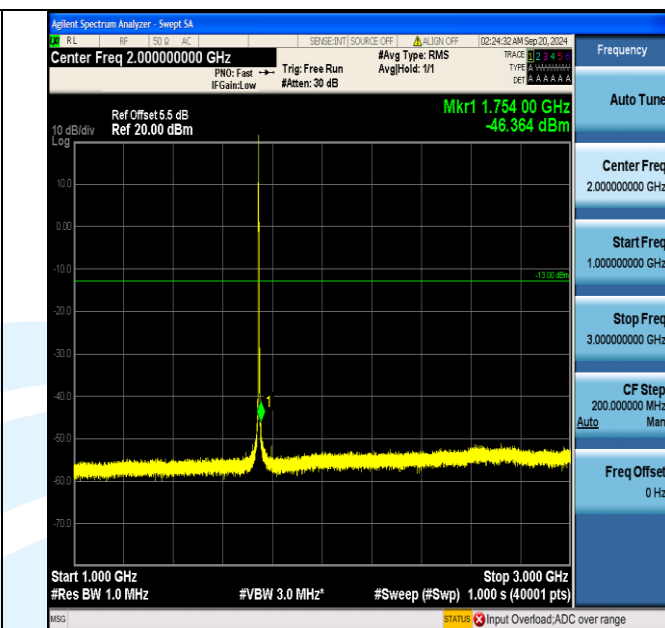
Band66_3MHz_16QAM_132322_1RB#0_1000~3000_1000~3000
