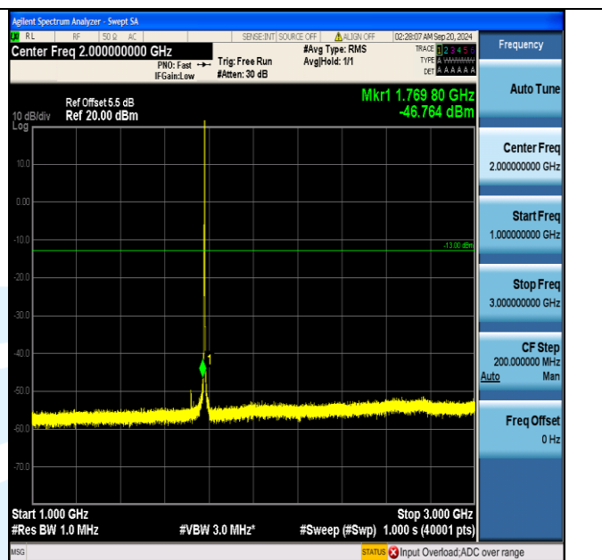
Band66_3MHz_16QAM_132657_1RB#14_1000~3000_1000~3000
