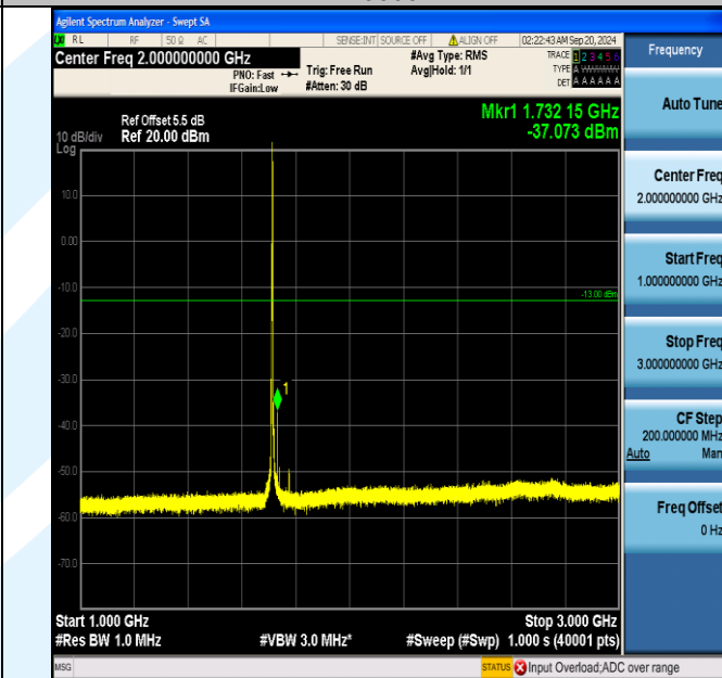
Band66_3MHz_16QAM_131987_1RB#14_1000~3000_1000~3000
