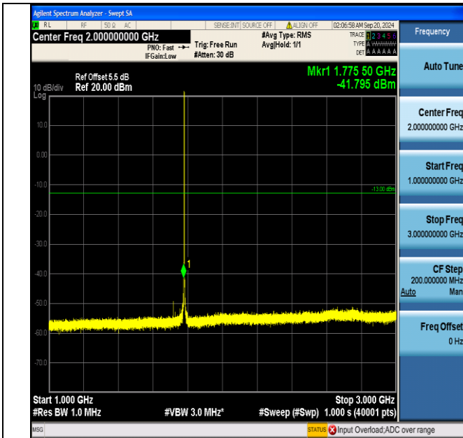
Band66_1.4MHz_16QAM_132665_1RB#0_1000~3000_1000~3000
