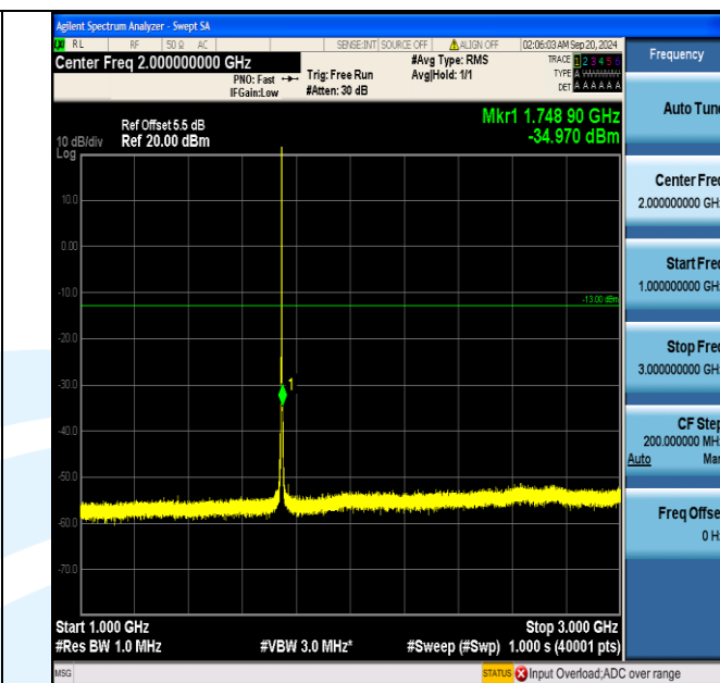
Band66_1.4MHz_16QAM_132322_6RB#0_1000~3000_1000~3000
