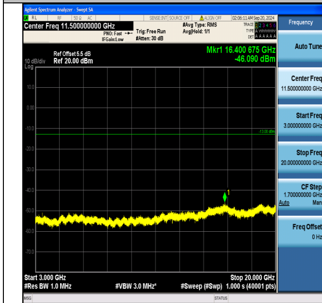
Band66_1.4MHz_16QAM_132322_6RB#0_3000~20000_3000~20000
