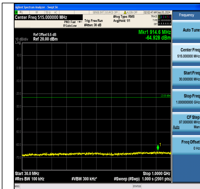
Band66_1.4MHz_QPSK_131979_6RB#0_30~1000_30~1000
