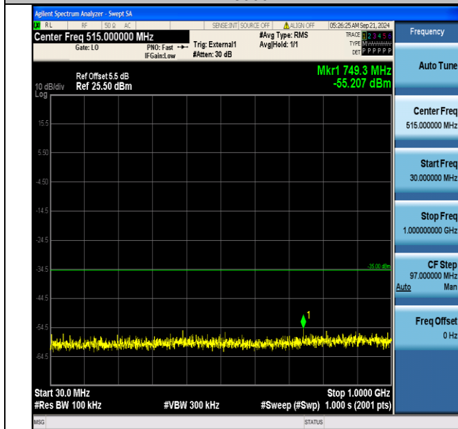
Band41_20MHz_16QAM_41140_100RB#0_30~1000_30~1000
