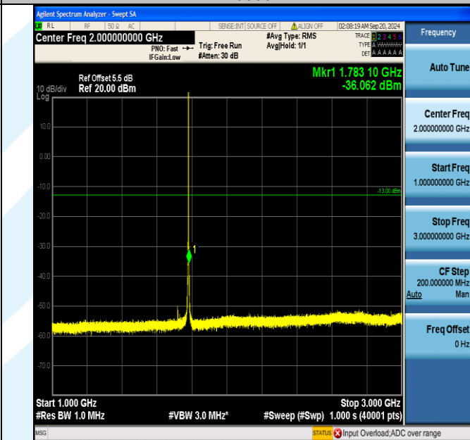
Band66_1.4MHz_QPSK_132665_6RB#0_1000~3000_1000~3000
