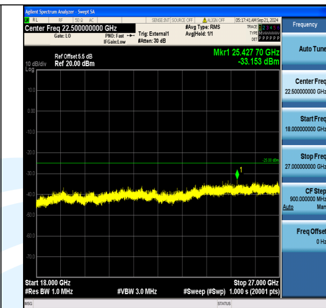
Band41_20MHz_16QAM_40690_100RB#0_18000~27000_18000~27000
