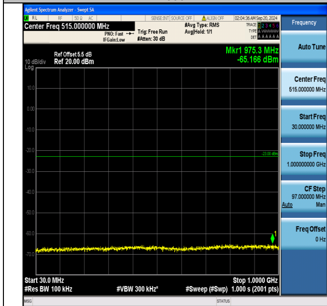
Band66_1.4MHz_QPSK_132322_1RB#5_30~1000_30~1000
