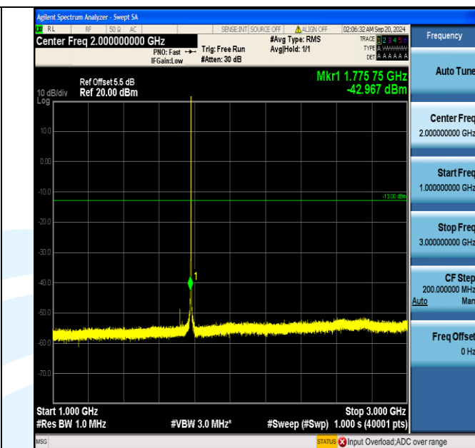
Band66_1.4MHz_QPSK_132665_1RB#0_1000~3000_1000~3000
