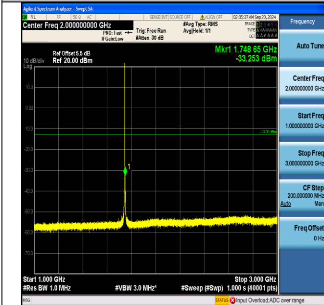
Band66_1.4MHz_QPSK_132322_6RB#0_1000~3000_1000~3000
