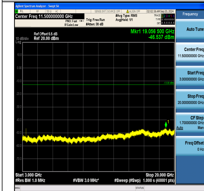
Band66_1.4MHz_16QAM_131979_1RB#5_3000~20000_3000~20000
