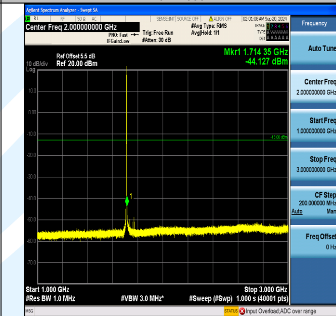
Band66_1.4MHz_QPSK_131979_1RB#0_1000~3000_1000~3000
