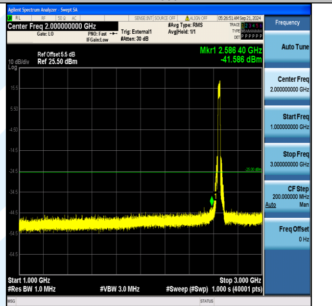
Band41_20MHz_16QAM_41140_100RB#0_1000~3000_1000~3000
