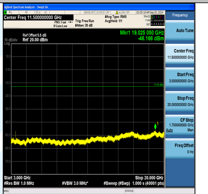
Band66_1.4MHz_16QAM_132322_1RB#5_3000~20000_3000~20000
