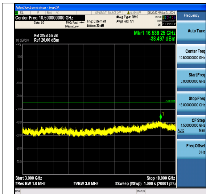
Band41_20MHz_16QAM_41140_1RB#0_3000~18000_3000~18000
