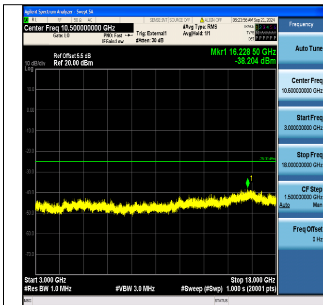
Band41_20MHz_16QAM_41140_1RB#99_3000~18000_3000~18000
