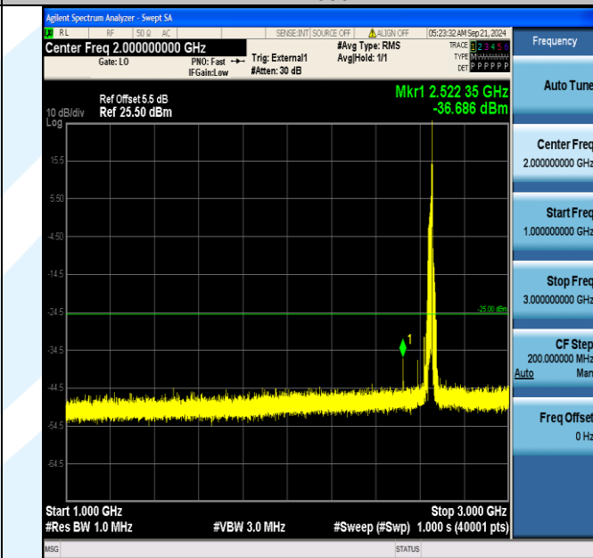
Band41_20MHz_16QAM_41140_1RB#99_1000~3000_1000~3000
