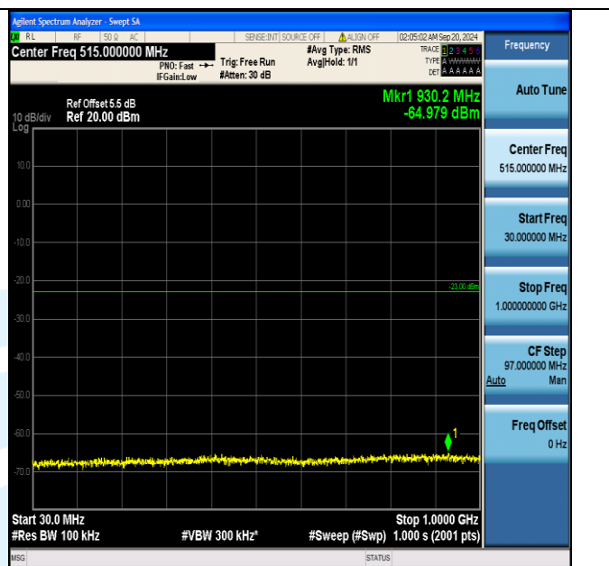
Band66_1.4MHz_16QAM_132322_1RB#5_30~1000_30~1000
