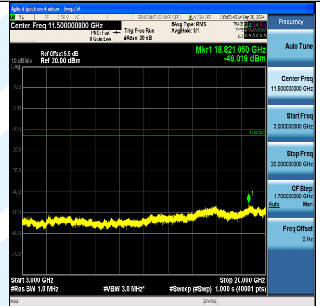
Band66_1.4MHz_QPSK_132322_6RB#0_3000~20000_3000~20000
