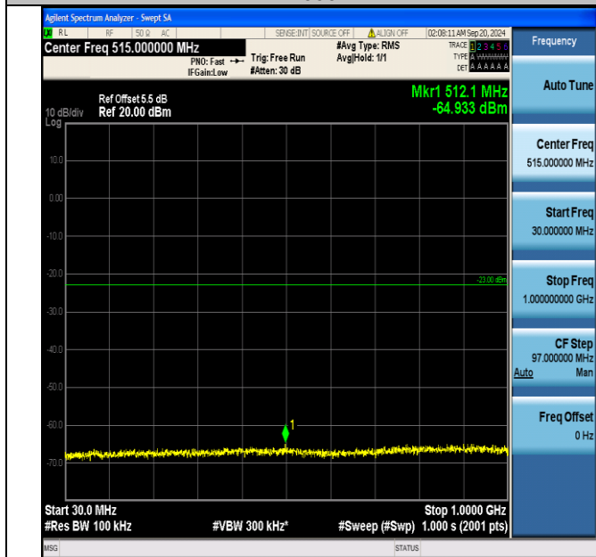
Band66_1.4MHz_QPSK_132665_6RB#0_30~1000_30~1000
