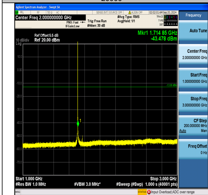
Band66_1.4MHz_QPSK_131979_1RB#5_1000~3000_1000~3000
