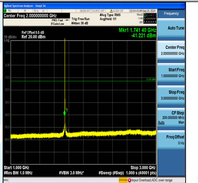
Band66_1.4MHz_QPSK_132322_1RB#5_1000~3000_1000~3000
