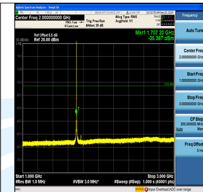
Band66_1.4MHz_QPSK_131979_6RB#0_1000~3000_1000~3000
