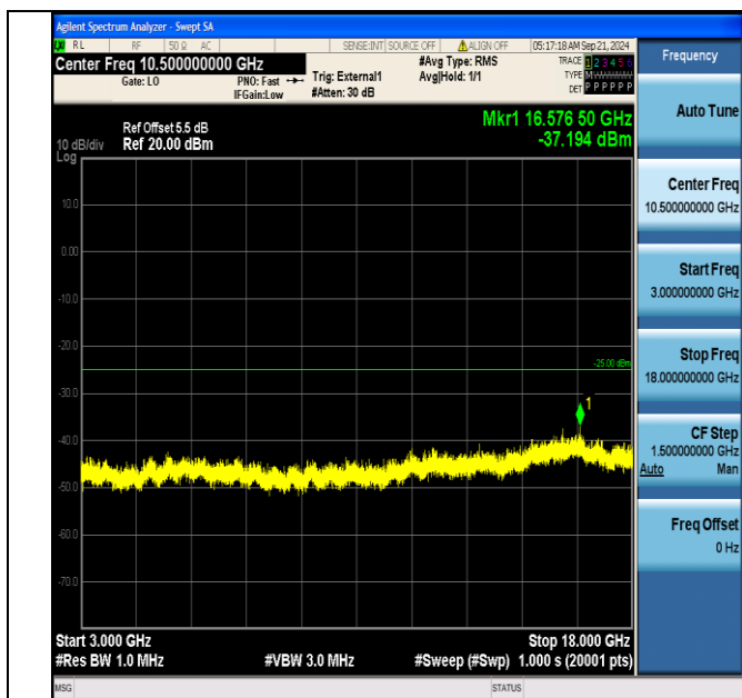
Band41_20MHz_16QAM_40690_100RB#0_3000~18000_3000~18000
