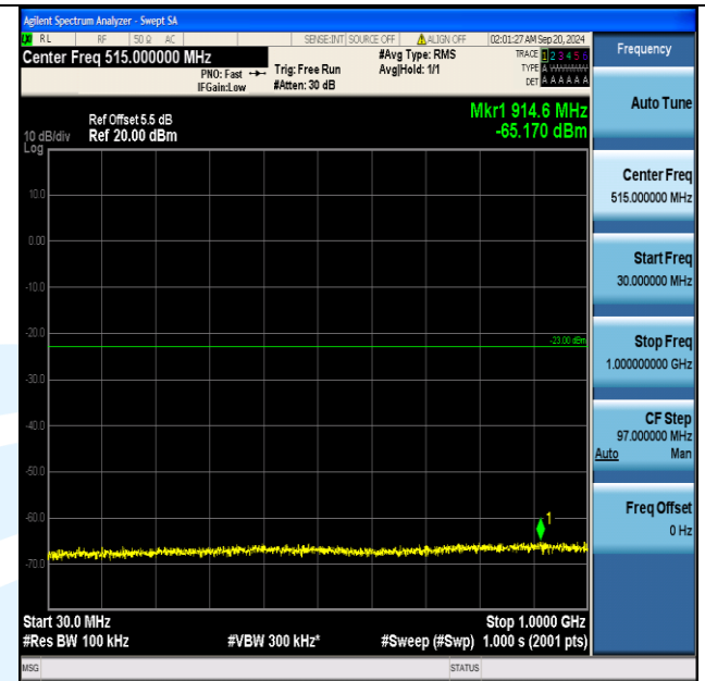
Band66_1.4MHz_16QAM_131979_1RB#0_30~1000_30~1000
