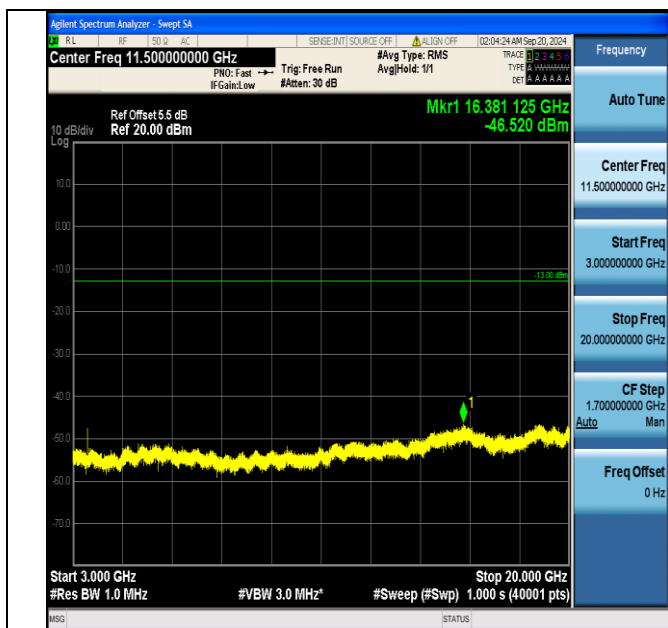
Band66_1.4MHz_16QAM_132322_1RB#0_3000~20000_3000~20000
