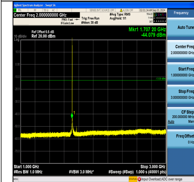
Band66_1.4MHz_16QAM_131979_1RB#0_1000~3000_1000~3000
