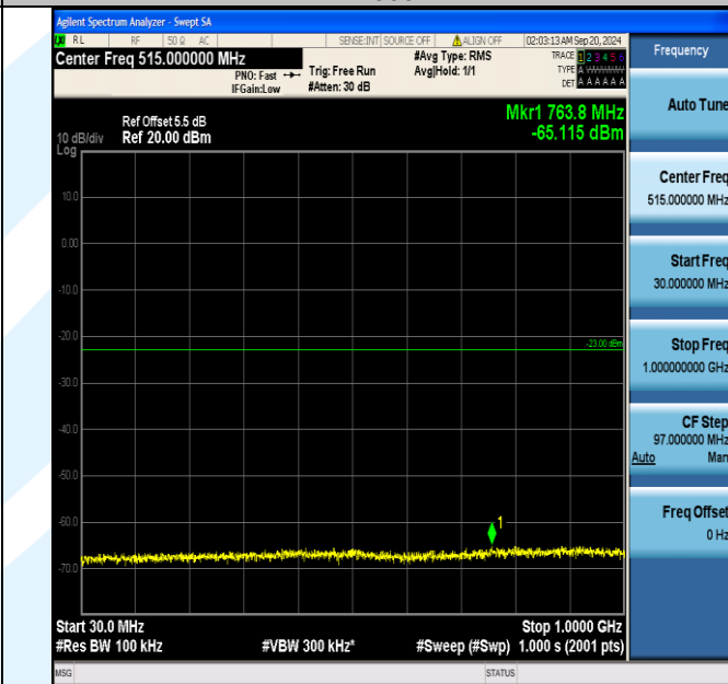
Band66_1.4MHz_16QAM_131979_6RB#0_30~1000_30~1000
