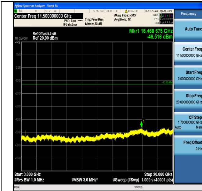
Band66_1.4MHz_QPSK_132322_1RB#5_3000~20000_3000~20000
