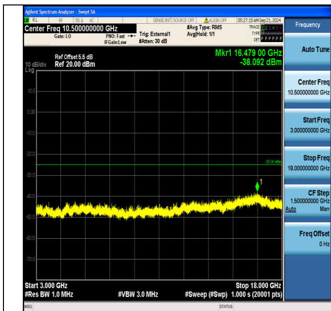
Band41_20MHz_16QAM_41140_100RB#0_3000~18000_3000~18000
