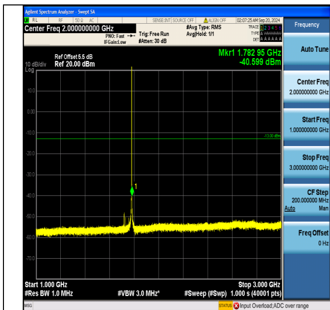
Band66_1.4MHz_QPSK_132665_1RB#5_1000~3000_1000~3000
