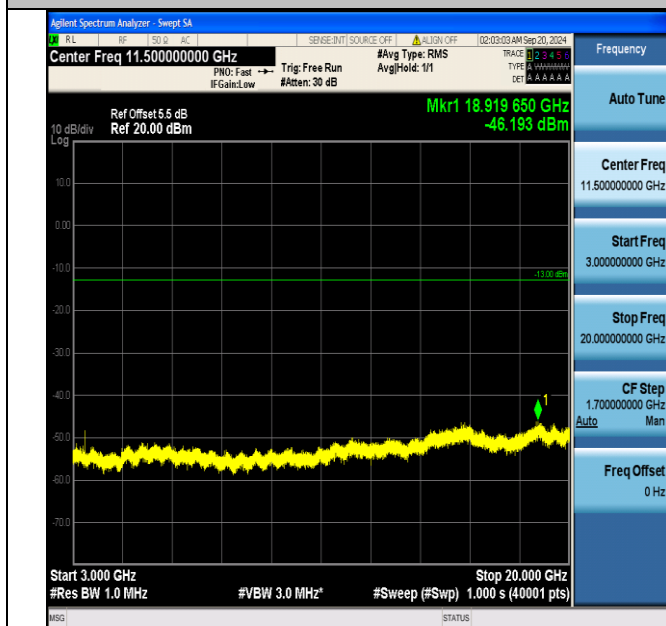
Band66_1.4MHz_QPSK_131979_6RB#0_3000~20000_3000~20000
