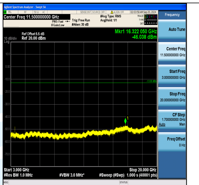
Band66_1.4MHz_QPSK_132322_1RB#0_3000~20000_3000~20000
