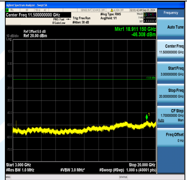
Band66_1.4MHz_16QAM_131979_1RB#0_3000~20000_3000~20000
