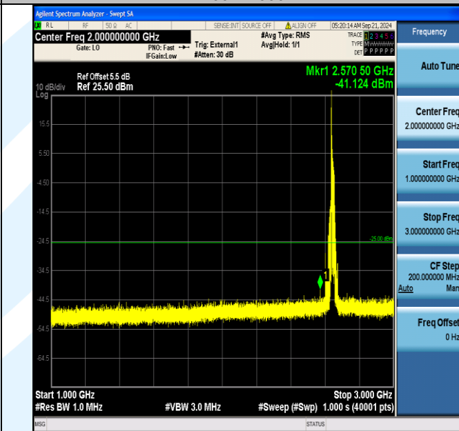
Band41_20MHz_16QAM_41140_1RB#0_1000~3000_1000~3000
