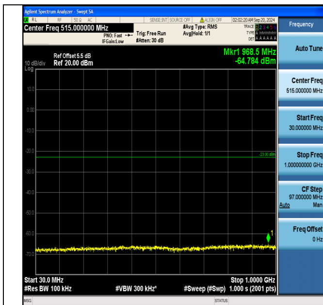
Band66_1.4MHz_16QAM_131979_1RB#5_30~1000_30~1000
