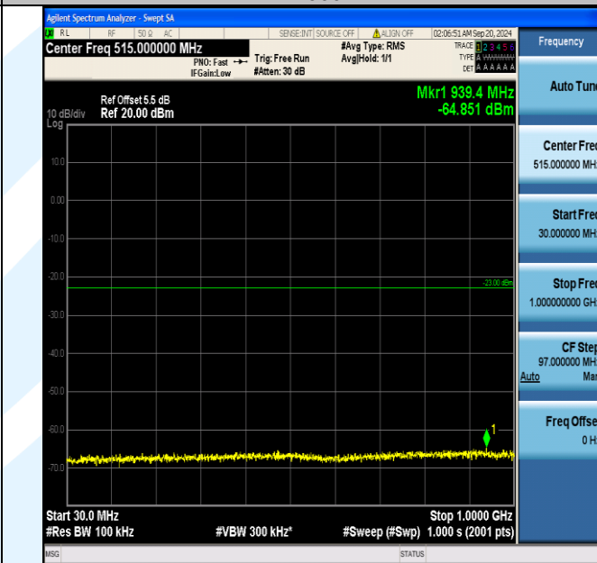
Band66_1.4MHz_16QAM_132665_1RB#0_30~1000_30~1000
