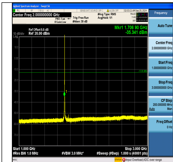
Band66_1.4MHz_16QAM_131979_6RB#0_1000~3000_1000~3000
