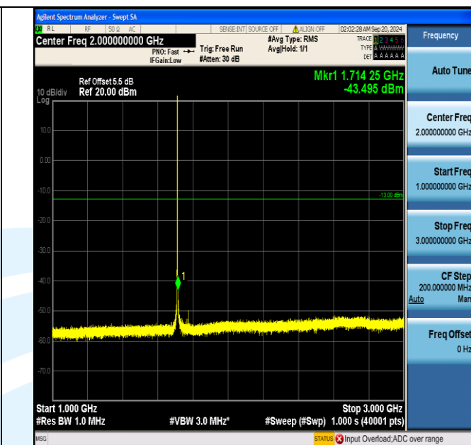
Band66_1.4MHz_16QAM_131979_1RB#5_1000~3000_1000~3000
