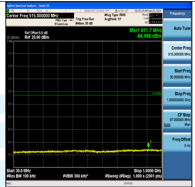
Band66_1.4MHz_QPSK_132322_6RB#0_30~1000_30~1000
