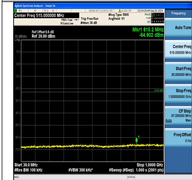
Band66_1.4MHz_16QAM_132322_1RB#0_30~1000_30~1000
