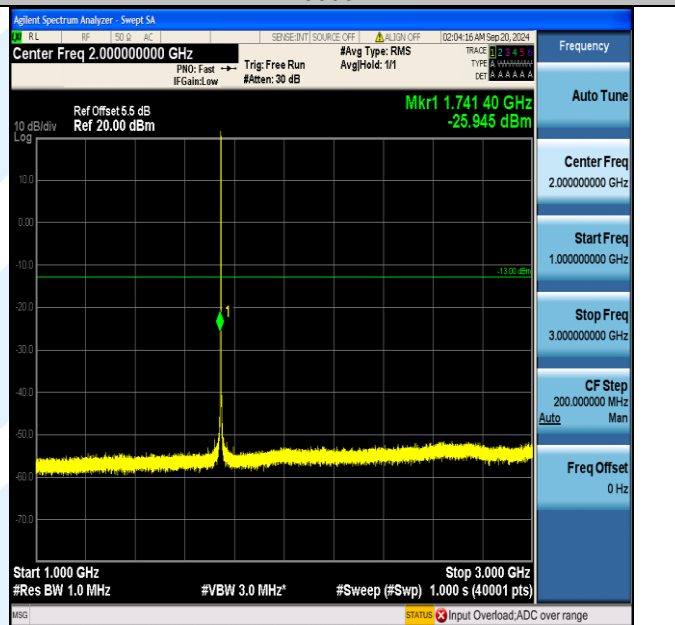
Band66_1.4MHz_16QAM_132322_1RB#0_1000~3000_1000~3000
