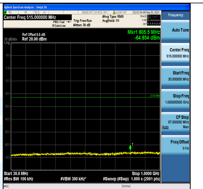
Band66_1.4MHz_QPSK_131979_1RB#5_30~1000_30~1000
