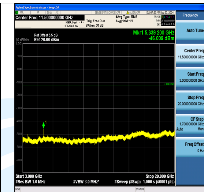
Band66_1.4MHz_QPSK_132665_1RB#5_3000~20000_3000~20000
