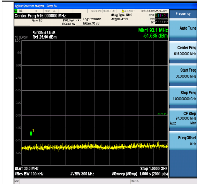
Band41_20MHz_16QAM_41140_1RB#99_30~1000_30~1000
