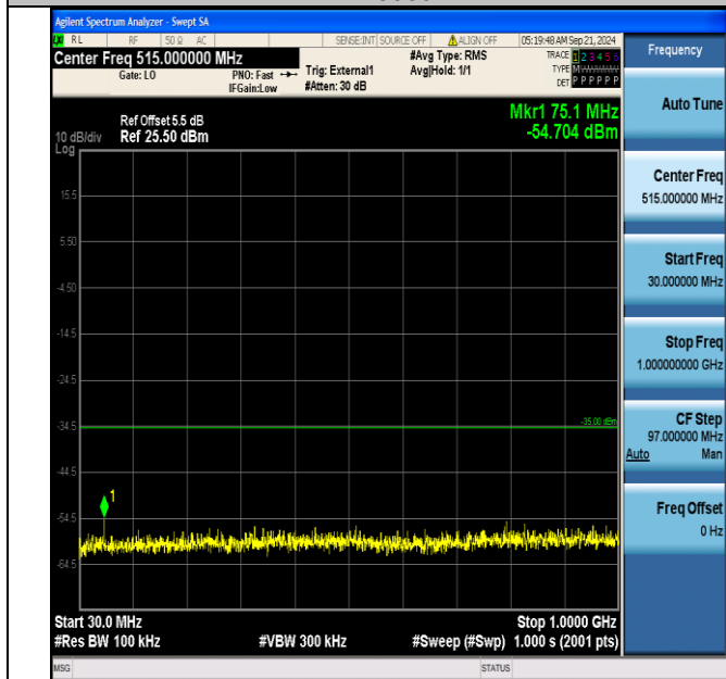
Band41_20MHz_16QAM_41140_1RB#0_30~1000_30~1000
