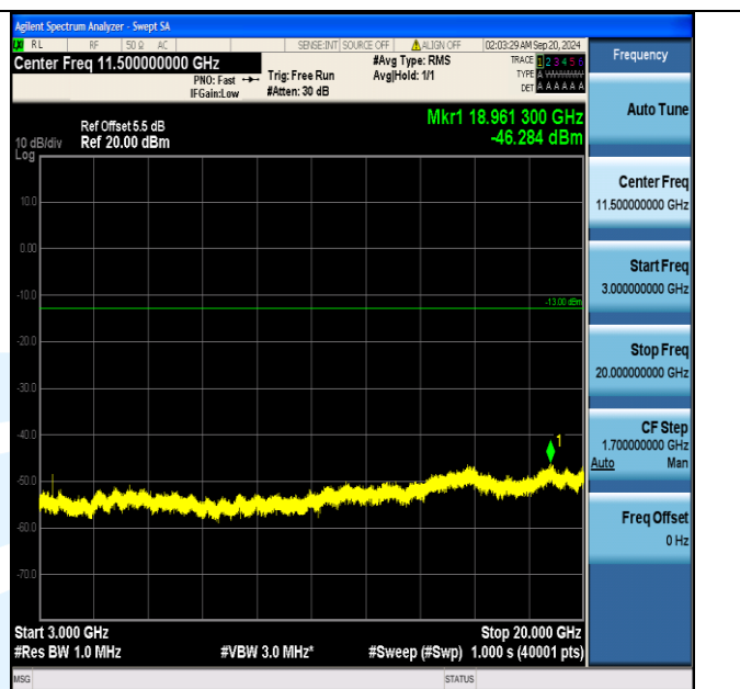
Band66_1.4MHz_16QAM_131979_6RB#0_3000~20000_3000~20000
