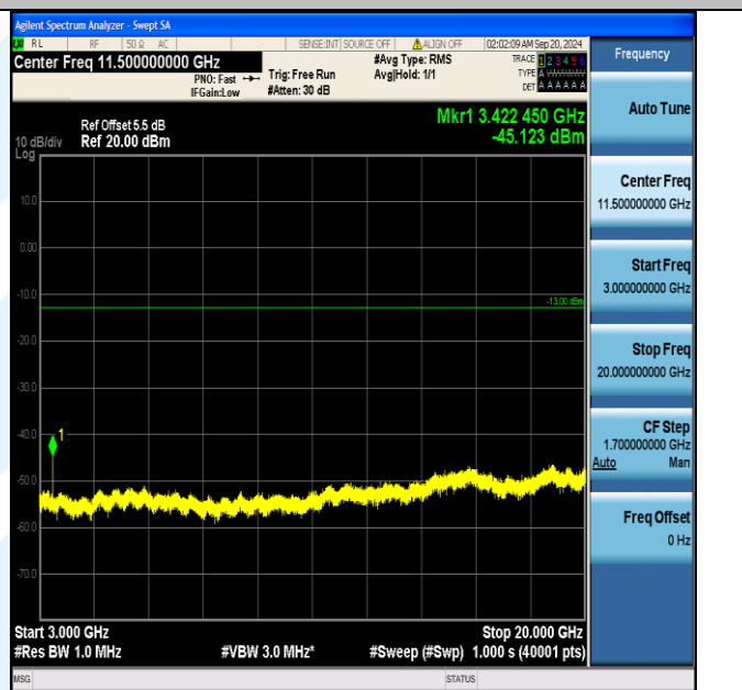
Band66_1.4MHz_QPSK_131979_1RB#5_3000~20000_3000~20000
