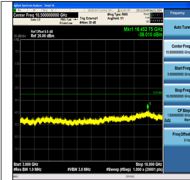
Band41_20MHz_QPSK_40690_1RB#99_3000~18000_3000~18000
