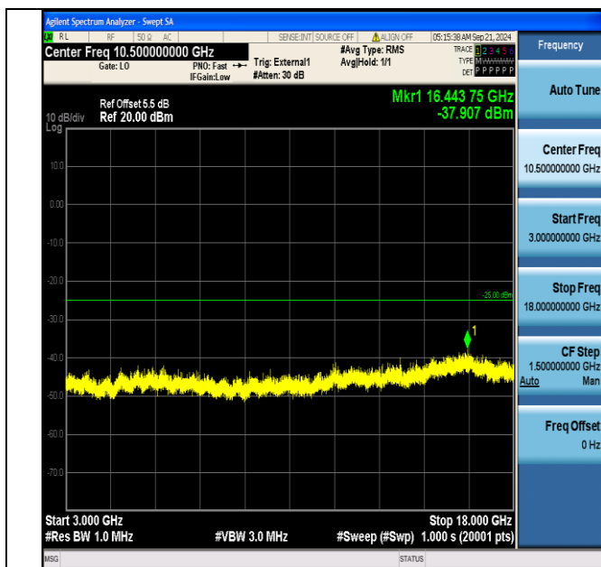
Band41_20MHz_QPSK_40690_100RB#0_3000~18000_3000~18000
