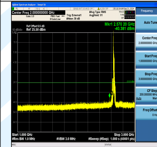
Band41_20MHz_QPSK_41140_1RB#0_1000~3000_1000~3000
