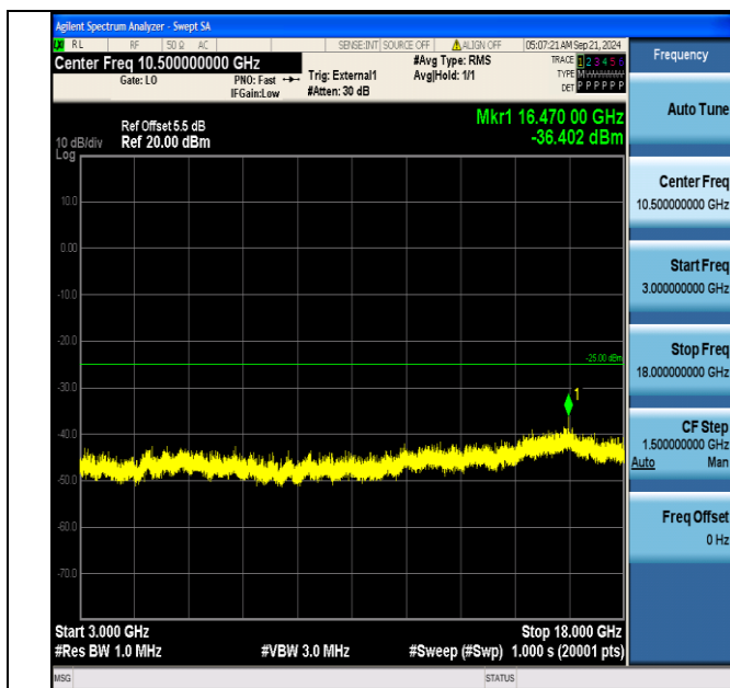
Band41_20MHz_16QAM_40340_100RB#0_3000~18000_3000~18000
