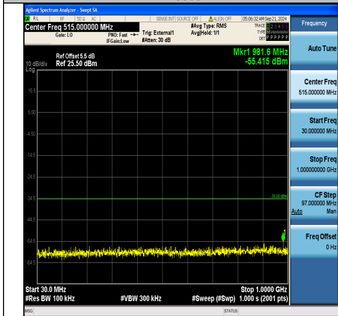
Band41_20MHz_16QAM_40340_100RB#0_30~1000_30~1000
