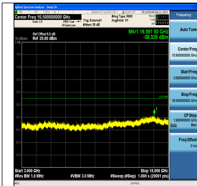
Band41_20MHz_QPSK_41140_1RB#0_3000~18000_3000~18000
