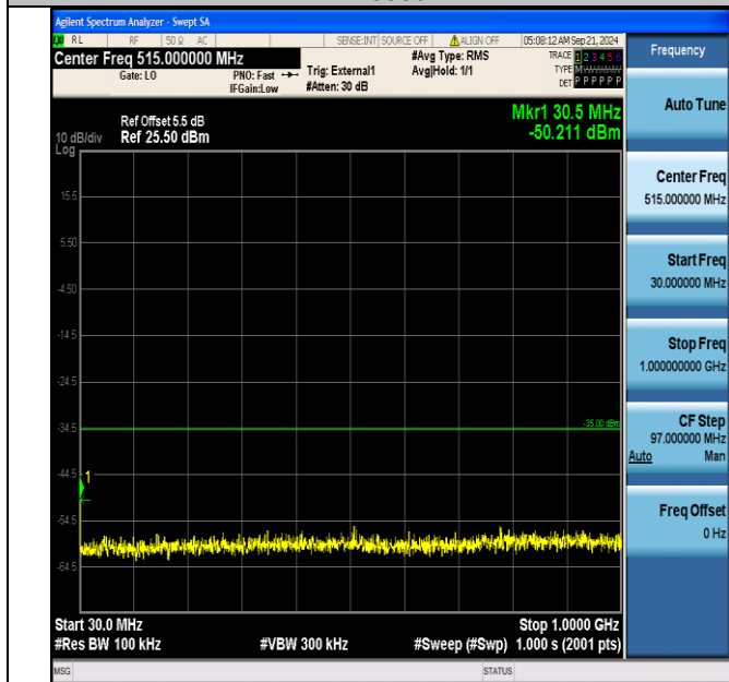
Band41_20MHz_QPSK_40690_1RB#0_30~1000_30~1000
