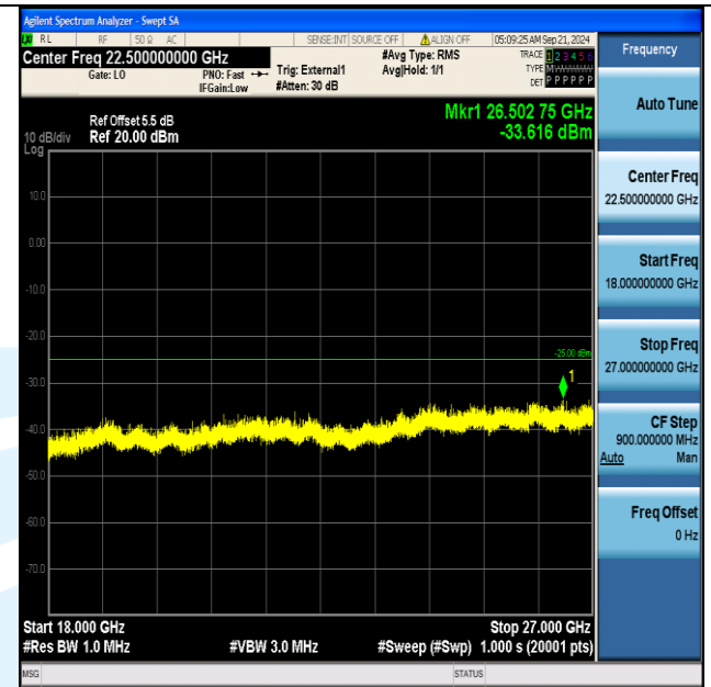
Band41_20MHz_QPSK_40690_1RB#0_18000~27000_18000~27000
