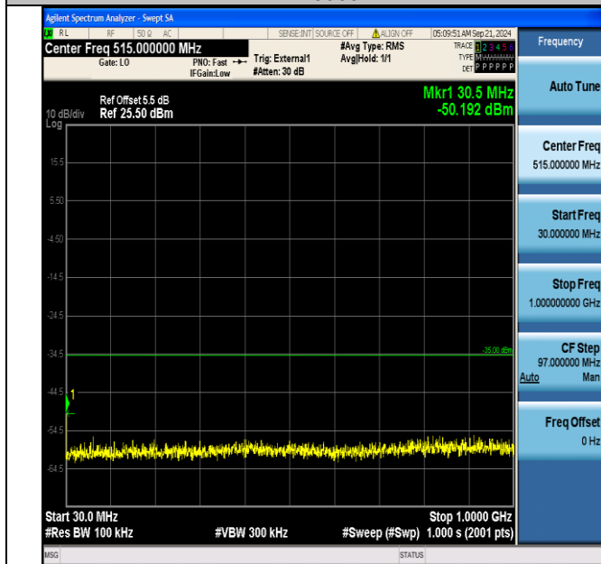
Band41_20MHz_16QAM_40690_1RB#0_30~1000_30~1000
