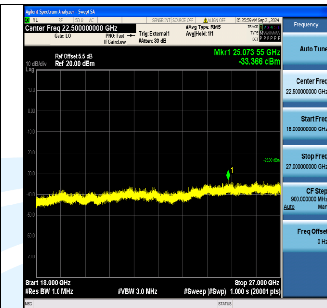
Band41_20MHz_QPSK_41140_100RB#0_18000~27000_18000~27000
