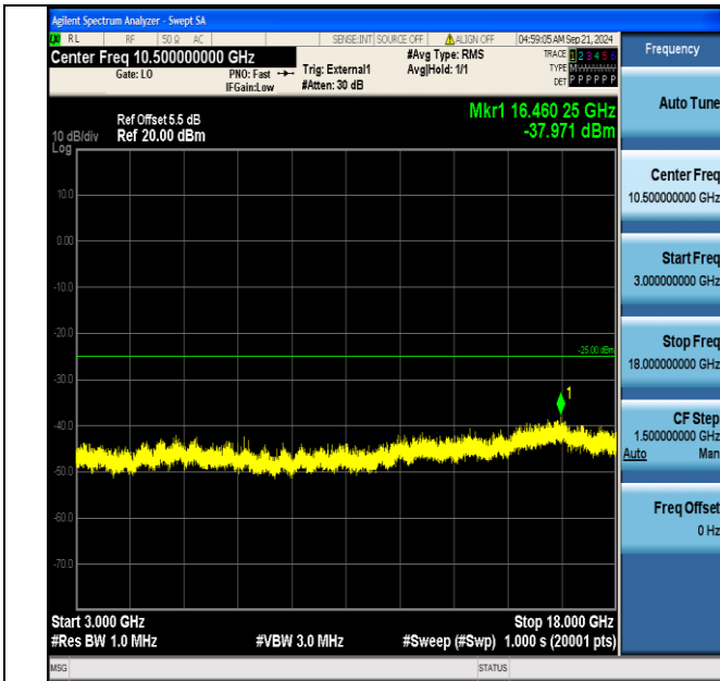
Band41_20MHz_QPSK_40340_1RB#0_3000~18000_3000~18000
