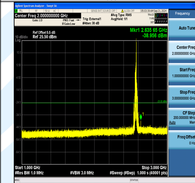
Band41_20MHz_16QAM_40340_1RB#99_1000~3000_1000~3000
