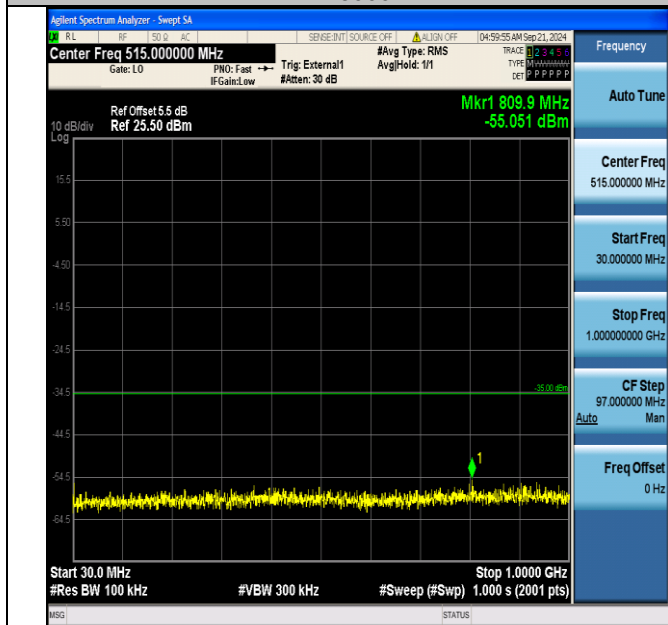
Band41_20MHz_16QAM_40340_1RB#0_30~1000_30~1000
