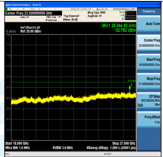
Band41_20MHz_QPSK_40340_1RB#0_18000~27000_18000~27000
