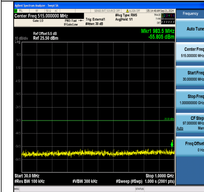
Band41_20MHz_QPSK_40690_100RB#0_30~1000_30~1000
