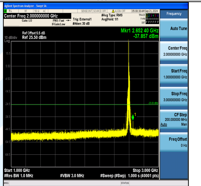
Band41_20MHz_QPSK_40690_1RB#0_1000~3000_1000~3000
