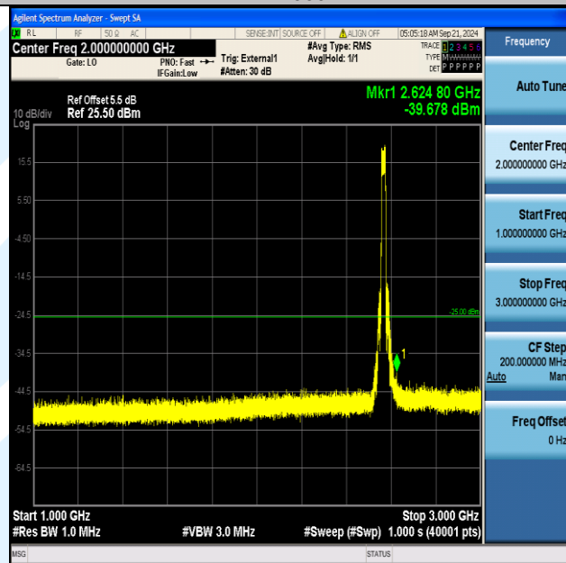
Band41_20MHz_QPSK_40340_100RB#0_1000~3000_1000~3000
