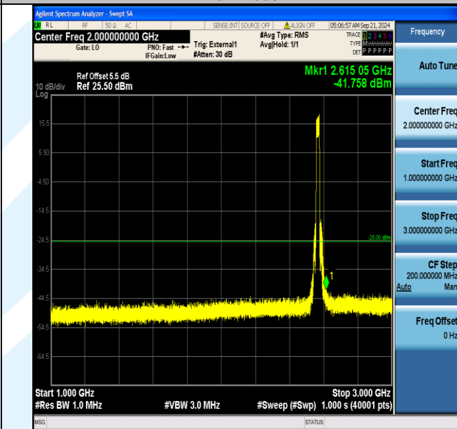
Band41_20MHz_16QAM_40340_100RB#0_1000~3000_1000~3000
