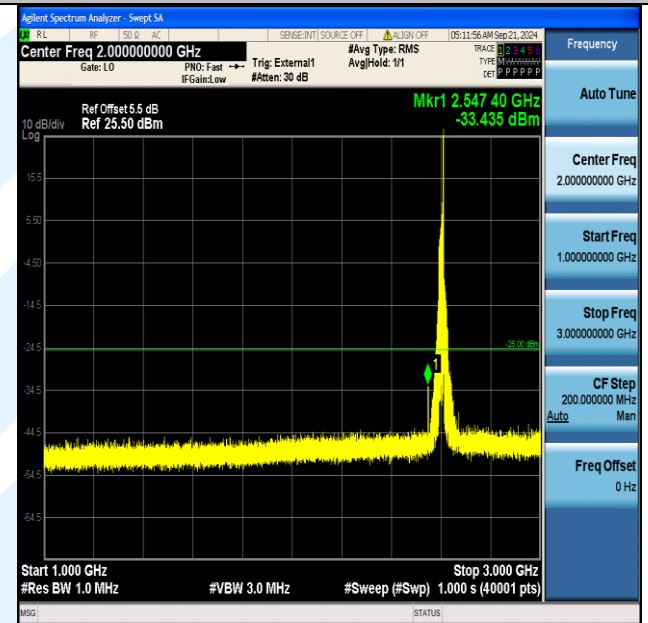
Band41_20MHz_QPSK_40690_1RB#99_1000~3000_1000~3000
