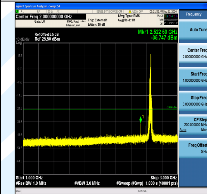
Band41_20MHz_QPSK_41140_1RB#99_1000~3000_1000~3000
