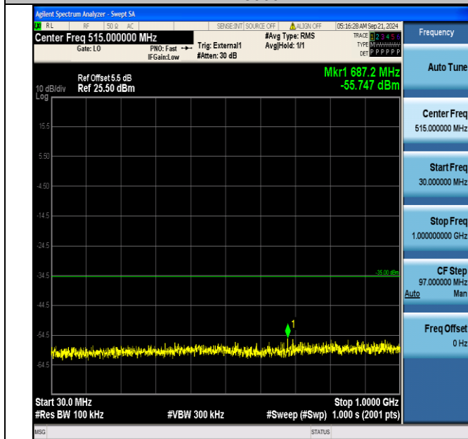
Band41_20MHz_16QAM_40690_100RB#0_30~1000_30~1000
