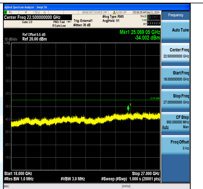
Band41_20MHz_QPSK_40340_100RB#0_18000~27000_18000~27000
