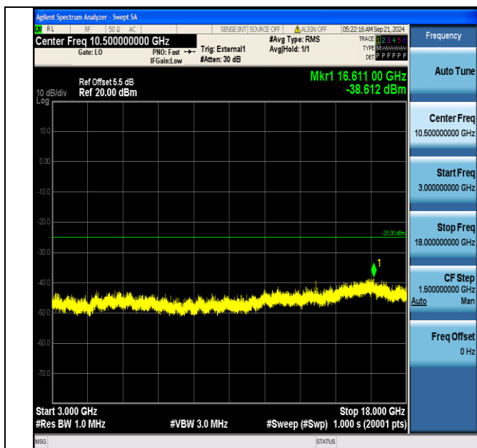
Band41_20MHz_QPSK_41140_1RB#99_3000~18000_3000~18000
