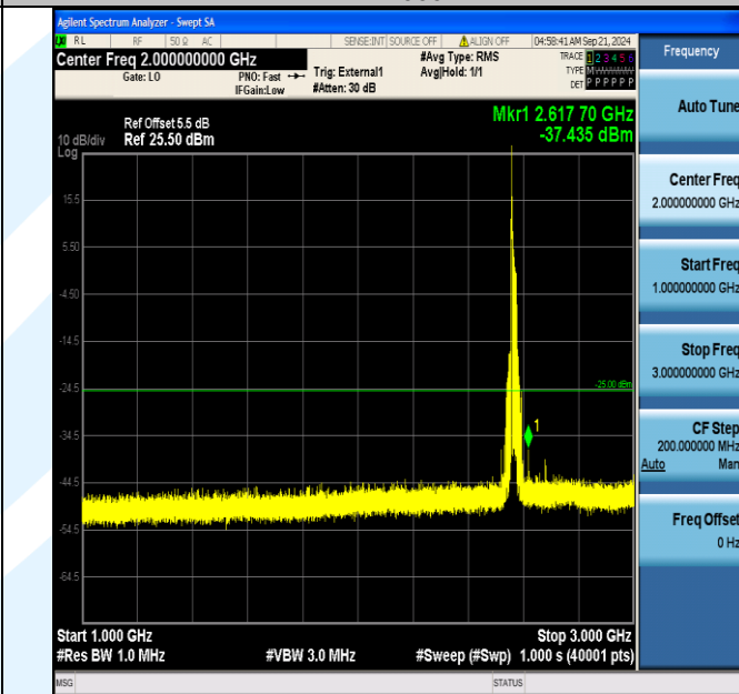
Band41_20MHz_QPSK_40340_1RB#0_1000~3000_1000~3000
