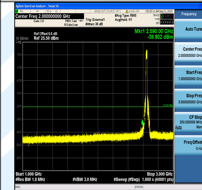
Band41_20MHz_QPSK_41140_100RB#0_1000~3000_1000~3000
