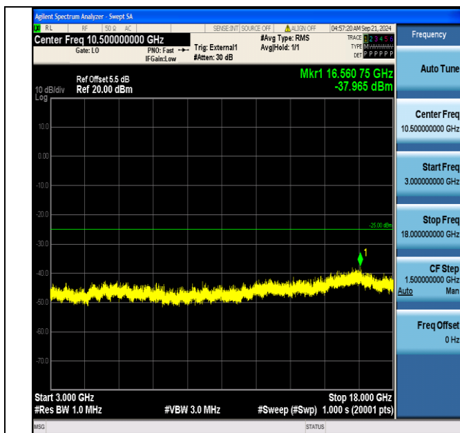
Band41_15MHz_16QAM_41165_75RB#0_3000~18000_3000~18000
