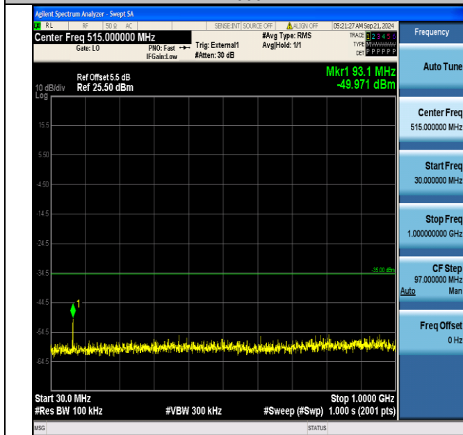
Band41_20MHz_QPSK_41140_1RB#99_30~1000_30~1000
