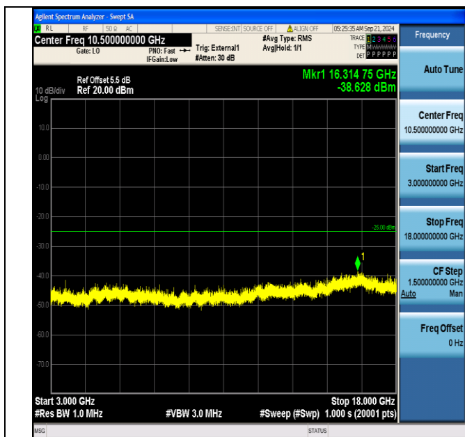
Band41_20MHz_QPSK_41140_100RB#0_3000~18000_3000~18000
