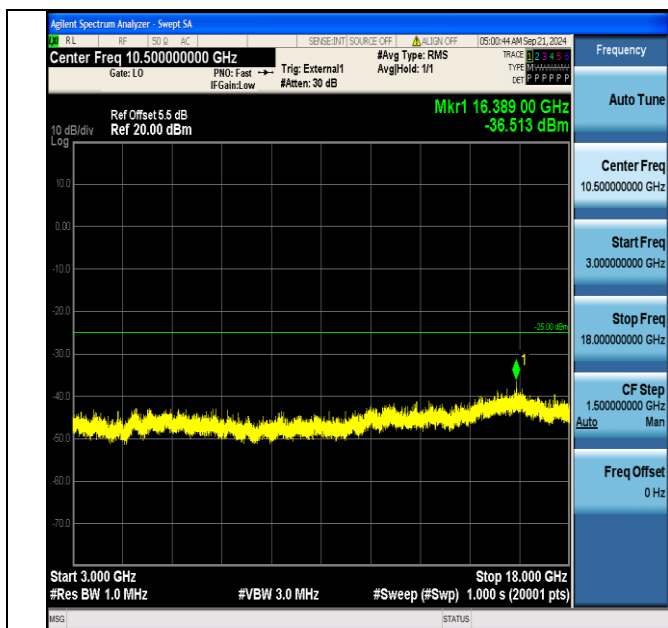
Band41_20MHz_16QAM_40340_1RB#0_3000~18000_3000~18000
