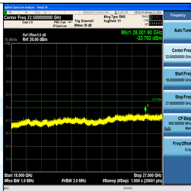
Band41_20MHz_QPSK_40340_1RB#99_18000~27000_18000~27000
