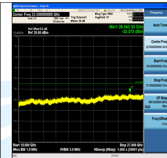
Band41_20MHz_QPSK_41140_1RB#99_18000~27000_18000~27000
