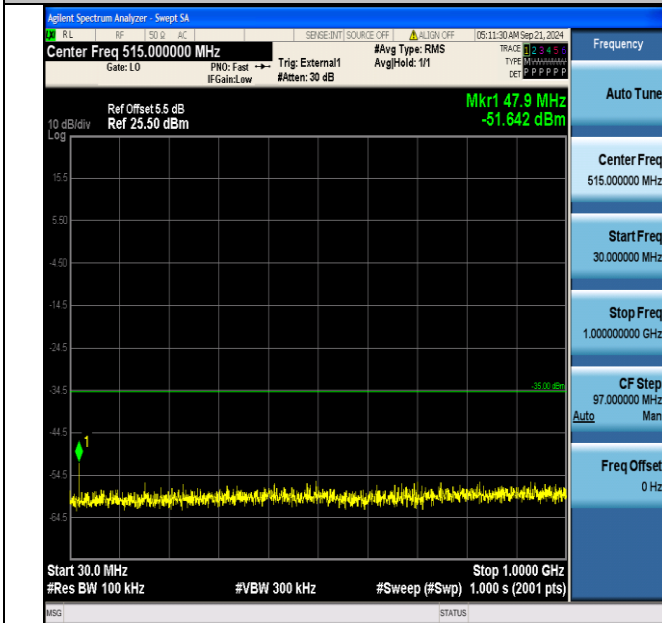
Band41_20MHz_QPSK_40690_1RB#99_30~1000_30~1000
