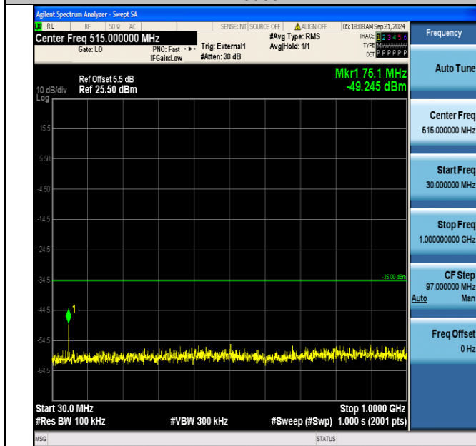
Band41_20MHz_QPSK_41140_1RB#0_30~1000_30~1000
