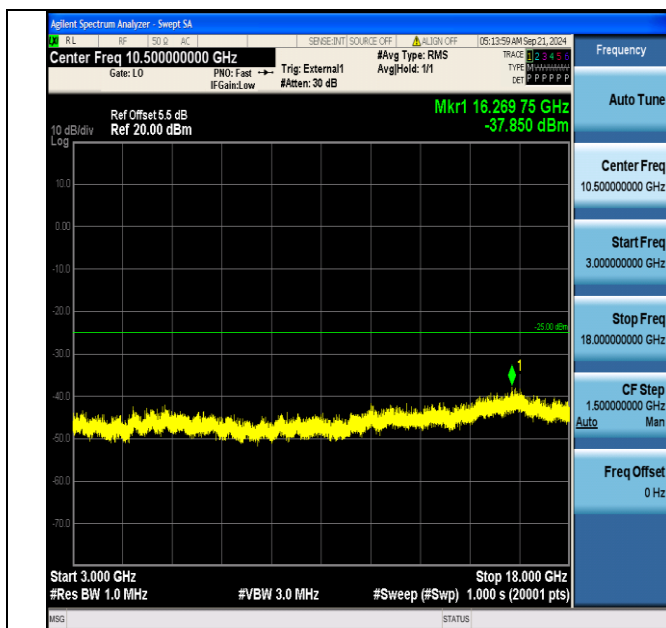
Band41_20MHz_16QAM_40690_1RB#99_3000~18000_3000~18000
