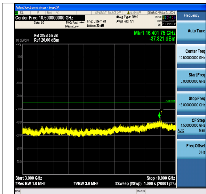
Band41_20MHz_QPSK_40340_100RB#0_3000~18000_3000~18000
