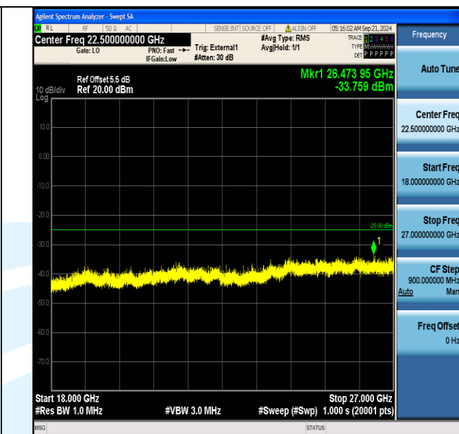
Band41_20MHz_QPSK_40690_100RB#0_18000~27000_18000~27000
