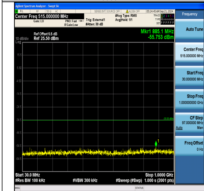
Band41_20MHz_QPSK_41140_100RB#0_30~1000_30~1000
