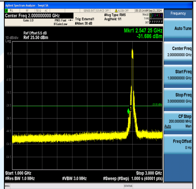
Band41_20MHz_QPSK_40690_100RB#0_1000~3000_1000~3000
