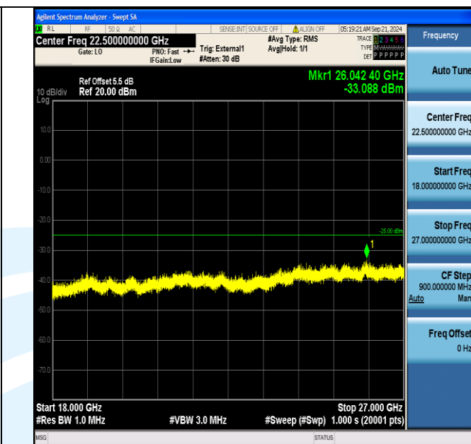
Band41_20MHz_QPSK_41140_1RB#0_18000~27000_18000~27000
