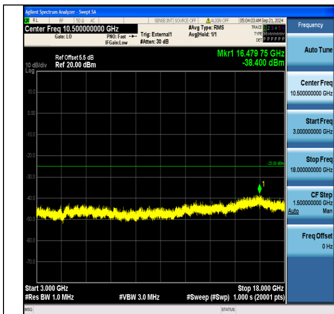
Band41_20MHz_16QAM_40340_1RB#99_3000~18000_3000~18000
