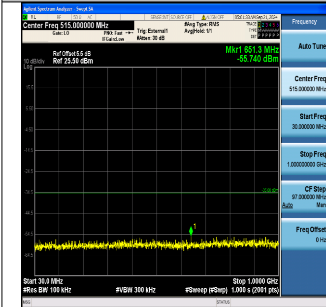
Band41_20MHz_QPSK_40340_1RB#99_30~1000_30~1000
