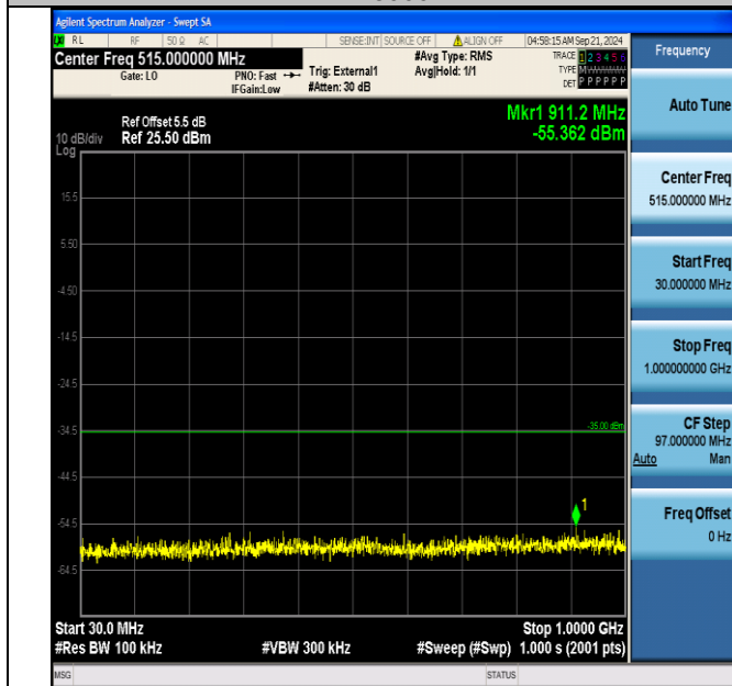
Band41_20MHz_QPSK_40340_1RB#0_30~1000_30~1000
