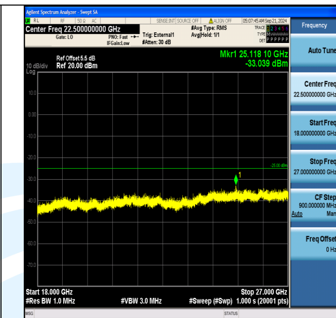
Band41_20MHz_16QAM_40340_100RB#0_18000~27000_18000~27000
