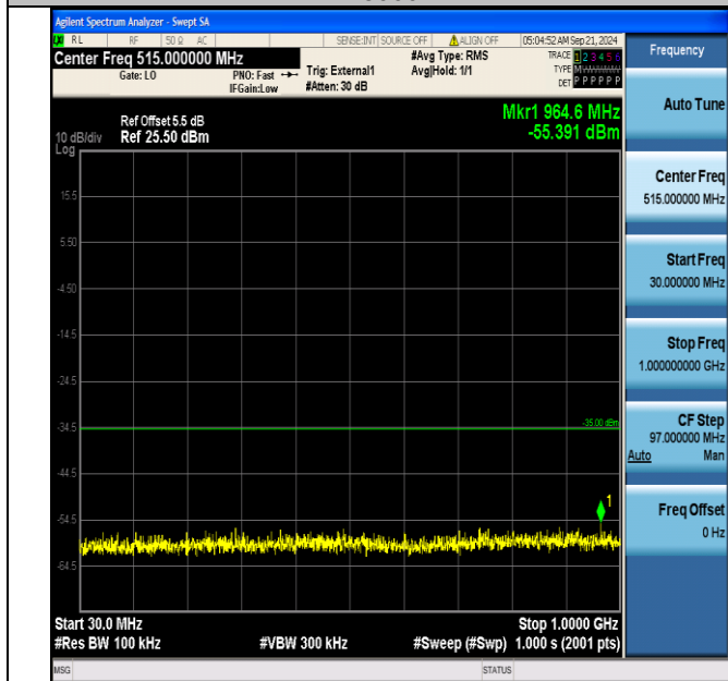
Band41_20MHz_QPSK_40340_100RB#0_30~1000_30~1000
