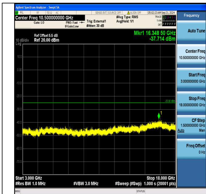
Band41_20MHz_QPSK_40340_1RB#99_3000~18000_3000~18000
