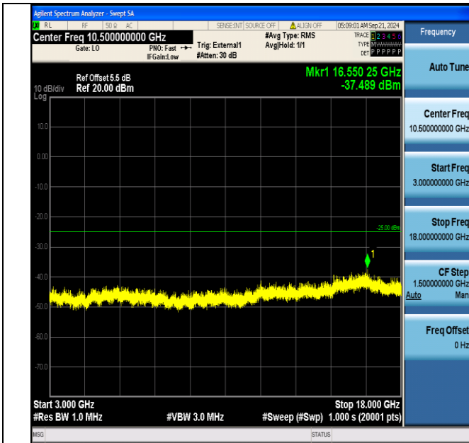
Band41_20MHz_QPSK_40690_1RB#0_3000~18000_3000~18000
