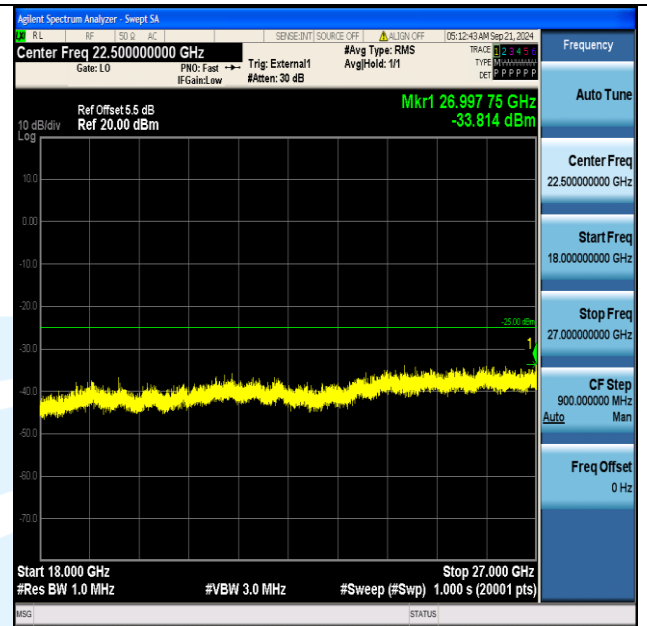
Band41_20MHz_QPSK_40690_1RB#99_18000~27000_18000~27000
