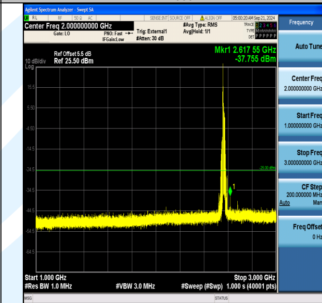
Band41_20MHz_16QAM_40340_1RB#0_1000~3000_1000~3000
