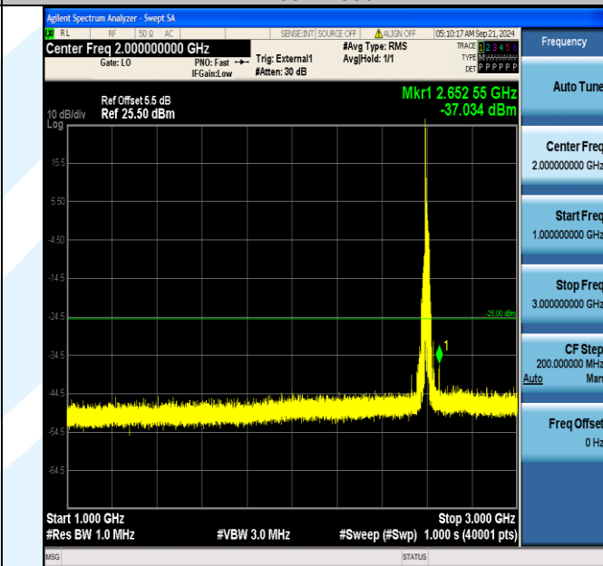
Band41_20MHz_16QAM_40690_1RB#0_1000~3000_1000~3000
