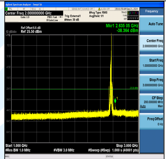
Band41_20MHz_QPSK_40340_1RB#99_1000~3000_1000~3000
