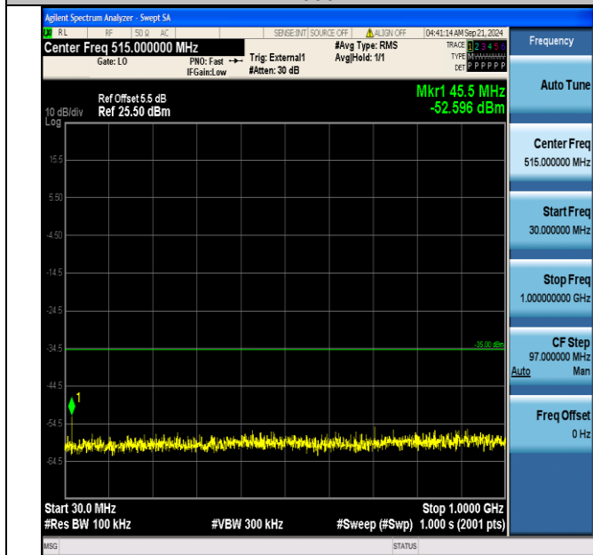
Band41_15MHz_QPSK_40690_1RB#74_30~1000_30~1000
