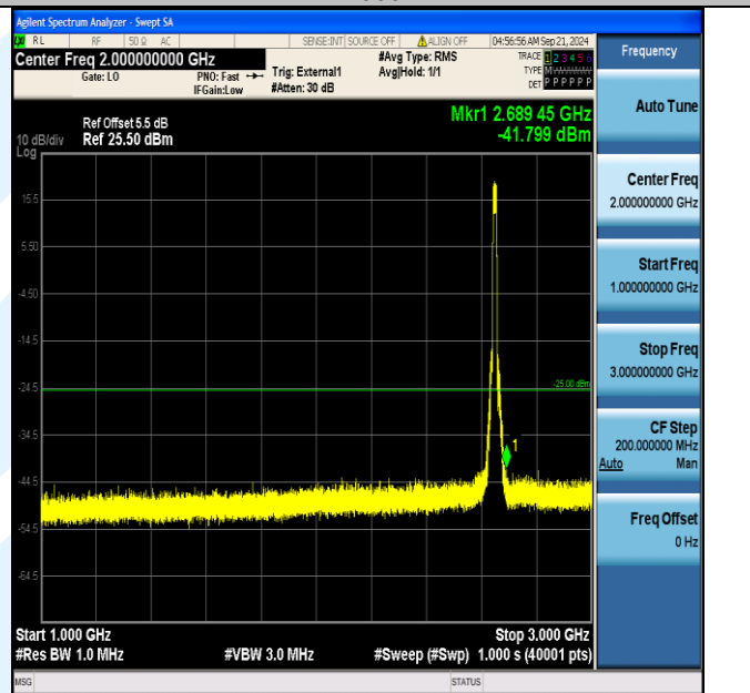
Band41_15MHz_16QAM_41165_75RB#0_1000~3000_1000~3000
