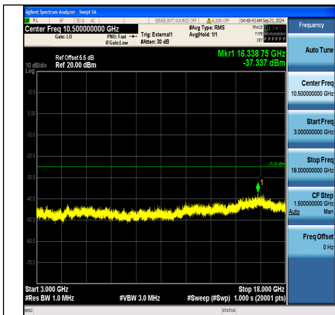
Band41_15MHz_QPSK_41165_1RB#0_3000~18000_3000~18000
