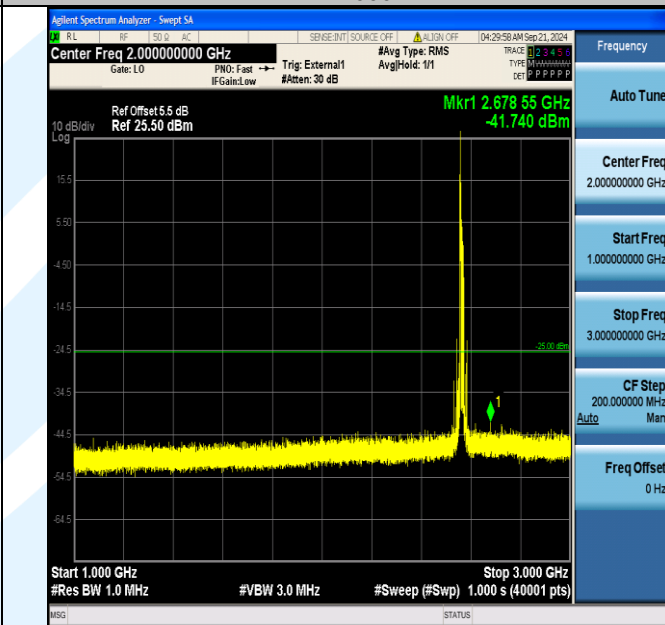
Band41_15MHz_16QAM_40315_1RB#0_1000~3000_1000~3000
