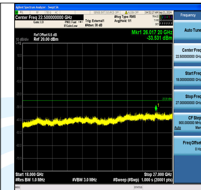
Band41_15MHz_QPSK_41165_1RB#74_18000~27000_18000~27000
