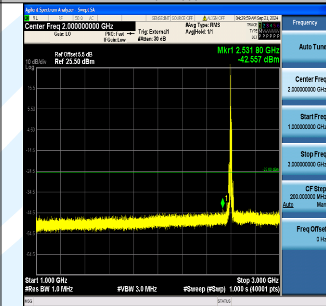
Band41_15MHz_16QAM_40690_1RB#0_1000~3000_1000~3000
