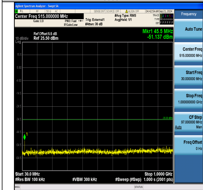
Band41_15MHz_16QAM_40690_1RB#74_30~1000_30~1000
