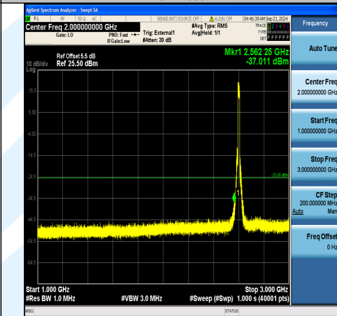
Band41_15MHz_16QAM_40690_75RB#0_1000~3000_1000~3000
