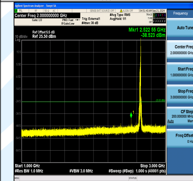
Band41_15MHz_QPSK_41165_1RB#74_1000~3000_1000~3000
