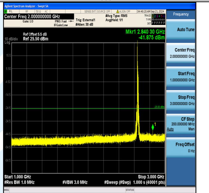
Band41_15MHz_QPSK_41165_1RB#0_1000~3000_1000~3000
