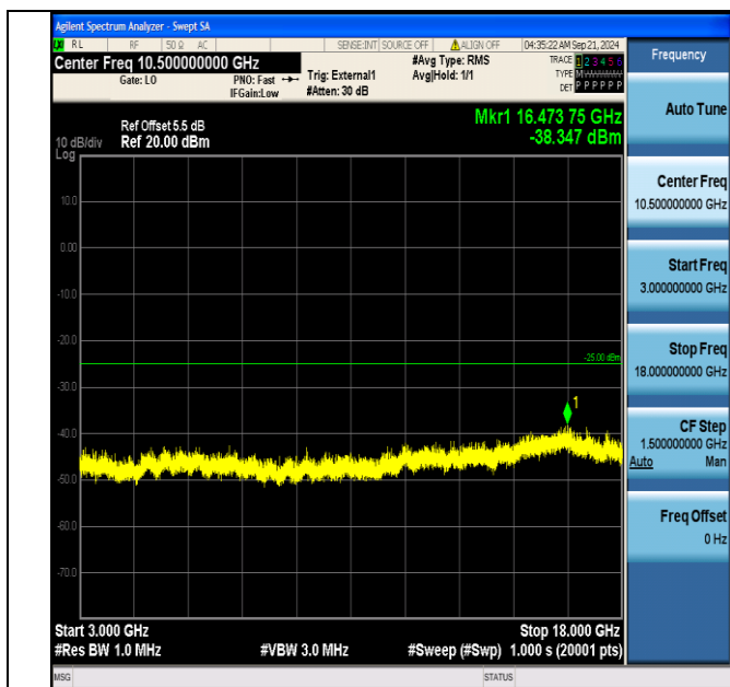
Band41_15MHz_QPSK_40315_75RB#0_3000~18000_3000~18000
