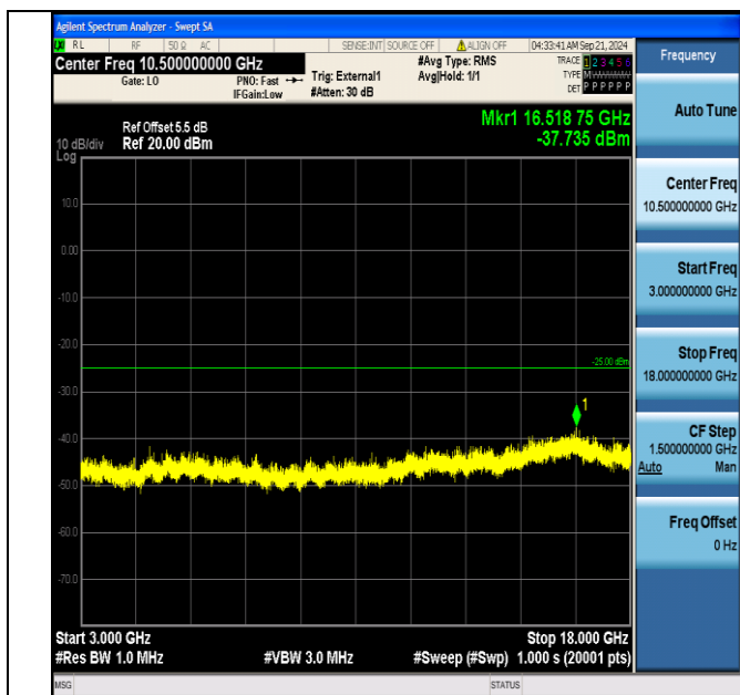
Band41_15MHz_16QAM_40315_1RB#74_3000~18000_3000~18000
