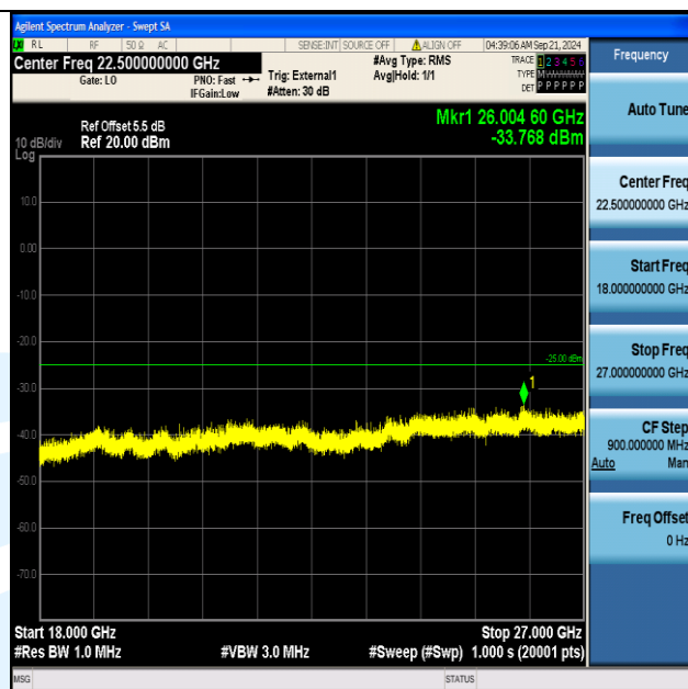
Band41_15MHz_QPSK_40690_1RB#0_18000~27000_18000~27000
