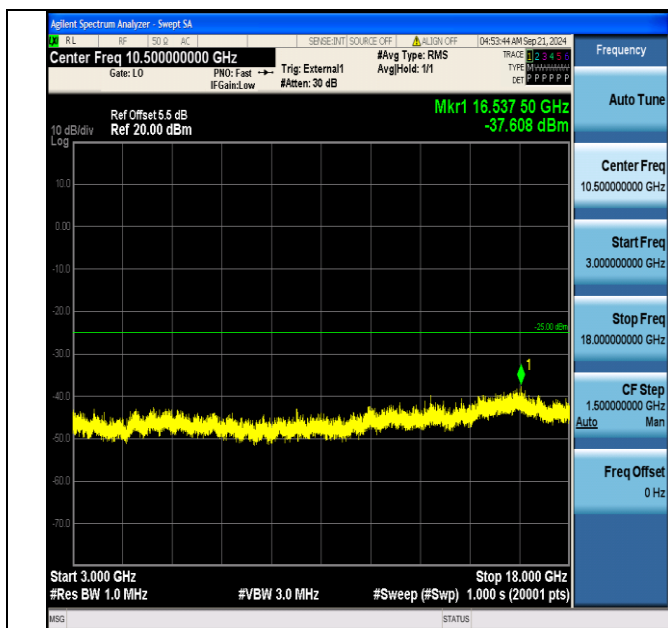
Band41_15MHz_16QAM_41165_1RB#74_3000~18000_3000~18000
