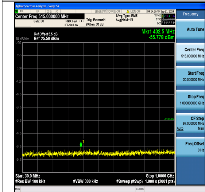
Band41_15MHz_QPSK_41165_75RB#0_30~1000_30~1000
