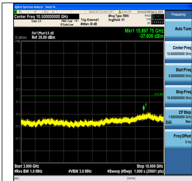
Band41_15MHz_QPSK_40690_1RB#74_3000~18000_3000~18000
