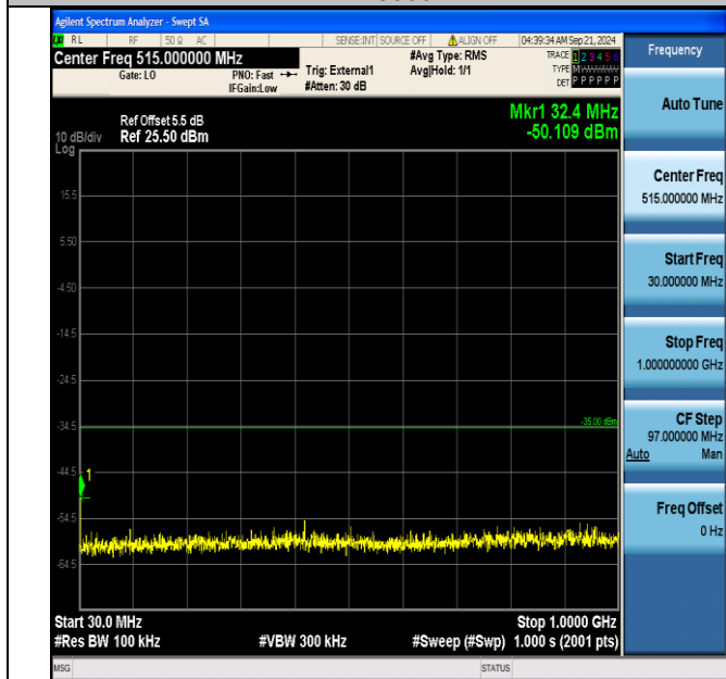
Band41_15MHz_16QAM_40690_1RB#0_30~1000_30~1000
