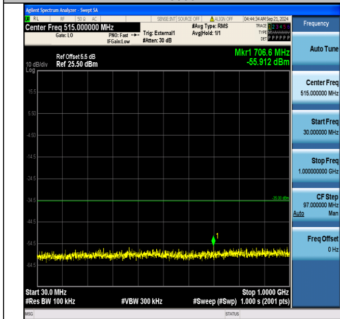
Band41_15MHz_QPSK_40690_75RB#0_30~1000_30~1000
