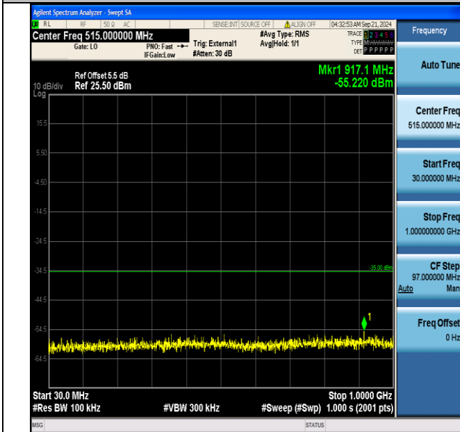
Band41_15MHz_16QAM_40315_1RB#74_30~1000_30~1000
