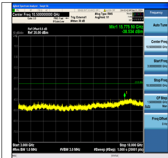
Band41_15MHz_16QAM_40690_1RB#74_3000~18000_3000~18000
