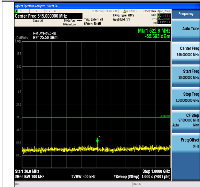
Band41_15MHz_16QAM_40315_1RB#0_30~1000_30~1000
