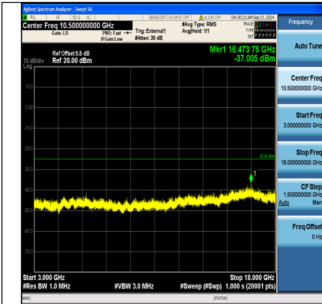
Band41_15MHz_16QAM_40315_1RB#0_3000~18000_3000~18000
