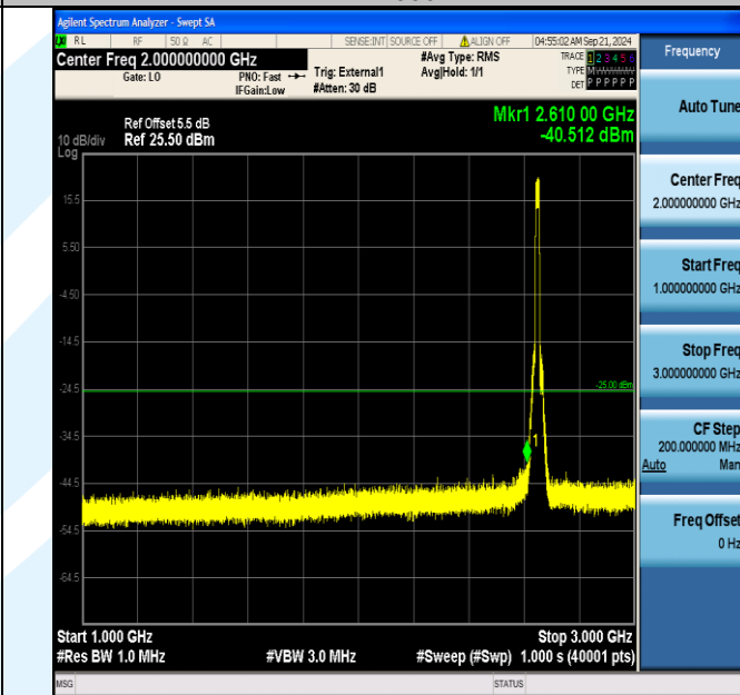
Band41_15MHz_QPSK_41165_75RB#0_1000~3000_1000~3000
