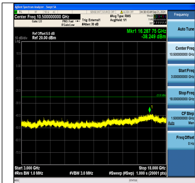
Band41_15MHz_QPSK_40690_1RB#0_3000~18000_3000~18000
