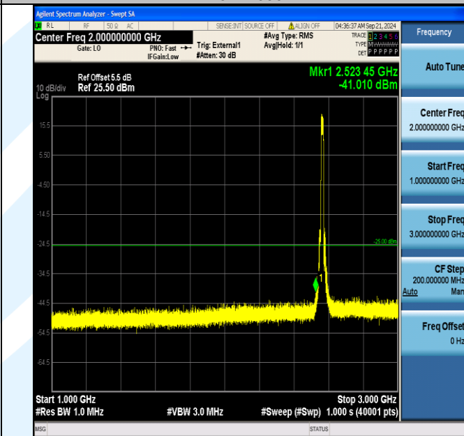
Band41_15MHz_16QAM_40315_75RB#0_1000~3000_1000~3000
