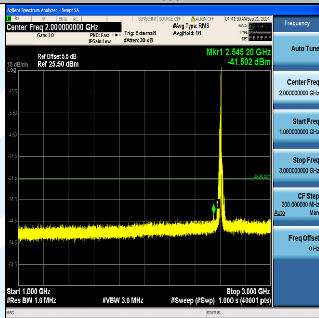
Band41_15MHz_QPSK_40690_1RB#74_1000~3000_1000~3000
