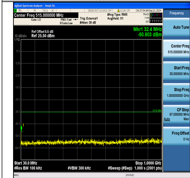
Band41_15MHz_QPSK_40690_1RB#0_30~1000_30~1000
