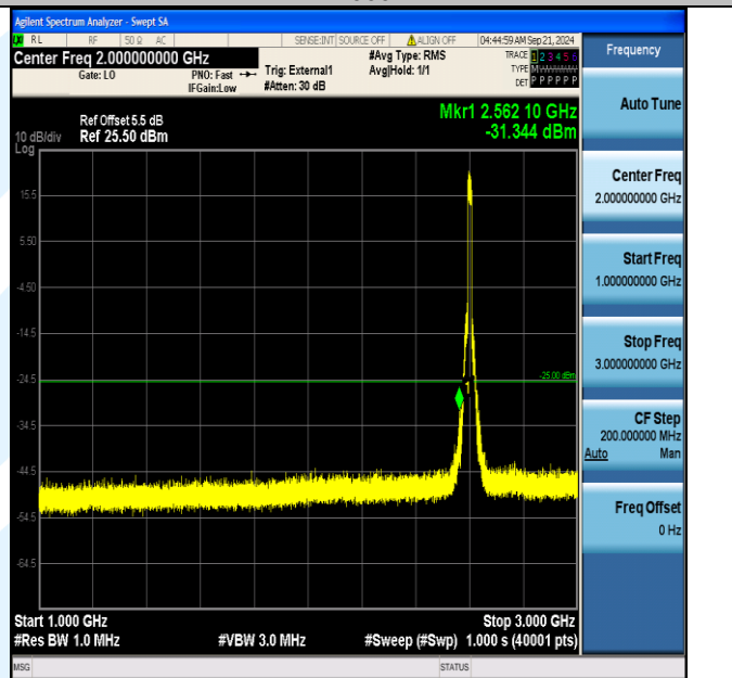
Band41_15MHz_QPSK_40690_75RB#0_1000~3000_1000~3000
