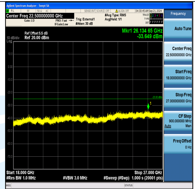
Band41_15MHz_16QAM_40315_1RB#0_18000~27000_18000~27000
