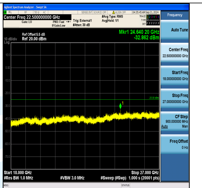
Band41_15MHz_QPSK_40315_75RB#0_18000~27000_18000~27000
