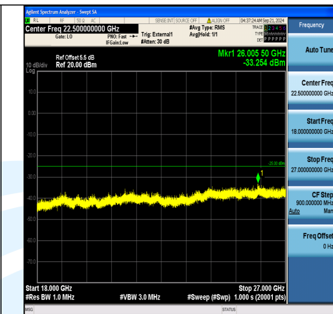
Band41_15MHz_16QAM_40315_75RB#0_18000~27000_18000~27000
