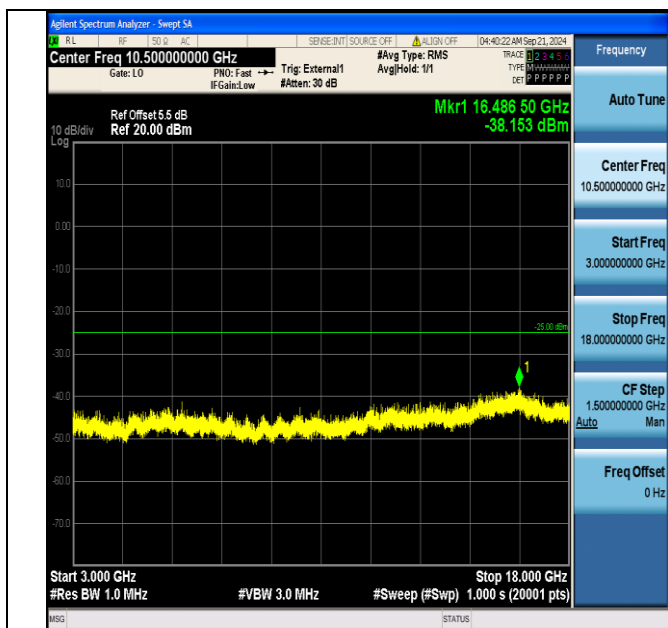
Band41_15MHz_16QAM_40690_1RB#0_3000~18000_3000~18000
