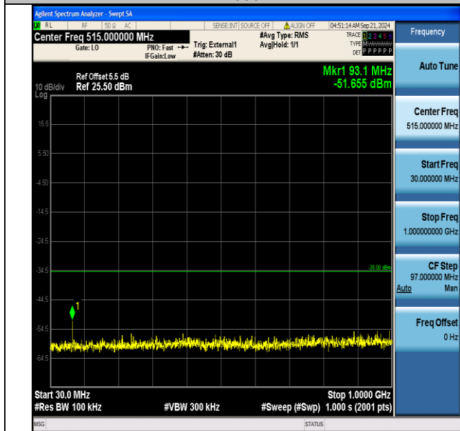
Band41_15MHz_QPSK_41165_1RB#74_30~1000_30~1000
