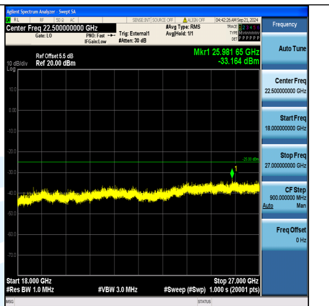
Band41_15MHz_QPSK_40690_1RB#74_18000~27000_18000~27000
