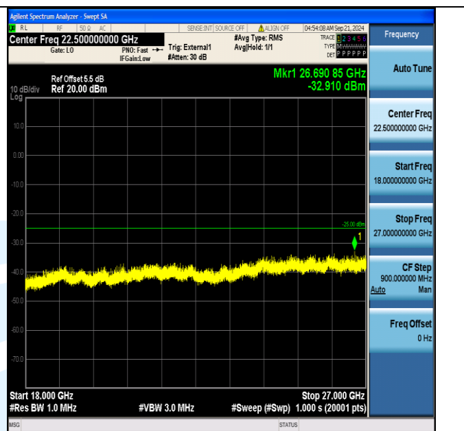
Band41_15MHz_16QAM_41165_1RB#74_18000~27000_18000~27000
