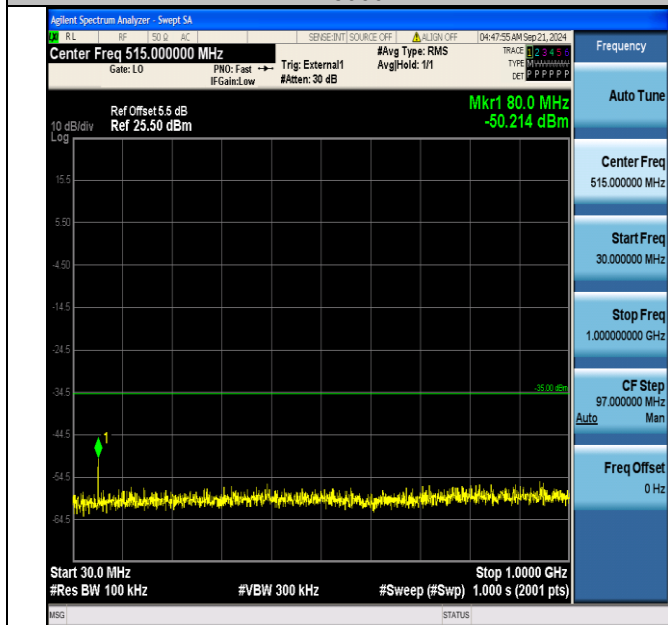
Band41_15MHz_QPSK_41165_1RB#0_30~1000_30~1000
