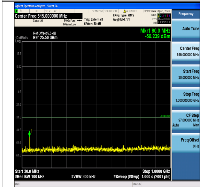
Band41_15MHz_16QAM_41165_1RB#0_30~1000_30~1000
