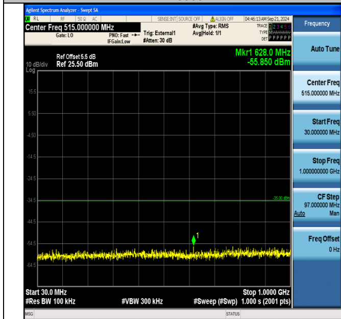
Band41_15MHz_16QAM_40690_75RB#0_30~1000_30~1000
