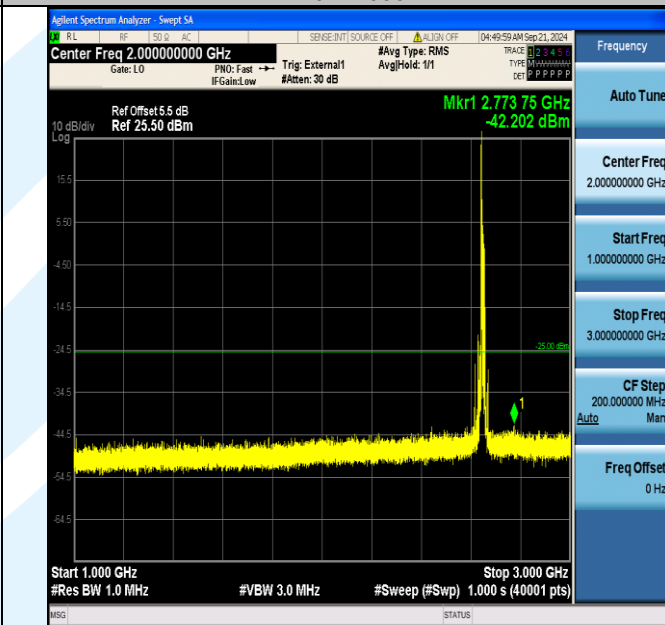
Band41_15MHz_16QAM_41165_1RB#0_1000~3000_1000~3000
