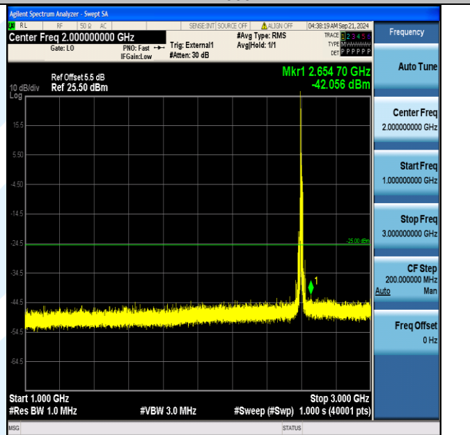
Band41_15MHz_QPSK_40690_1RB#0_1000~3000_1000~3000
