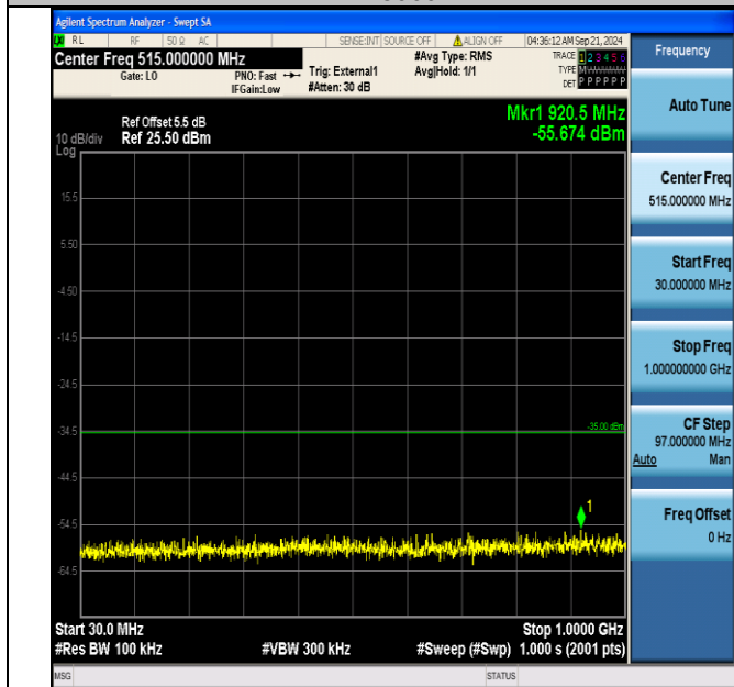
Band41_15MHz_16QAM_40315_75RB#0_30~1000_30~1000
