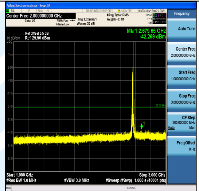
Band41_15MHz_16QAM_40315_1RB#74_1000~3000_1000~3000
