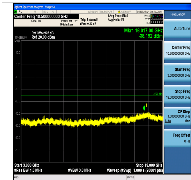
Band41_15MHz_QPSK_41165_75RB#0_3000~18000_3000~18000
