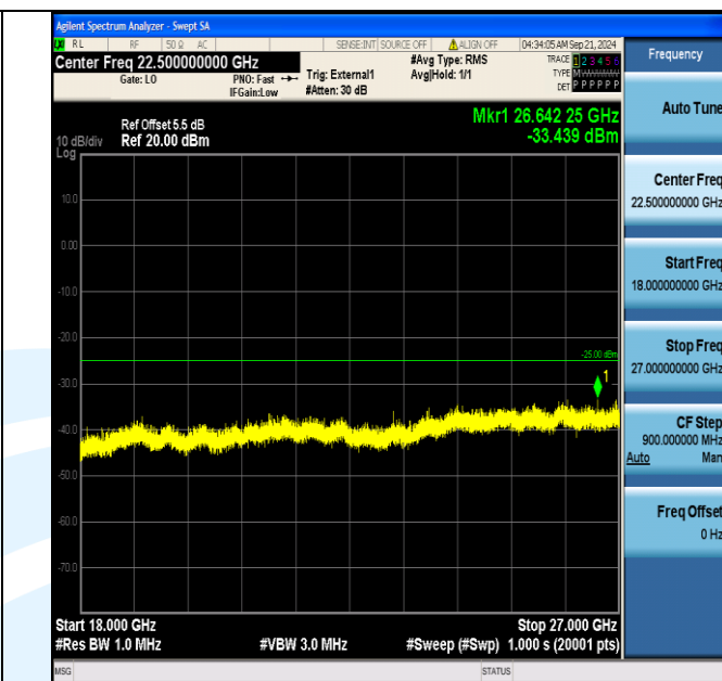
Band41_15MHz_16QAM_40315_1RB#74_18000~27000_18000~27000
