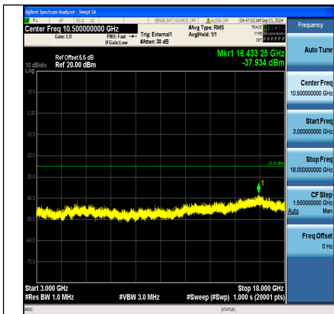
Band41_15MHz_16QAM_40690_75RB#0_3000~18000_3000~18000
