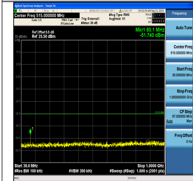
Band41_15MHz_16QAM_41165_1RB#74_30~1000_30~1000
