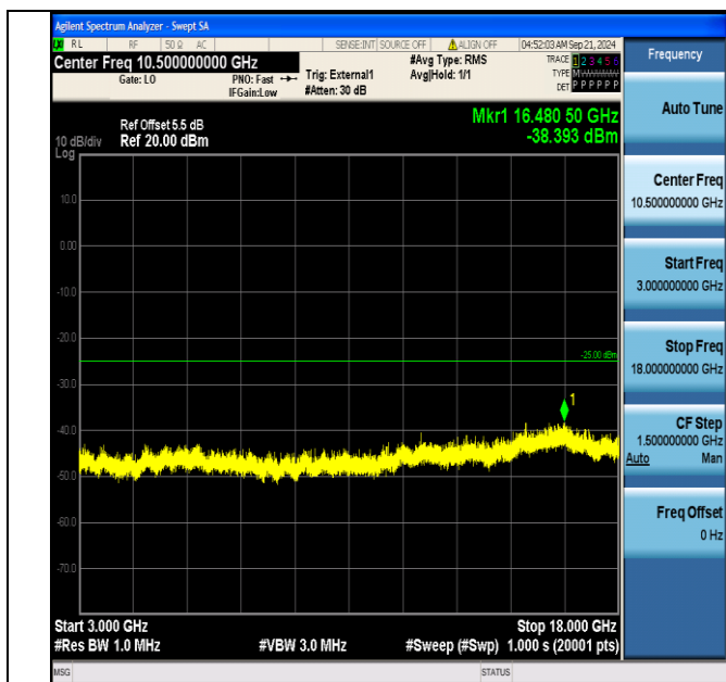
Band41_15MHz_QPSK_41165_1RB#74_3000~18000_3000~18000
