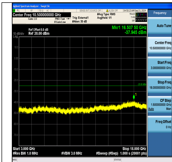
Band41_15MHz_16QAM_41165_1RB#0_3000~18000_3000~18000
