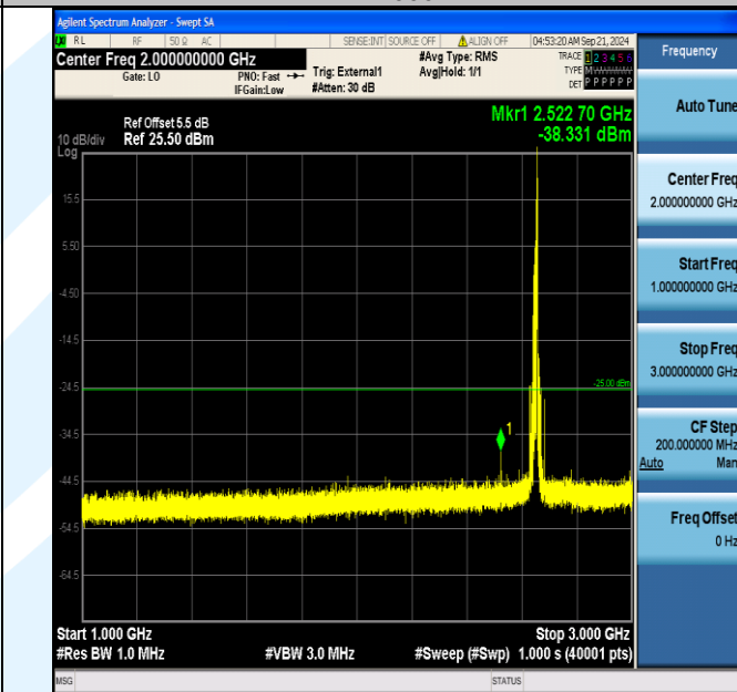
Band41_15MHz_16QAM_41165_1RB#74_1000~3000_1000~3000
