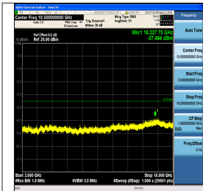
Band41_15MHz_16QAM_40315_75RB#0_3000~18000_3000~18000
