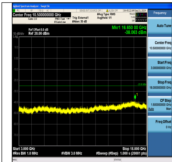
Band41_15MHz_QPSK_40690_75RB#0_3000~18000_3000~18000
