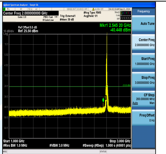
Band41_15MHz_16QAM_40690_1RB#74_1000~3000_1000~3000
