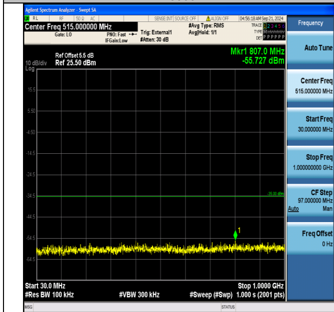
Band41_15MHz_16QAM_41165_75RB#0_30~1000_30~1000
