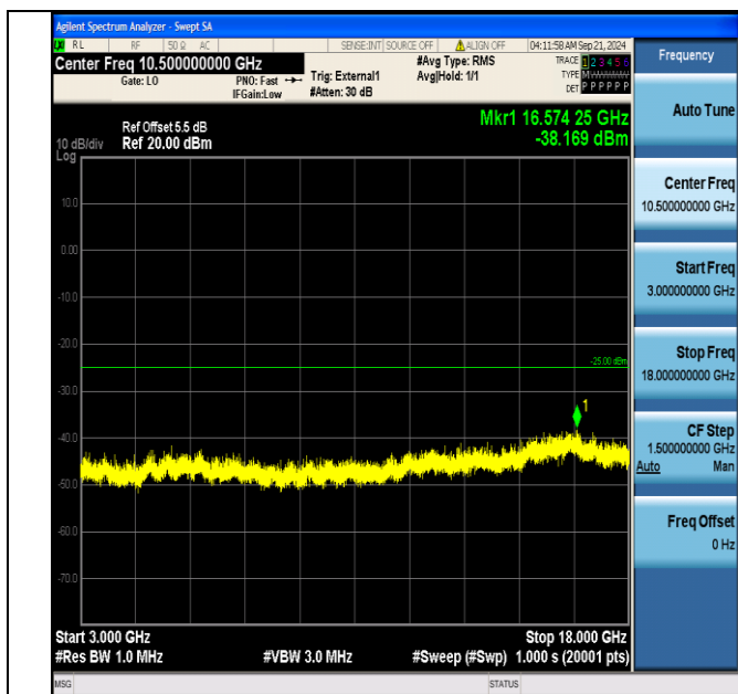
Band41_10MHz_QPSK_40690_1RB#49_3000~18000_3000~18000
