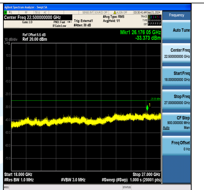
Band41_5MHz_16QAM_40265_1RB#0_18000~27000_18000~27000
