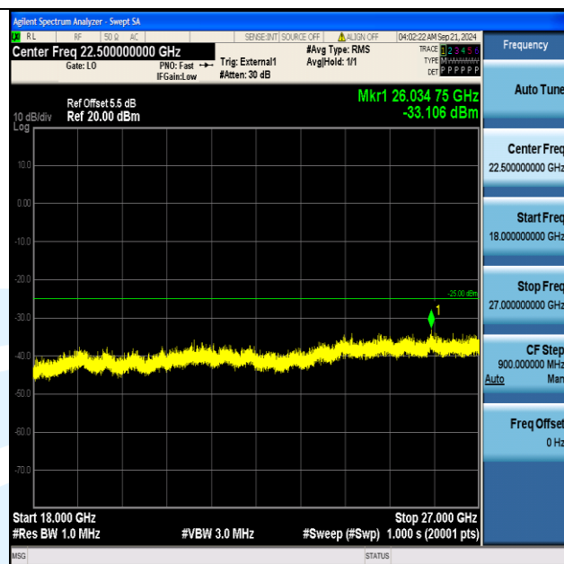
Band41_10MHz_QPSK_40290_1RB#49_18000~27000_18000~27000
