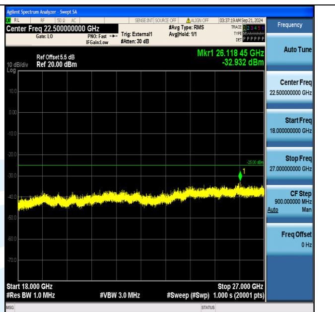
Band41_5MHz_16QAM_40265_25RB#0_18000~27000_18000~27000
