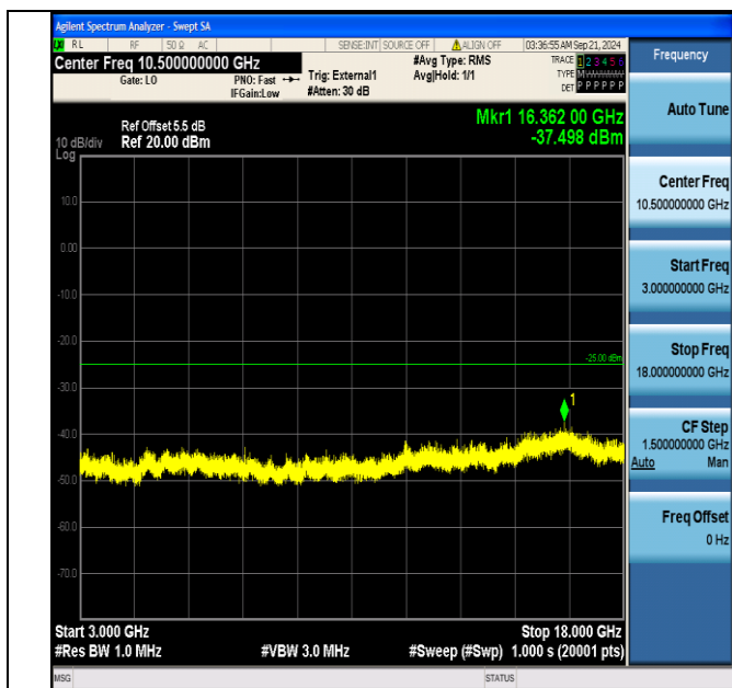
Band41_5MHz_16QAM_40265_25RB#0_3000~18000_3000~18000
