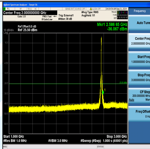
Band41_10MHz_QPSK_40290_50RB#0_1000~3000_1000~3000
