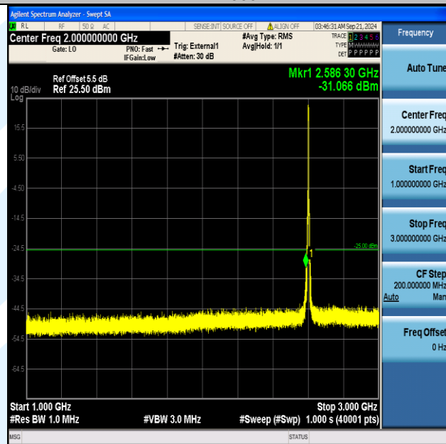
Band41_5MHz_16QAM_40690_25RB#0_1000~3000_1000~3000
