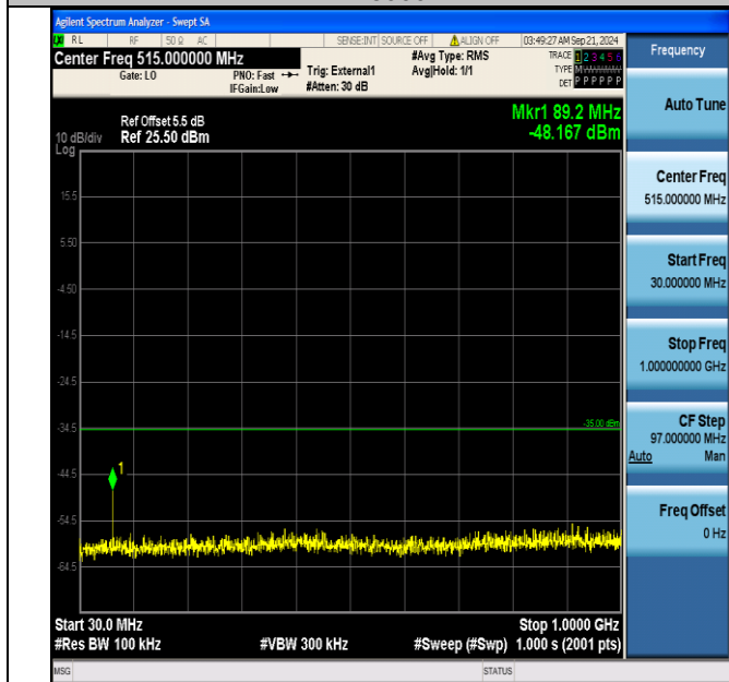
Band41_5MHz_16QAM_41215_1RB#0_30~1000_30~1000
