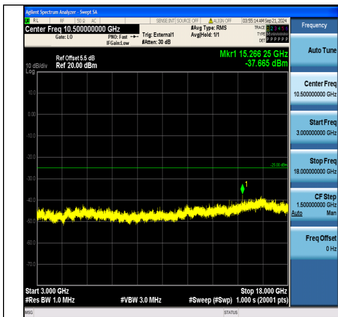
Band41_5MHz_QPSK_41215_25RB#0_3000~18000_3000~18000
