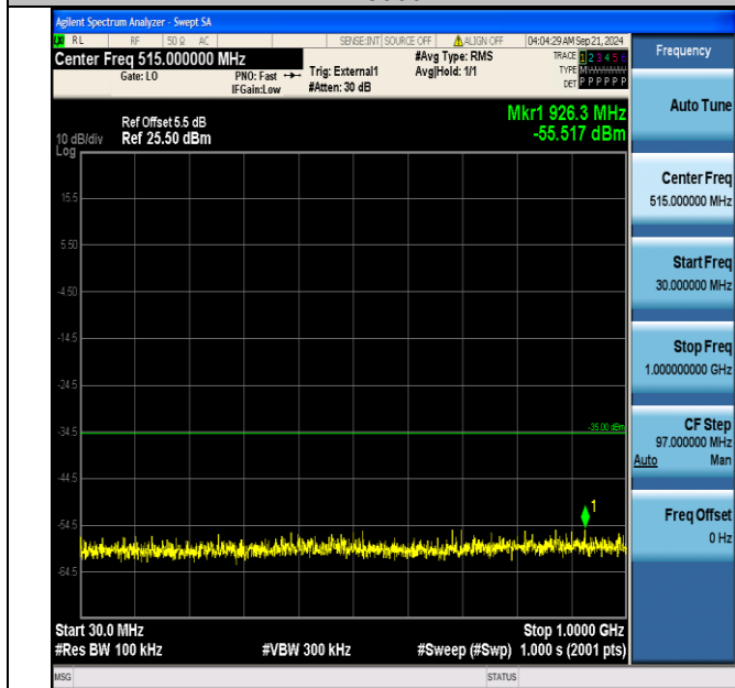
Band41_10MHz_QPSK_40290_50RB#0_30~1000_30~1000
