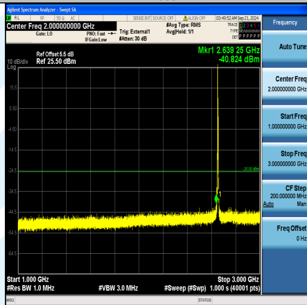
Band41_5MHz_16QAM_41215_1RB#0_1000~3000_1000~3000
