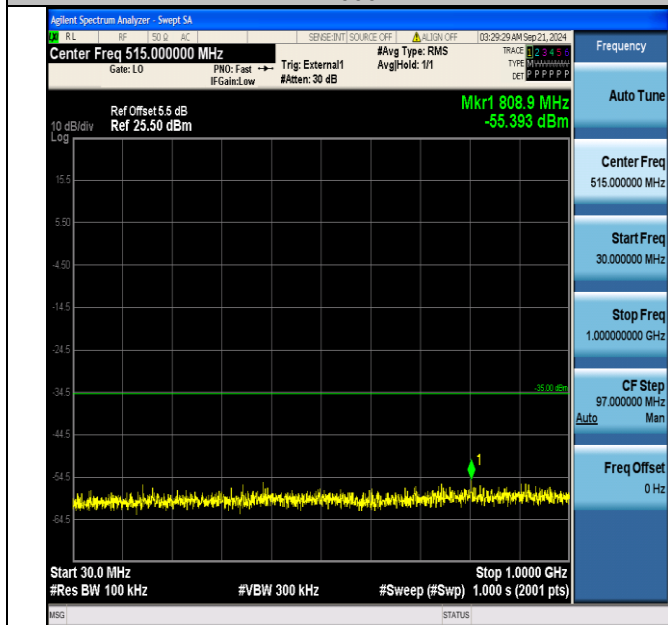
Band41_5MHz_16QAM_40265_1RB#0_30~1000_30~1000
