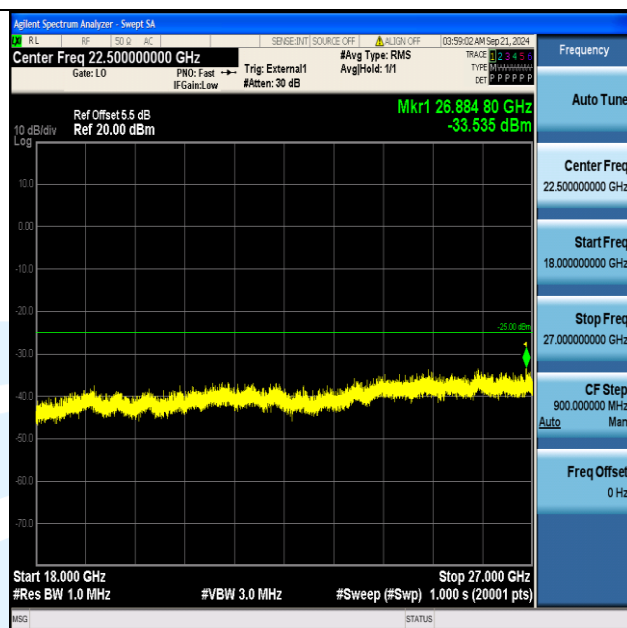
Band41_10MHz_QPSK_40290_1RB#0_18000~27000_18000~27000
