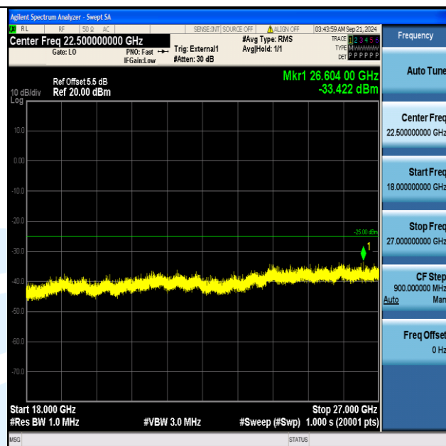
Band41_5MHz_16QAM_40690_1RB#24_18000~27000_18000~27000
