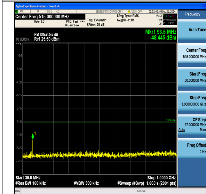
Band41_5MHz_16QAM_41215_1RB#24_30~1000_30~1000
