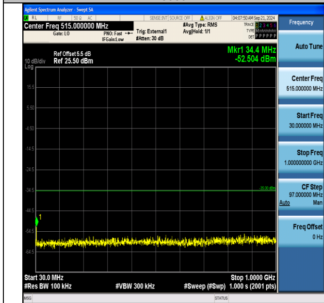
Band41_10MHz_QPSK_40690_1RB#0_30~1000_30~1000
