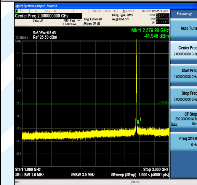
Band41_5MHz_16QAM_40265_1RB#0_1000~3000_1000~3000
