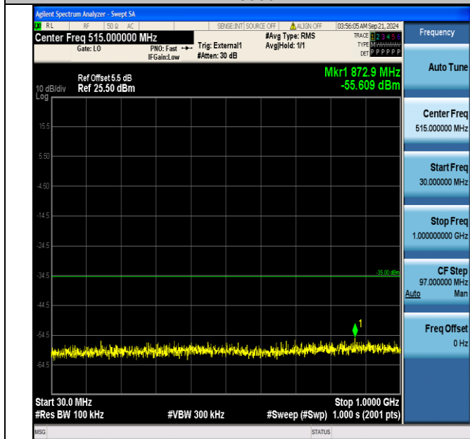
Band41_5MHz_16QAM_41215_25RB#0_30~1000_30~1000
