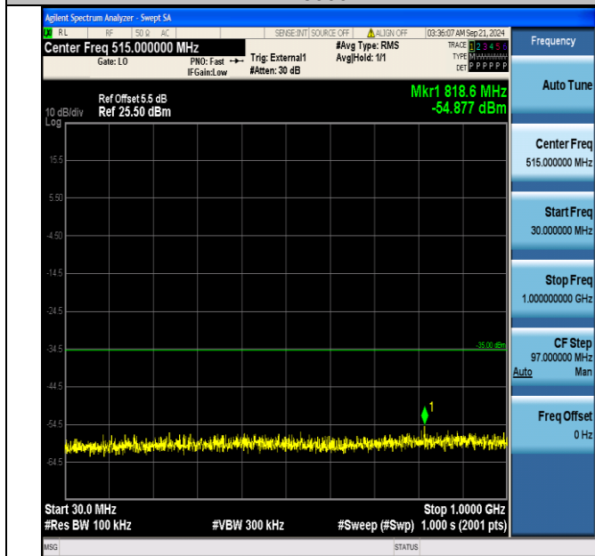
Band41_5MHz_16QAM_40265_25RB#0_30~1000_30~1000
