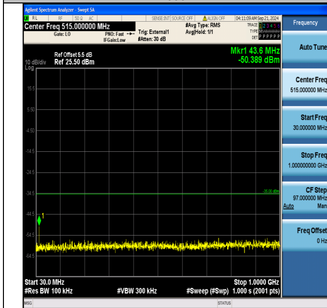
Band41_10MHz_QPSK_40690_1RB#49_30~1000_30~1000
