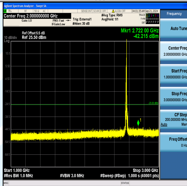
Band41_10MHz_QPSK_40290_1RB#49_1000~3000_1000~3000
