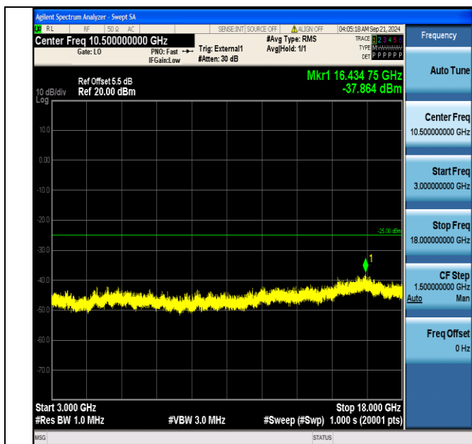
Band41_10MHz_QPSK_40290_50RB#0_3000~18000_3000~18000
