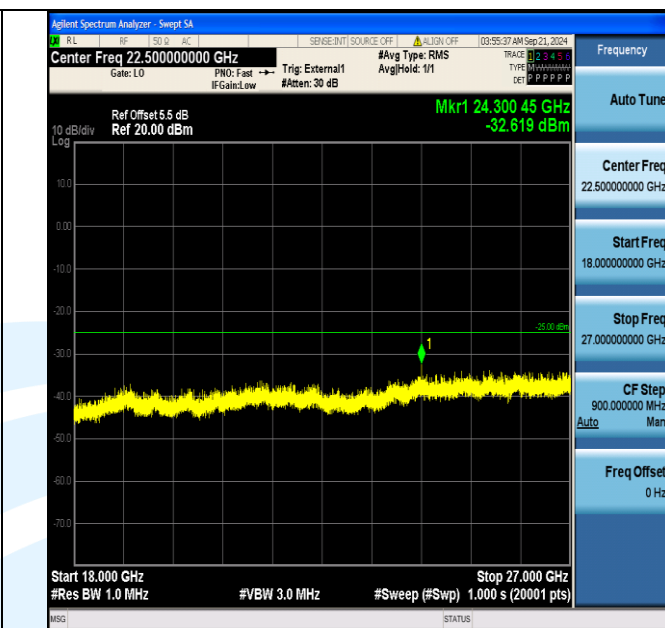
Band41_5MHz_QPSK_41215_25RB#0_18000~27000_18000~27000
