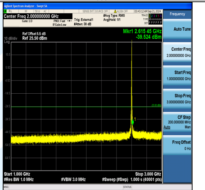
Band41_5MHz_16QAM_40690_1RB#24_1000~3000_1000~3000
