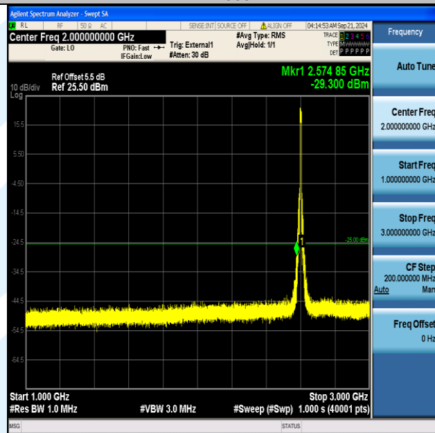
Band41_10MHz_QPSK_40690_50RB#0_1000~3000_1000~3000
