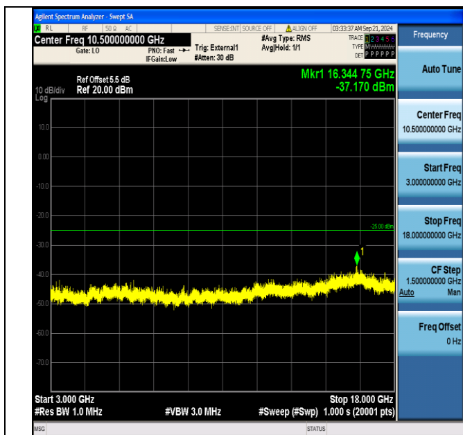
Band41_5MHz_16QAM_40265_1RB#24_3000~18000_3000~18000
