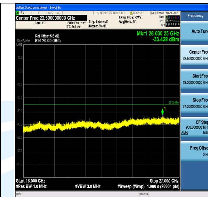
Band41_5MHz_16QAM_41215_1RB#0_18000~27000_18000~27000
