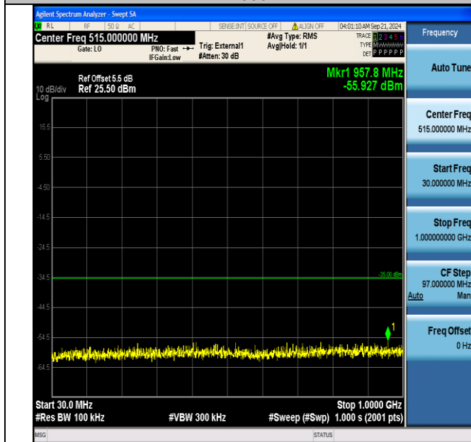
Band41_10MHz_QPSK_40290_1RB#49_30~1000_30~1000
