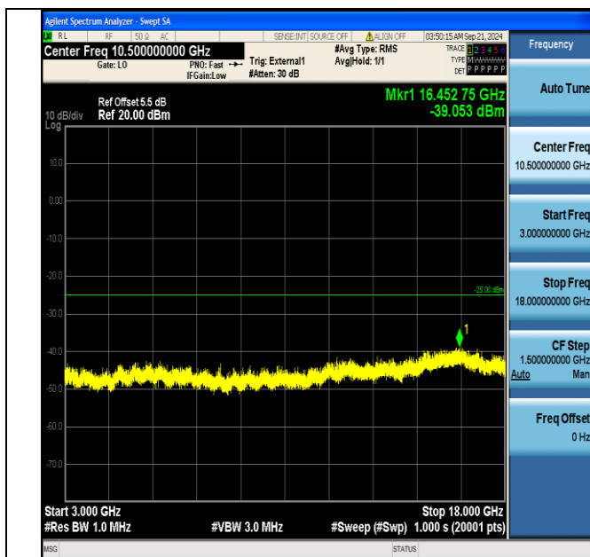
Band41_5MHz_16QAM_41215_1RB#0_3000~18000_3000~18000
