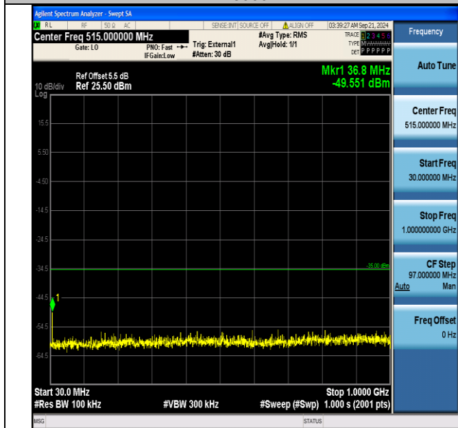
Band41_5MHz_16QAM_40690_1RB#0_30~1000_30~1000
