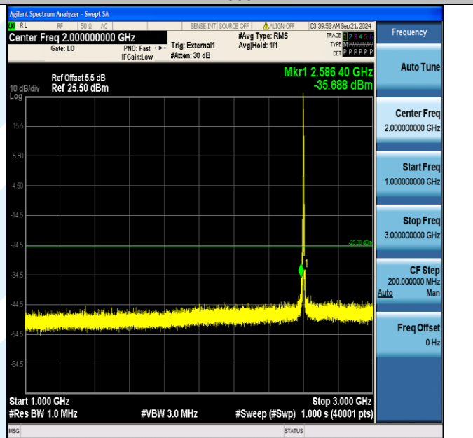
Band41_5MHz_16QAM_40690_1RB#0_1000~3000_1000~3000
