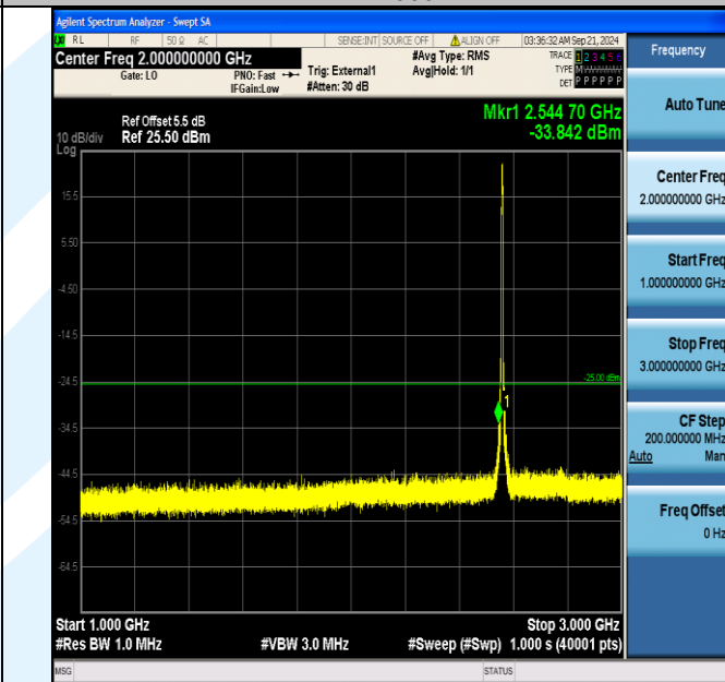
Band41_5MHz_16QAM_40265_25RB#0_1000~3000_1000~3000
