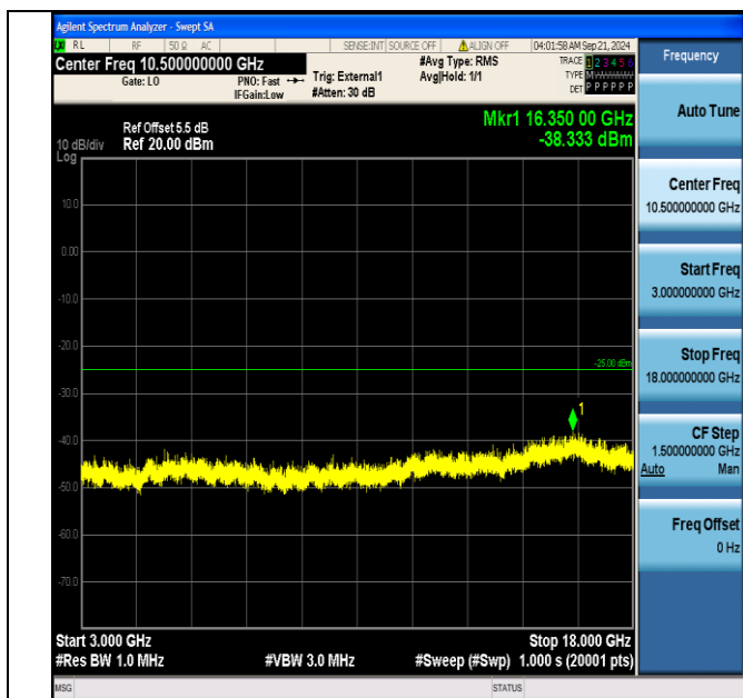
Band41_10MHz_QPSK_40290_1RB#49_3000~18000_3000~18000
