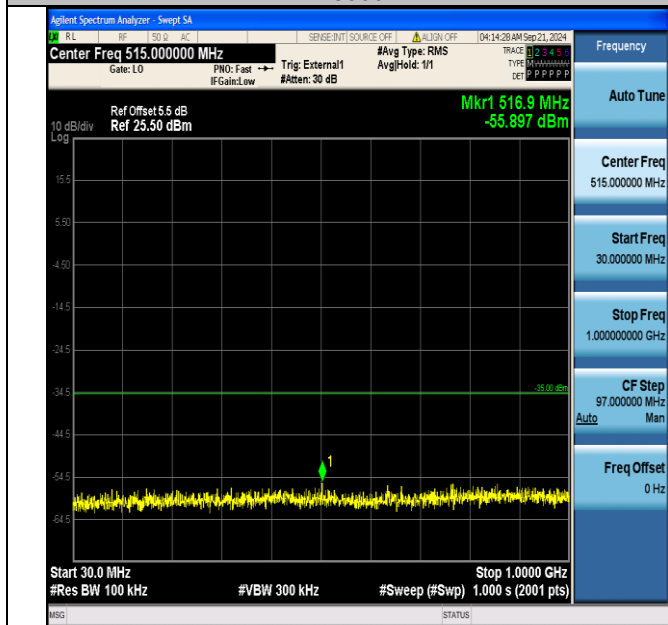
Band41_10MHz_QPSK_40690_50RB#0_30~1000_30~1000
