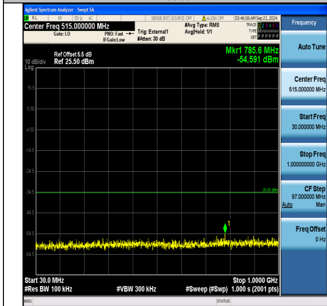
Band41_5MHz_16QAM_40690_25RB#0_30~1000_30~1000
