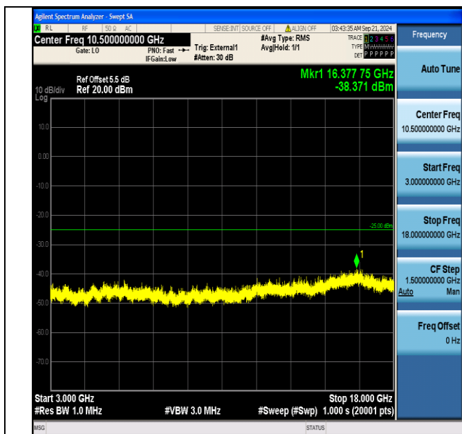
Band41_5MHz_16QAM_40690_1RB#24_3000~18000_3000~18000
