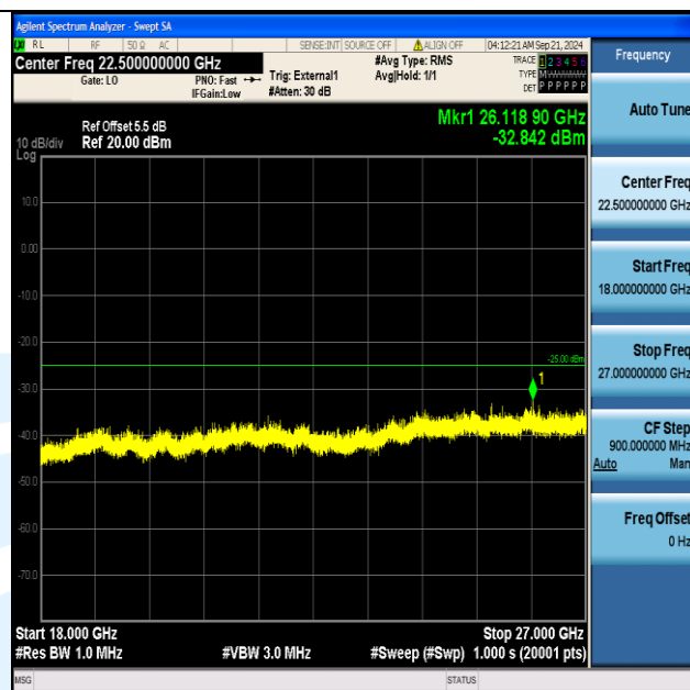
Band41_10MHz_QPSK_40690_1RB#49_18000~27000_18000~27000
