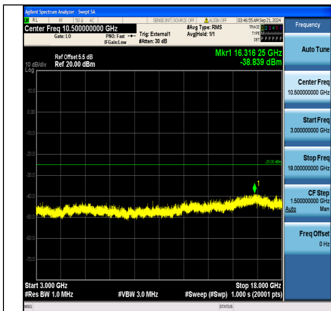
Band41_5MHz_16QAM_40690_25RB#0_3000~18000_3000~18000
