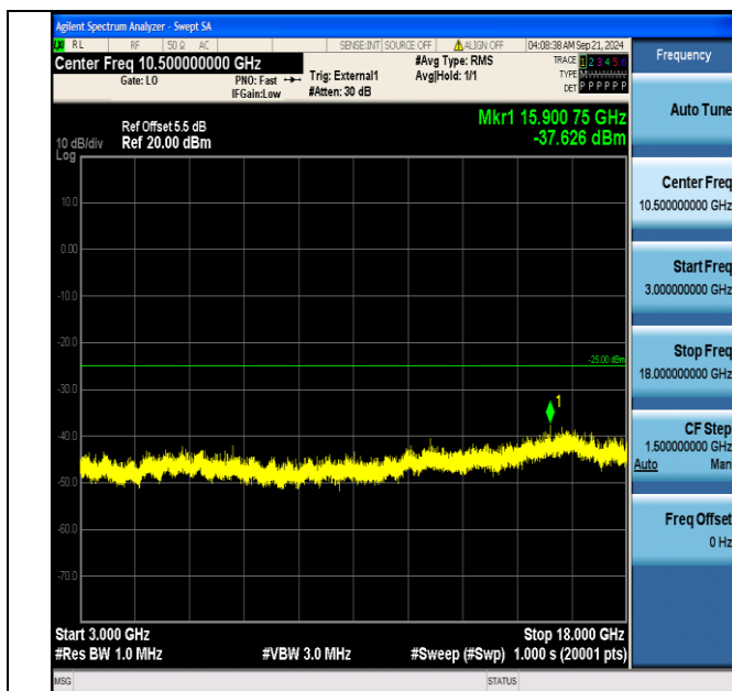
Band41_10MHz_QPSK_40690_1RB#0_3000~18000_3000~18000
