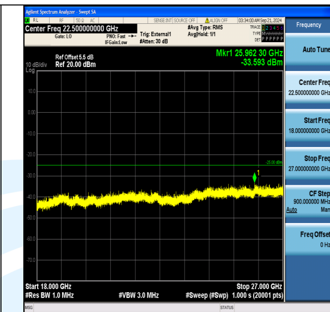
Band41_5MHz_16QAM_40265_1RB#24_18000~27000_18000~27000
