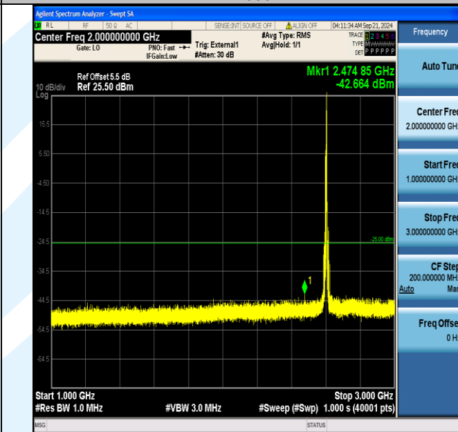
Band41_10MHz_QPSK_40690_1RB#49_1000~3000_1000~3000
