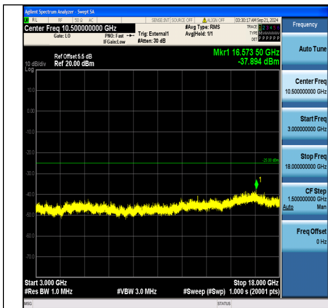
Band41_5MHz_16QAM_40265_1RB#0_3000~18000_3000~18000
