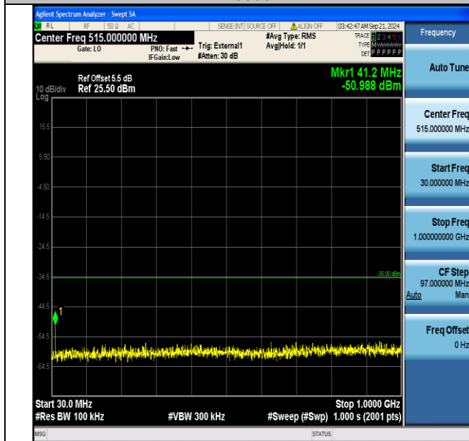
Band41_5MHz_16QAM_40690_1RB#24_30~1000_30~1000
