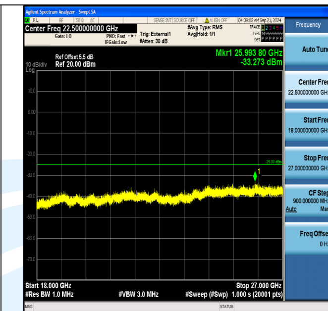
Band41_10MHz_QPSK_40690_1RB#0_18000~27000_18000~27000
