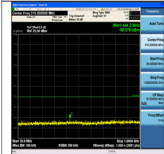
Band41_5MHz_16QAM_40265_1RB#24_30~1000_30~1000
