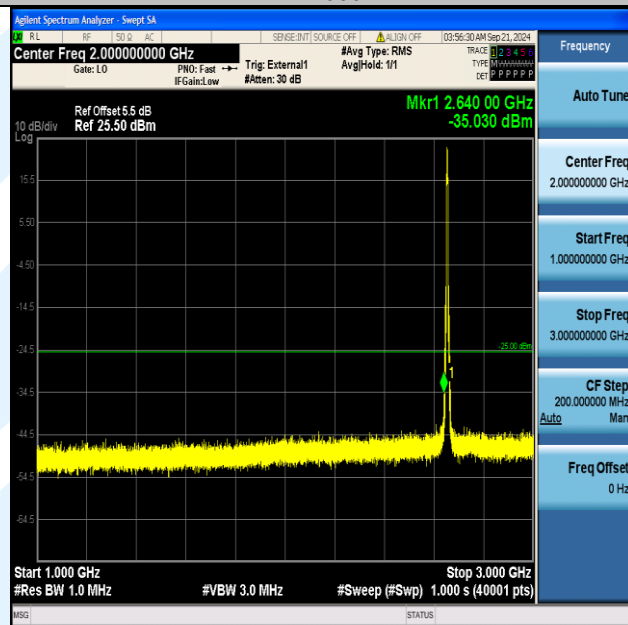
Band41_5MHz_16QAM_41215_25RB#0_1000~3000_1000~3000
