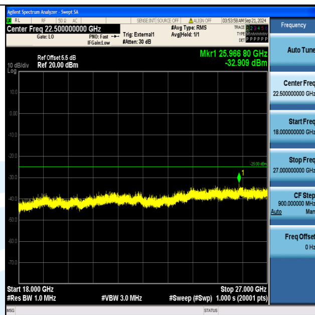
Band41_5MHz_16QAM_41215_1RB#24_18000~27000_18000~27000
