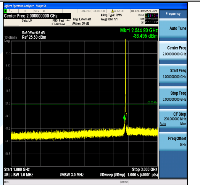
Band41_5MHz_16QAM_40265_1RB#24_1000~3000_1000~3000
