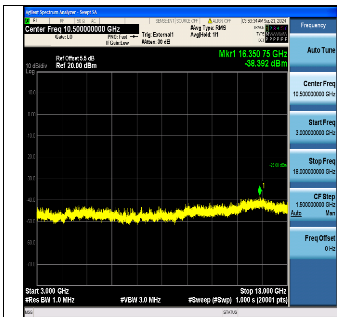
Band41_5MHz_16QAM_41215_1RB#24_3000~18000_3000~18000
