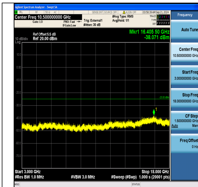
Band41_10MHz_QPSK_40290_1RB#0_3000~18000_3000~18000
