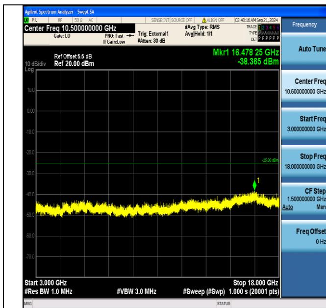
Band41_5MHz_16QAM_40690_1RB#0_3000~18000_3000~18000
