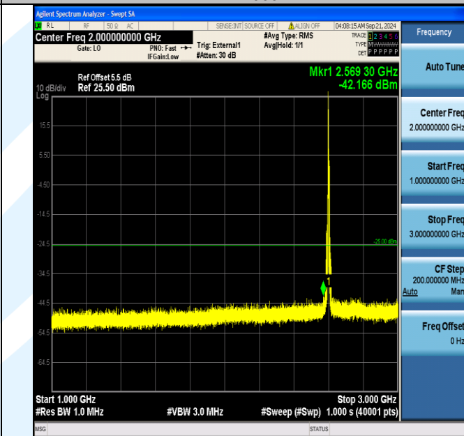
Band41_10MHz_QPSK_40690_1RB#0_1000~3000_1000~3000
