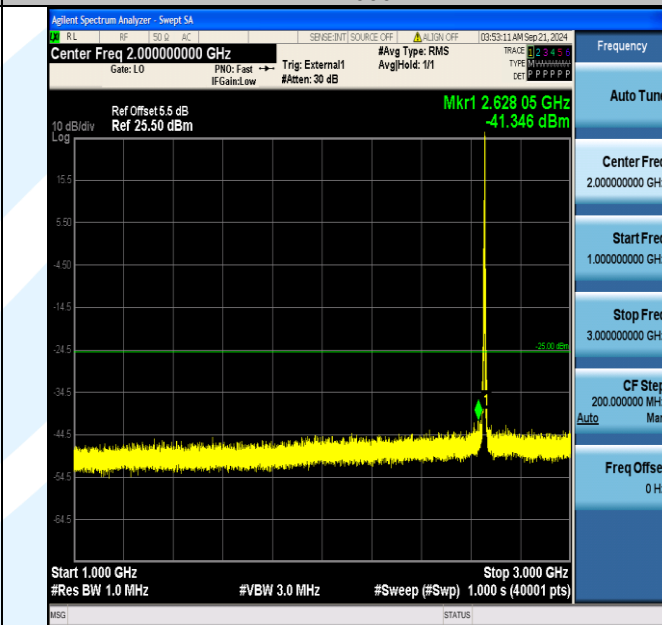
Band41_5MHz_16QAM_41215_1RB#24_1000~3000_1000~3000
