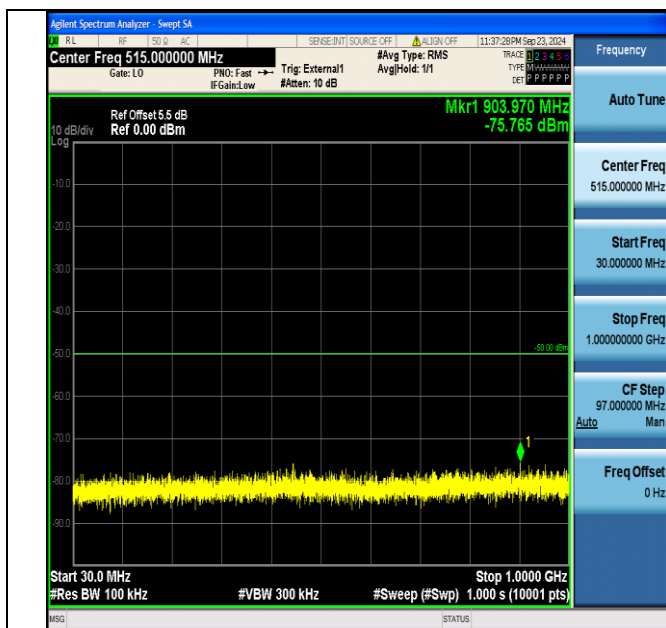
Band40_5MHz_QPSK_39225_1RB#0_30~1000_30~1000
