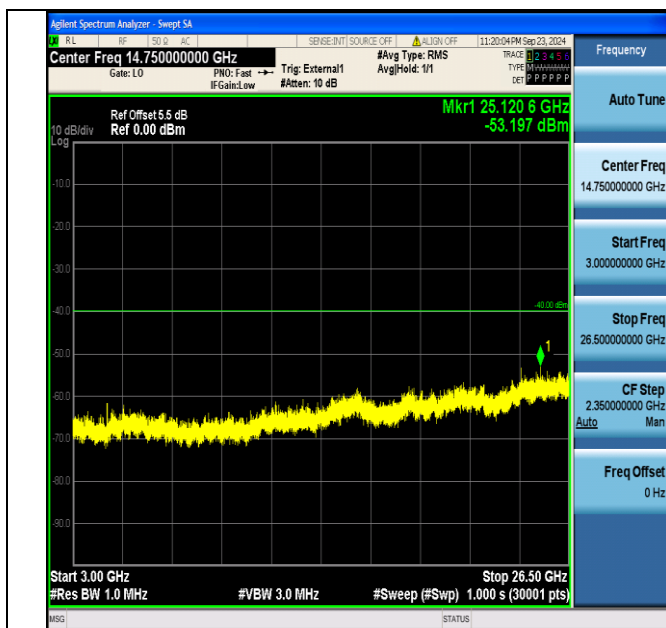
Band40_10MHz_QPSK_38750_50RB#0_3000~26500_3000~26500
