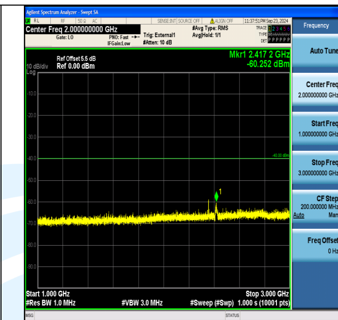
Band40_5MHz_QPSK_39225_1RB#0_1000~3000_1000~3000
