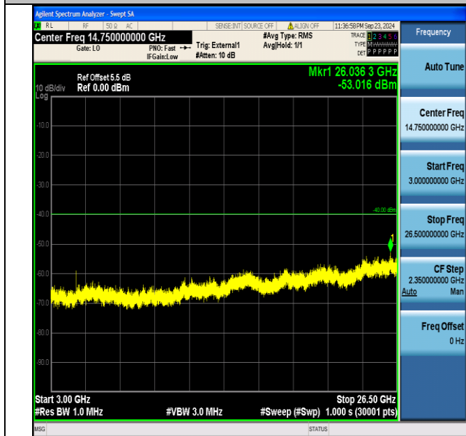
Band40_5MHz_16QAM_39200_25RB#0_3000~26500_3000~26500
