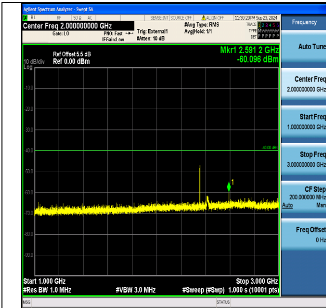
Band40_5MHz_QPSK_39200_1RB#0_1000~3000_1000~3000
