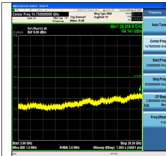
Band40_5MHz_QPSK_39200_1RB#24_3000~26500_3000~26500
