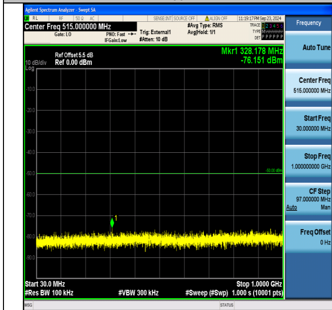
Band40_10MHz_QPSK_38750_50RB#0_30~1000_30~1000
