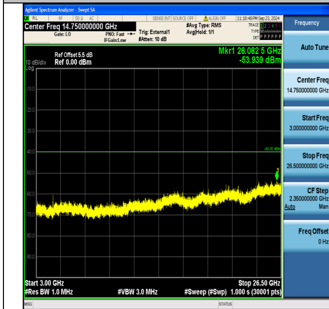
Band40_10MHz_16QAM_38750_1RB#49_3000~26500_3000~26500
