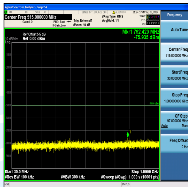
Band40_5MHz_QPSK_39175_1RB#24_30~1000_30~1000
