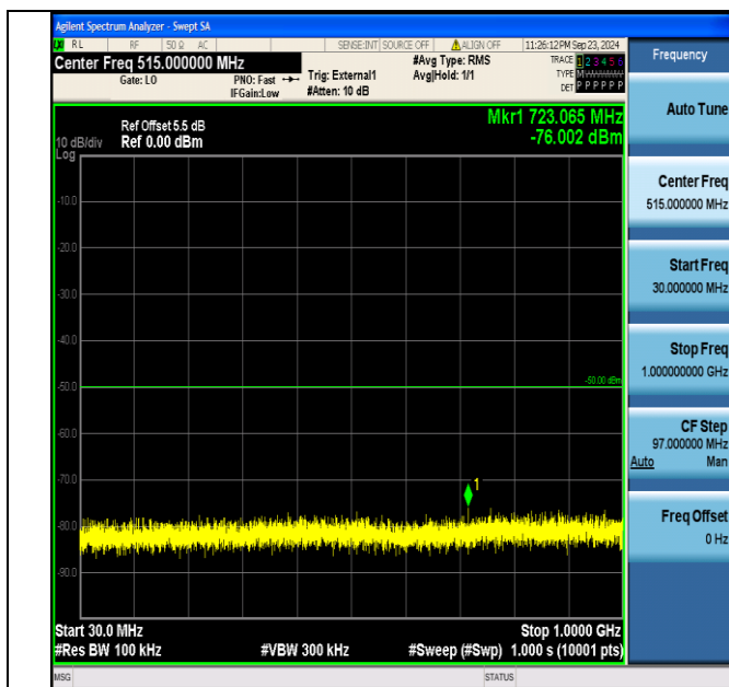
Band40_5MHz_16QAM_39175_1RB#24_30~1000_30~1000
