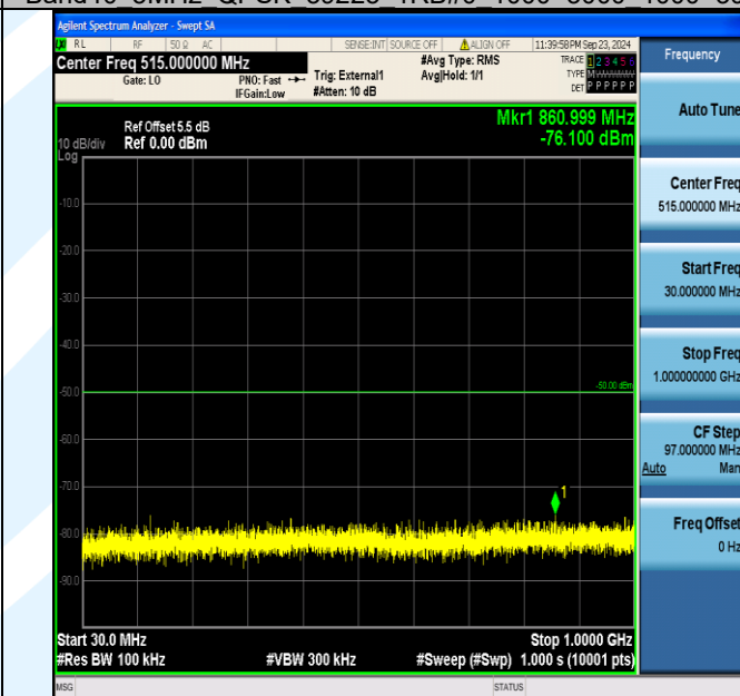
Band40_5MHz_QPSK_39225_1RB#24_30~1000_30~1000
