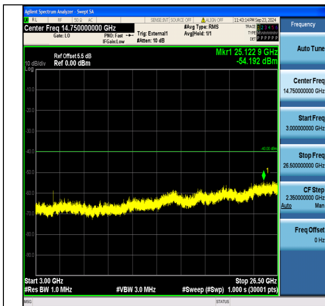
Band40_5MHz_QPSK_39225_25RB#0_3000~26500_3000~26500
