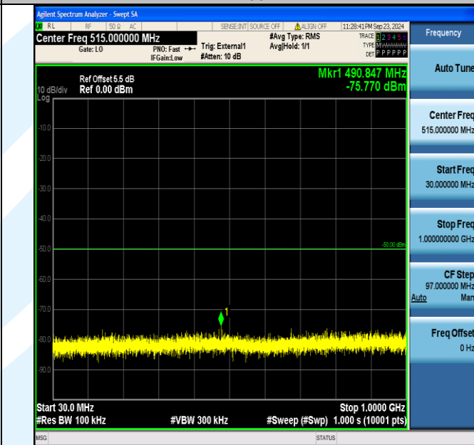
Band40_5MHz_16QAM_39175_25RB#0_30~1000_30~1000
