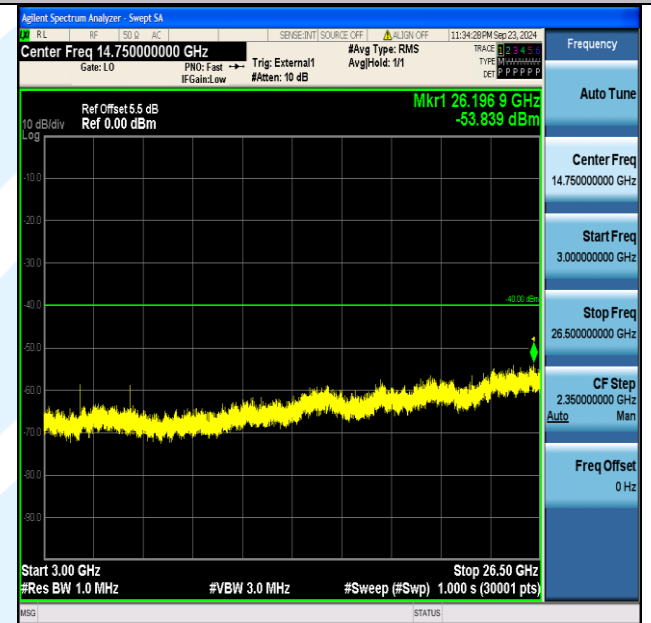
Band40_5MHz_16QAM_39200_1RB#24_3000~26500_3000~26500
