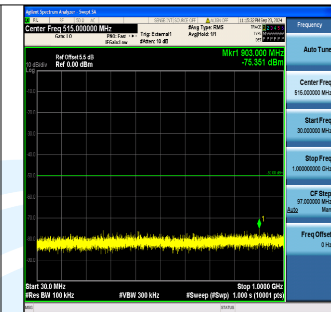
Band40_10MHz_16QAM_38750_1RB#0_30~1000_30~1000
