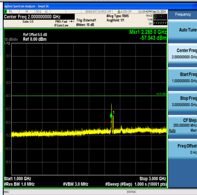
Band40_10MHz_QPSK_38750_50RB#0_1000~3000_1000~3000
