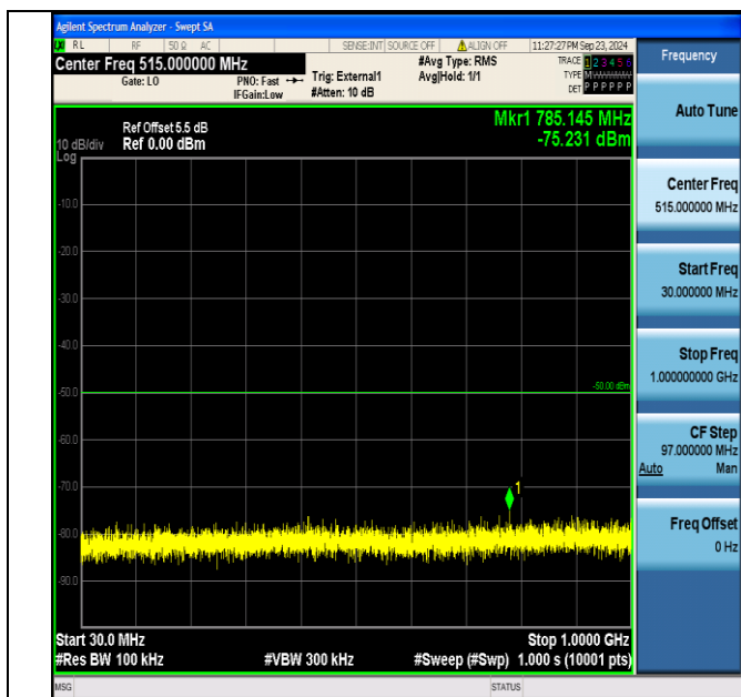
Band40_5MHz_QPSK_39175_25RB#0_30~1000_30~1000
