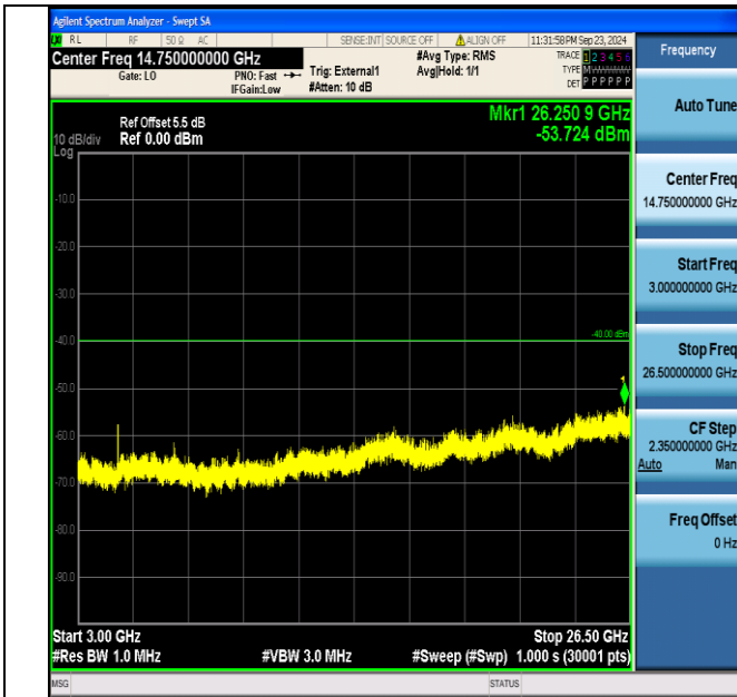
Band40_5MHz_16QAM_39200_1RB#0_3000~26500_3000~26500
