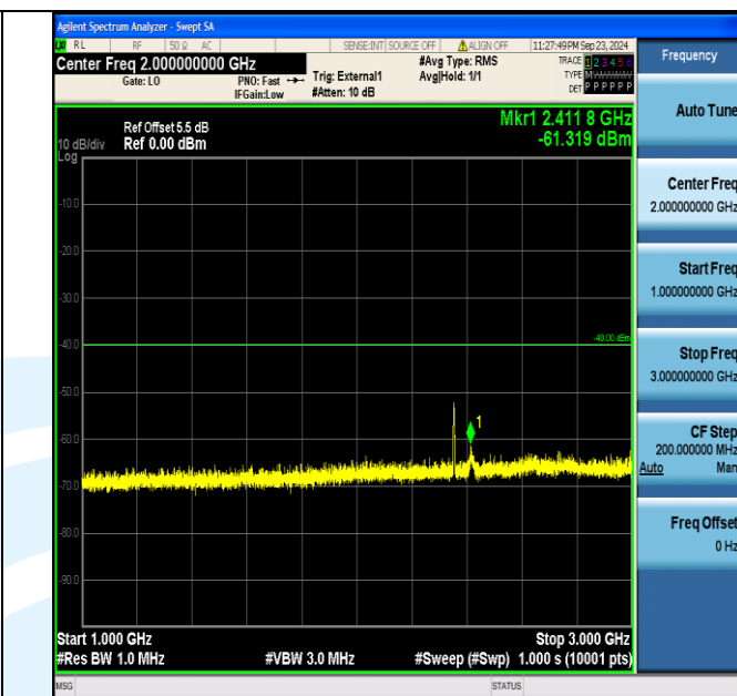
Band40_5MHz_QPSK_39175_25RB#0_1000~3000_1000~3000
