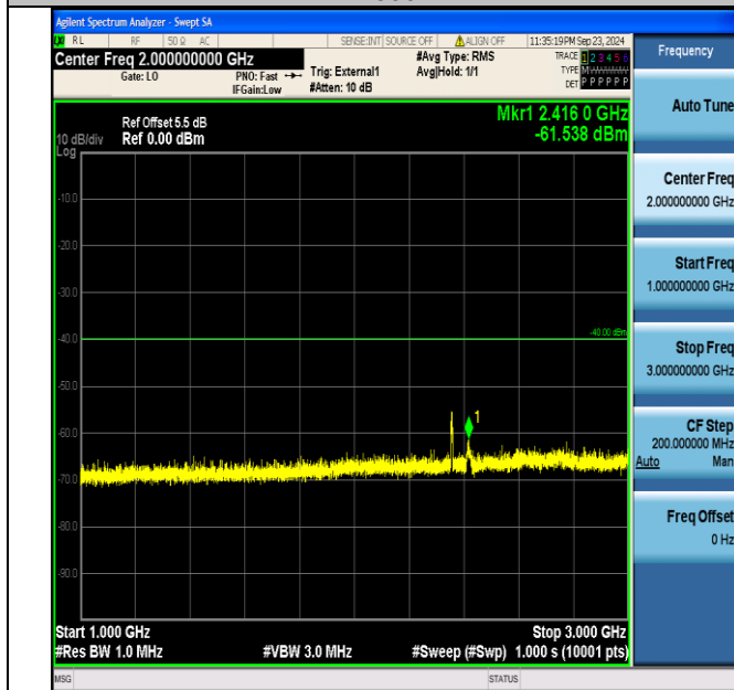
Band40_5MHz_QPSK_39200_25RB#0_1000~3000_1000~3000
