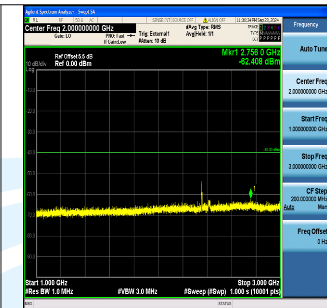
Band40_5MHz_16QAM_39200_25RB#0_1000~3000_1000~3000
