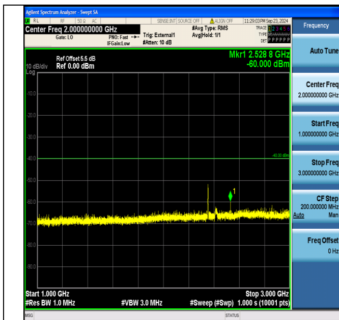
Band40_5MHz_16QAM_39175_25RB#0_1000~3000_1000~3000
