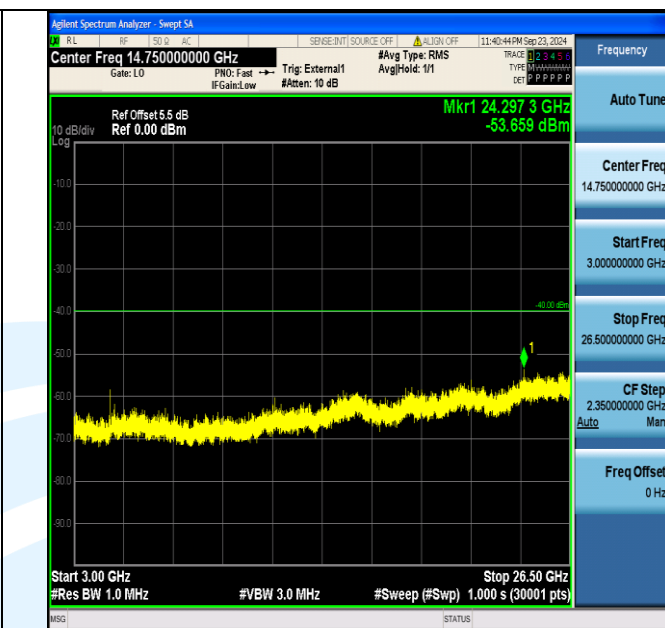
Band40_5MHz_QPSK_39225_1RB#24_3000~26500_3000~26500
