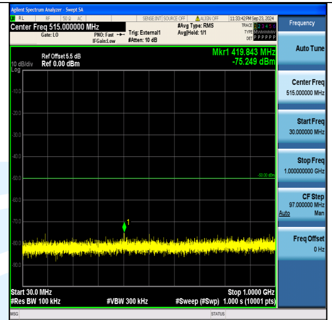
Band40_5MHz_16QAM_39200_1RB#24_30~1000_30~1000
