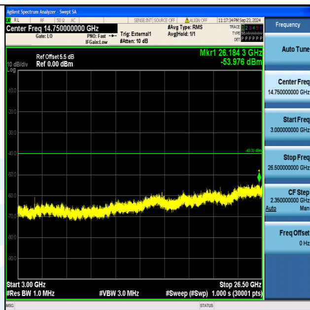
Band40_10MHz_QPSK_38750_1RB#49_3000~26500_3000~26500
