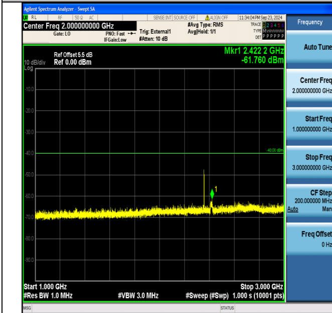
Band40_5MHz_16QAM_39200_1RB#24_1000~3000_1000~3000
