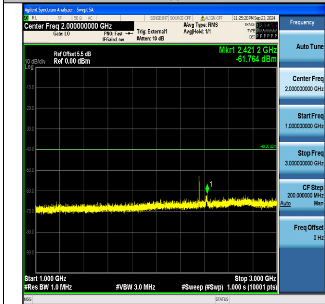
Band40_5MHz_QPSK_39175_1RB#24_1000~3000_1000~3000
