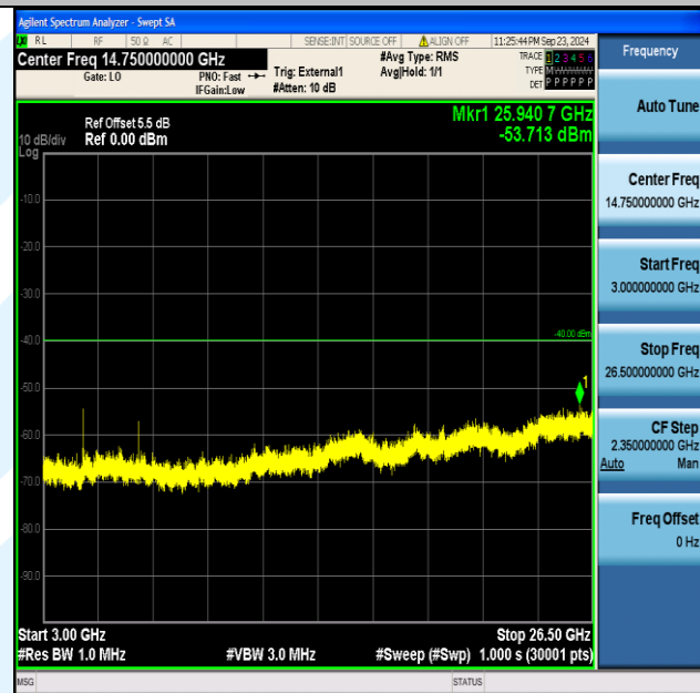
Band40_5MHz_QPSK_39175_1RB#24_3000~26500_3000~26500
