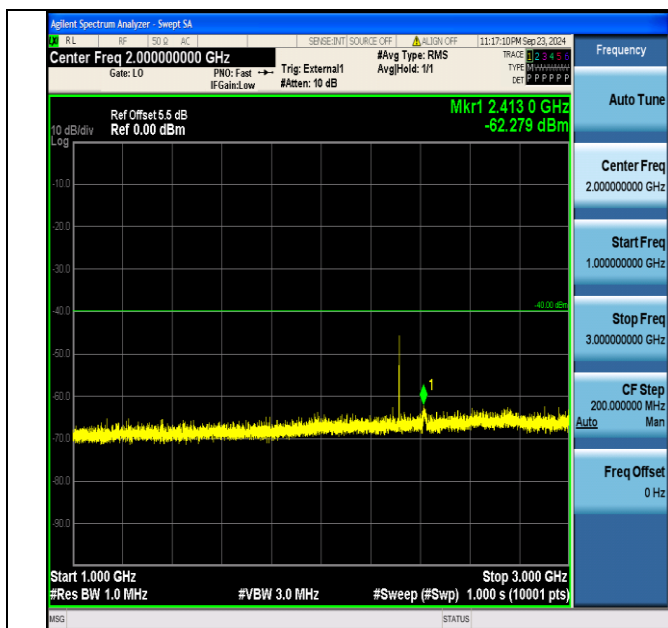
Band40_10MHz_QPSK_38750_1RB#49_1000~3000_1000~3000
