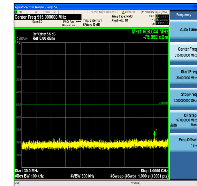
Band40_10MHz_16QAM_38750_1RB#49_30~1000_30~1000
