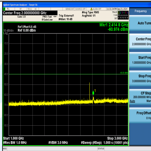
Band40_5MHz_16QAM_39200_1RB#0_1000~3000_1000~3000
