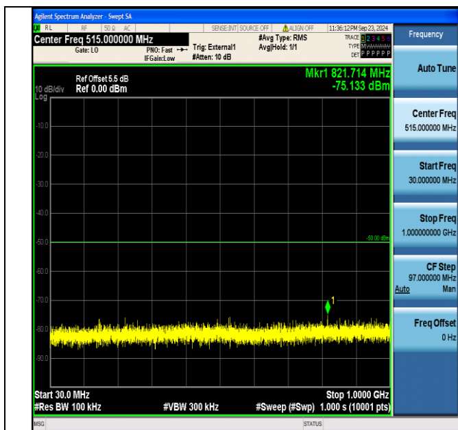
Band40_5MHz_16QAM_39200_25RB#0_30~1000_30~1000
