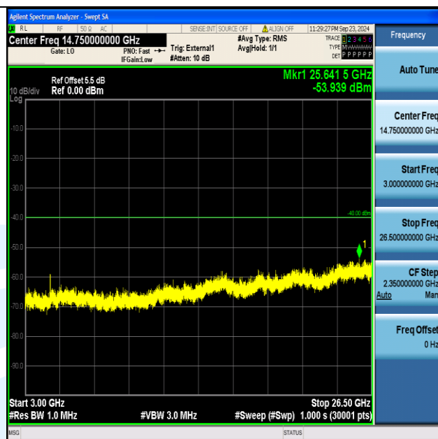
Band40_5MHz_16QAM_39175_25RB#0_3000~26500_3000~26500
