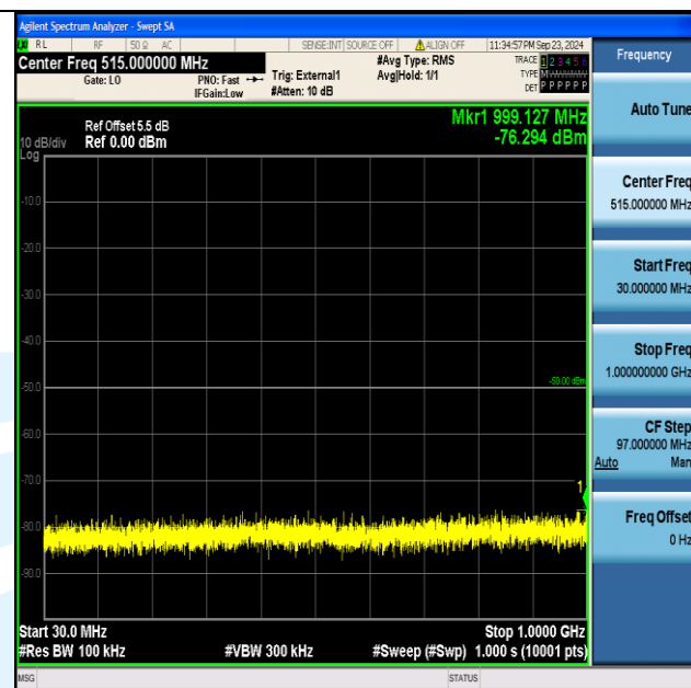
Band40_5MHz_QPSK_39200_25RB#0_30~1000_30~1000
