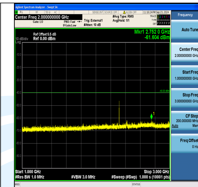
Band40_10MHz_16QAM_38750_1RB#49_1000~3000_1000~3000
