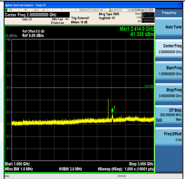
Band40_5MHz_QPSK_39200_1RB#24_1000~3000_1000~3000
