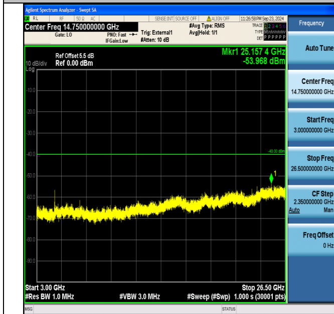
Band40_5MHz_16QAM_39175_1RB#24_3000~26500_3000~26500
