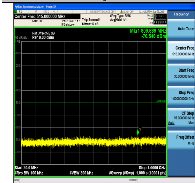
Band40_5MHz_QPSK_39225_25RB#0_30~1000_30~1000
