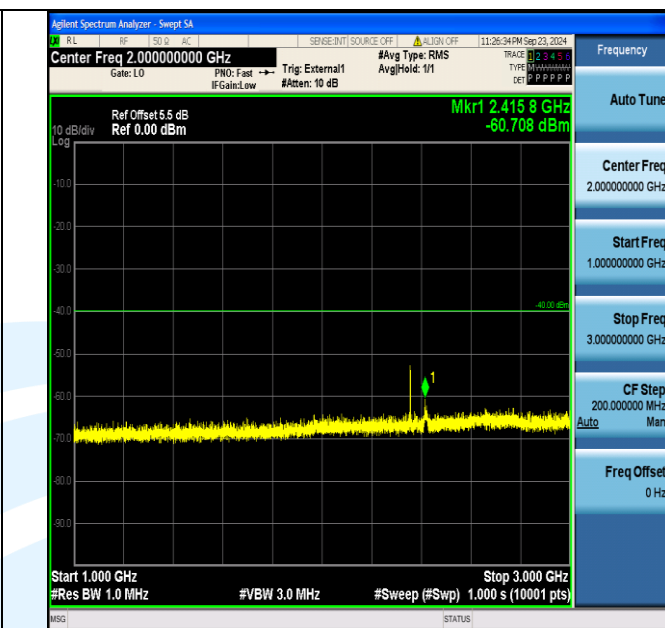
Band40_5MHz_16QAM_39175_1RB#24_1000~3000_1000~3000
