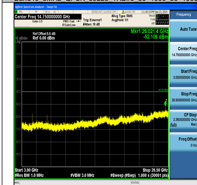
Band40_5MHz_QPSK_39225_1RB#0_3000~26500_3000~26500
