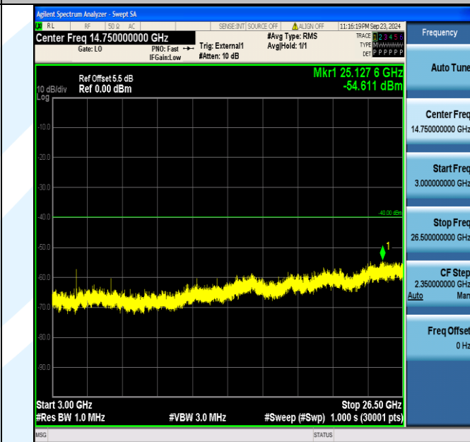
Band40_10MHz_16QAM_38750_1RB#0_3000~26500_3000~26500
