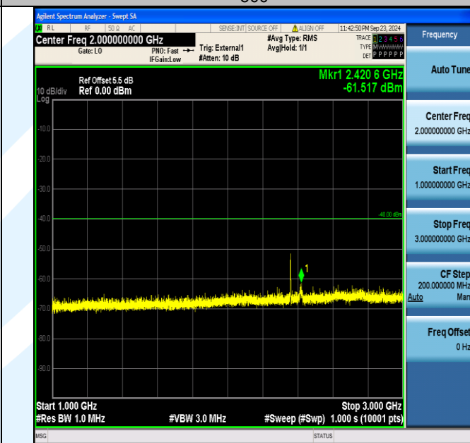
Band40_5MHz_QPSK_39225_25RB#0_1000~3000_1000~3000
