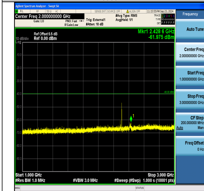
Band40_10MHz_16QAM_38750_1RB#0_1000~3000_1000~3000
