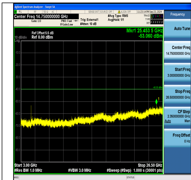
Band40_5MHz_QPSK_39175_1RB#0_3000~26500_3000~26500
