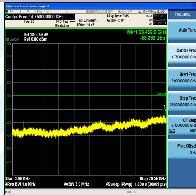
Band40_5MHz_QPSK_39200_25RB#0_3000~26500_3000~26500
