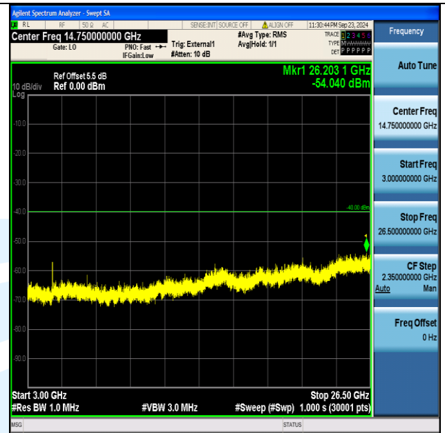
Band40_5MHz_QPSK_39200_1RB#0_3000~26500_3000~26500
