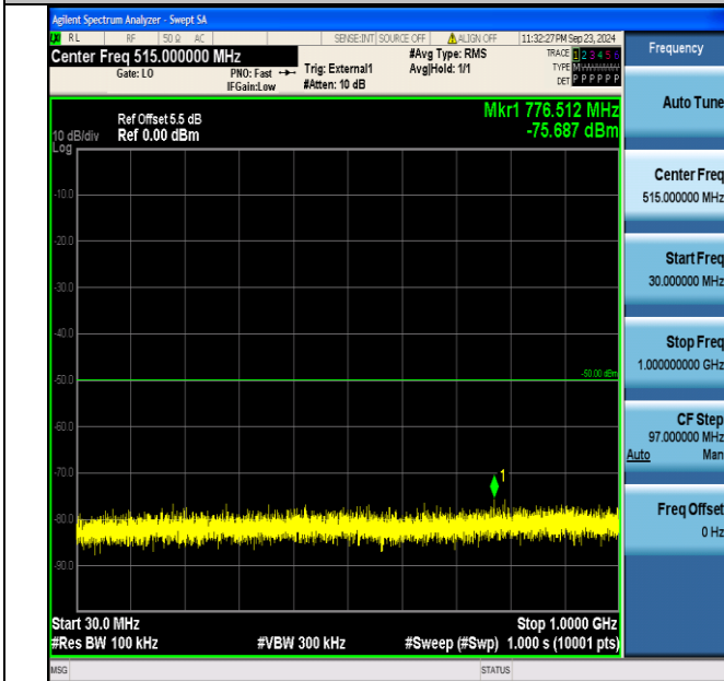
Band40_5MHz_QPSK_39200_1RB#24_30~1000_30~1000
