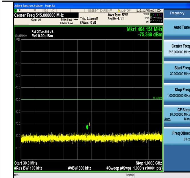
Band40_5MHz_16QAM_39200_1RB#0_30~1000_30~1000
