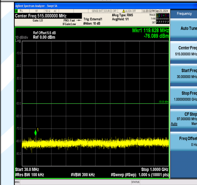
Band40_10MHz_16QAM_38750_50RB#0_30~1000_30~1000
