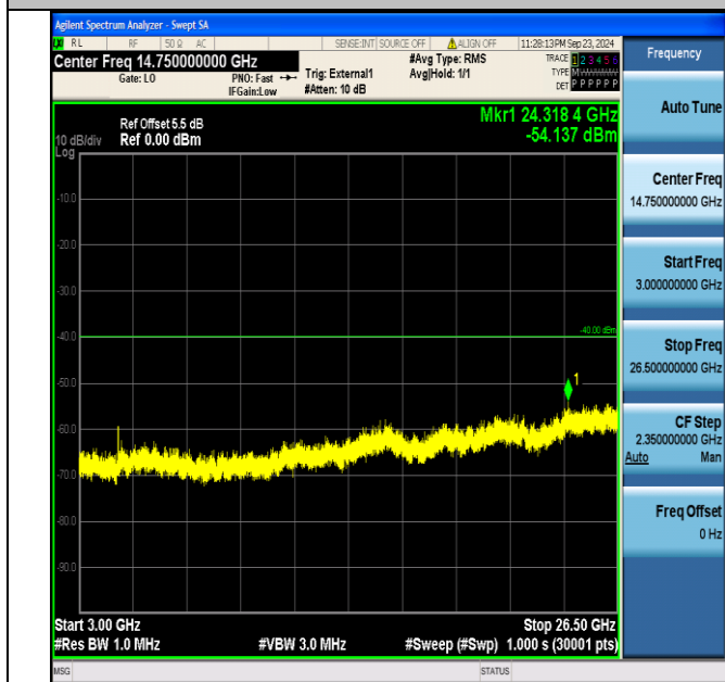
Band40_5MHz_QPSK_39175_25RB#0_3000~26500_3000~26500
