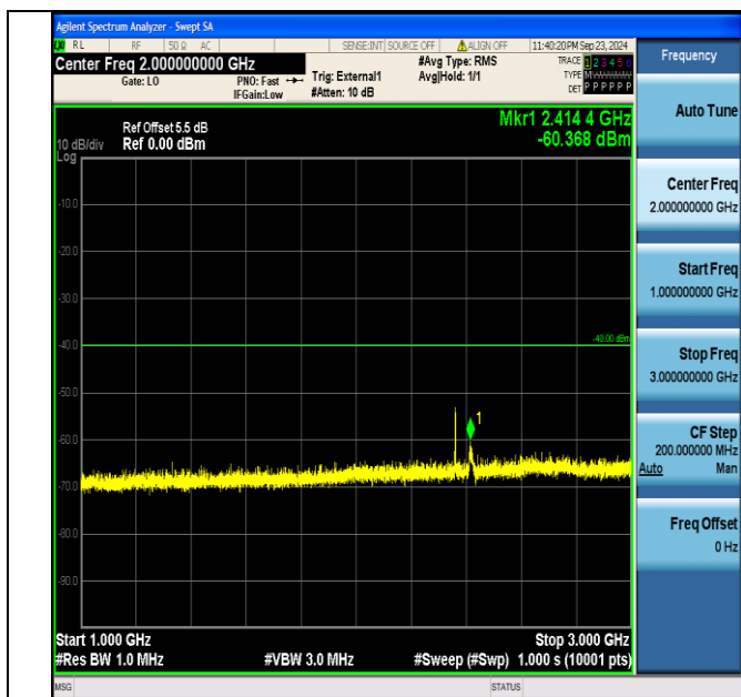
Band40_5MHz_QPSK_39225_1RB#24_1000~3000_1000~3000
