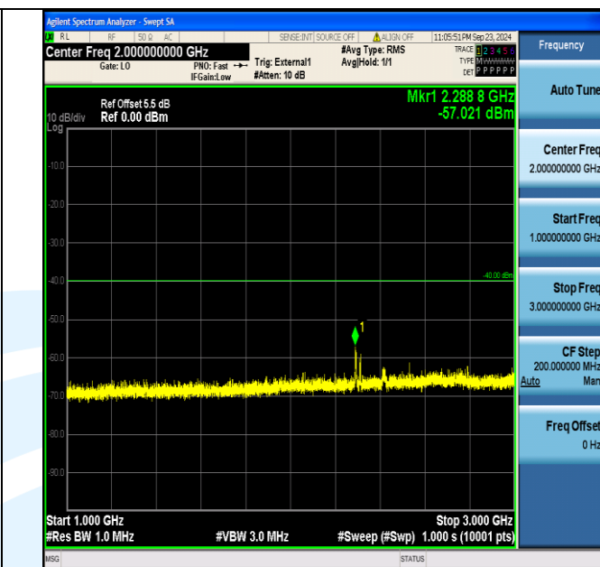
Band40_5MHz_16QAM_38750_25RB#0_1000~3000_1000~3000
