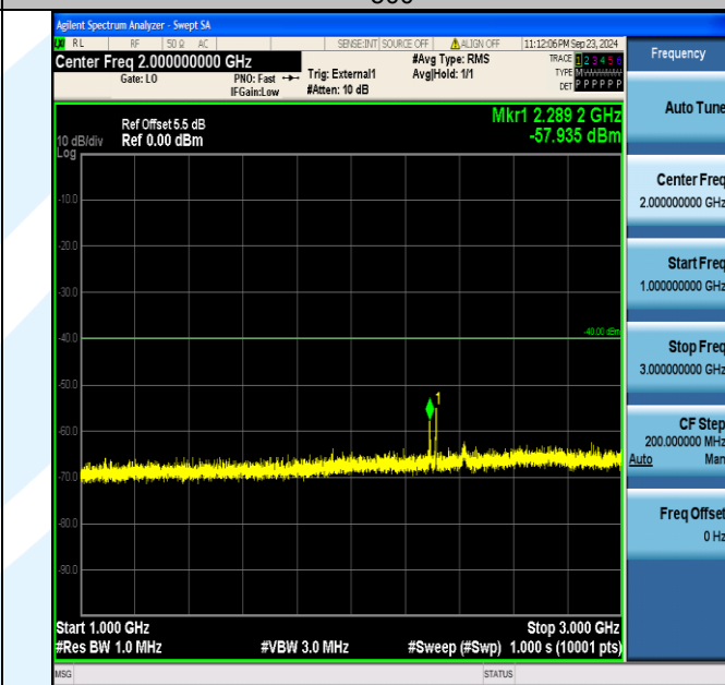
Band40_5MHz_QPSK_38775_25RB#0_1000~3000_1000~3000
