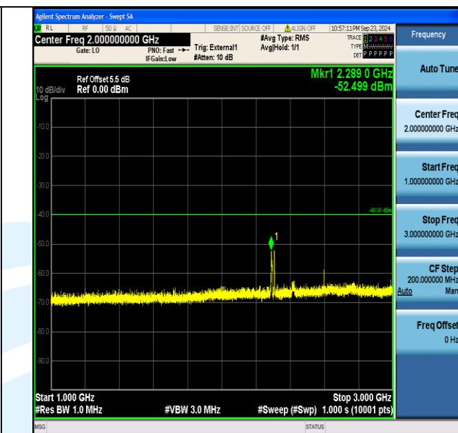
Band40_5MHz_QPSK_38725_25RB#0_1000~3000_1000~3000
