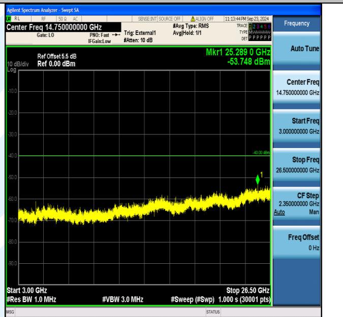
Band40_5MHz_16QAM_38775_25RB#0_3000~26500_3000~26500
