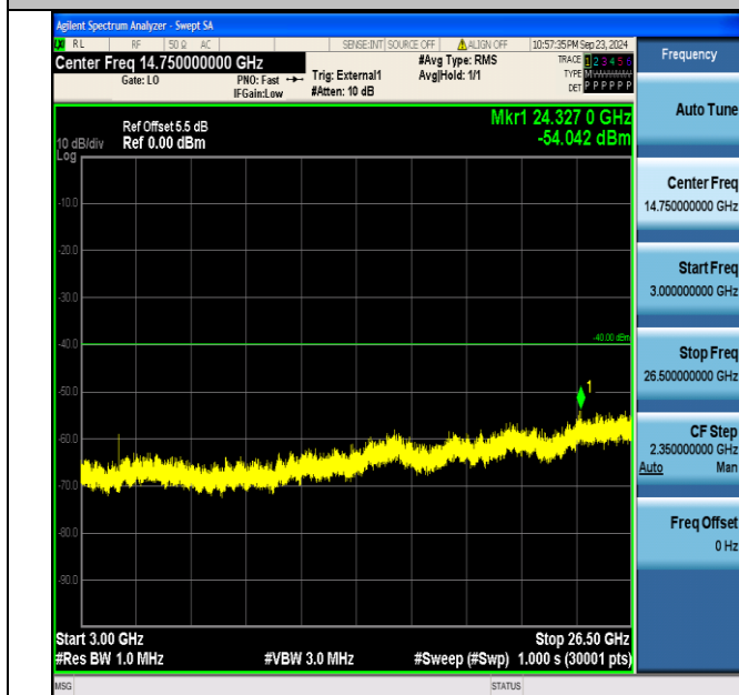
Band40_5MHz_QPSK_38725_25RB#0_3000~26500_3000~26500
