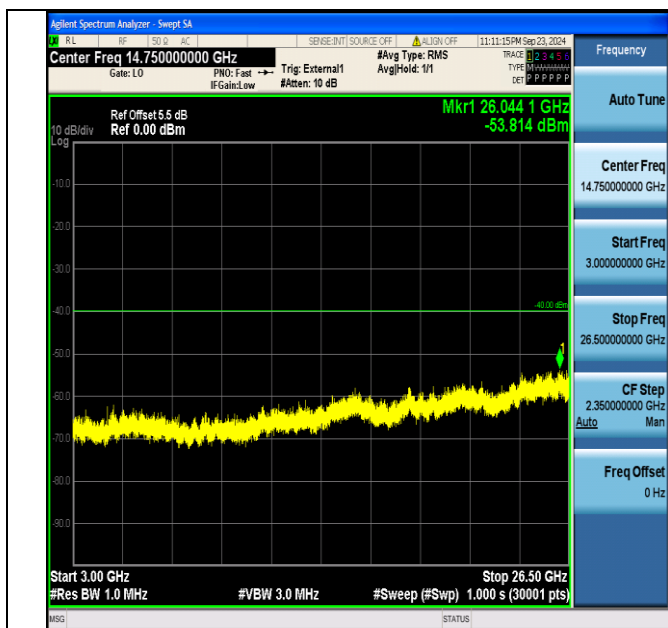
Band40_5MHz_16QAM_38775_1RB#24_3000~26500_3000~26500
