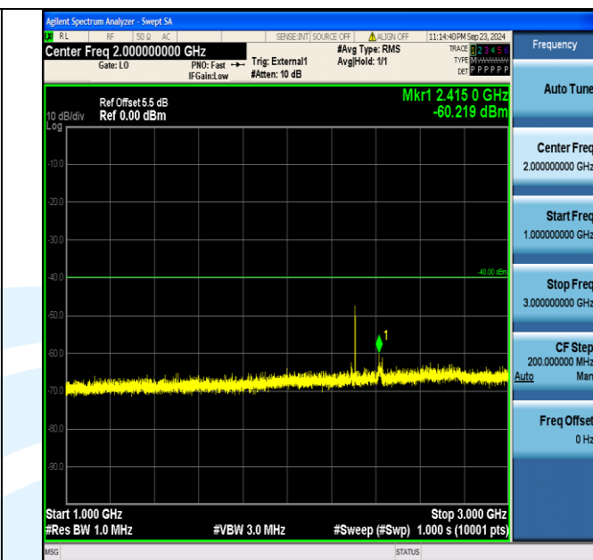
Band40_10MHz_QPSK_38750_1RB#0_1000~3000_1000~3000
