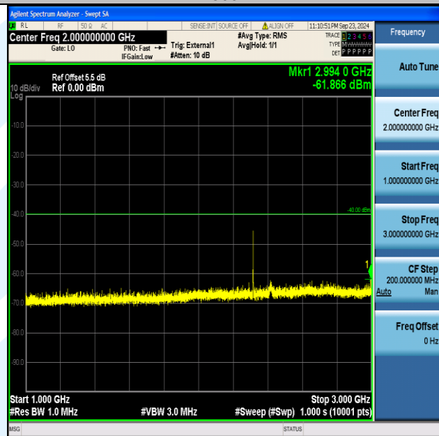
Band40_5MHz_16QAM_38775_1RB#24_1000~3000_1000~3000
