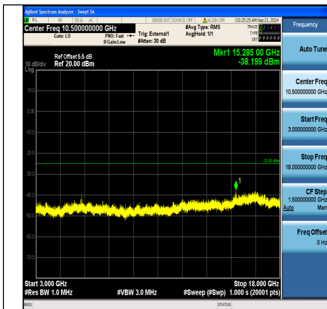
Band38_20MHz_16QAM_38150_100RB#0_3000~18000_3000~18000
