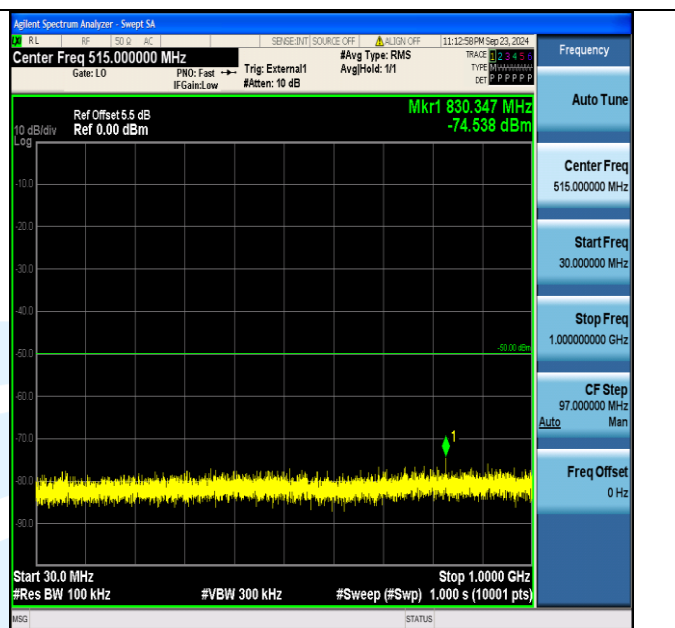
Band40_5MHz_16QAM_38775_25RB#0_30~1000_30~1000
