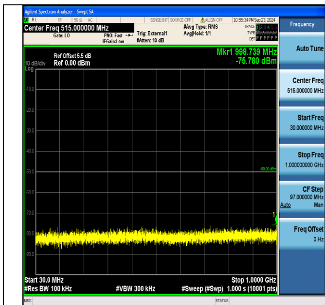
Band40_5MHz_16QAM_38725_1RB#24_30~1000_30~1000
