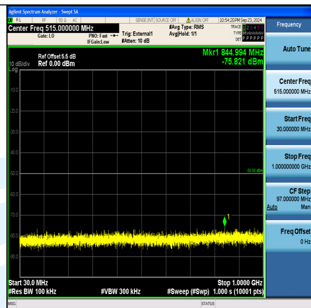
Band40_5MHz_QPSK_38725_1RB#24_30~1000_30~1000
