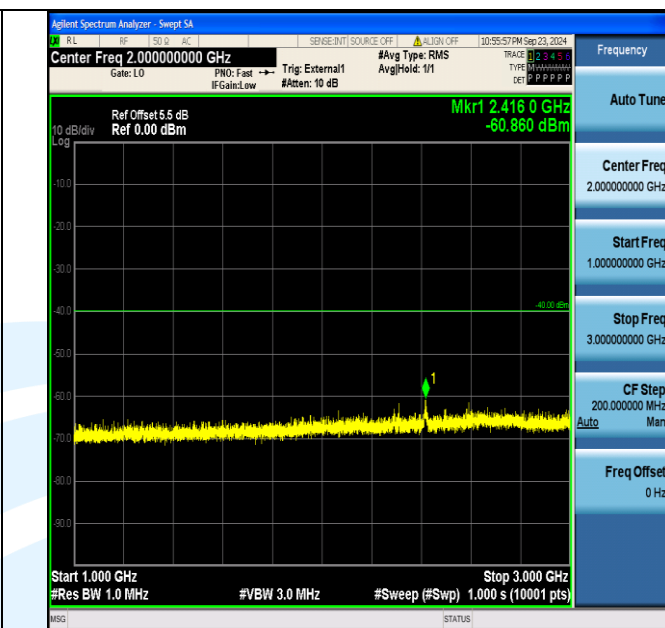
Band40_5MHz_16QAM_38725_1RB#24_1000~3000_1000~3000
