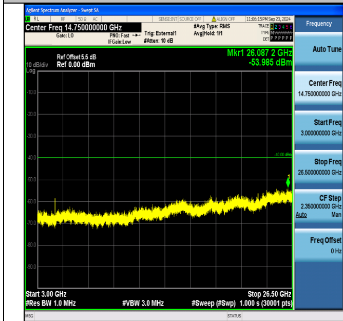
Band40_5MHz_16QAM_38750_25RB#0_3000~26500_3000~26500
