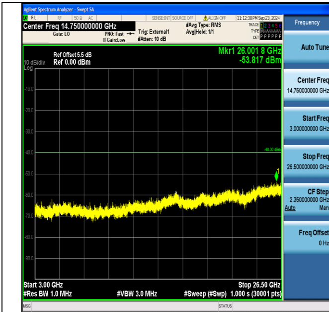
Band40_5MHz_QPSK_38775_25RB#0_3000~26500_3000~26500
