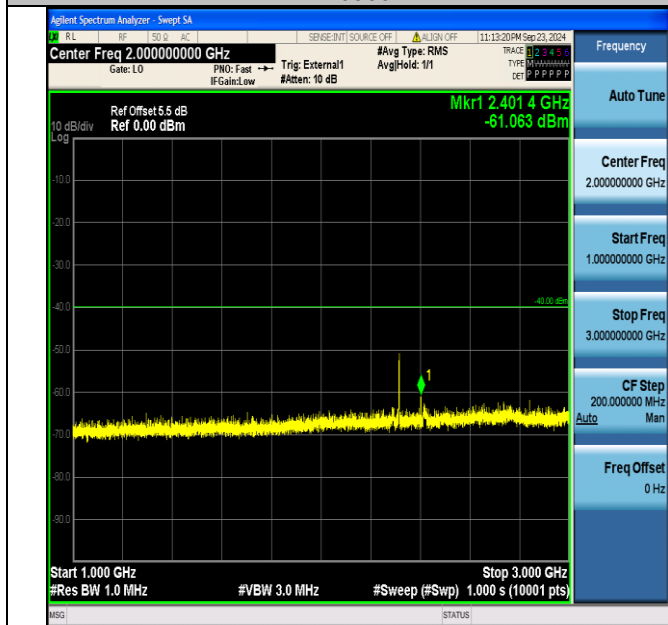
Band40_5MHz_16QAM_38775_25RB#0_1000~3000_1000~3000
