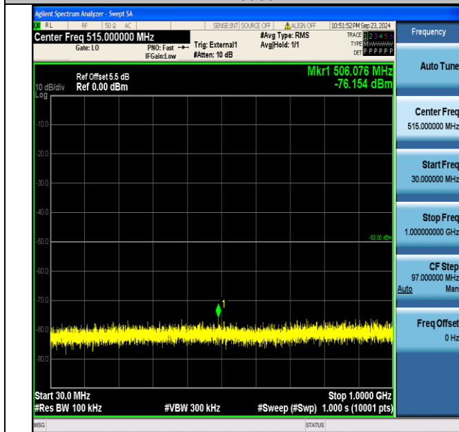
Band40_5MHz_QPSK_38725_1RB#0_30~1000_30~1000
