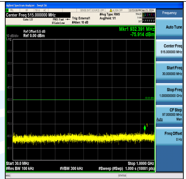
Band40_5MHz_16QAM_38725_1RB#0_30~1000_30~1000
