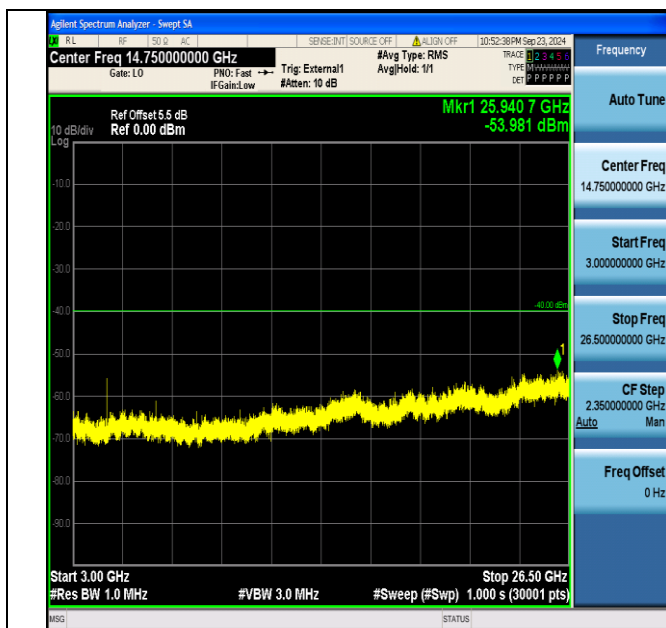
Band40_5MHz_QPSK_38725_1RB#0_3000~26500_3000~26500
