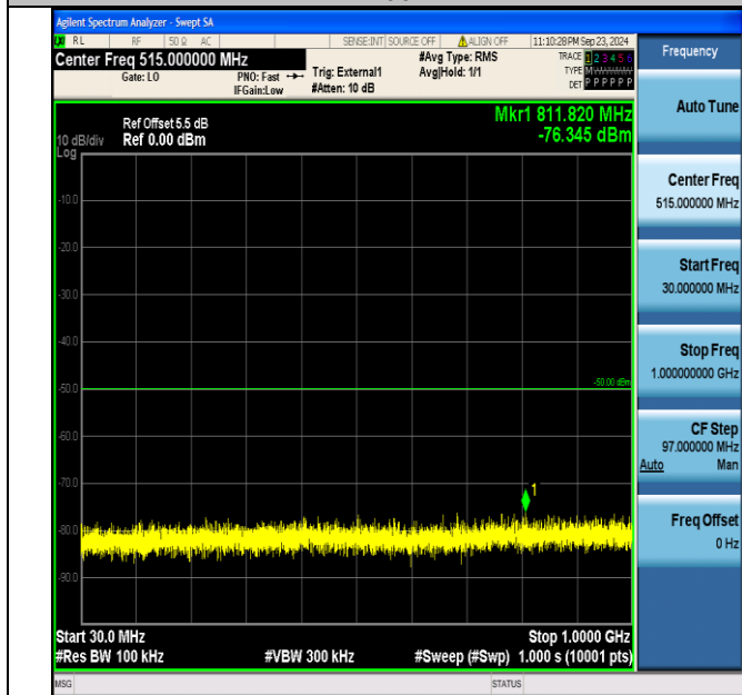
Band40_5MHz_16QAM_38775_1RB#24_30~1000_30~1000
