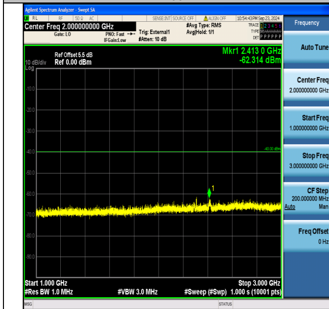
Band40_5MHz_QPSK_38725_1RB#24_1000~3000_1000~3000
