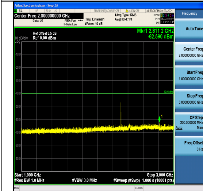
Band40_5MHz_16QAM_38725_1RB#0_1000~3000_1000~3000
