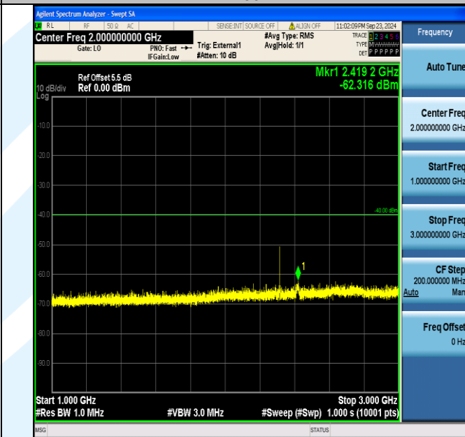
Band40_5MHz_QPSK_38750_1RB#24_1000~3000_1000~3000
