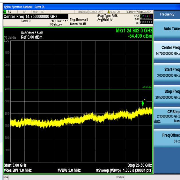
Band40_5MHz_16QAM_38725_25RB#0_3000~26500_3000~26500
