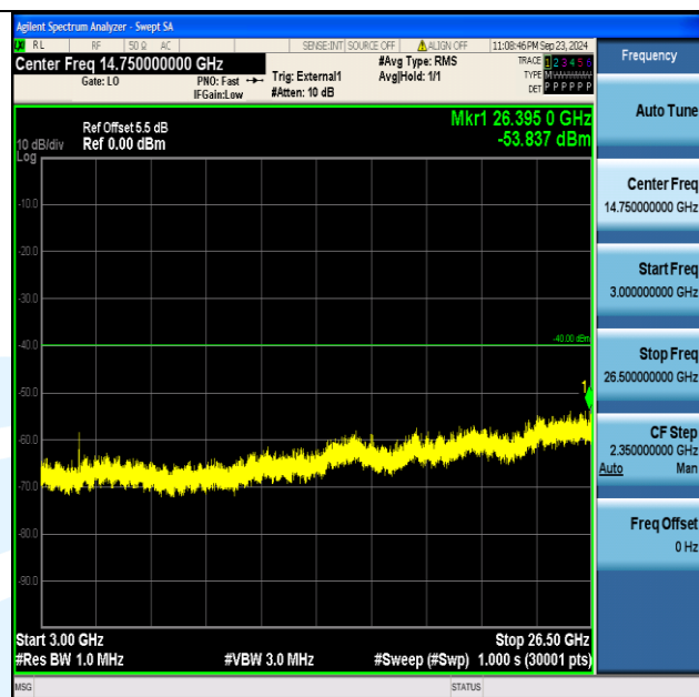
Band40_5MHz_16QAM_38775_1RB#0_3000~26500_3000~26500
