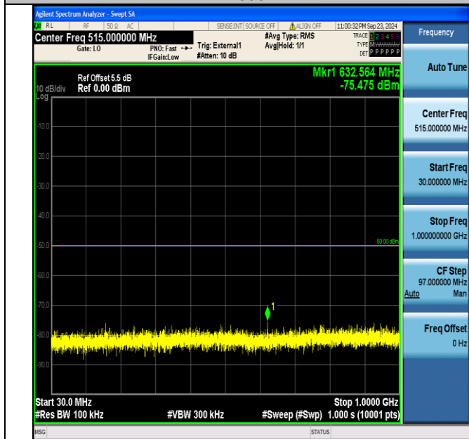
Band40_5MHz_16QAM_38750_1RB#0_30~1000_30~1000
