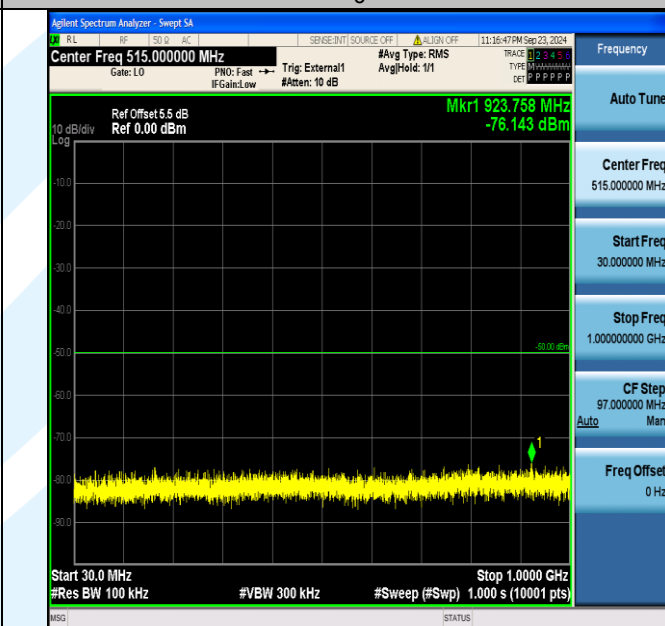
Band40_10MHz_QPSK_38750_1RB#49_30~1000_30~1000
