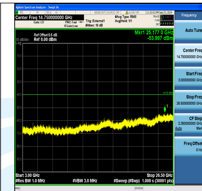
Band40_5MHz_QPSK_38775_1RB#24_3000~26500_3000~26500
