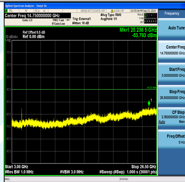
Band40_5MHz_QPSK_38725_1RB#24_3000~26500_3000~26500
