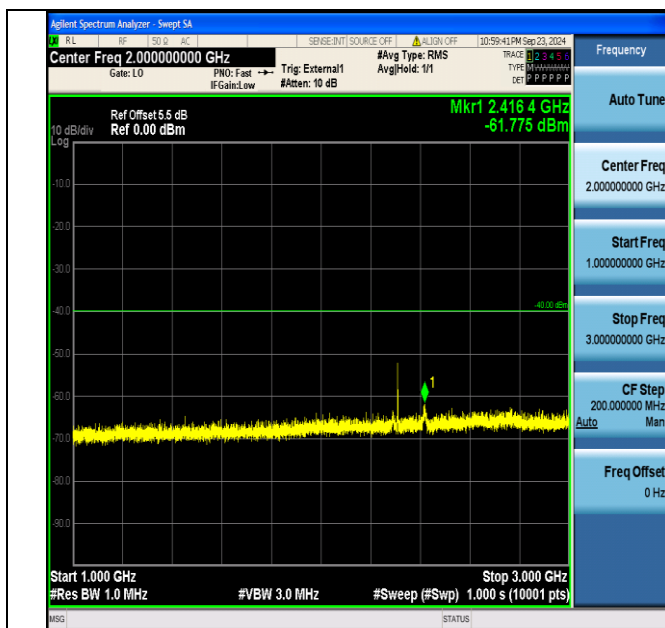
Band40_5MHz_QPSK_38750_1RB#0_1000~3000_1000~3000
