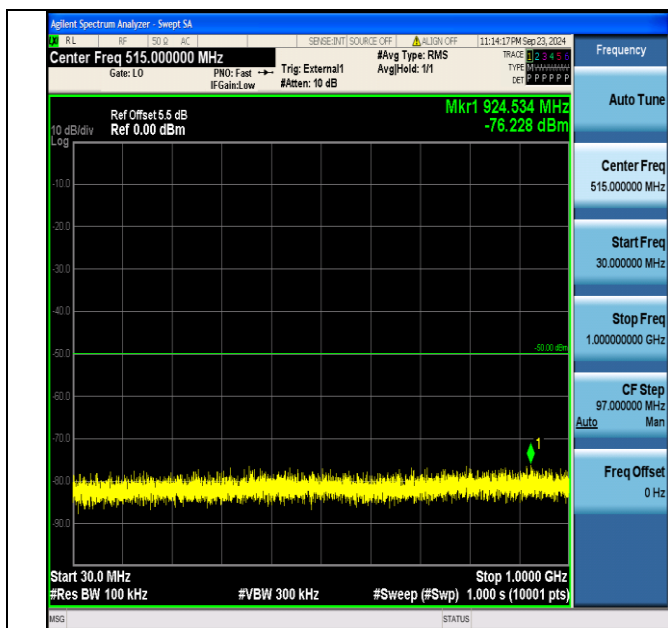
Band40_10MHz_QPSK_38750_1RB#0_30~1000_30~1000
