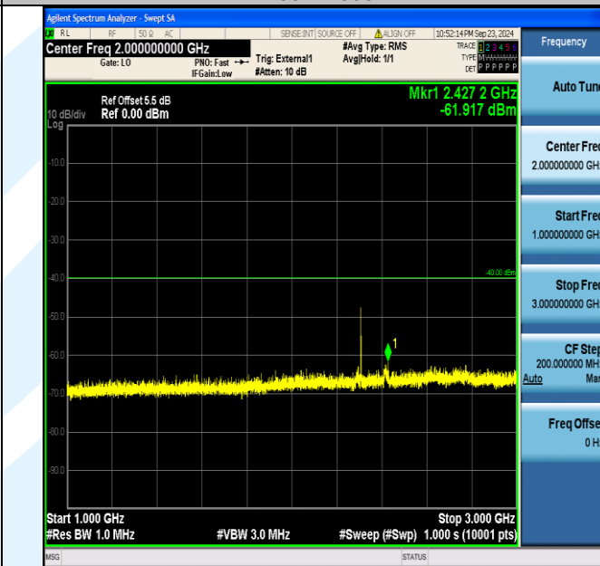
Band40_5MHz_QPSK_38725_1RB#0_1000~3000_1000~3000
