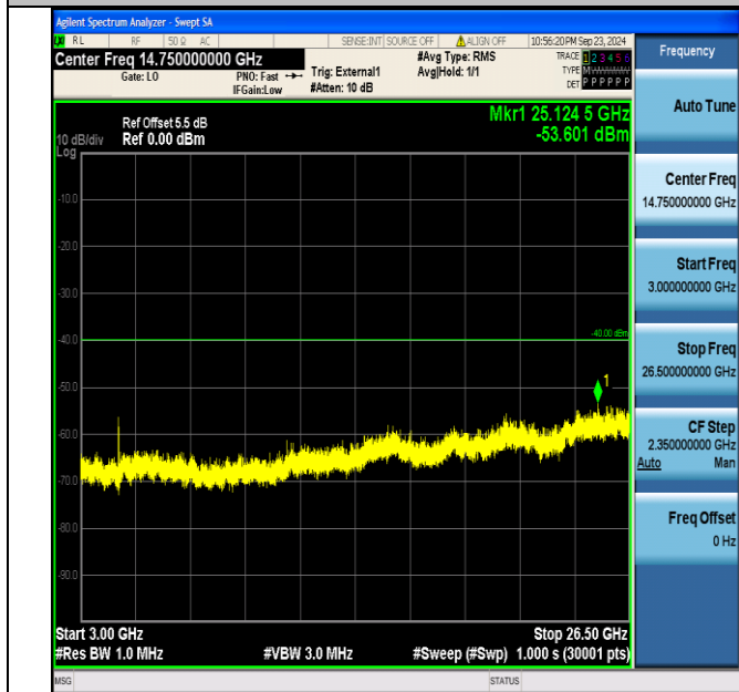
Band40_5MHz_16QAM_38725_1RB#24_3000~26500_3000~26500
