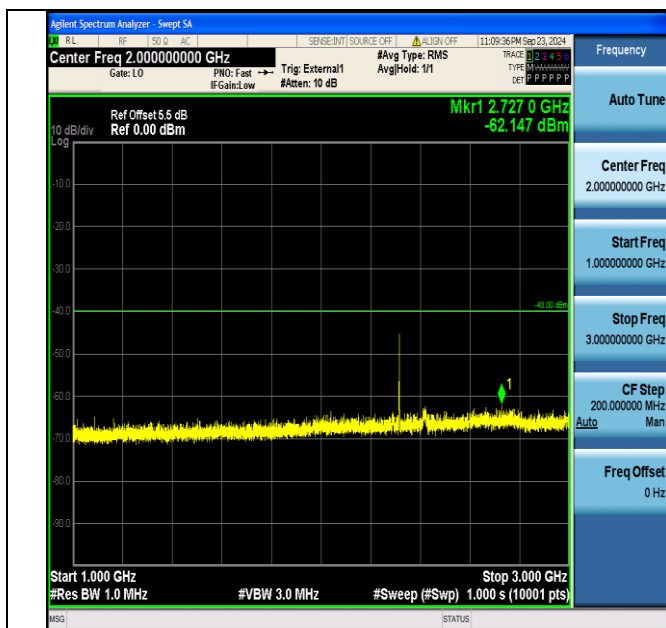
Band40_5MHz_QPSK_38775_1RB#24_1000~3000_1000~3000
