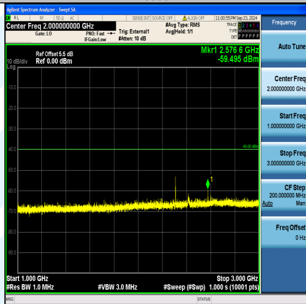
Band40_5MHz_16QAM_38750_1RB#0_1000~3000_1000~3000
