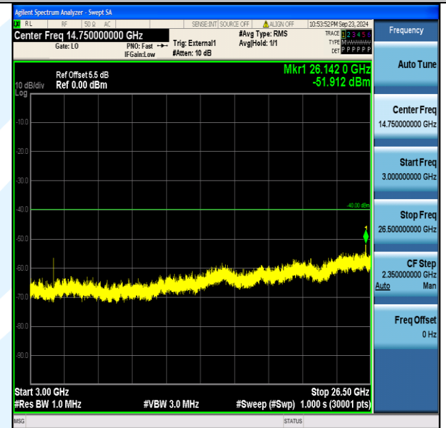
Band40_5MHz_16QAM_38725_1RB#0_3000~26500_3000~26500
