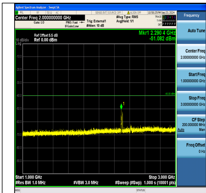
Band40_5MHz_16QAM_38725_25RB#0_1000~3000_1000~3000
