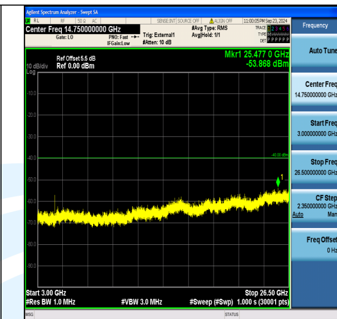
Band40_5MHz_QPSK_38750_1RB#0_3000~26500_3000~26500
