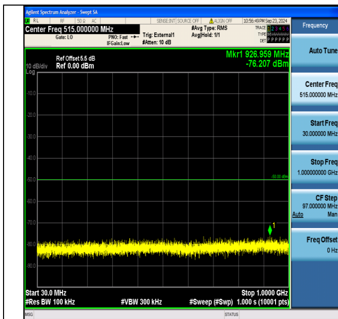
Band40_5MHz_QPSK_38725_25RB#0_30~1000_30~1000
