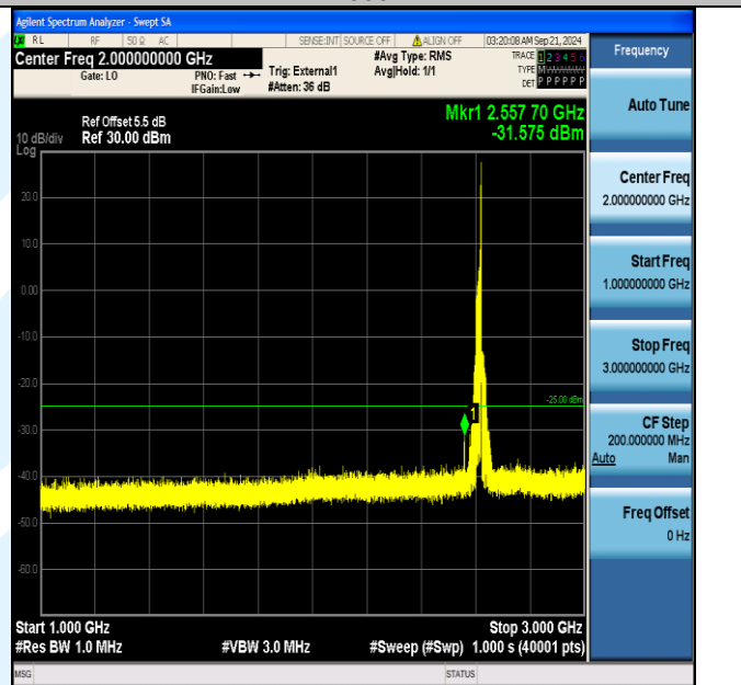
Band38_20MHz_QPSK_38150_1RB#99_1000~3000_1000~3000
