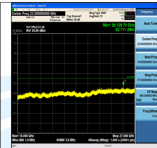
Band38_20MHz_16QAM_37850_1RB#0_18000~27000_18000~27000
