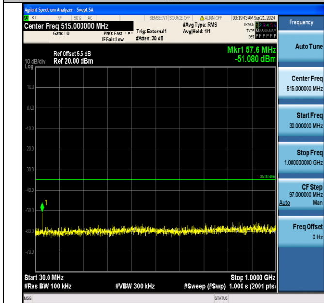
Band38_20MHz_QPSK_38150_1RB#99_30~1000_30~1000
