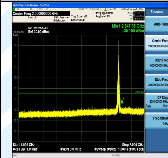
Band38_20MHz_16QAM_38000_1RB#0_1000~3000_1000~3000
