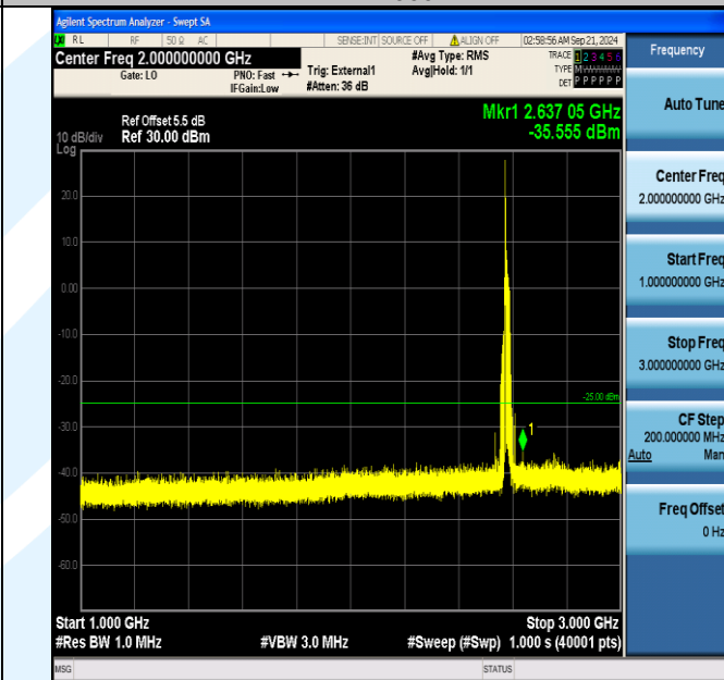
Band38_20MHz_16QAM_37850_1RB#0_1000~3000_1000~3000
