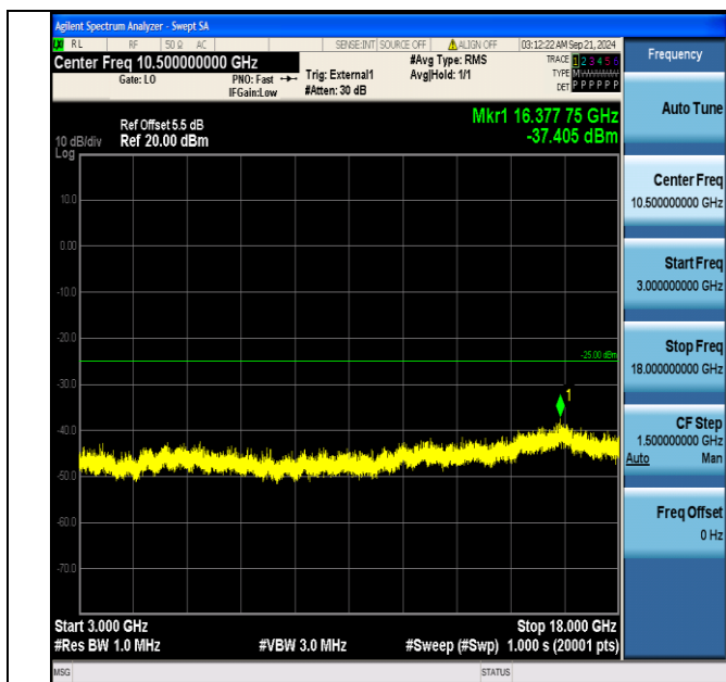
Band38_20MHz_16QAM_38000_1RB#99_3000~18000_3000~18000
