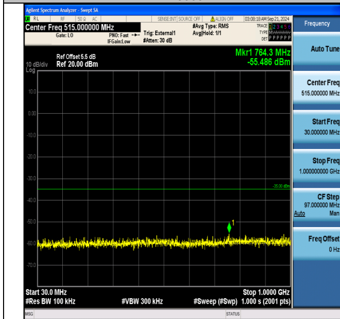
Band38_20MHz_16QAM_38000_1RB#0_30~1000_30~1000
