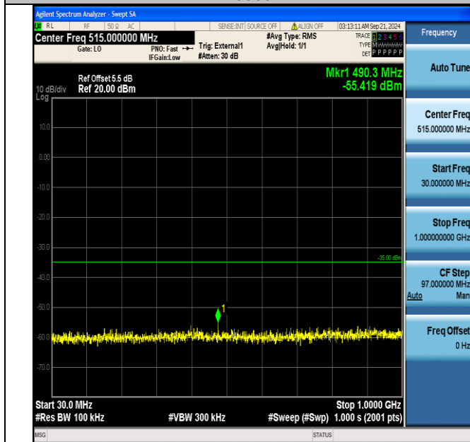
Band38_20MHz_QPSK_38000_100RB#0_30~1000_30~1000
