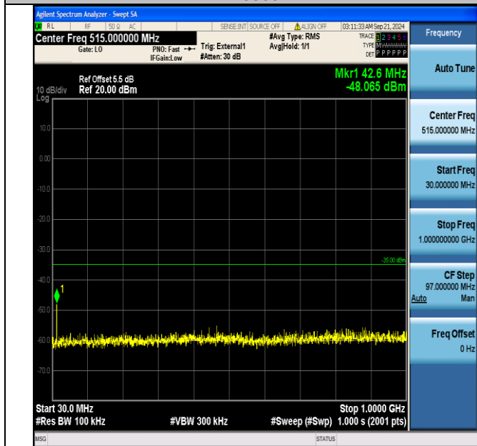
Band38_20MHz_16QAM_38000_1RB#99_30~1000_30~1000
