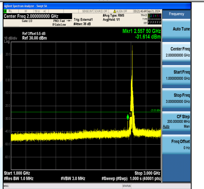
Band38_20MHz_16QAM_38150_1RB#99_1000~3000_1000~3000
