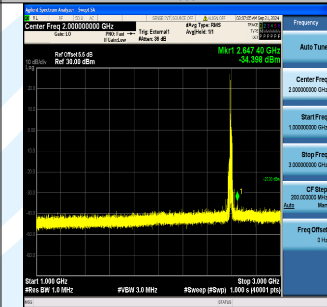
Band38_20MHz_QPSK_38000_1RB#0_1000~3000_1000~3000 0
