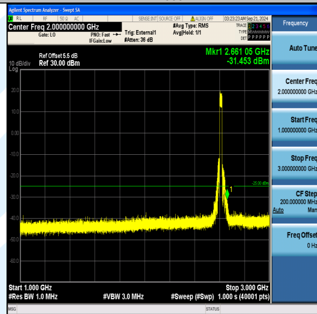
Band38_20MHz_QPSK_38150_100RB#0_1000~3000_1000~3000
