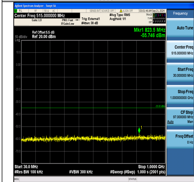
Band38_20MHz_16QAM_37850_1RB#99_30~1000_30~1000
