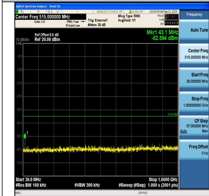
Band38_20MHz_QPSK_38000_1RB#99_30~1000_30~1000
