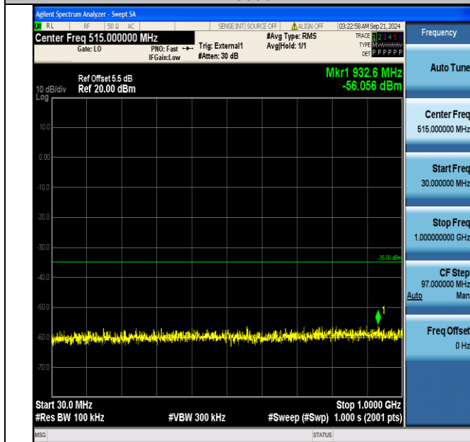
Band38_20MHz_QPSK_38150_100RB#0_30~1000_30~1000
