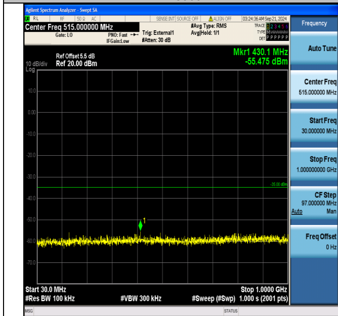
Band38_20MHz_16QAM_38150_100RB#0_30~1000_30~1000
