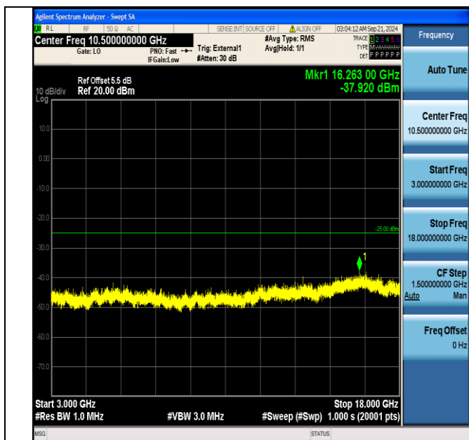
Band38_20MHz_QPSK_37850_100RB#0_3000~18000_3000~18000
