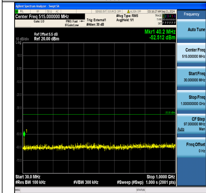
Band38_20MHz_QPSK_38150_1RB#0_30~1000_30~1000
