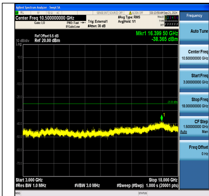
Band38_20MHz_QPSK_38000_100RB#0_3000~18000_3000~18000
