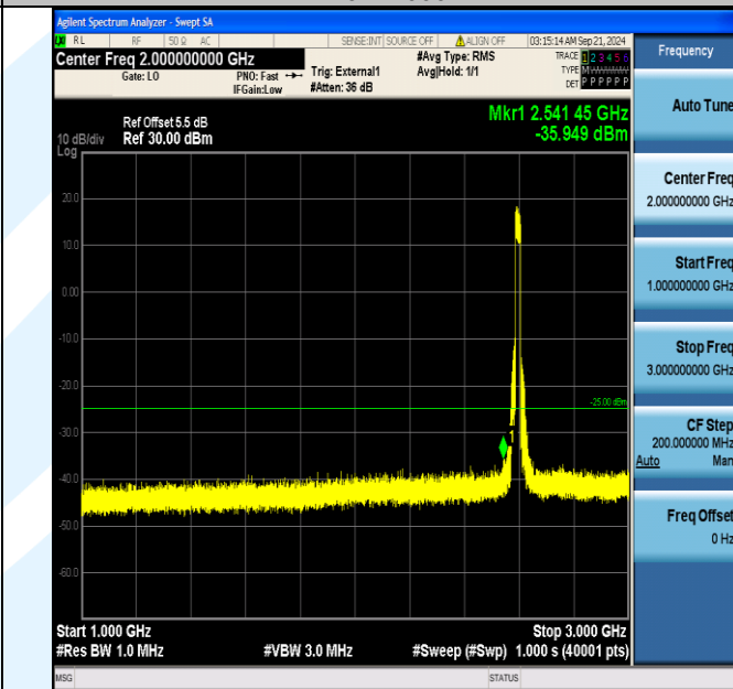
Band38_20MHz_16QAM_38000_100RB#0_1000~3000_1000~3000
