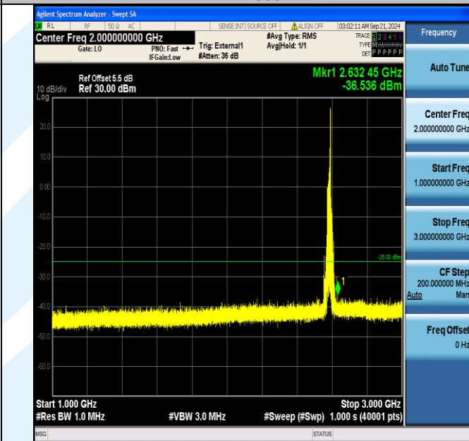
Band38_20MHz_16QAM_37850_1RB#99_1000~3000_1000~3000
