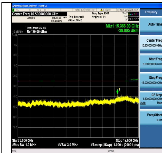
Band38_20MHz_QPSK_38150_1RB#99_3000~18000_3000~18000
