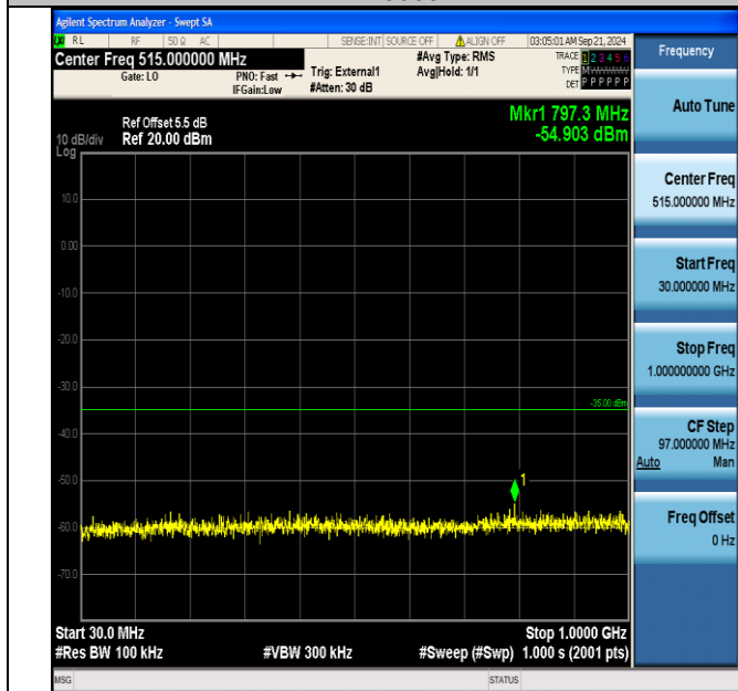
Band38_20MHz_16QAM_37850_100RB#0_30~1000_30~1000
