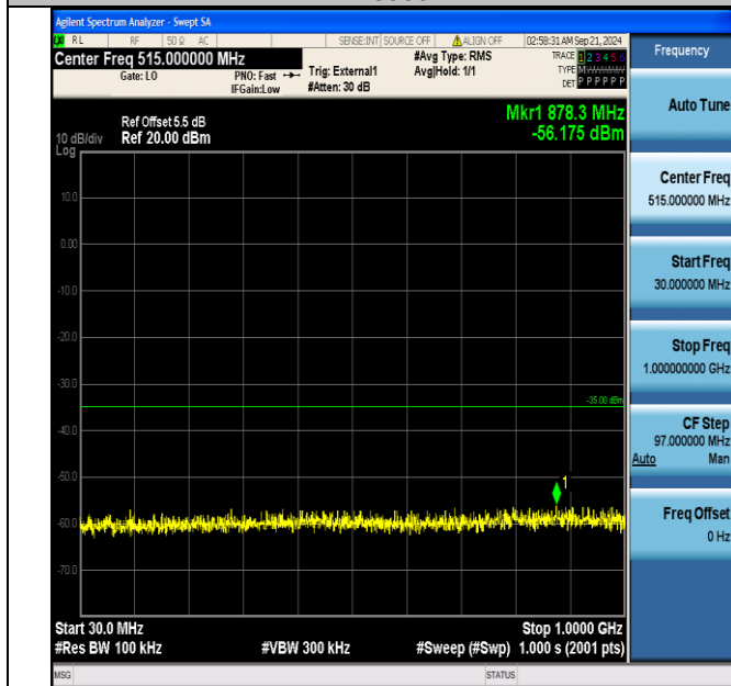
Band38_20MHz_16QAM_37850_1RB#0_30~1000_30~1000
