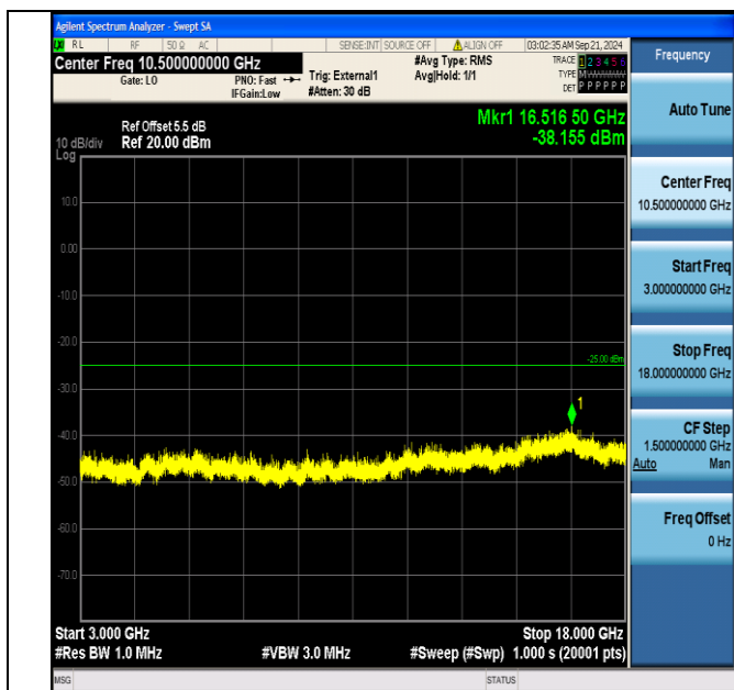
Band38_20MHz_16QAM_37850_1RB#99_3000~18000_3000~18000
