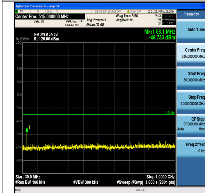
Band38_20MHz_16QAM_38150_1RB#99_30~1000_30~1000
