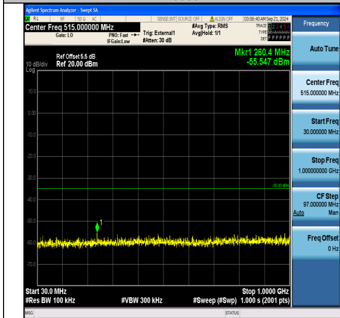
Band38_20MHz_QPSK_38000_1RB#0_30~1000_30~1000
