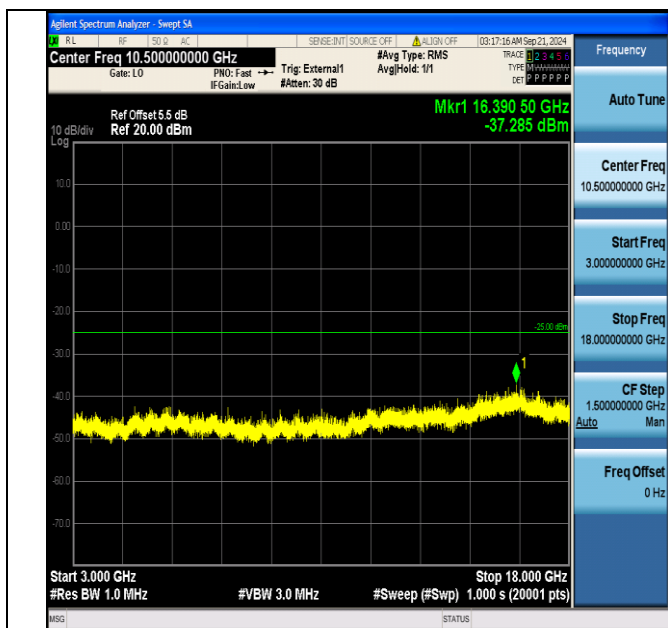
Band38_20MHz_QPSK_38150_1RB#0_3000~18000_3000~18000
