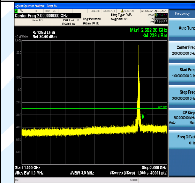
Band38_20MHz_QPSK_38150_1RB#0_1000~3000_1000~3000 0
