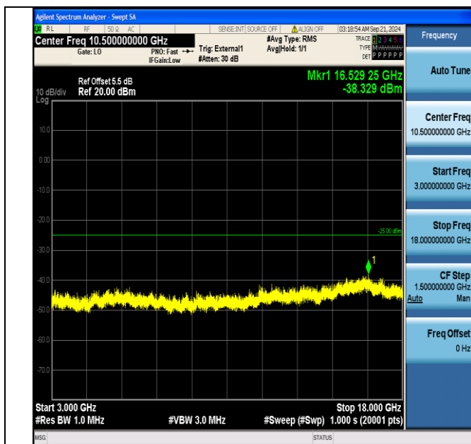
Band38_20MHz_16QAM_38150_1RB#0_3000~18000_3000~18000
