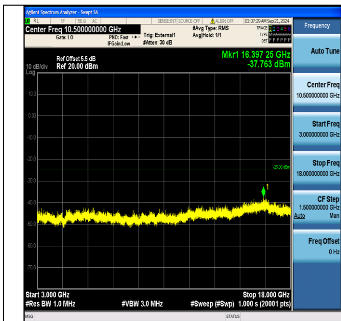
Band38_20MHz_QPSK_38000_1RB#0_3000~18000_3000~18000
