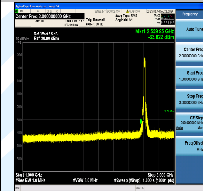
Band38_20MHz_16QAM_38150_100RB#0_1000~3000_1000~3000
