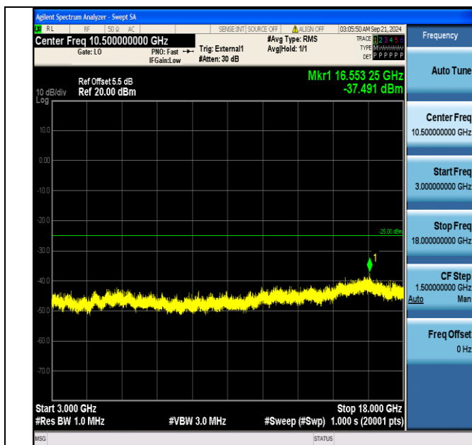
Band38_20MHz_16QAM_37850_100RB#0_3000~18000_3000~18000
