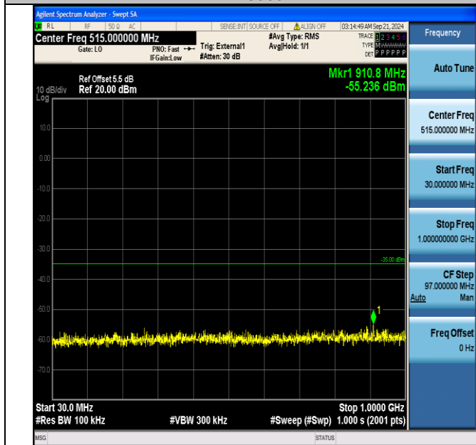
Band38_20MHz_16QAM_38000_100RB#0_30~1000_30~1000
