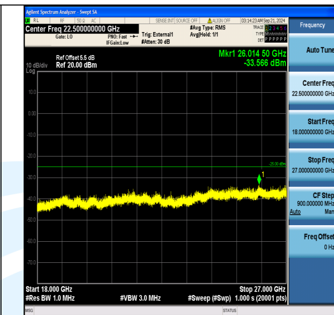
Band38_20MHz_QPSK_38000_100RB#0_18000~27000_18000~27000
