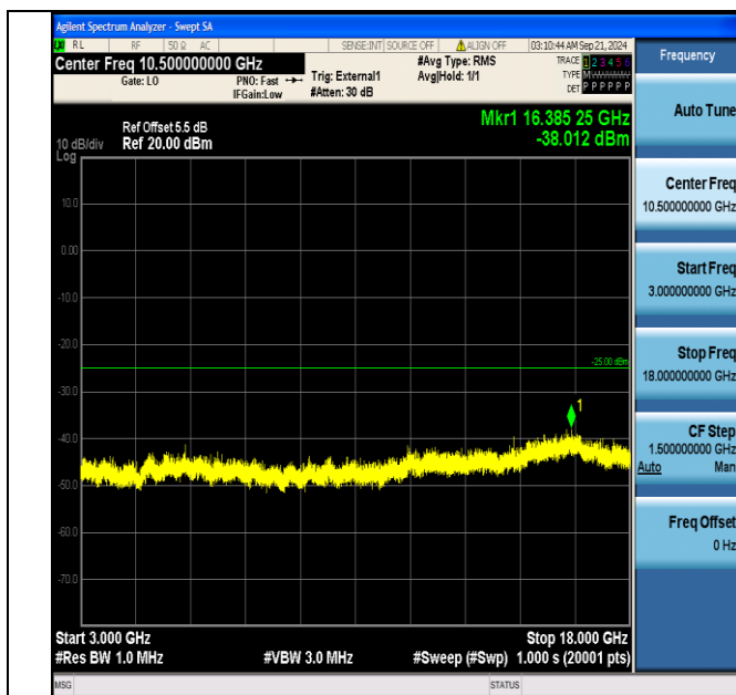
Band38_20MHz_QPSK_38000_1RB#99_3000~18000_3000~18000
