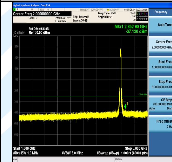
Band38_20MHz_16QAM_37850_100RB#0_1000~3000_1000~3000
