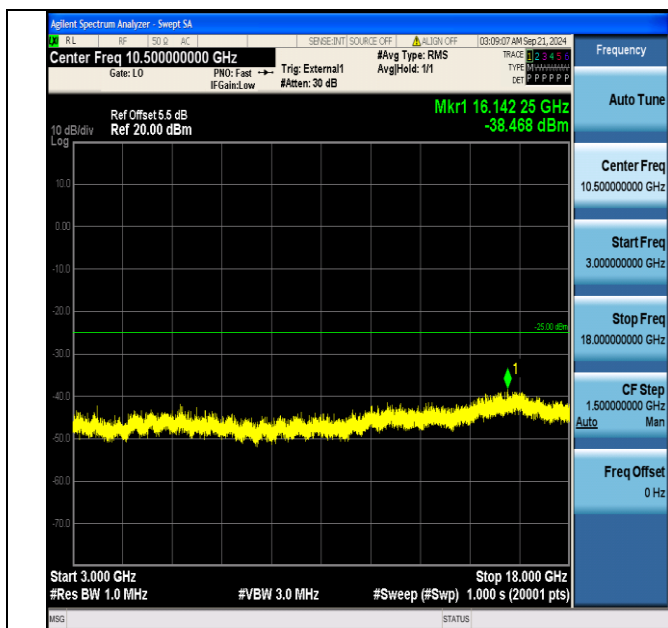
Band38_20MHz_16QAM_38000_1RB#0_3000~18000_3000~18000
