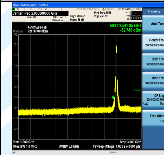
Band38_20MHz_QPSK_38000_100RB#0_1000~3000_1000~3000
