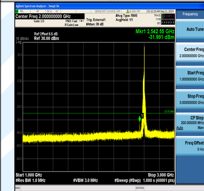
Band38_20MHz_QPSK_38000_1RB#99_1000~3000_1000~3000
