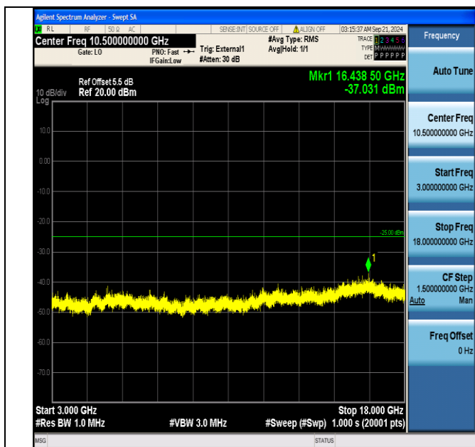
Band38_20MHz_16QAM_38000_100RB#0_3000~18000_3000~18000
