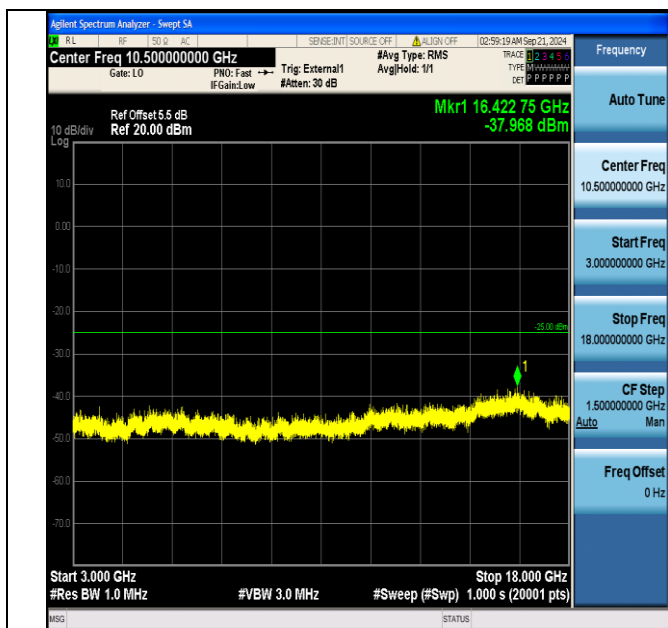
Band38_20MHz_16QAM_37850_1RB#0_3000~18000_3000~18000
