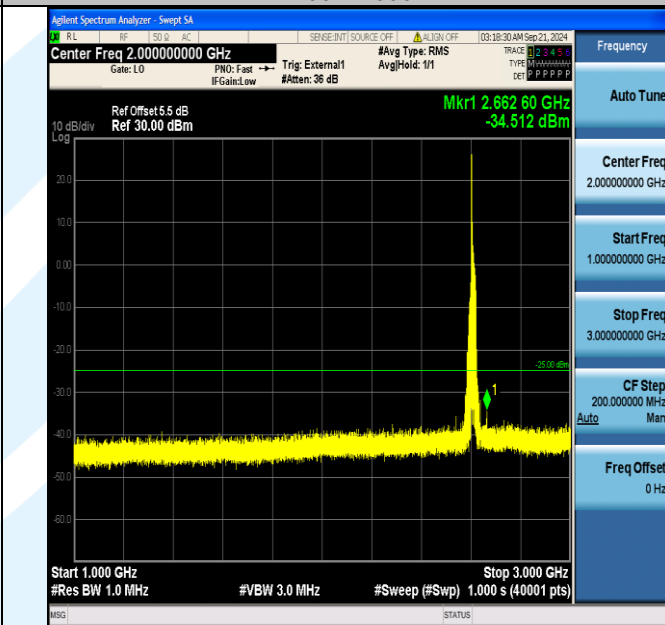
Band38_20MHz_16QAM_38150_1RB#0_1000~3000_1000~3000
