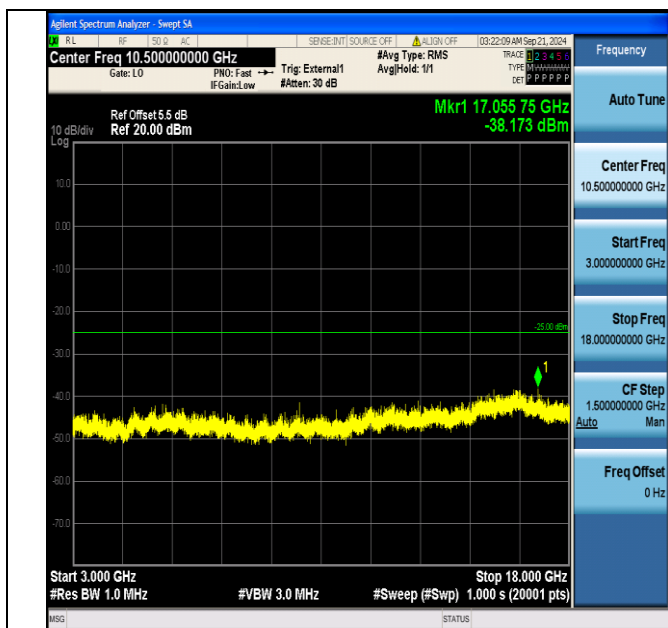
Band38_20MHz_16QAM_38150_1RB#99_3000~18000_3000~18000
