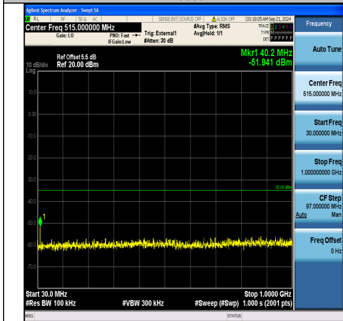
Band38_20MHz_16QAM_38150_1RB#0_30~1000_30~1000
