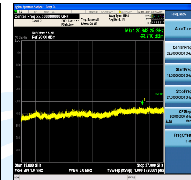
Band38_20MHz_16QAM_37850_100RB#0_18000~27000_18000~27000
