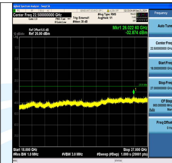
Band38_15MHz_16QAM_37825_1RB#74_18000~27000_18000~27000
