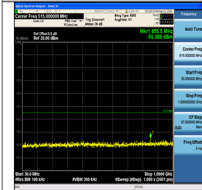
Band38_15MHz_16QAM_37825_1RB#0_30~1000_30~1000
