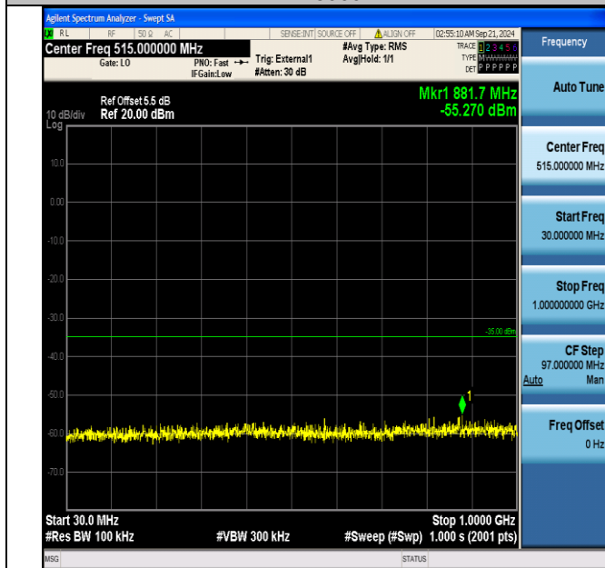
Band38_15MHz_16QAM_38175_75RB#0_30~1000_30~1000
