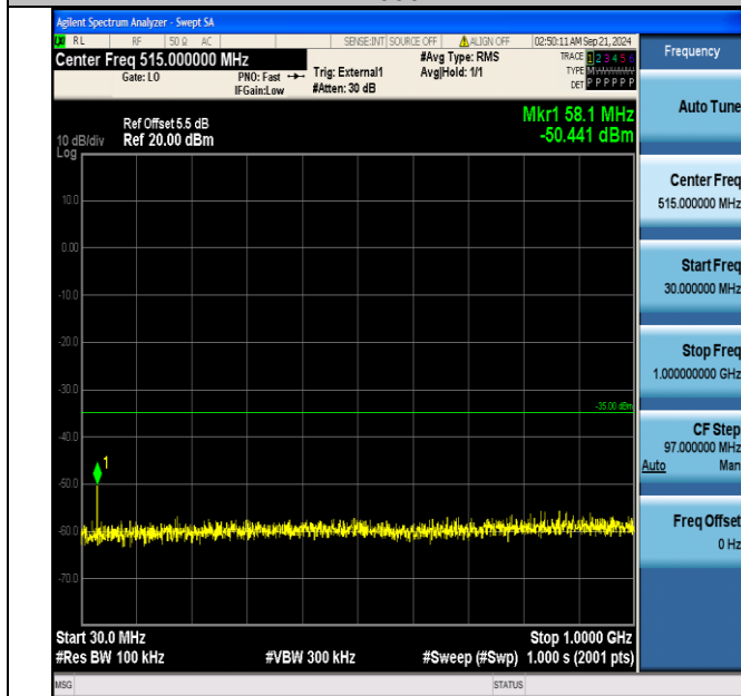
Band38_15MHz_QPSK_38175_1RB#74_30~1000_30~1000
