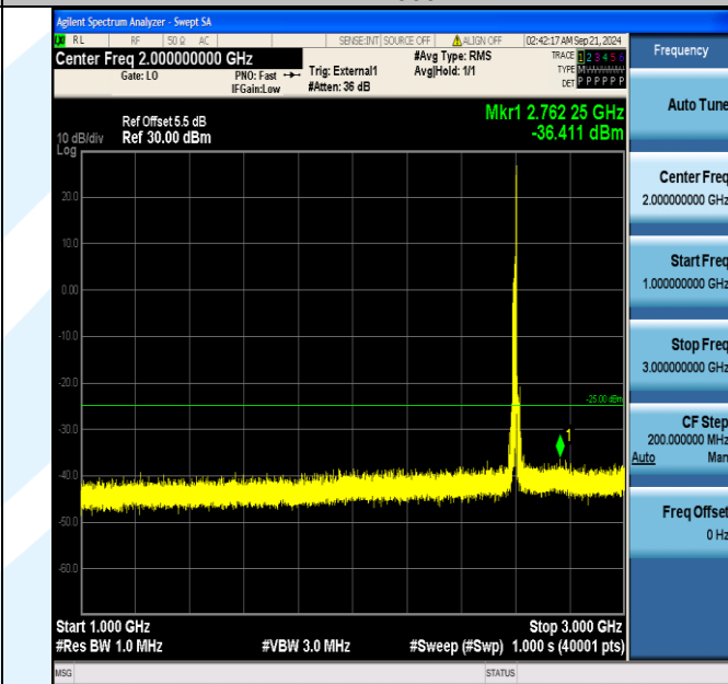
Band38_15MHz_16QAM_38000_1RB#74_1000~3000_1000~3000
