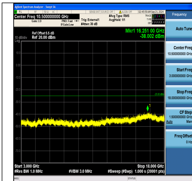
Band38_15MHz_16QAM_38000_75RB#0_3000~18000_3000~18000
