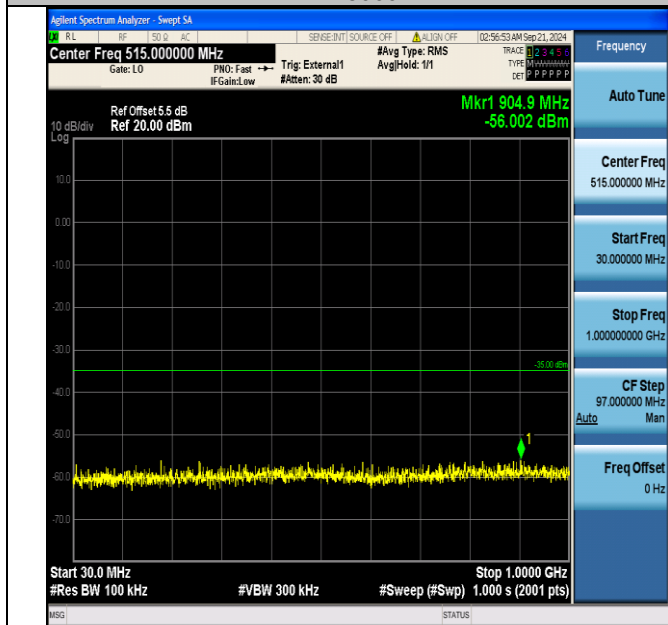
Band38_20MHz_QPSK_37850_1RB#0_30~1000_30~1000
