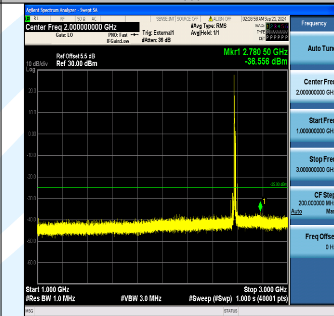
Band38_15MHz_16QAM_37825_1RB#0_1000~3000_1000~3000
