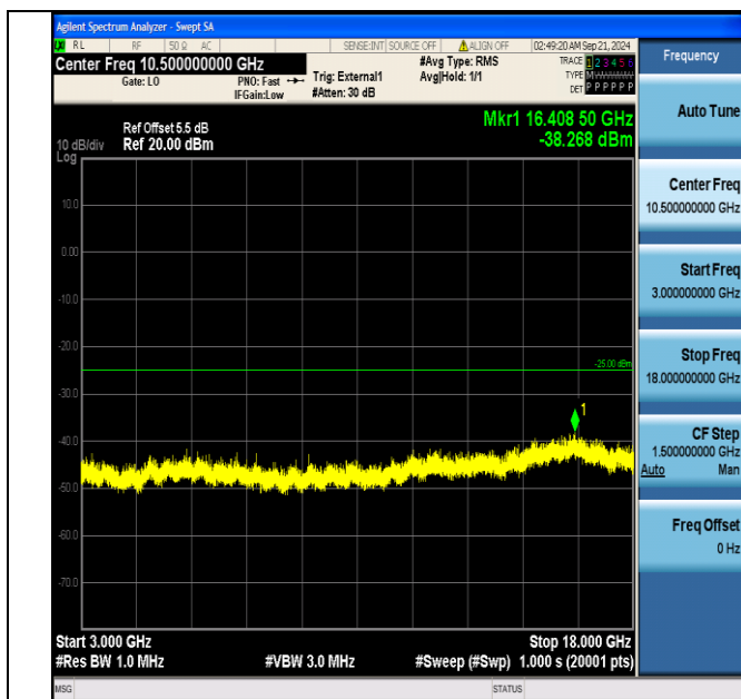
Band38_15MHz_16QAM_38175_1RB#0_3000~18000_3000~18000
