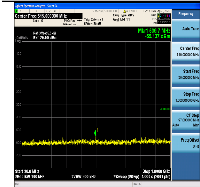
Band38_15MHz_QPSK_38175_75RB#0_30~1000_30~1000
