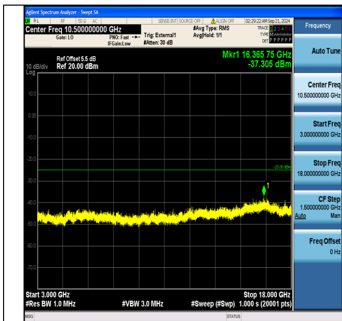
Band38_15MHz_16QAM_37825_1RB#0_3000~18000_3000~18000
