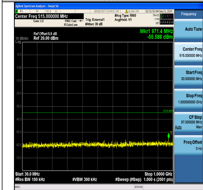
Band38_15MHz_16QAM_37825_1RB#74_30~1000_30~1000
