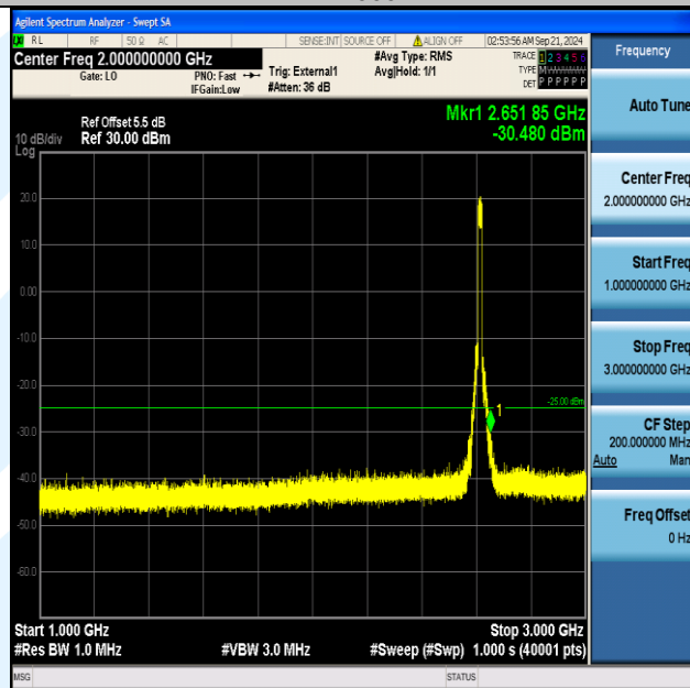
Band38_15MHz_QPSK_38175_75RB#0_1000~3000_1000~3000
