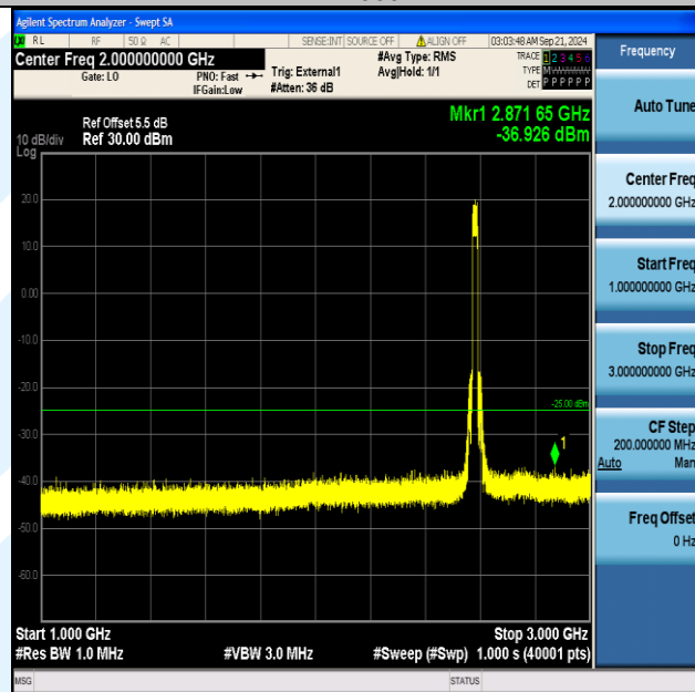
Band38_20MHz_QPSK_37850_100RB#0_1000~3000_1000~3000
