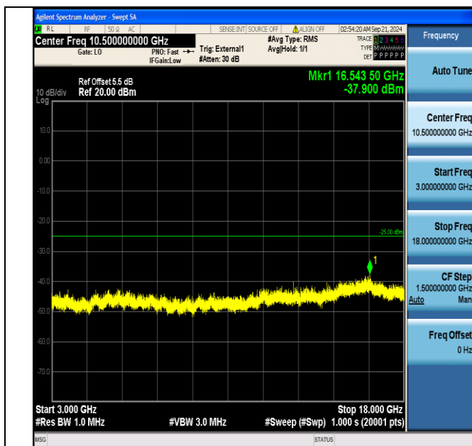
Band38_15MHz_QPSK_38175_75RB#0_3000~18000_3000~18000
