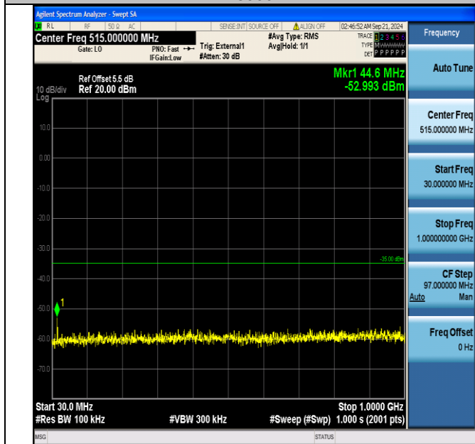
Band38_15MHz_QPSK_38175_1RB#0_30~1000_30~1000
