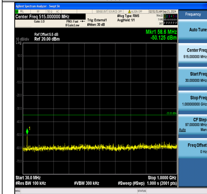
Band38_15MHz_16QAM_38175_1RB#74_30~1000_30~1000
