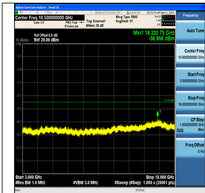
Band38_15MHz_16QAM_37825_1RB#74_3000~18000_3000~18000
