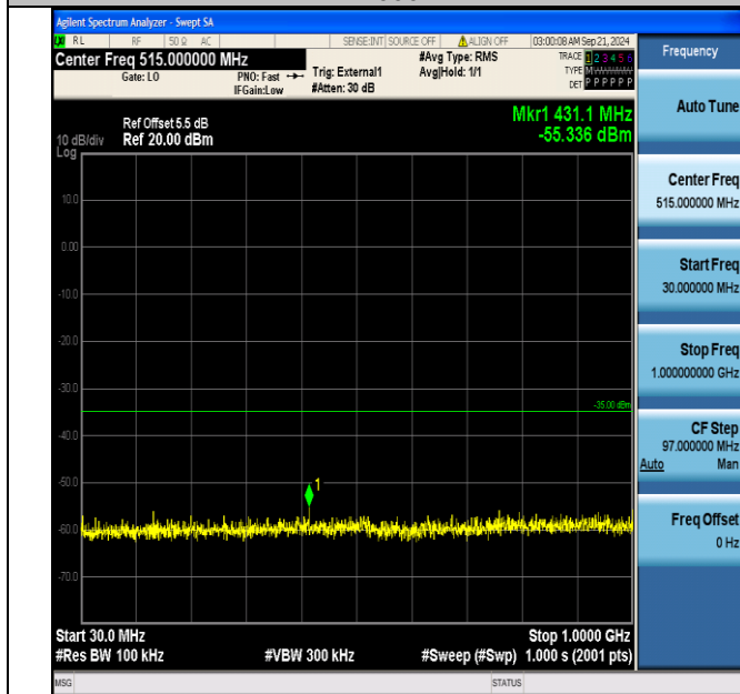
Band38_20MHz_QPSK_37850_1RB#99_30~1000_30~1000
