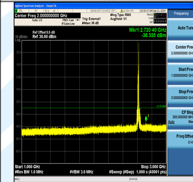
Band38_15MHz_QPSK_38175_1RB#74_1000~3000_1000~3000
