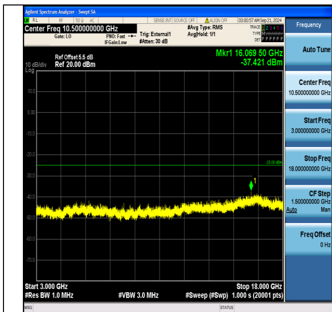
Band38_20MHz_QPSK_37850_1RB#99_3000~18000_3000~18000
