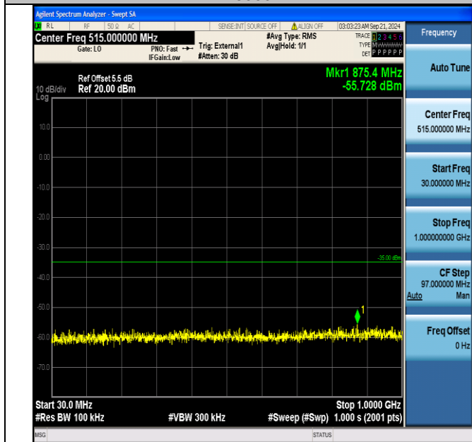
Band38_20MHz_QPSK_37850_100RB#0_30~1000_30~1000
