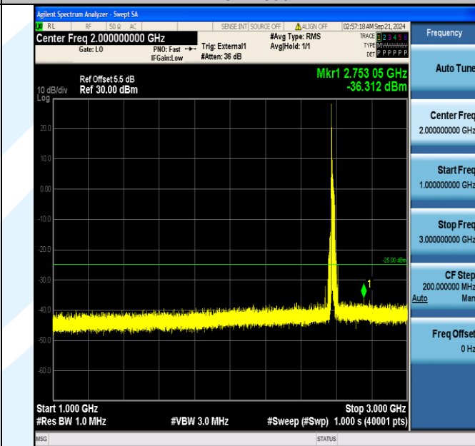
Band38_20MHz_QPSK_37850_1RB#0_1000~3000_1000~3000
