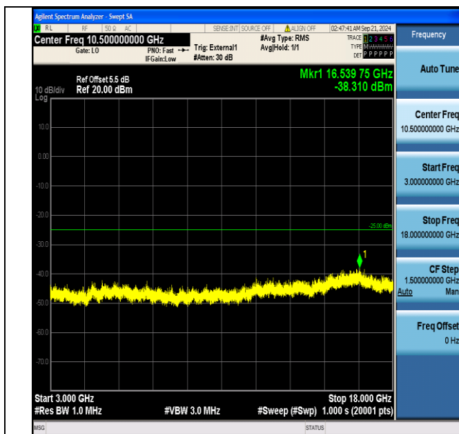
Band38_15MHz_QPSK_38175_1RB#0_3000~18000_3000~18000
