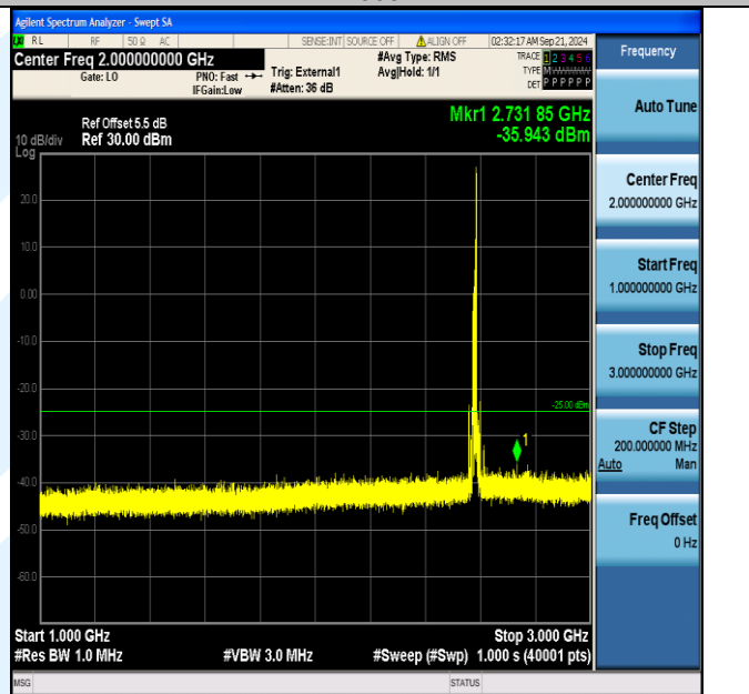
Band38_15MHz_16QAM_37825_1RB#74_1000~3000_1000~3000
