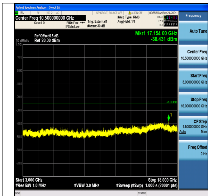
Band38_15MHz_16QAM_38175_75RB#0_3000~18000_3000~18000
