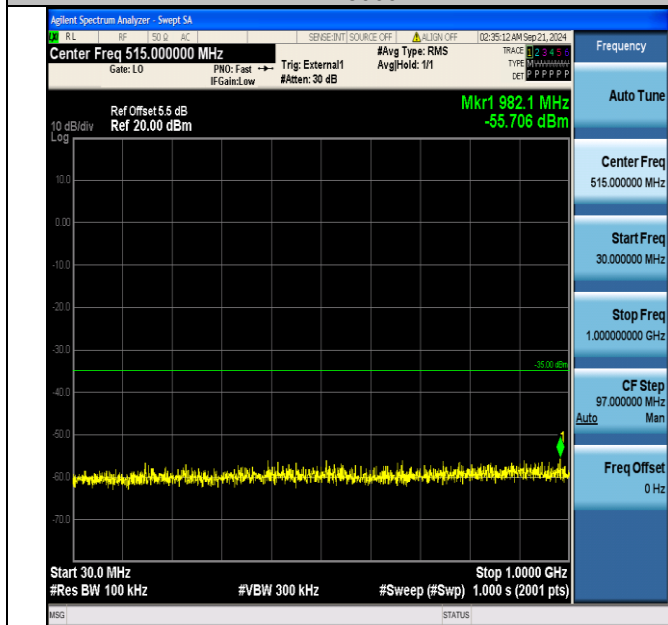
Band38_15MHz_16QAM_37825_75RB#0_30~1000_30~1000
