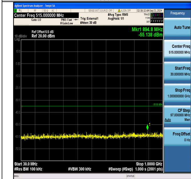
Band38_15MHz_16QAM_38000_1RB#0_30~1000_30~1000
