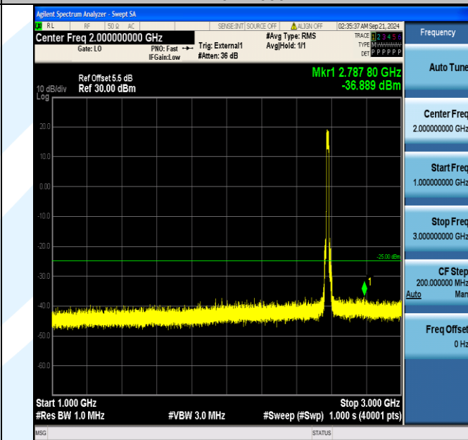
Band38_15MHz_16QAM_37825_75RB#0_1000~3000_1000~3000
