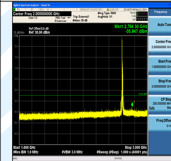
Band38_15MHz_16QAM_38175_1RB#0_1000~3000_1000~3000
