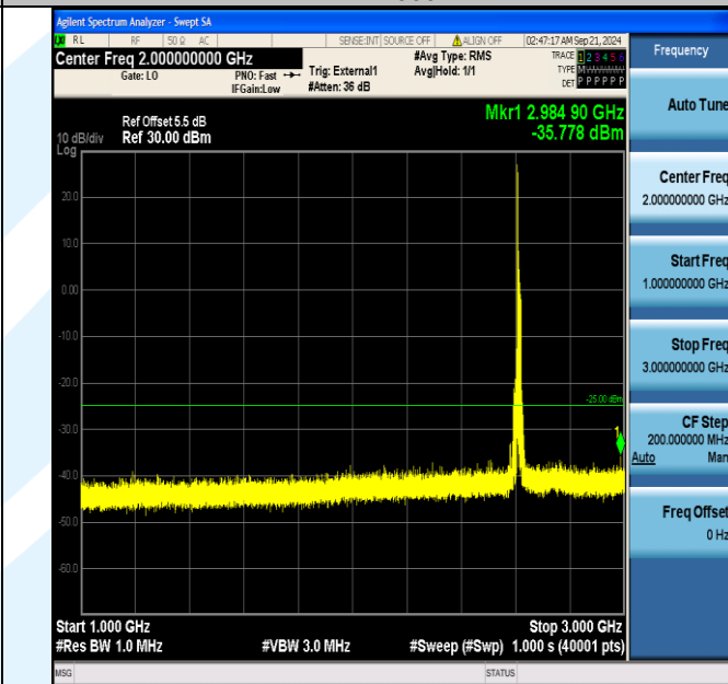
Band38_15MHz_QPSK_38175_1RB#0_1000~3000_1000~3000
