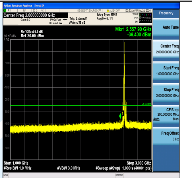
Band38_15MHz_16QAM_38175_1RB#74_1000~3000_1000~3000
