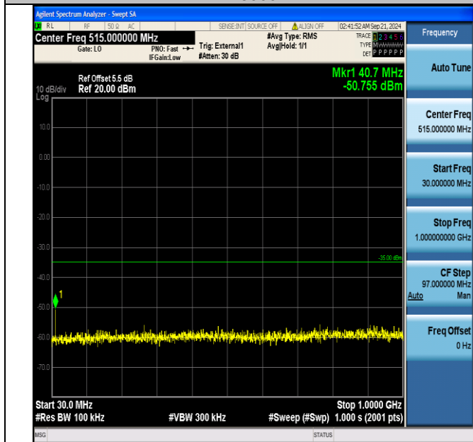
Band38_15MHz_16QAM_38000_1RB#74_30~1000_30~1000
