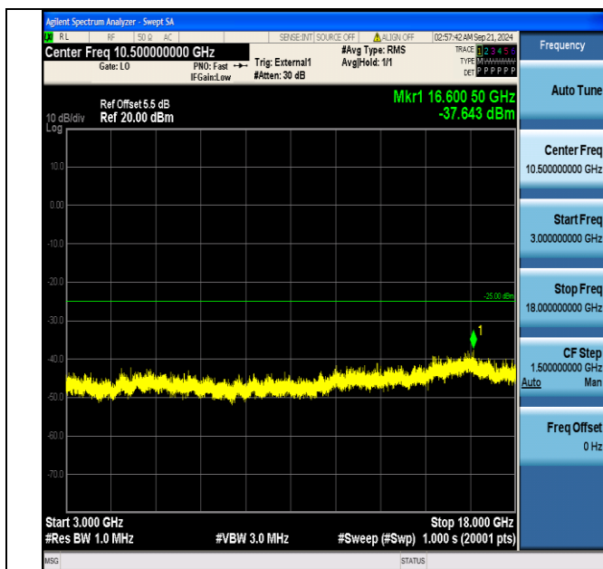
Band38_20MHz_QPSK_37850_1RB#0_3000~18000_3000~18000
