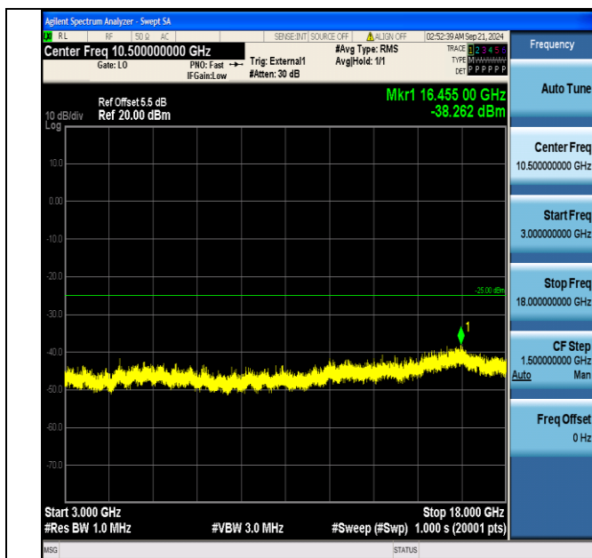
Band38_15MHz_16QAM_38175_1RB#74_3000~18000_3000~18000
