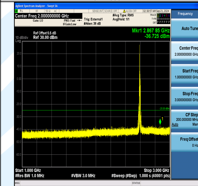
Band38_15MHz_16QAM_38000_1RB#0_1000~3000_1000~3000
