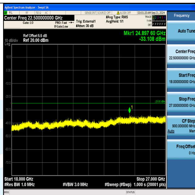
Band38_20MHz_QPSK_37850_1RB#99_18000~27000_18000~27000
