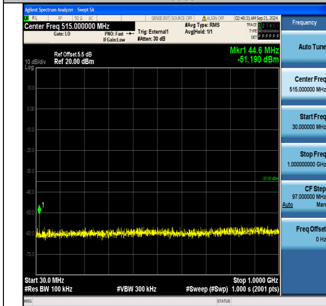
Band38_15MHz_16QAM_38175_1RB#0_30~1000_30~1000
