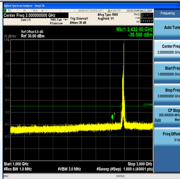
Band38_20MHz_QPSK_37850_1RB#99_1000~3000_1000~3000
