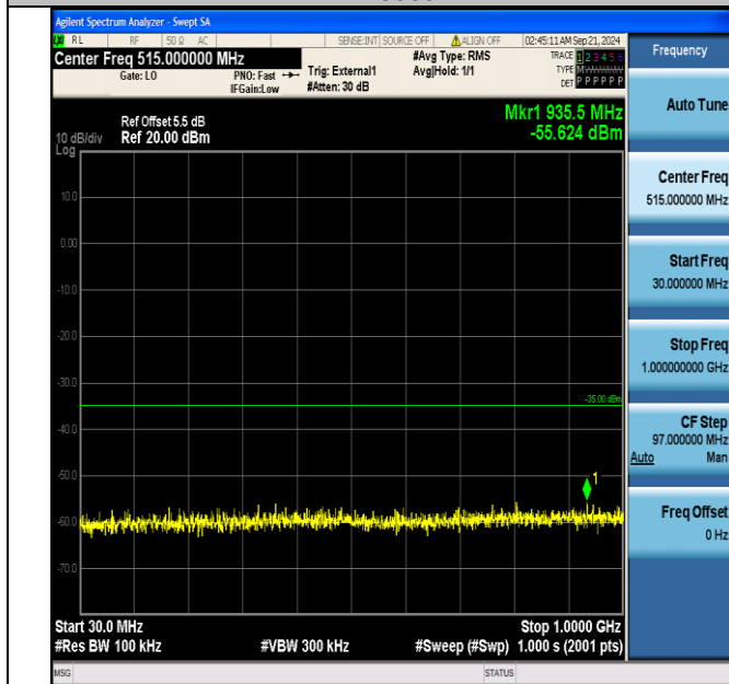
Band38_15MHz_16QAM_38000_75RB#0_30~1000_30~1000
