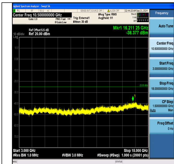
Band38_15MHz_QPSK_38000_75RB#0_3000~18000_3000~18000
