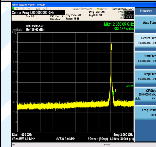
Band38_15MHz_16QAM_38175_75RB#0_1000~3000_1000~3000
