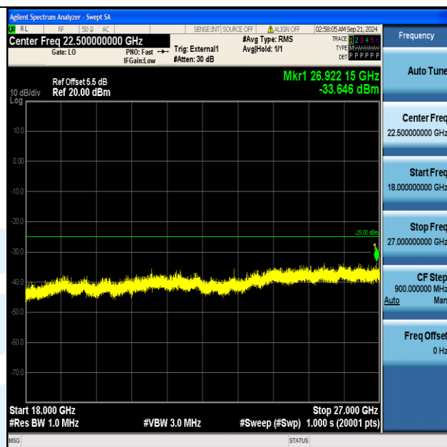
Band38_20MHz_QPSK_37850_1RB#0_18000~27000_18000~27000
