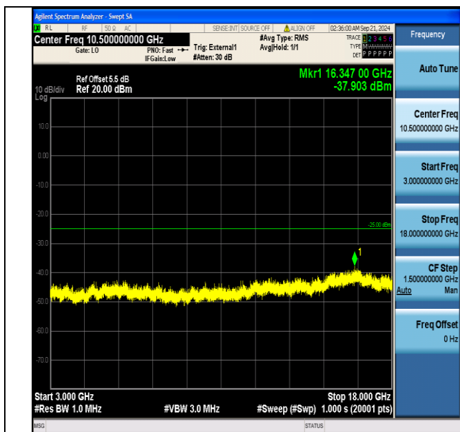
Band38_15MHz_16QAM_37825_75RB#0_3000~18000_3000~18000
