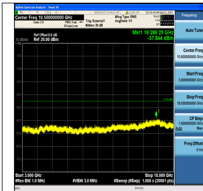
Band38_15MHz_16QAM_38000_1RB#74_3000~18000_3000~18000
