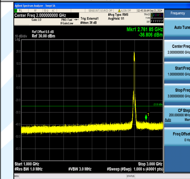
Band38_15MHz_16QAM_38000_75RB#0_1000~3000_1000~3000
