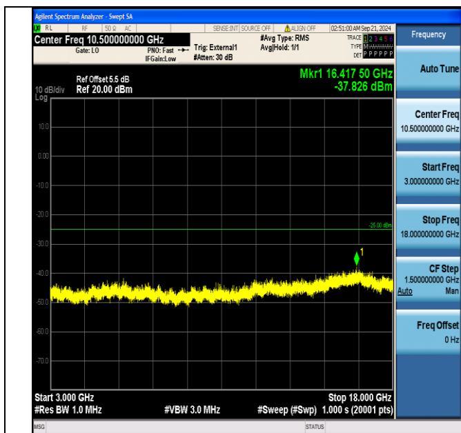
Band38_15MHz_QPSK_38175_1RB#74_3000~18000_3000~18000
