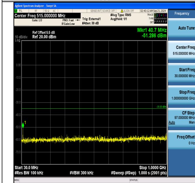
Band38_15MHz_QPSK_38000_1RB#74_30~1000_30~1000
