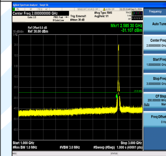
Band38_10MHz_16QAM_38200_50RB#0_1000~3000_1000~3000
