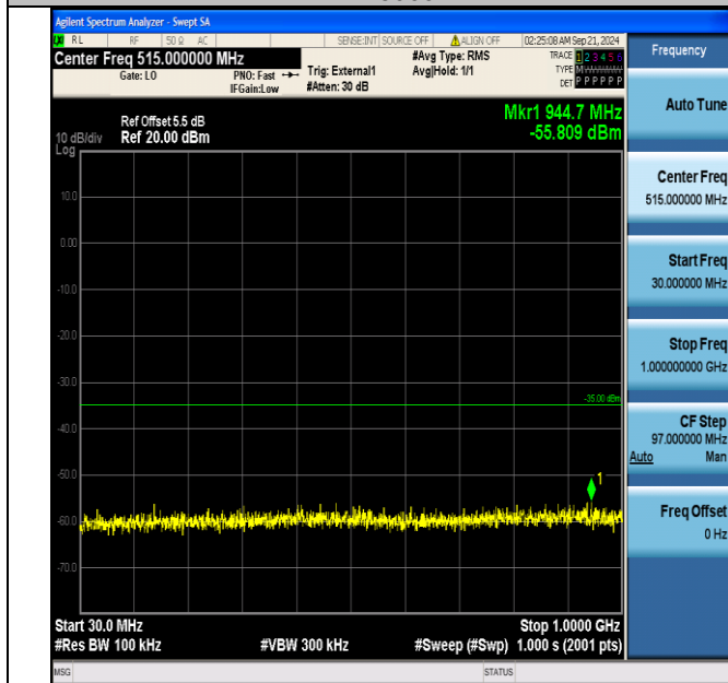
Band38_10MHz_16QAM_38200_50RB#0_30~1000_30~1000
