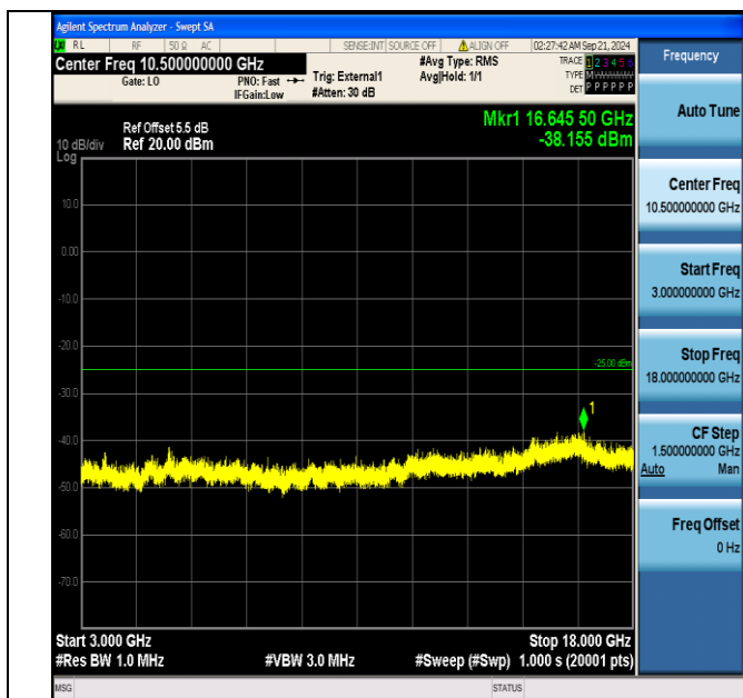
Band38_15MHz_QPSK_37825_1RB#0_3000~18000_3000~18000
