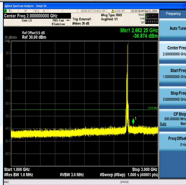
Band38_15MHz_QPSK_37825_1RB#74_1000~3000_1000~3000
