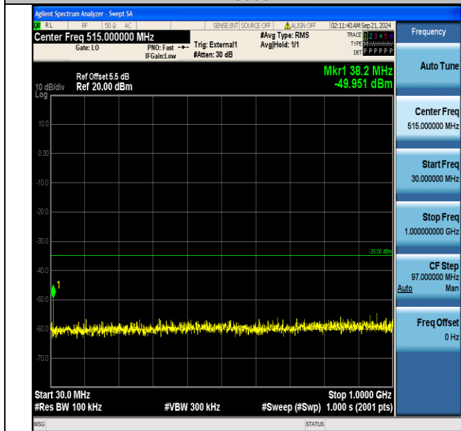
Band38_10MHz_16QAM_38000_1RB#49_30~1000_30~1000
