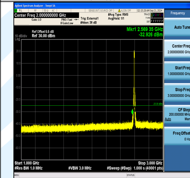
Band38_10MHz_16QAM_38000_50RB#0_1000~3000_1000~3000
