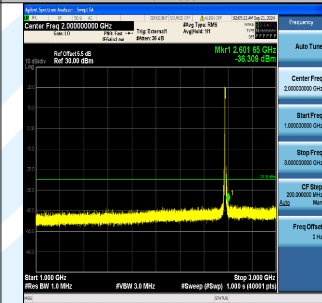
Band38_10MHz_16QAM_37800_50RB#0_1000~3000_1000~3000
