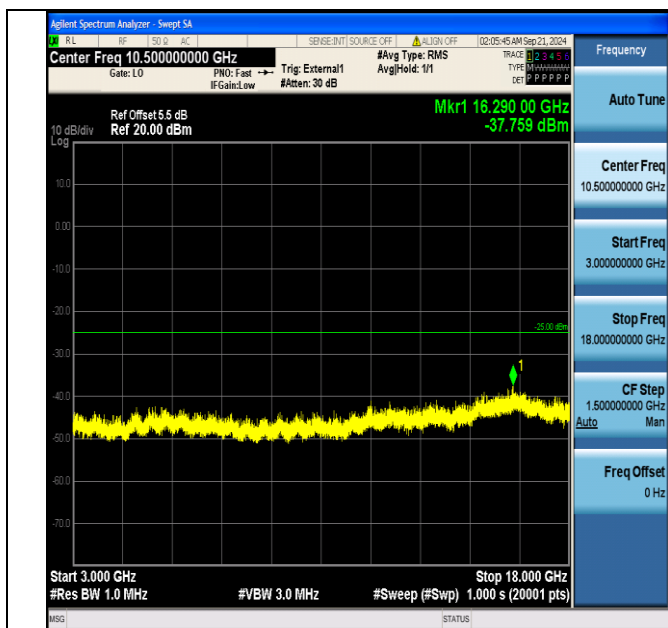
Band38_10MHz_16QAM_37800_50RB#0_3000~18000_3000~18000
