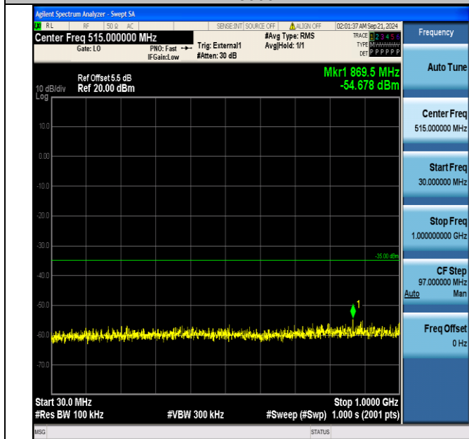
Band38_10MHz_16QAM_37800_1RB#49_30~1000_30~1000
