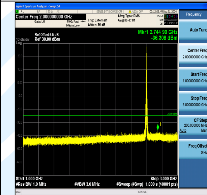
Band38_10MHz_16QAM_38000_1RB#49_1000~3000_1000~3000
