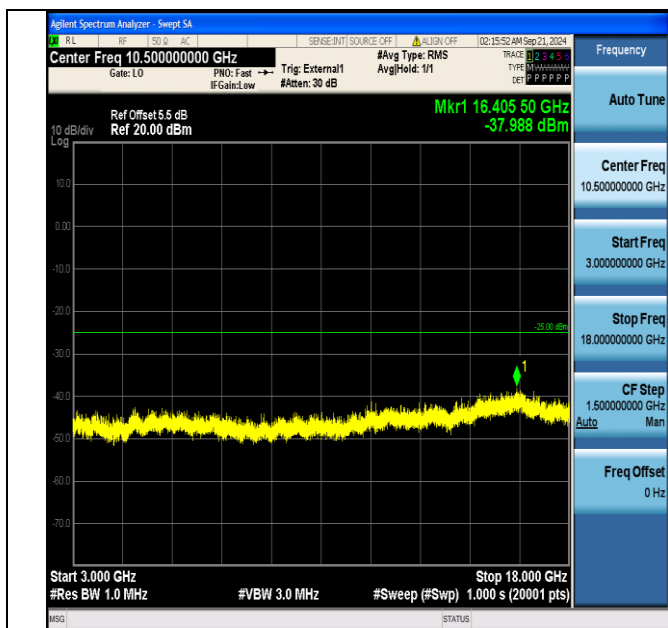
Band38_10MHz_16QAM_38000_50RB#0_3000~18000_3000~18000
