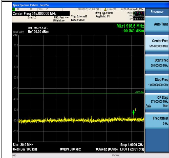
Band38_15MHz_QPSK_37825_1RB#74_30~1000_30~1000
