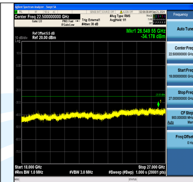
Band38_10MHz_16QAM_37800_50RB#0_18000~27000_18000~27000
