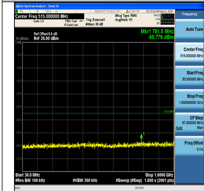
Band38_10MHz_16QAM_38000_50RB#0_30~1000_30~1000
