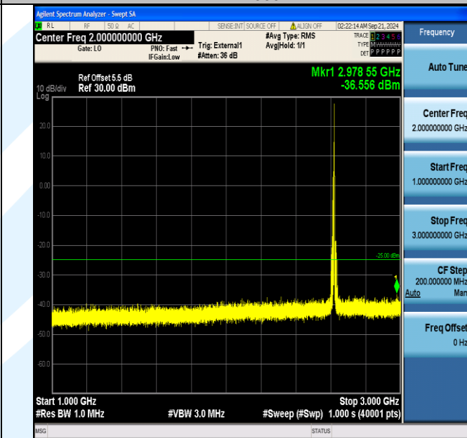
Band38_10MHz_16QAM_38200_1RB#49_1000~3000_1000~3000
