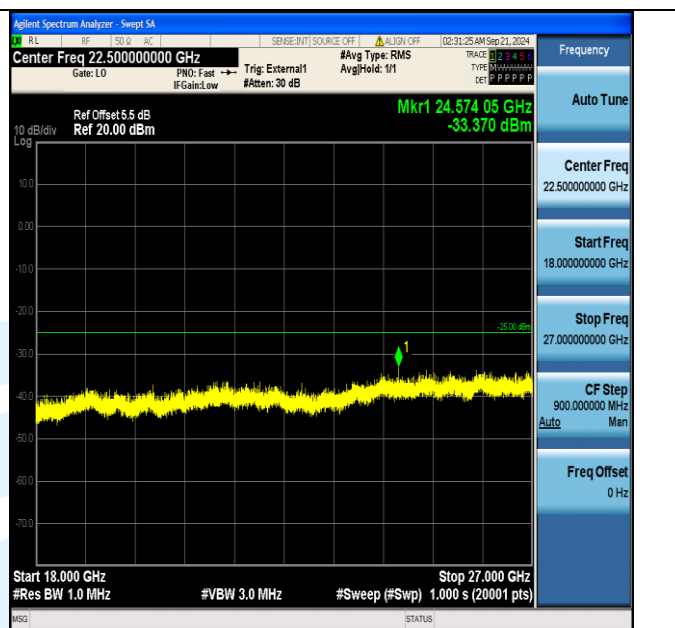
Band38_15MHz_QPSK_37825_1RB#74_18000~27000_18000~27000
