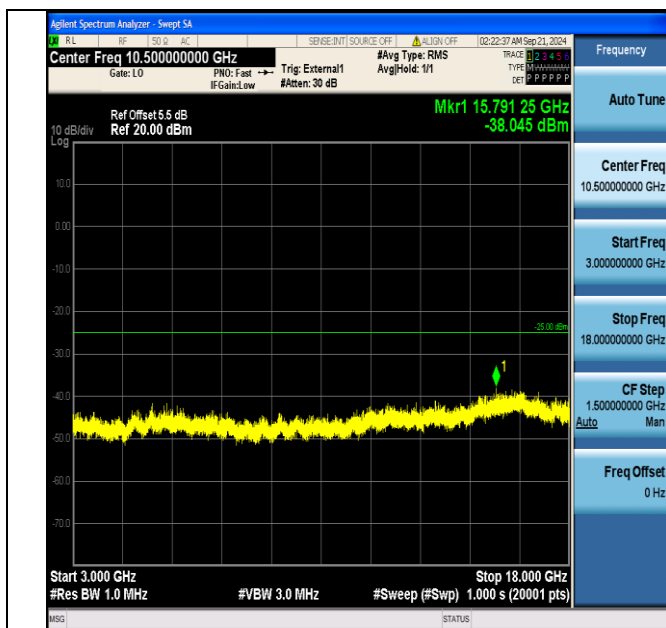
Band38_10MHz_16QAM_38200_1RB#49_3000~18000_3000~18000
