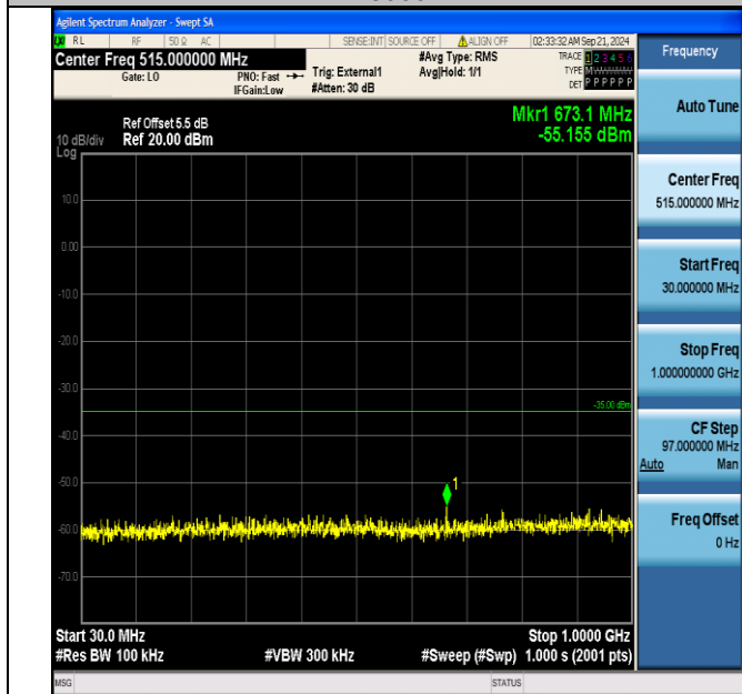
Band38_15MHz_QPSK_37825_75RB#0_30~1000_30~1000
