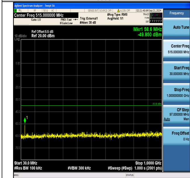
Band38_10MHz_16QAM_38200_1RB#49_30~1000_30~1000
