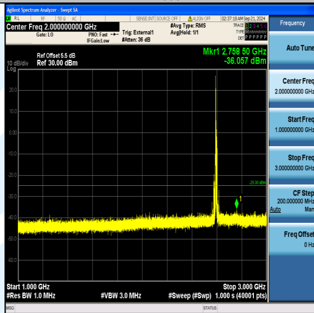
Band38_15MHz_QPSK_38000_1RB#0_1000~3000_1000~3000
