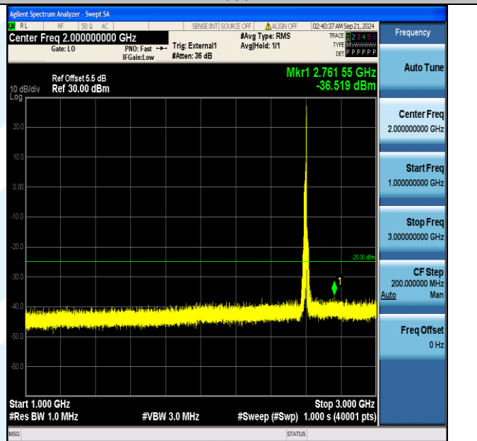
Band38_15MHz_QPSK_38000_1RB#74_1000~3000_1000~3000
