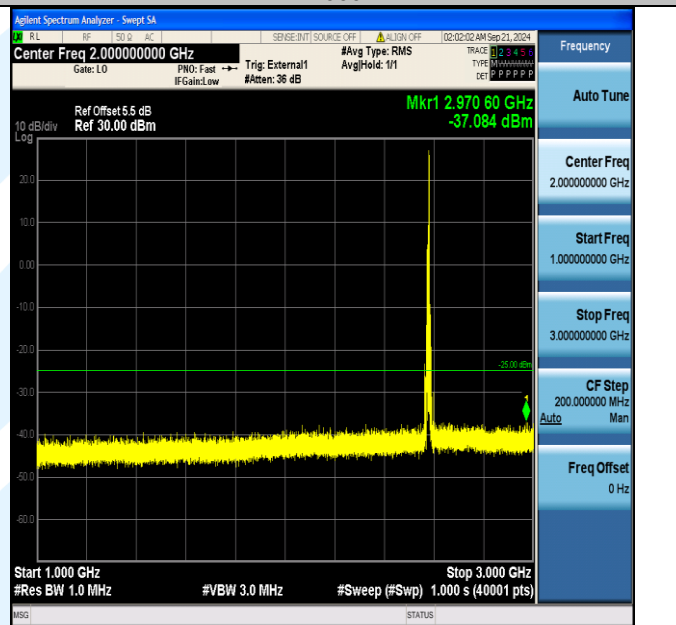
Band38_10MHz_16QAM_37800_1RB#49_1000~3000_1000~3000
