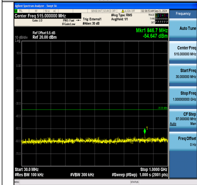
Band38_15MHz_QPSK_38000_1RB#0_30~1000_30~1000
