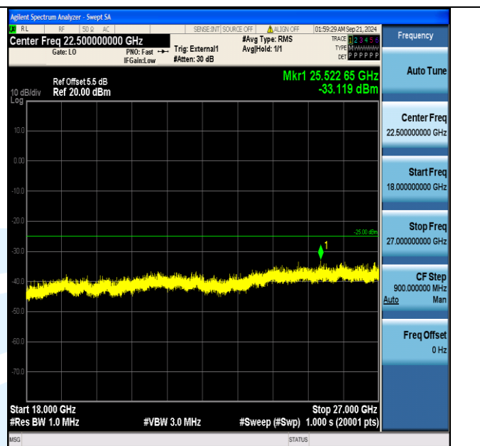
Band38_10MHz_16QAM_37800_1RB#0_18000~27000_18000~27000
