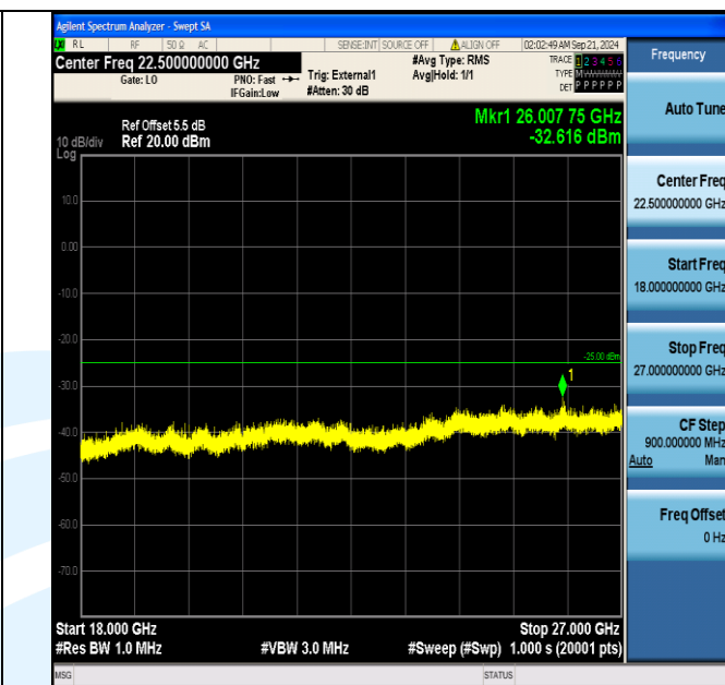
Band38_10MHz_16QAM_37800_1RB#49_18000~27000_18000~27000
