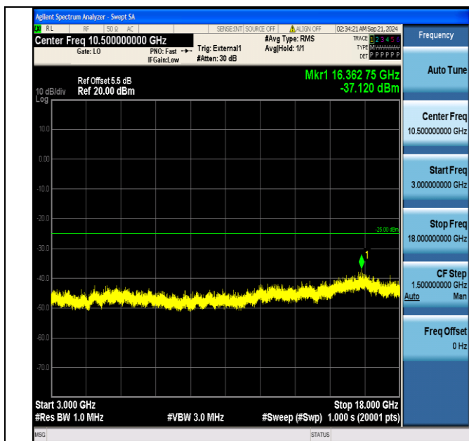
Band38_15MHz_QPSK_37825_75RB#0_3000~18000_3000~18000
