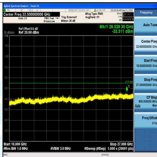
Band38_15MHz_QPSK_37825_1RB#0_18000~27000_18000~27000
