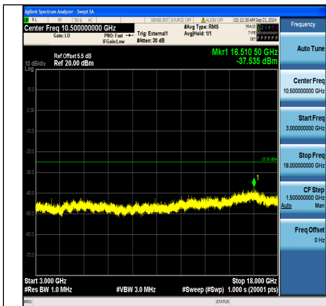
Band38_10MHz_16QAM_38000_1RB#49_3000~18000_3000~18000
