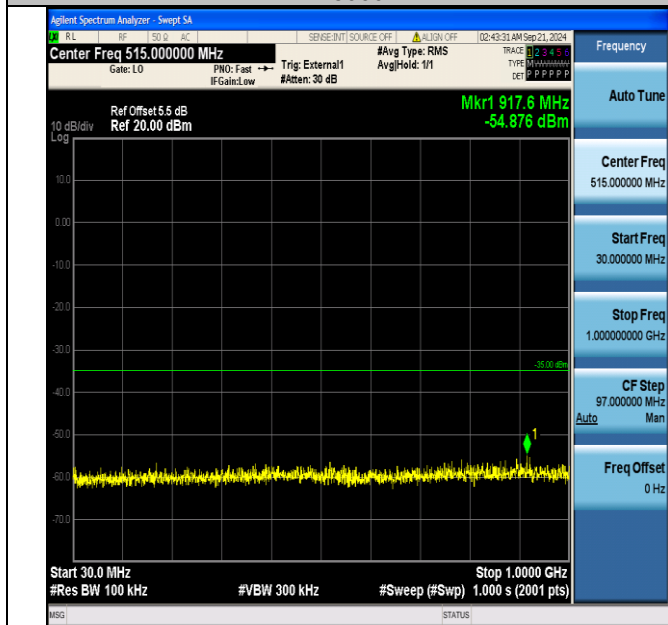
Band38_15MHz_QPSK_38000_75RB#0_30~1000_30~1000
