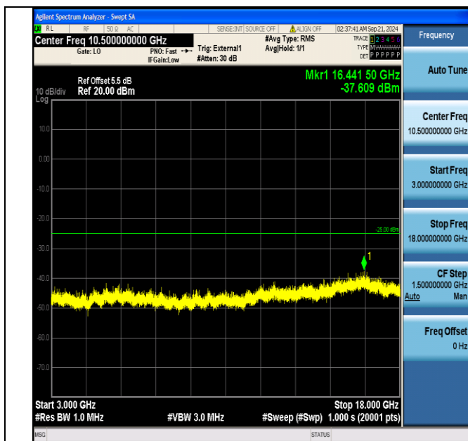
Band38_15MHz_QPSK_38000_1RB#0_3000~18000_3000~18000
