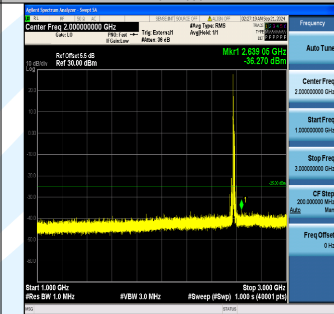
Band38_15MHz_QPSK_37825_1RB#0_1000~3000_1000~3000
