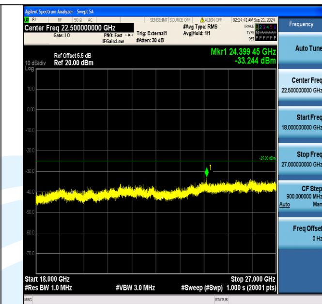
Band38_10MHz_QPSK_38200_50RB#0_18000~27000_18000~27000
