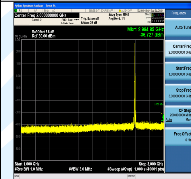
Band38_10MHz_16QAM_38000_1RB#0_1000~3000_1000~3000
