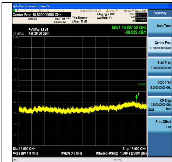
Band38_15MHz_QPSK_38000_1RB#74_3000~18000_3000~18000
