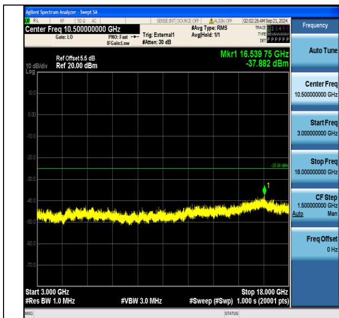
Band38_10MHz_16QAM_37800_1RB#49_3000~18000_3000~18000
