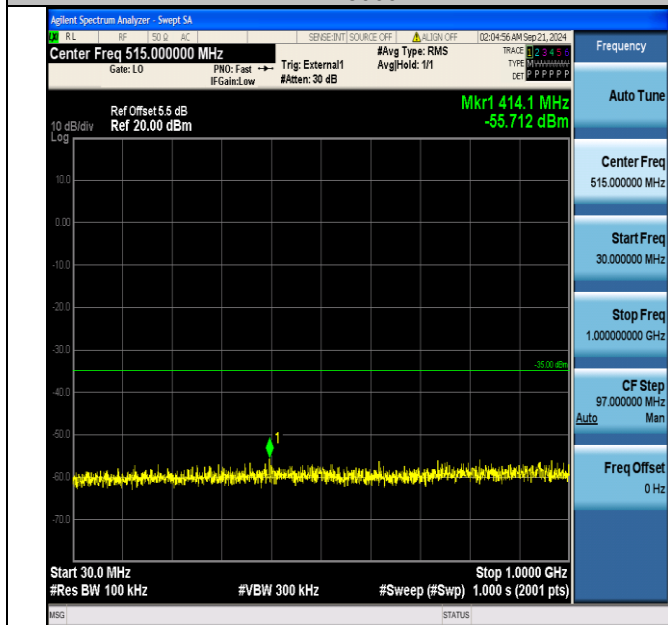
Band38_10MHz_16QAM_37800_50RB#0_30~1000_30~1000
