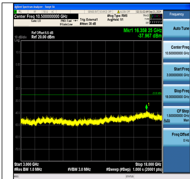
Band38_15MHz_QPSK_37825_1RB#74_3000~18000_3000~18000
