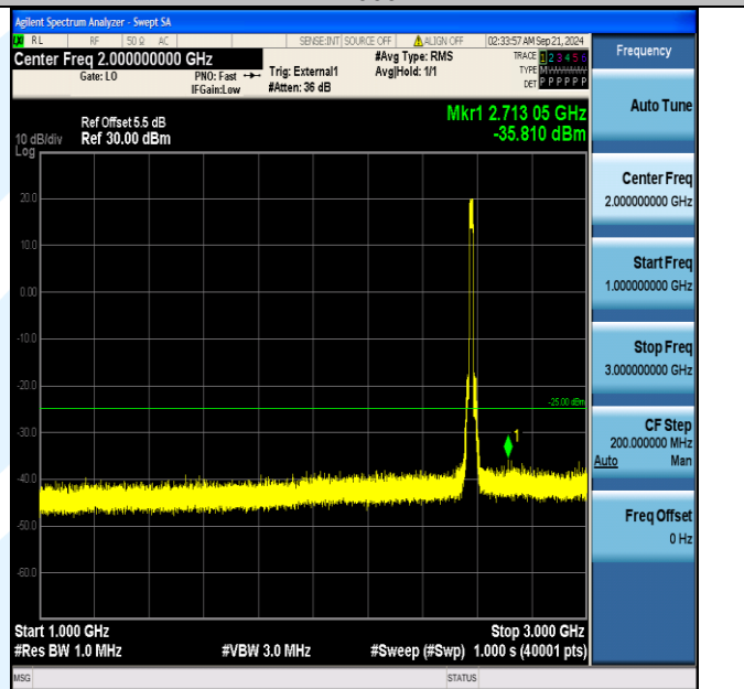
Band38_15MHz_QPSK_37825_75RB#0_1000~3000_1000~3000
