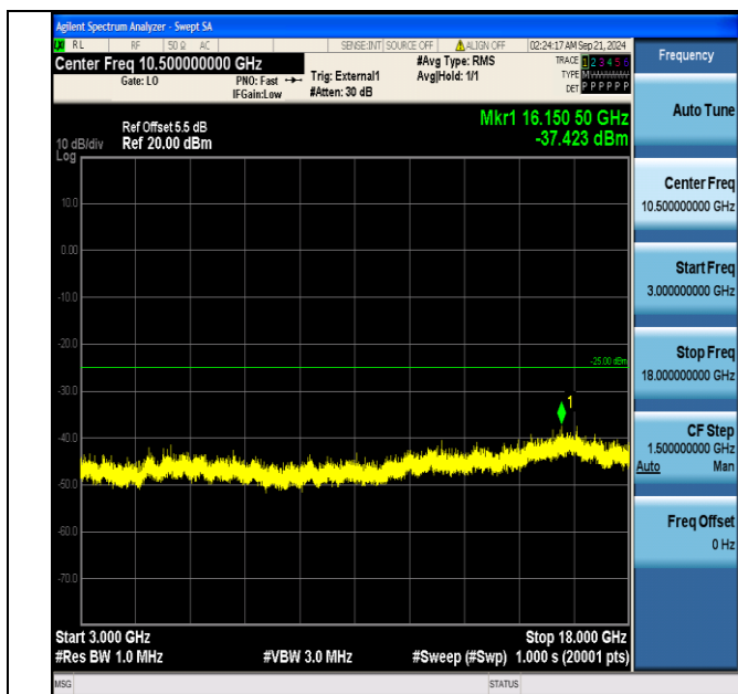
Band38_10MHz_QPSK_38200_50RB#0_3000~18000_3000~18000
