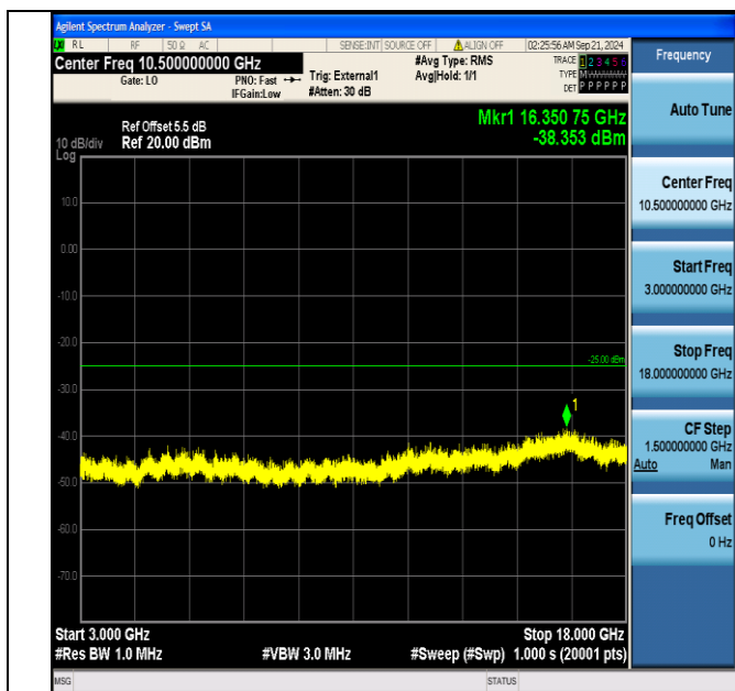
Band38_10MHz_16QAM_38200_50RB#0_3000~18000_3000~18000
