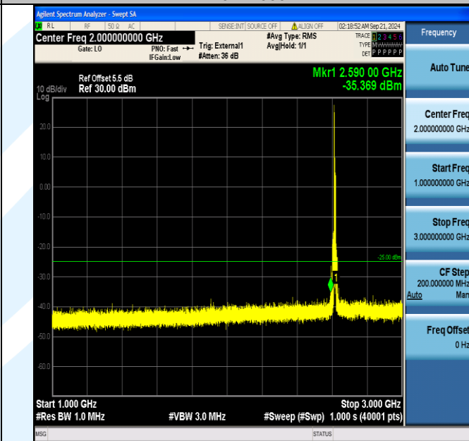
Band38_10MHz_16QAM_38200_1RB#0_1000~3000_1000~3000
