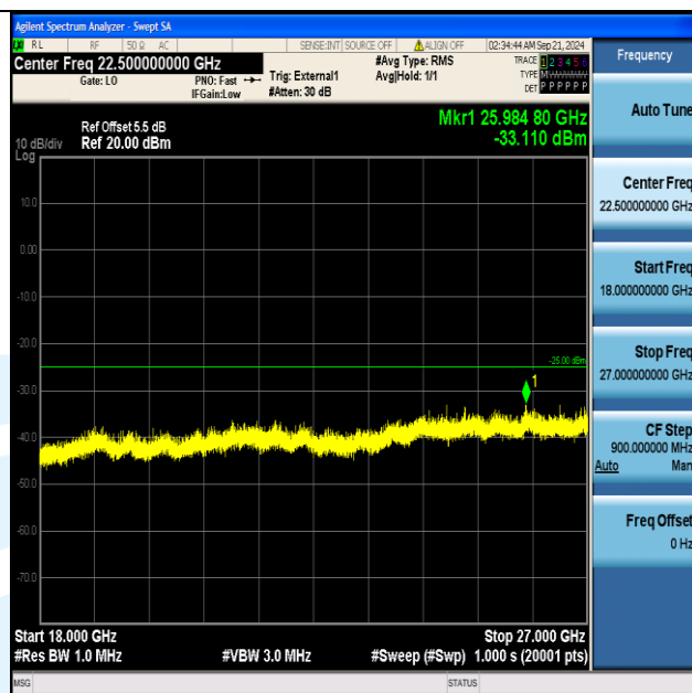
Band38_15MHz_QPSK_37825_75RB#0_18000~27000_18000~27000
