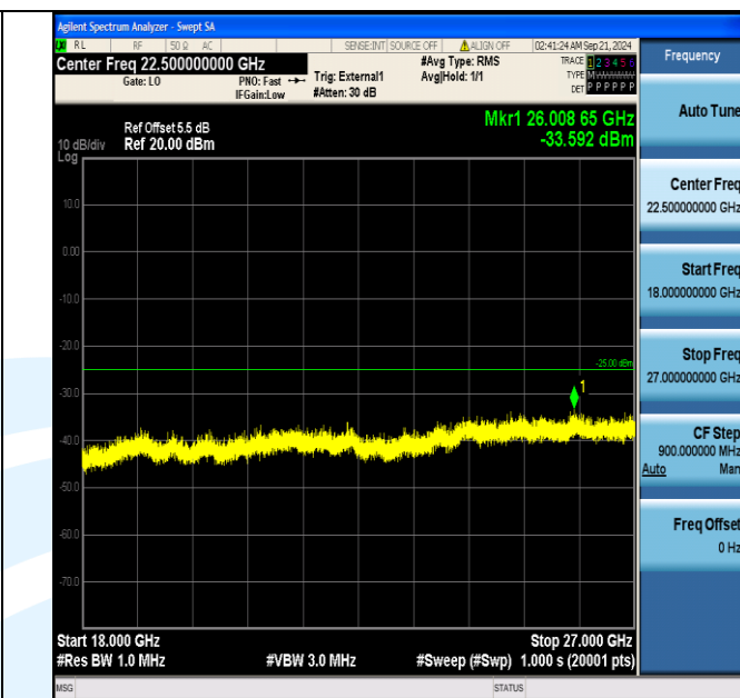
Band38_15MHz_QPSK_38000_1RB#74_18000~27000_18000~27000
